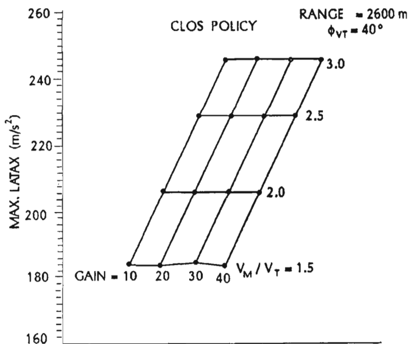
Figure B-3. Effect of V_M/V_T and gain on maximum latax
