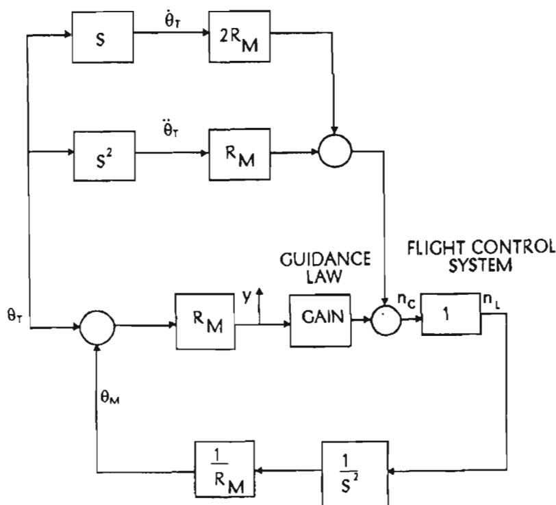
Figure 4-5. Command to line-of-sight guidance system
