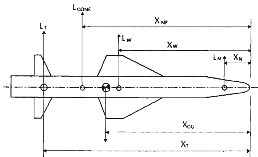
Figure 6-1. System model for the configuration
