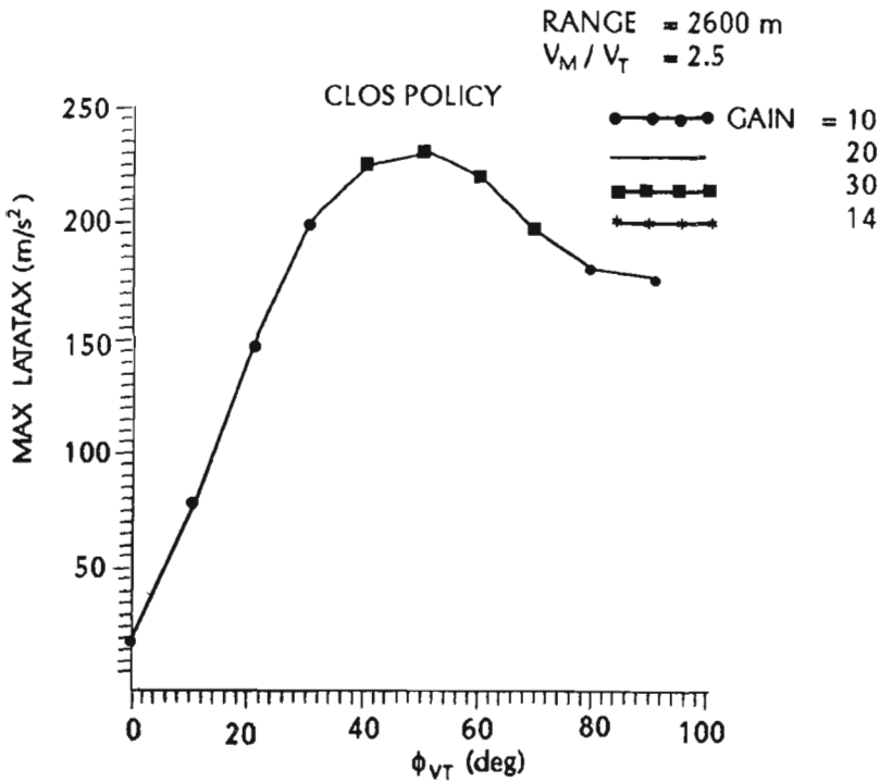
Figure B-1. Effect of \Phi_{VT} and gain on maximum latax
