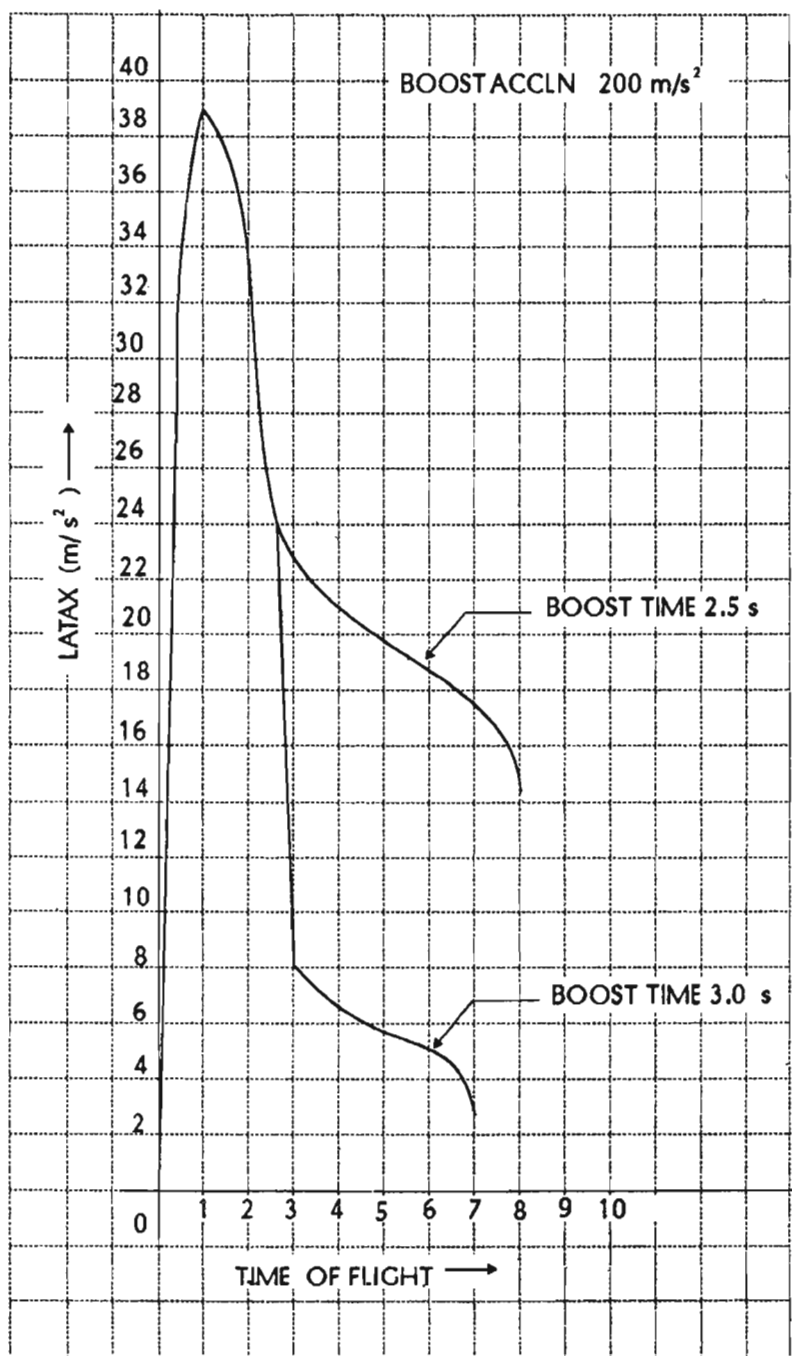
Figure C-5. History of lateral acceleration in boost-sustained trajectory
