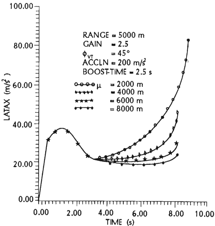
Figure C-6. Effect of \mu on latax history
