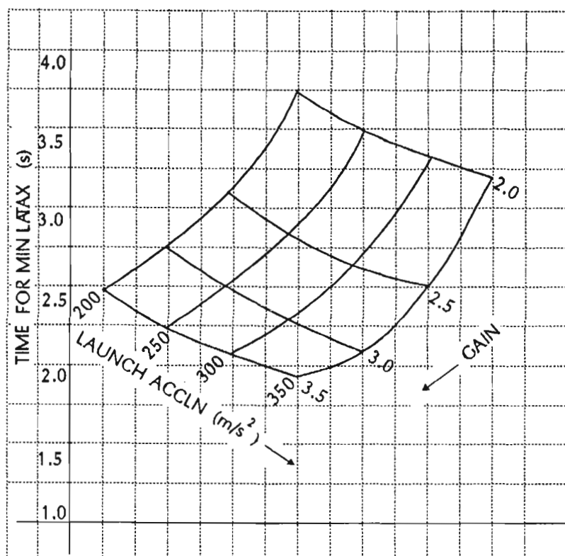
Figure C-4. Effect of gain and launch acceleration, on boosting time for minimum latax
