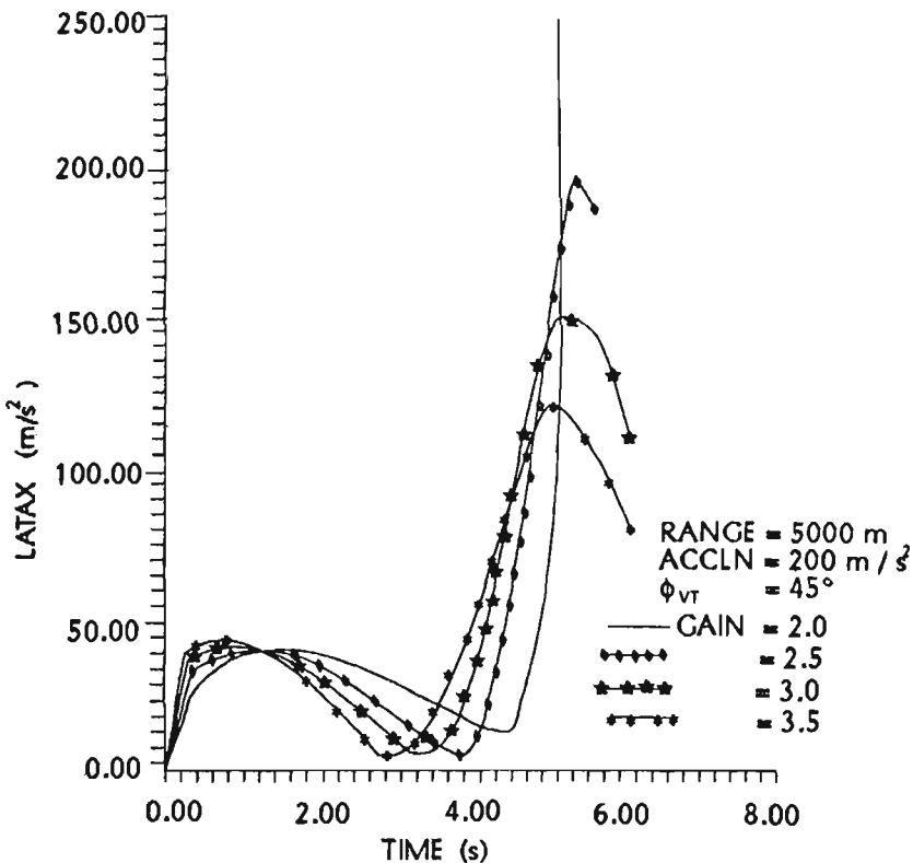
Figure C-2. Effect of guidance gain on latax history
