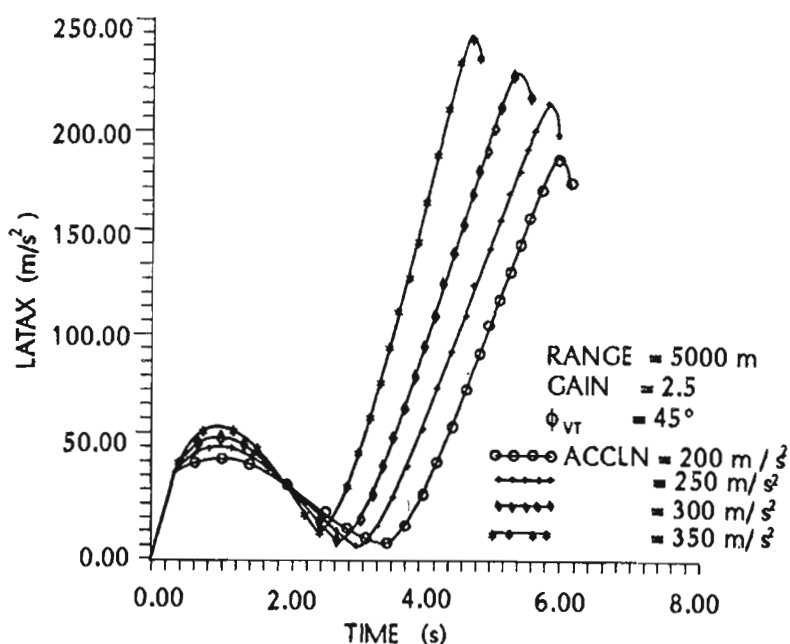
Figure C-3. Effect of longitudinal acceleration on latak history
