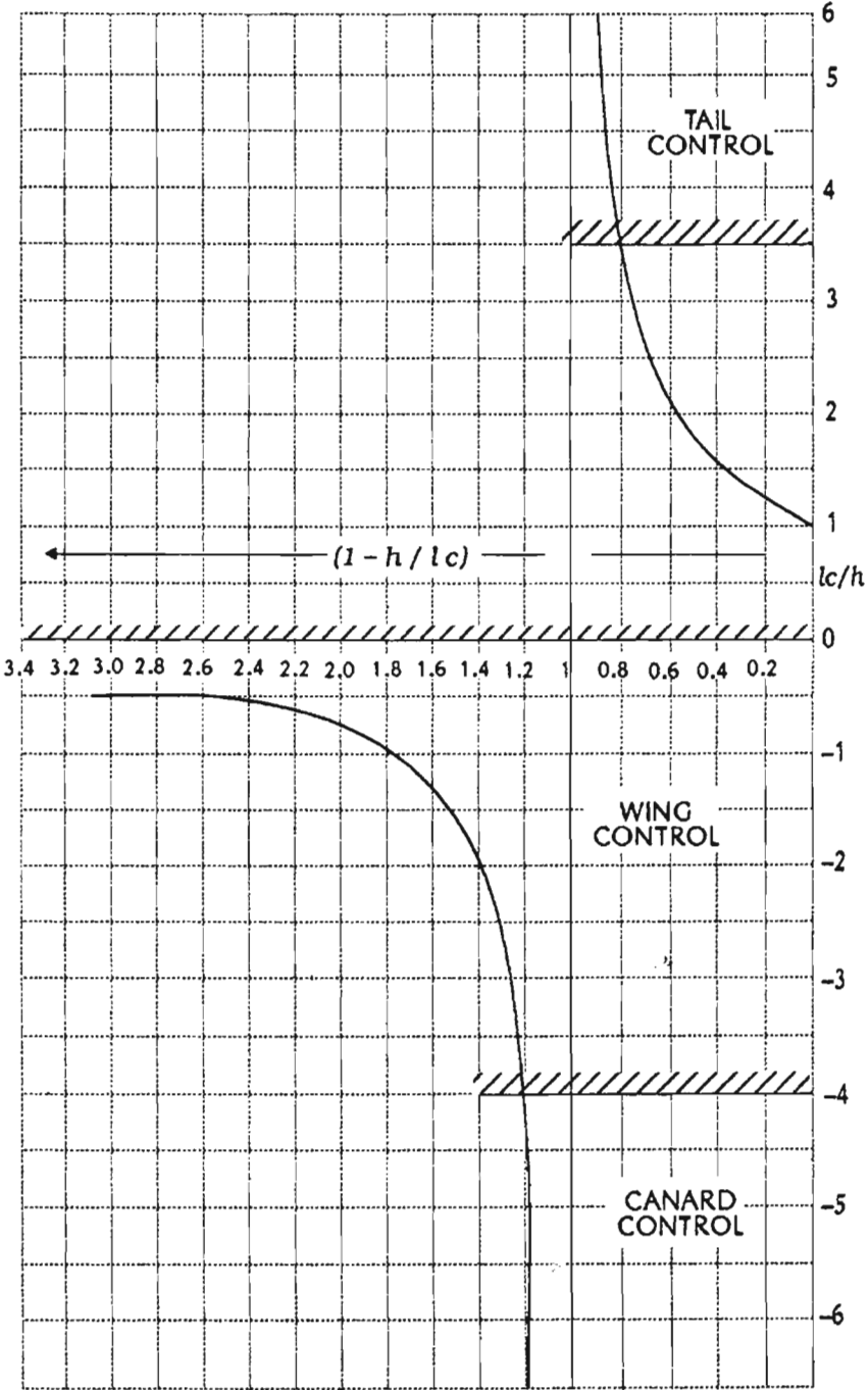
Figure 6-4. Control effectiveness as a function of (l_c/h)
