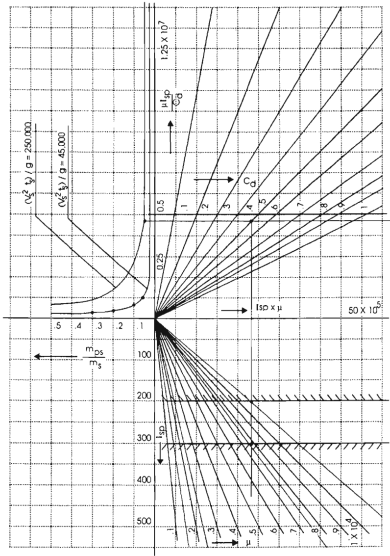
Figure 7-1. Nomogram for propulsion system design
