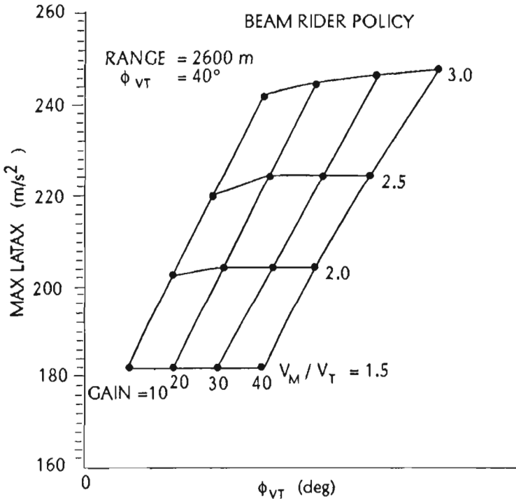
Figure A-4. Effect of V_M/V_T and gain on maximum latax
