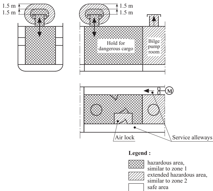
Fig. 17.2 Examples for service alleyways, lockable with door and air lock to the hold
