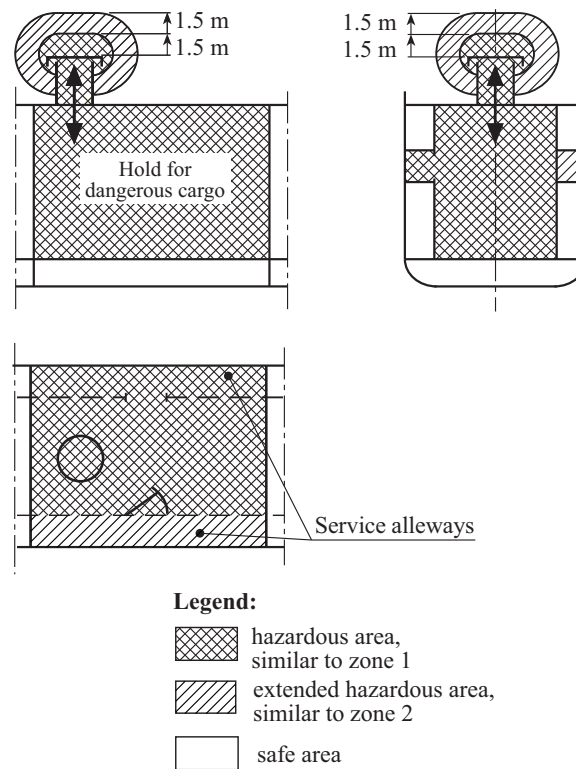
Fig. 17.1 Examples for service alleyways, open to the hold and lockable with door
