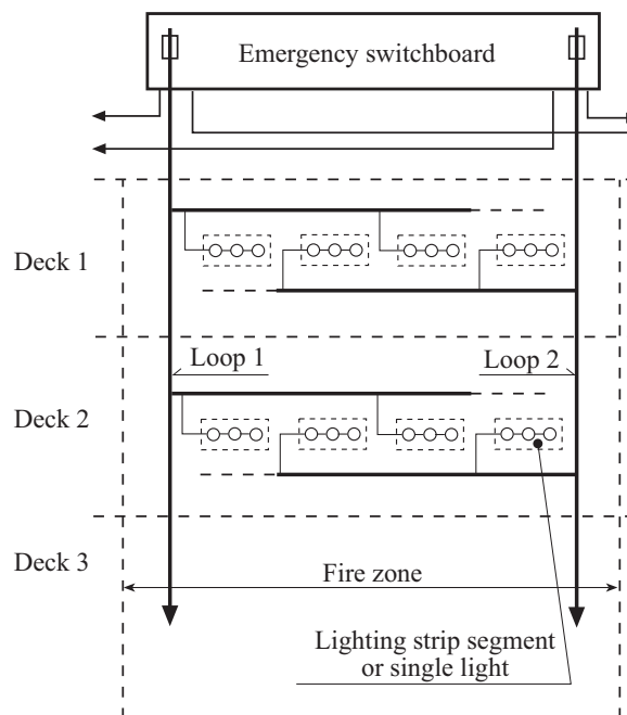
Fig. 14.1 Specimen of supply layout-low-location lighting
