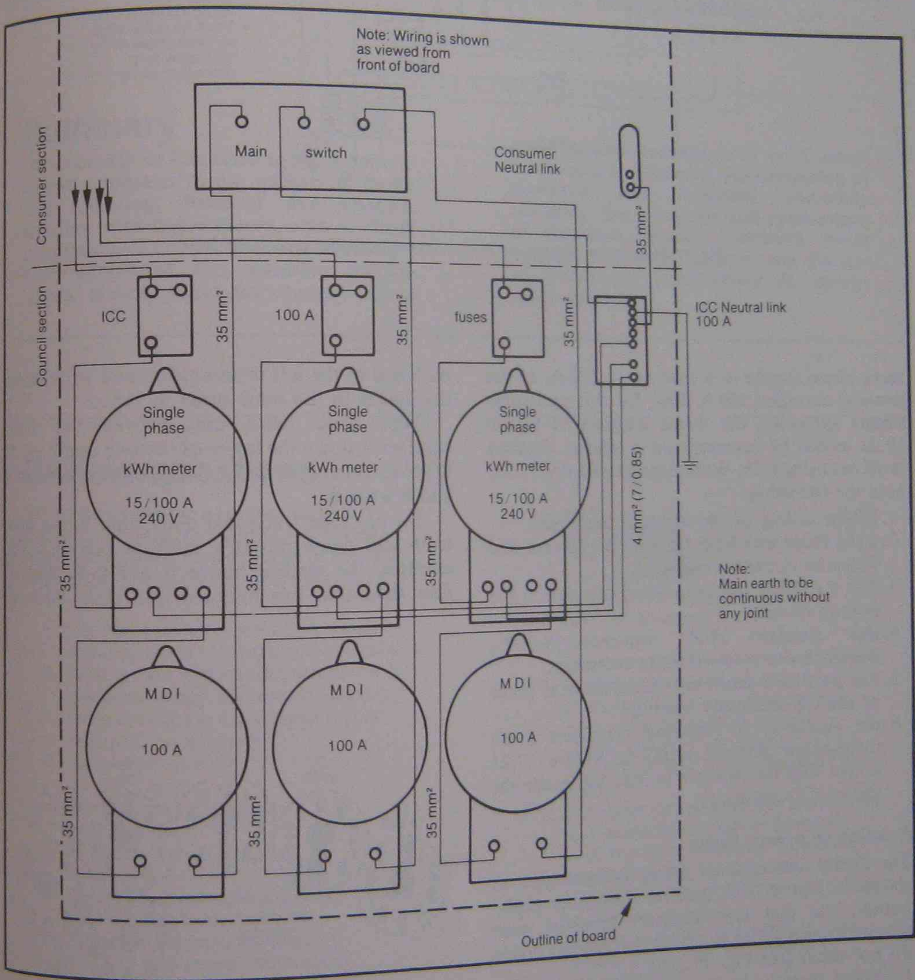
Fig. 17.21 Metering diagram for three-phase supply with MDI. 100 A maximum
