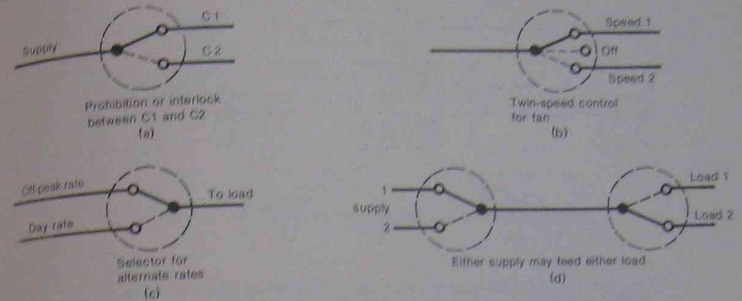
Fig. 7.15 Some other applications of two-way switches
