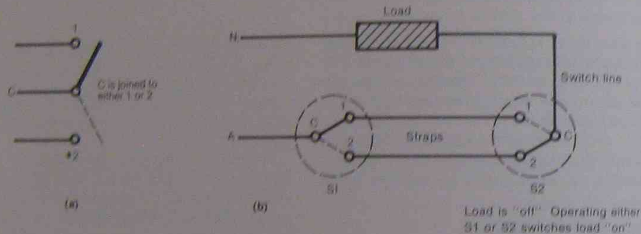
Fig. 7.12 Two-way switching
