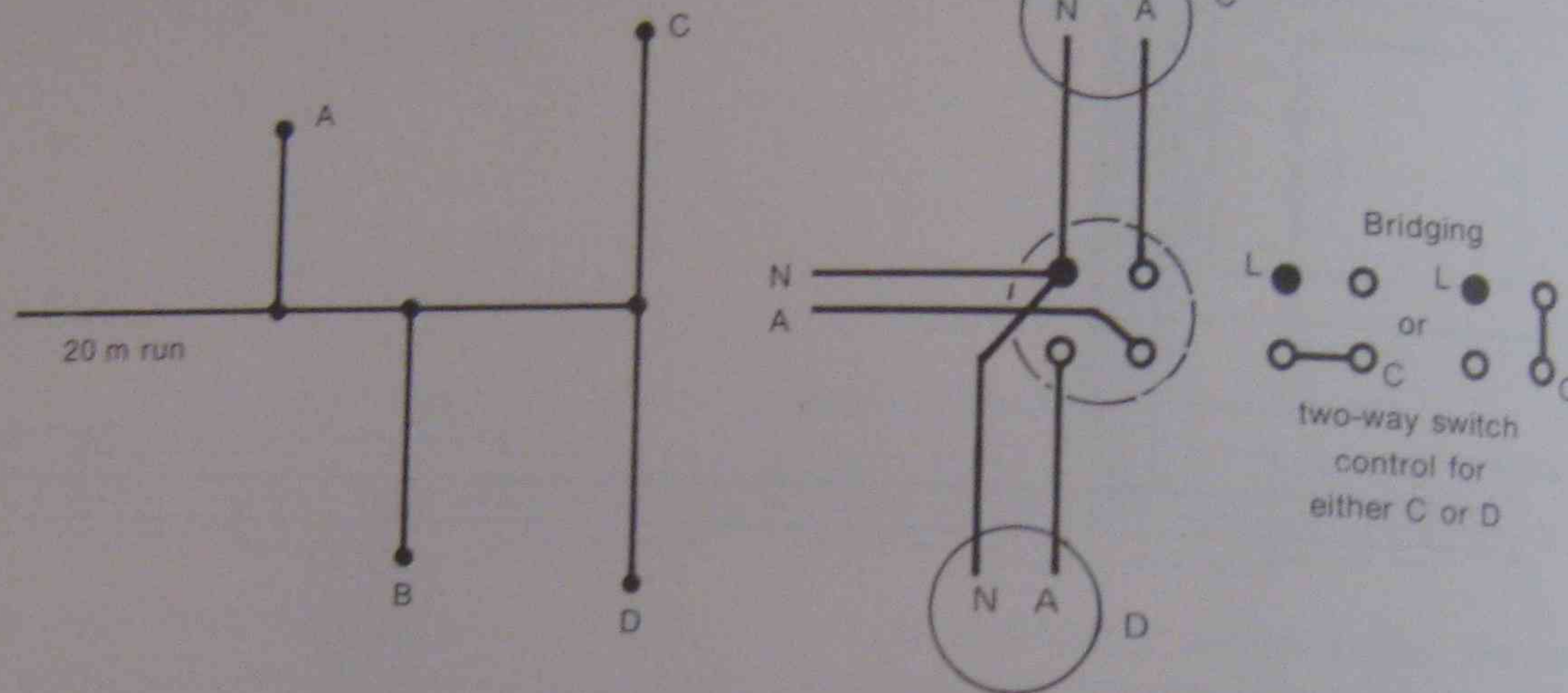
Fig. 7.27 An additional power outlet installed at D has not increased the effective number of points on this circuit by virtue of the two-way switching provided
