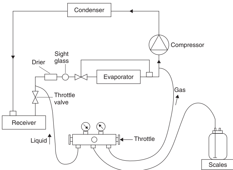
Figure 11.3 Charging connection
