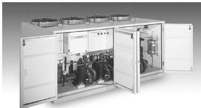
Figure 13.6 Scroll compressor pack within rooftop condenser (Hubbard)
