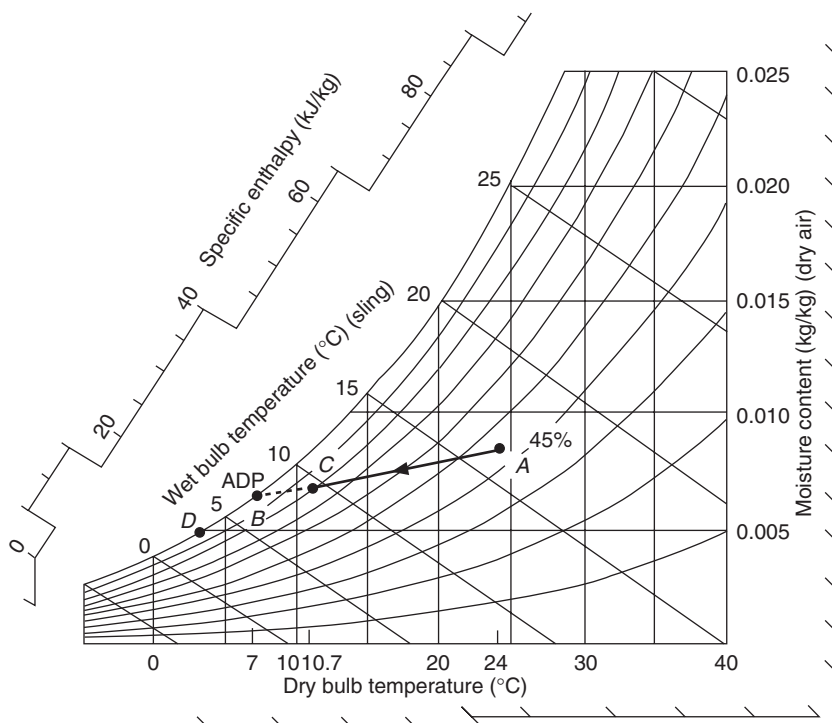
Figure 21.9 Cooling and dehumidifying coil – process line
