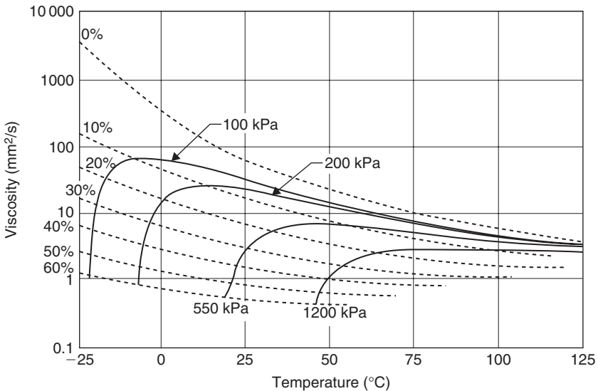
Figure 5.3 Viscosity/temperature/pressure diagram: shows percentage refrigerant in solution and corresponding viscosity.
