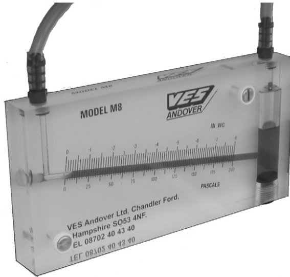
Figure 24.2 Inclined manometer (Business Edge)
