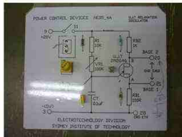
Page 131 UJT Relaxation Oscillator
