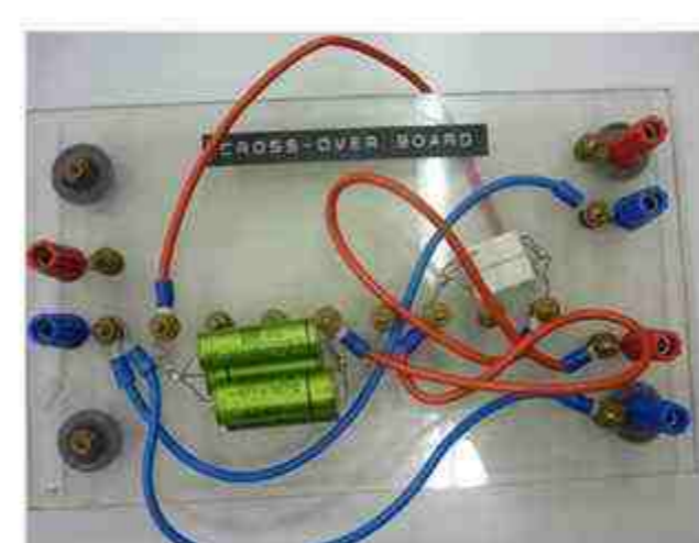
Page 179 Cross over board
