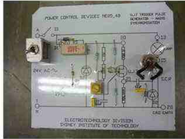
Page 146 Trigger pulse generator main synchronization
