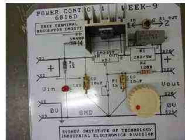
Page 137 Three terminals regulator
