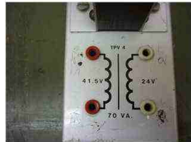
Page 275 Single phase transformer 41.5/24V
