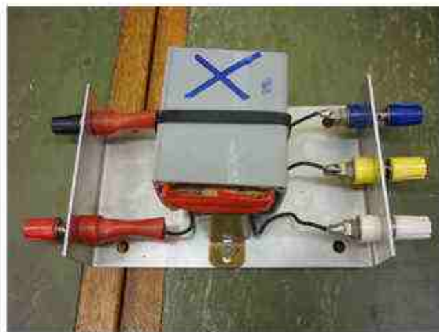
Page 270 Single phase transformer 240/24V
