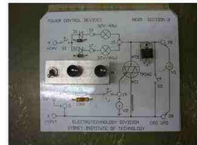
Page 134 SCR Power Control device
