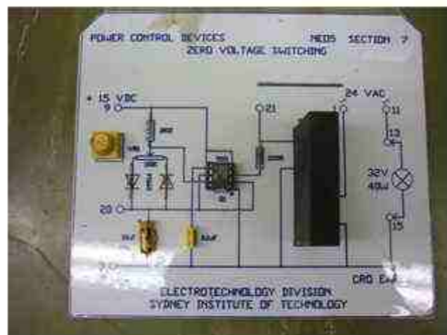
Page 140 Zero voltage switching
