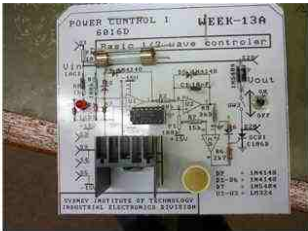
Page 152 1/2 wave regulator
