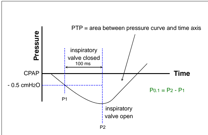
Figure 5-13. Calculation of P_{0.1} on the Drager Evita 4 ventilator. PTP = pressure-time product.
