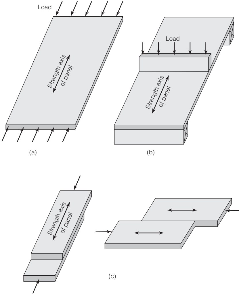
FIGURE 10.20 Load orientation conditions for determining mechanical properties of plywood: (a) axial, (b) bending, and (c) shear.
