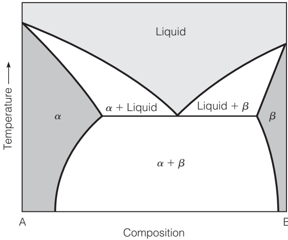
FIGURE 2.16 Binary phase diagram, partially soluble material.
