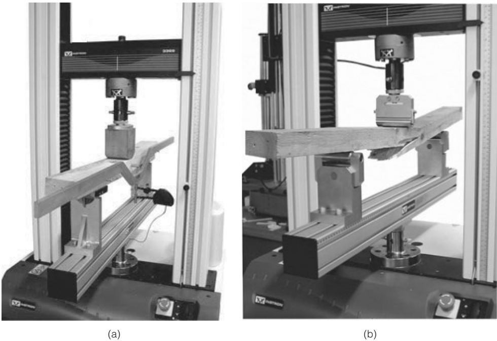
FIGURE A.66 Center-point loading on 4 \times 4 wood beam: (a) before loading, and (b) after failure.
