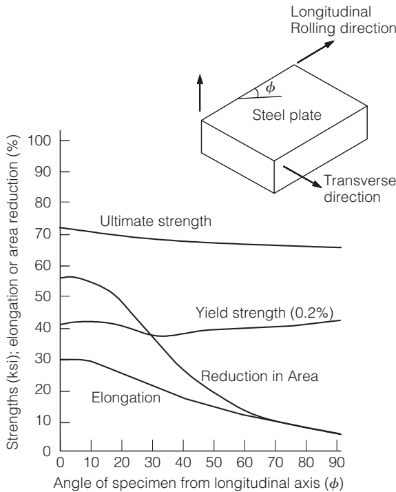
FIGURE 3.19 Example of effect of specimen orientation on measured tensile properties of steel.
