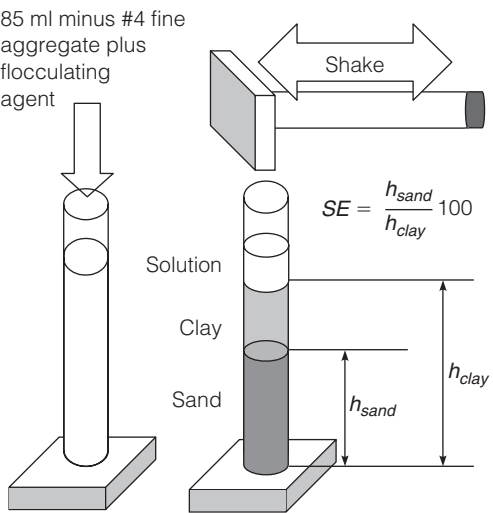
FIGURE 5.17 Concept of sand equivalency test.
