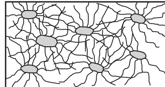
FIGURE 6.4 Development of structure in the cement paste: (a) initial C-S-H phase, (b) forming of gels, (c) initial set—development of weak skeleton, (d) final set—development of rigid skeleton, (e) hardening. (Hover and Phillco, 1990)
