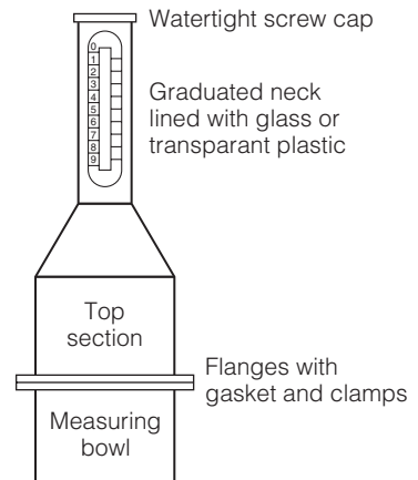
FIGURE 7.13 Volumetric method (Roll-A-Meter) apparatus for determining air voids in fresh concrete (Reprinted, with permission, from ASTM C173, Figure 1, copyright ASTM International, 100 Barr Harbor Drive, West Conshohocken, PA 19428.)
