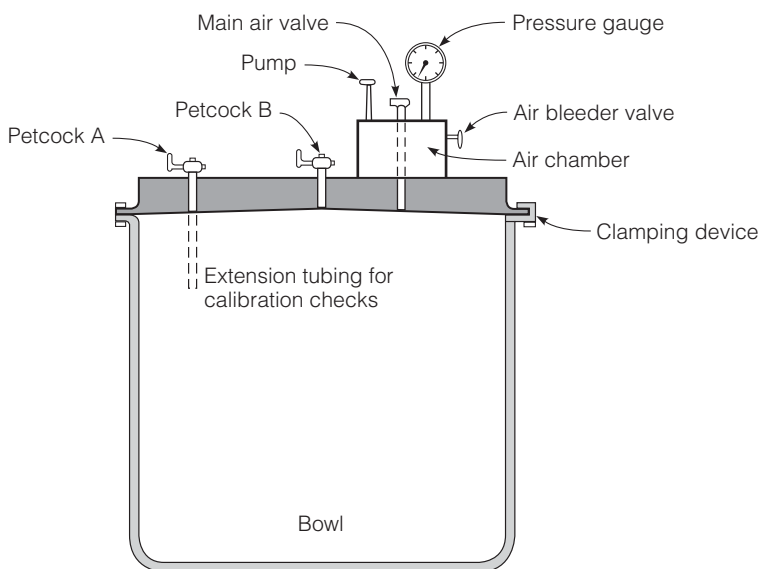
FIGURE 7.12 Pressure method apparatus for determining air voids in fresh concrete—Type B Meter (Reprinted, with permission, from ASTM C231, Figure 2, copyright ASTM International, 100 Barr Harbor Drive, West Conshohocken, PA 19428.)
