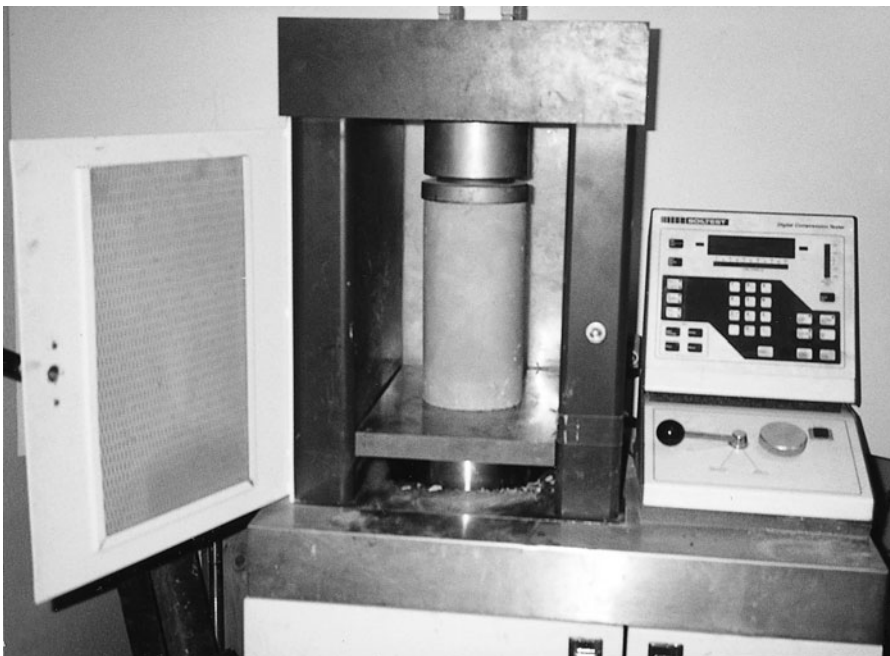
FIGURE A.38 Concrete cylindrical specimen being tested for compressive strength.
