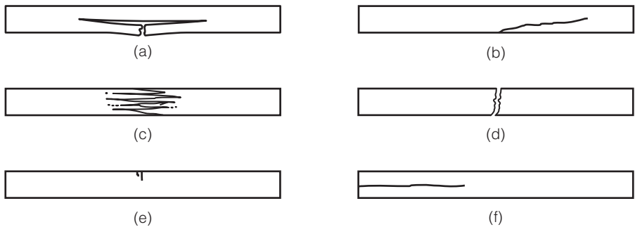
FIGURE A.69 Types of failure in static bending: (a) simple tension (side view), (b) cross-grain tension (side view), (c) splintering tension (view of tension surface), (d) brash tension (view of tension surface), (e) compression (side view), and (f) horizontal shear (side view).
