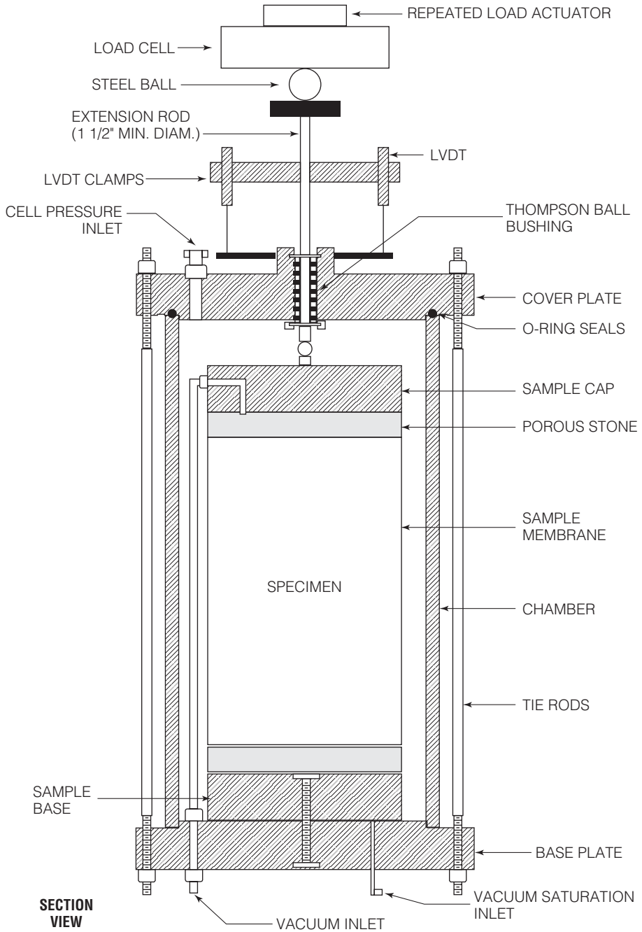
FIGURE 5.11 Triaxial chamber with external LVDTs and load cell.
