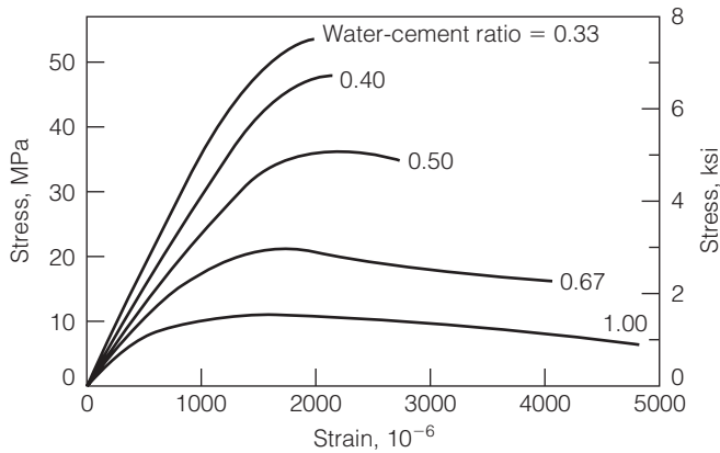
FIGURE 7.32 Typical stress-strain relations for compressive tests on 0.15 \times 0.30 -m concrete cylinders at an age of 28 days.
