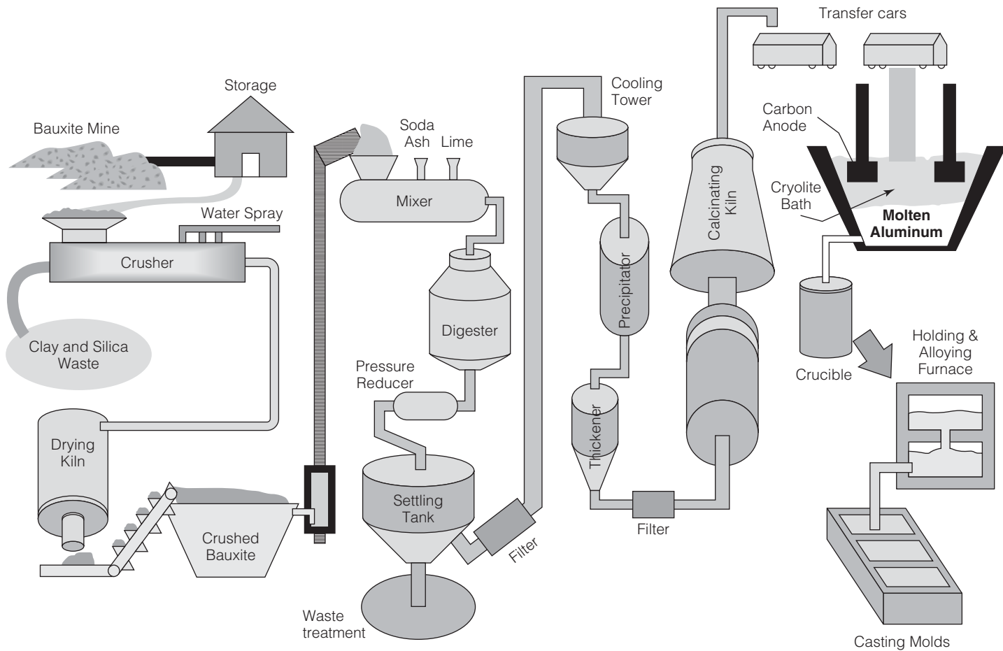
FIGURE 4.3 Aluminum production process.
