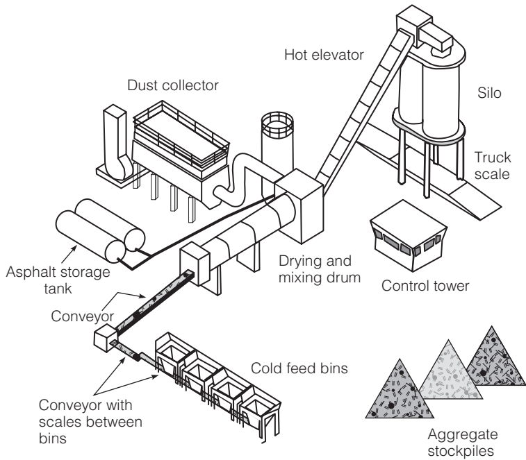
FIGURE 9.40 Drum asphalt mixing plant.
