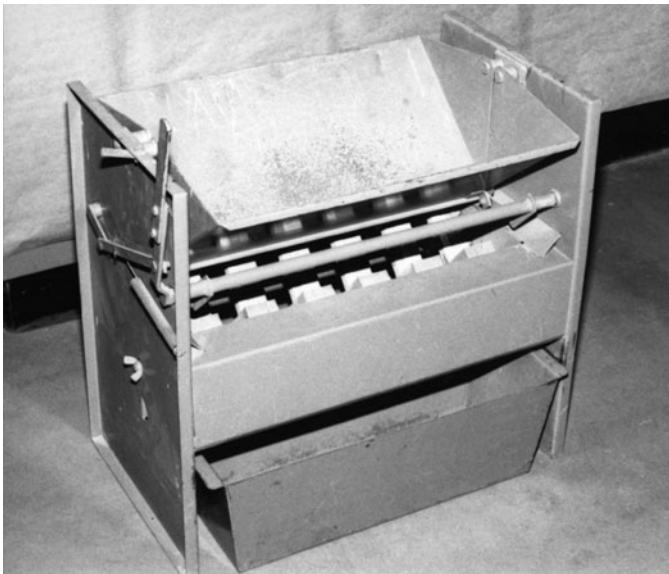
FIGURE 5.21 Aggregate sample splitter.
