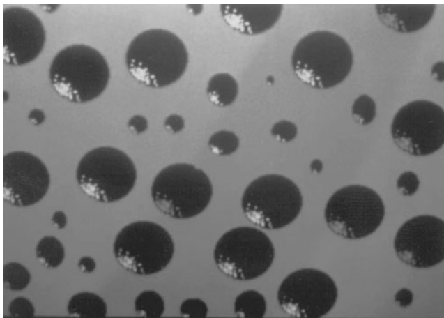
FIGURE 9.4 Photo of magnified asphalt emulsion showing minute droplets of asphalt cement dispersed in a water medium.
