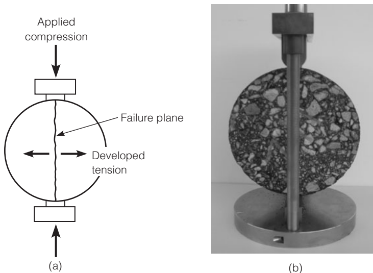
FIGURE 9.33 Split tension and diametral testing (a) schematic of split tension test; (b) sample prepared for diametral tensile resilient modulus test.
