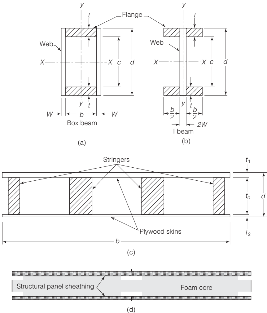
FIGURE 10.24 Composite structural members.
