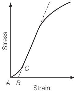
FIGURE 1.25 Correction of toe region in stress–strain curve.
