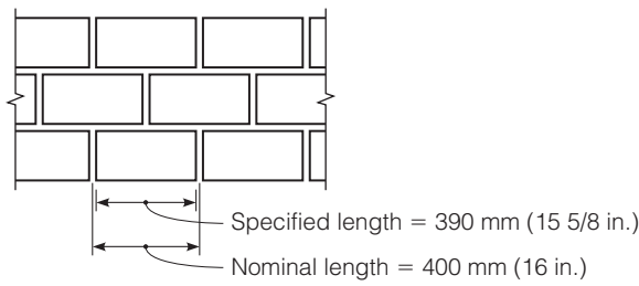
FIGURE 8.3 Nominal dimensions and specified (modular) dimensions.
