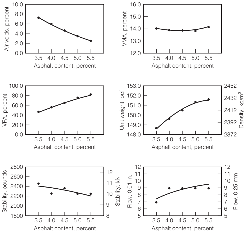
FIGURE 9.31 Graphs used for Marshall mix design analysis (The Asphalt Institute, 2001). (See Table 9.13)
