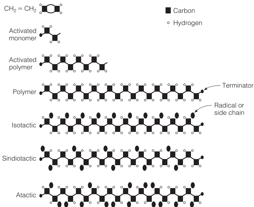
FIGURE 2.21 Polymer structures.
