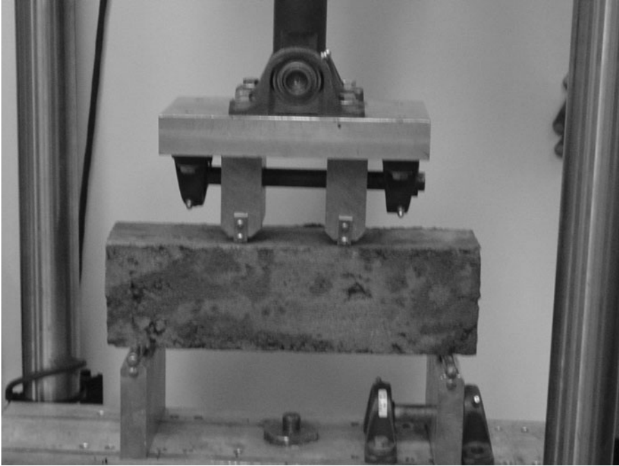
FIGURE A.42 Testing concrete beam in the flexure testing machine.
