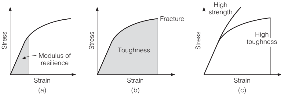
FIGURE 1.15 Areas under stress–strain curves: (a) modulus of resilience, (b) toughness, and (c) high-strength and high-toughness materials.
