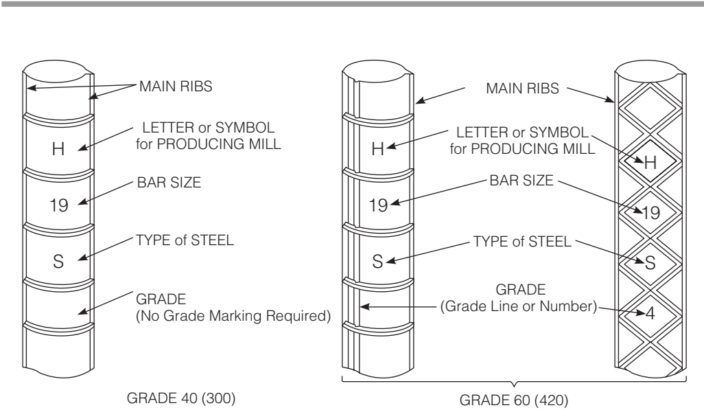
FIGURE 3.14 ASTM reinforcing bar identification codes.
