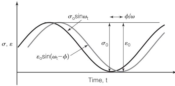
FIGURE 9.36 Stress and strain pulses for the dynamic modulus test.
