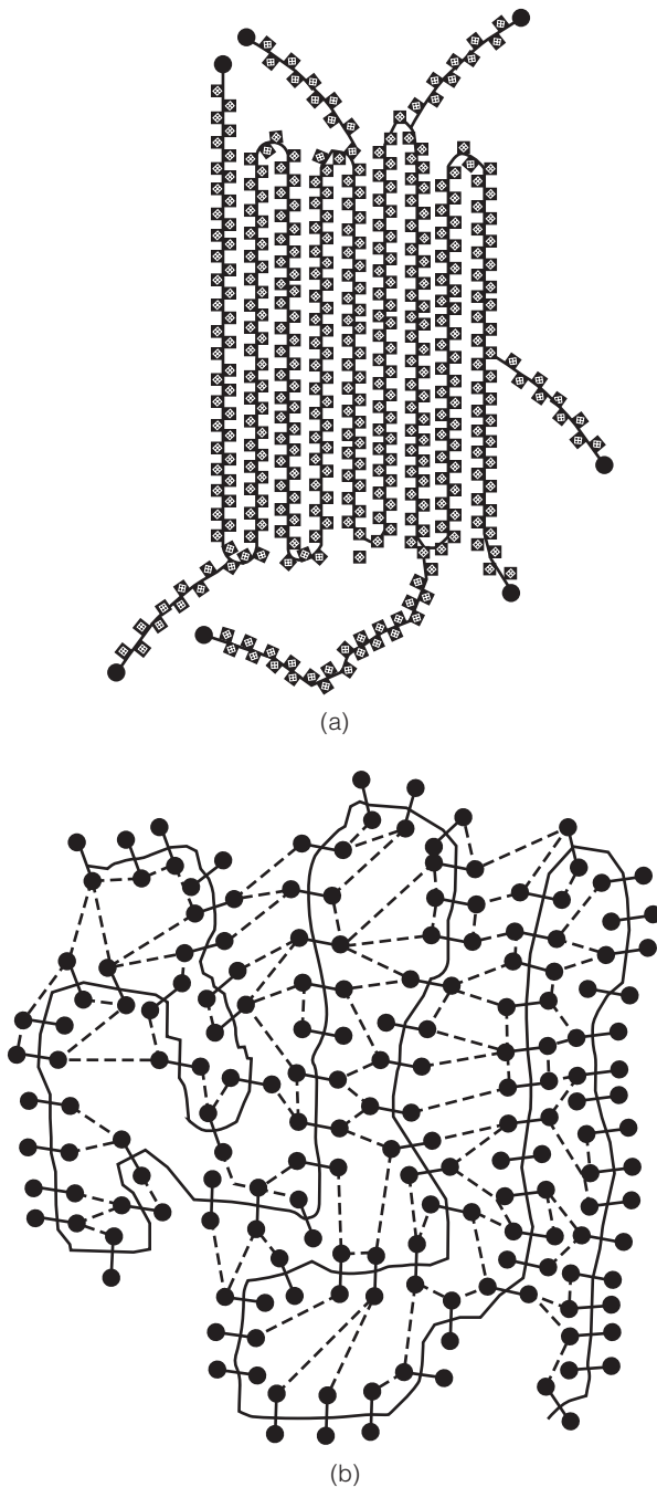
FIGURE 2.22 Polymer chain structures: (a) ordered structure of linear polymer and (b) cross linked structure of linear polygon.
