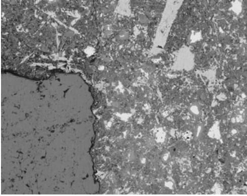
FIGURE 7.34 Scanning electron image showing the interface between a sand grain (lower left corner) and the paste.
