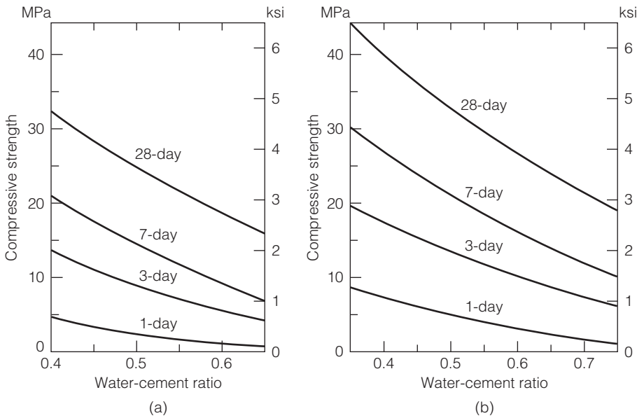
FIGURE 6.8 Typical age-strength relationships of concrete based on compression tests of 0.15 \times 0.30 m ( 6 \times 12 in.) cylinders, using Type I portland cement and moist-curing at 21^{\circ}\text{C} ( 70^{\circ}\text{F} ): (a) air entrained concrete, (b) non-air entrained concrete. (Courtesy of Portland Cement Association)
