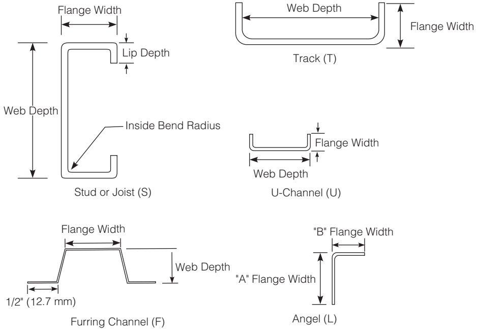
FIGURE 3.11 Generic cold-formed steel framing shapes.
