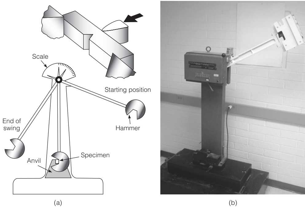
FIGURE 3.23 Charpy V notch impact testing machine (a) schematic and (b) apparatus.
