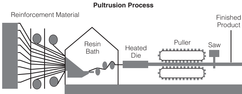
FIGURE 11.5 Pultrusion scheme used in fabricating structural shape fiber-reinforced composites. (Courtesy of Creative Pultrusions, Inc.)
