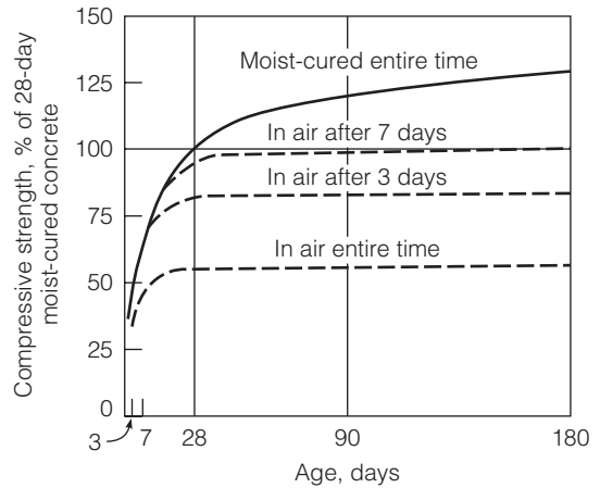
FIGURE 7.22 Compressive strength of concrete at different ages and curing levels.
