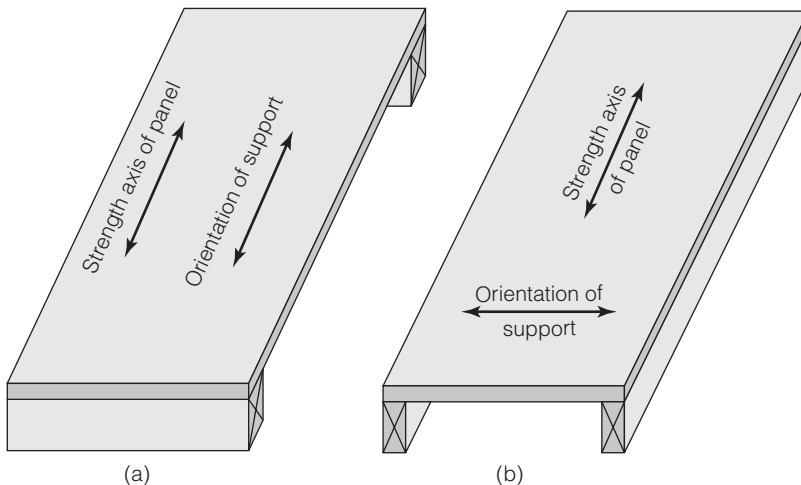
FIGURE 10.19 Typical plywood panel: (a) strength axis parallel to orientation of support and (b) strength axis perpendicular to orientation of support.
