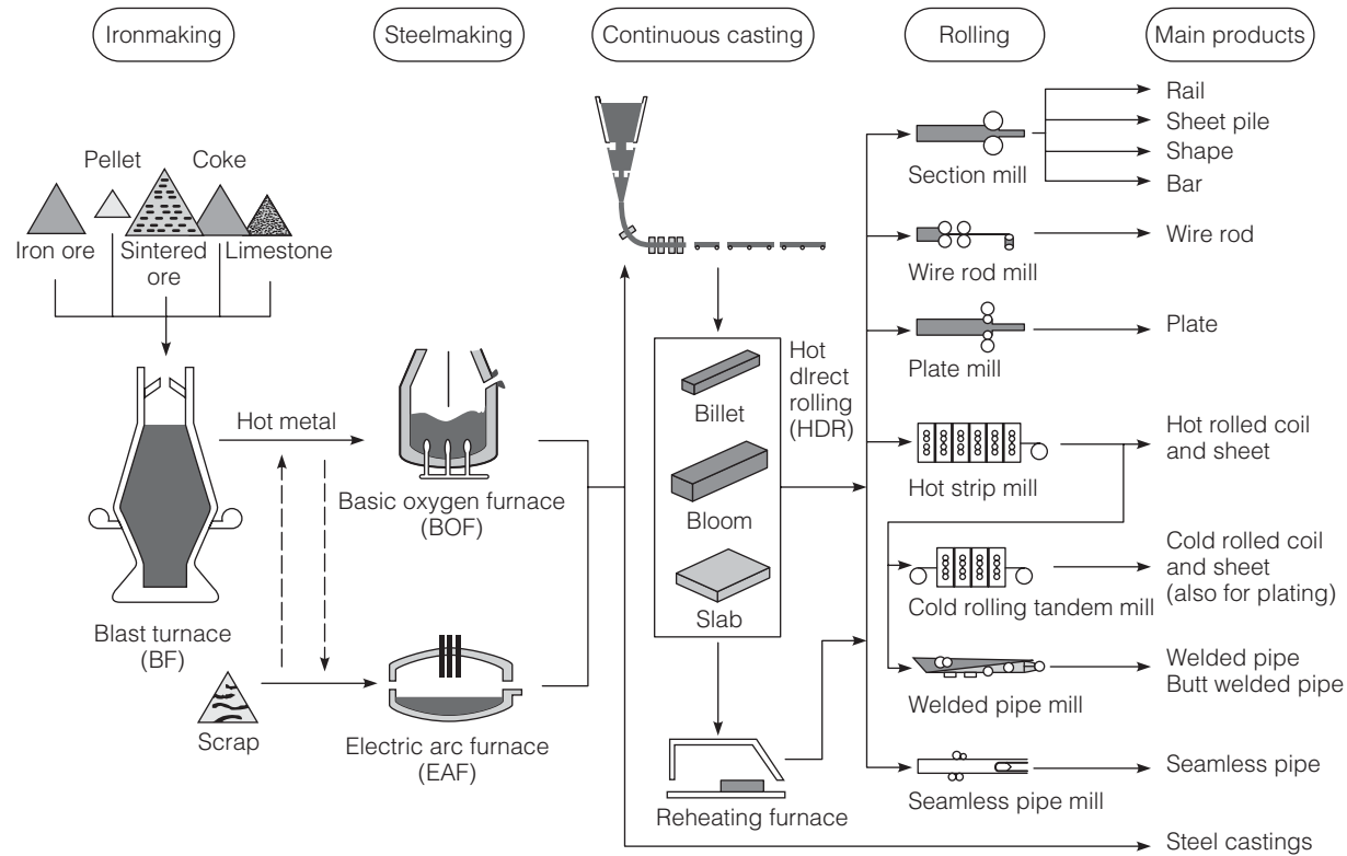
FIGURE 3.3 Conversion of raw material into different steel shapes.
