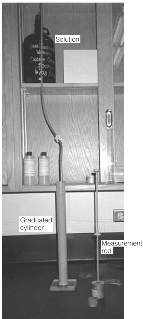
FIGURE 5.18 Sand equivalency test apparatus.
