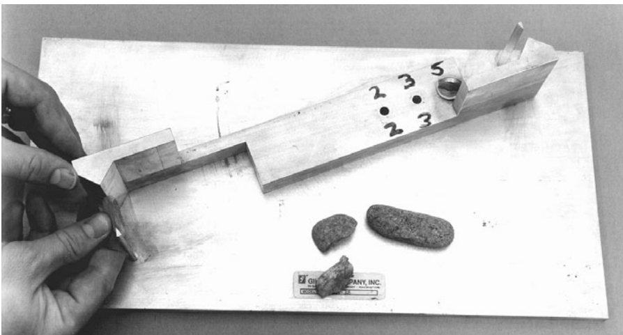
FIGURE 5.6 Superpave flat and elongated apparatus.
