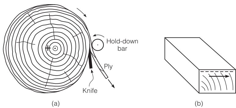
FIGURE 10.17 Cutting of plies for plywood and glulam: (a) rotary cutting and (b) slicing. (© Pearson Education, Inc. Used by permission.)
