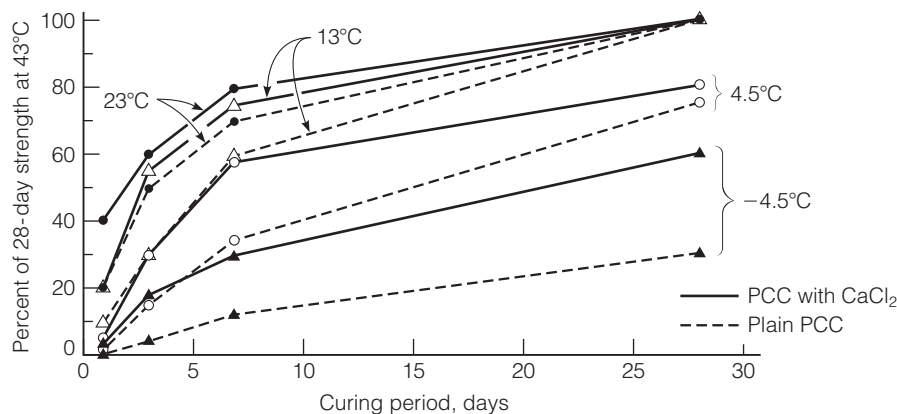
FIGURE 6.11 Effect of \text{CaCl}_2 on strength development at different curing temperatures.
