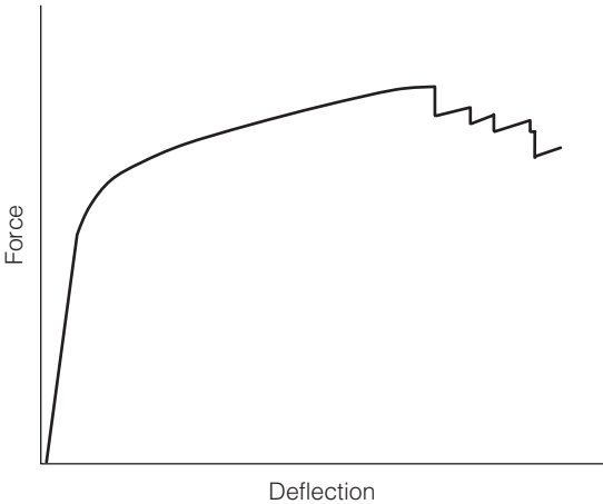
FIGURE A.67 Typical load-deflection plot.
