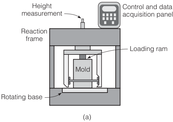
FIGURE 9.26 Superpave gyratory compactor.
