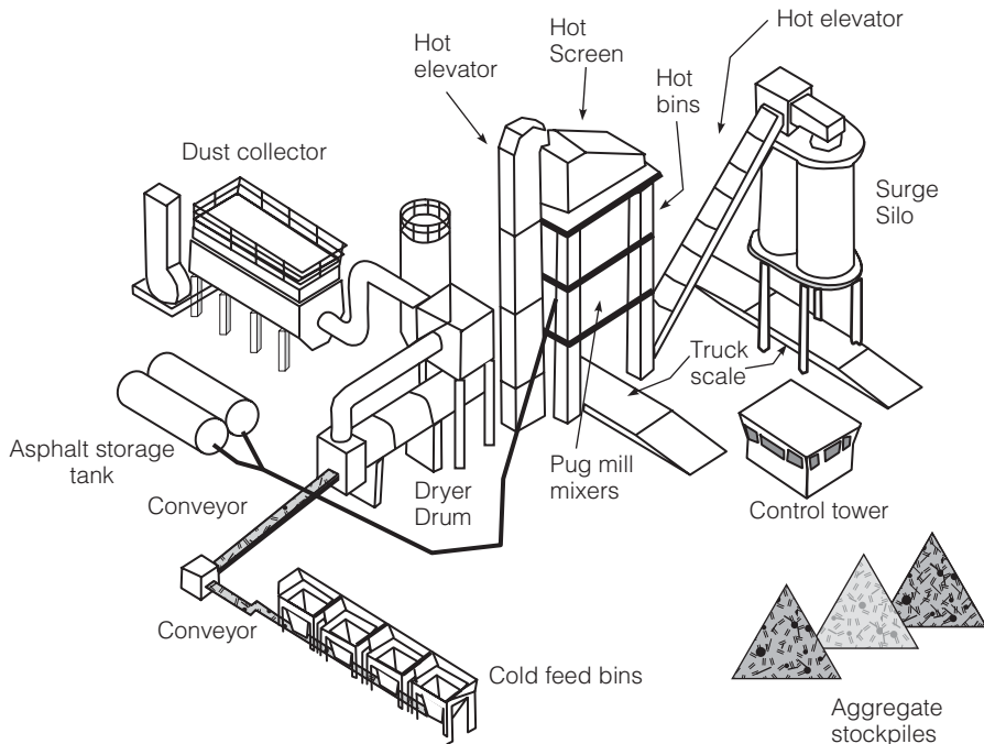
FIGURE 9.39 Batch asphalt mixing plant.
