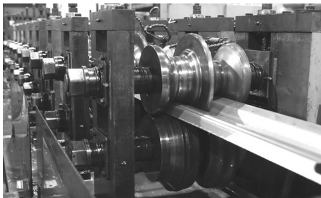
FIGURE 3.10 Roll-forming of cold-formed steel framing member.
