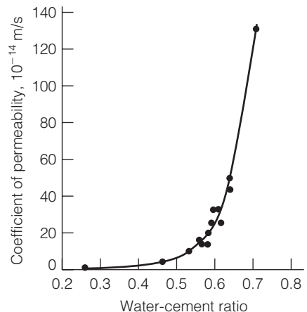
FIGURE 7.31 Relation between water–cement ratio and permeability of mature cement paste.
