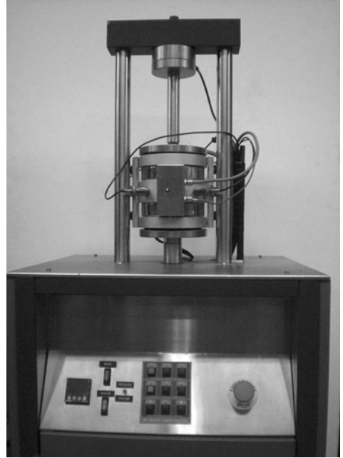
FIGURE 9.35 Asphalt Mixture Performance Tester.
