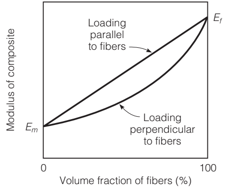
FIGURE 11.15 Modulus of elasticity of the composite versus fiber volume fraction.
