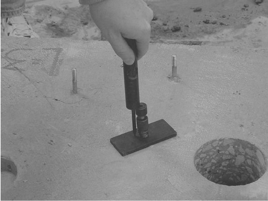
FIGURE A.47 Measuring penetration of one probe.
