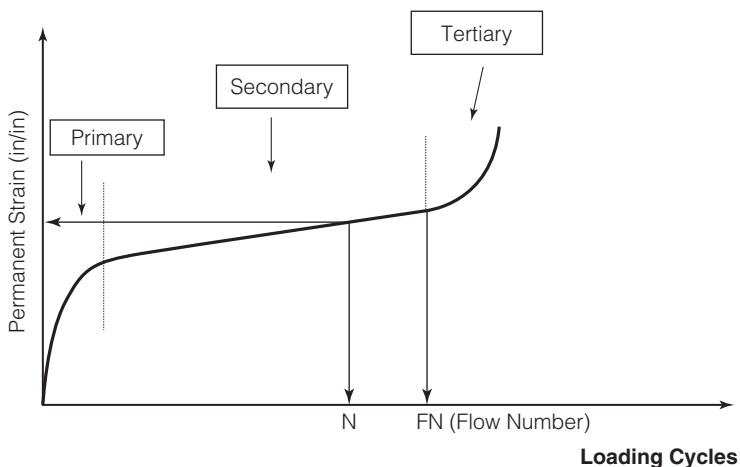
FIGURE 9.38 Typical relationship between total cumulative plastic strain and loading cycles.
