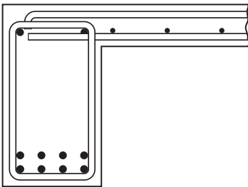
FIGURE 11.13 An example of steel-reinforced concrete beam and slab details.
