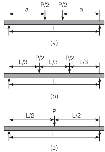
FIGURE 10.15 Methods of loading a wood beam: (a) two-point loading, (b) third-point loading, and (c) center-point loading.
