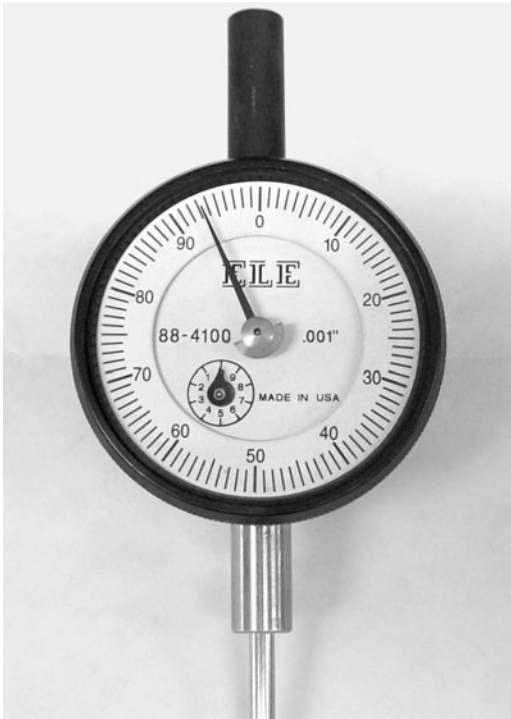
FIGURE 1.26 Dial gauge.
