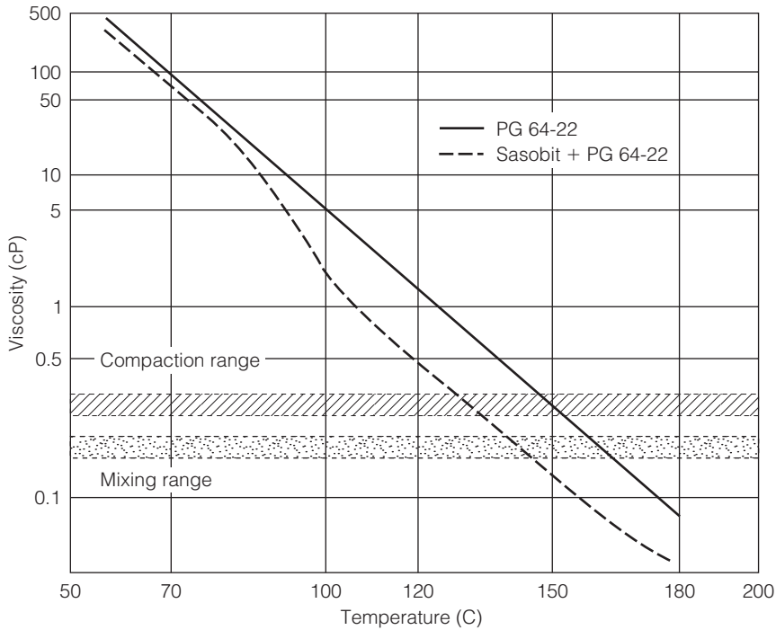
FIGURE 9.44 Temperature-viscosity chart for Sasobit warm mix modifier, Sasobit.
