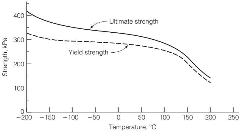
FIGURE 4.6 Tensile strength of aluminum at different temperatures. The Aluminum Association, 1987.
