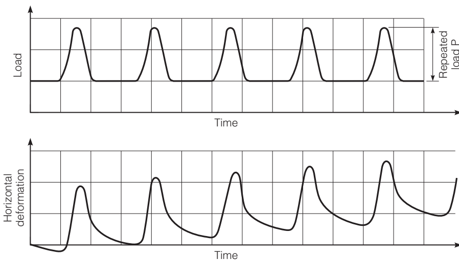
FIGURE 9.34 Typical load and horizontal deformation versus time during the resilient modulus test.
