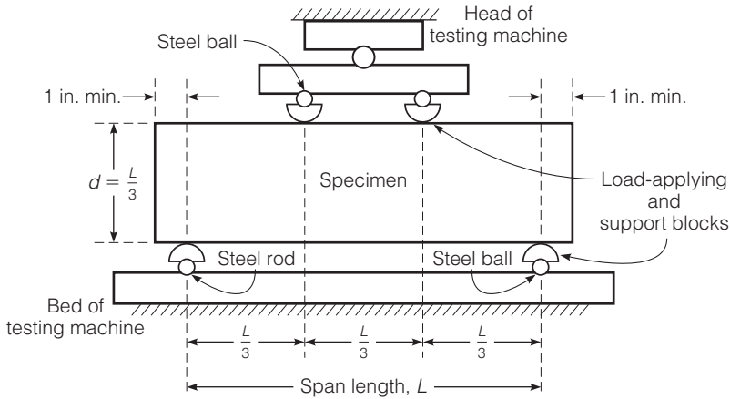
FIGURE 7.36 Apparatus for flexure test of concrete by third-point loading method (Reprinted, with permission, from ASTM C78, Figure 1, copyright ASTM International, 100 Barr Harbor Drive, West Conshohocken, PA 19428.)
