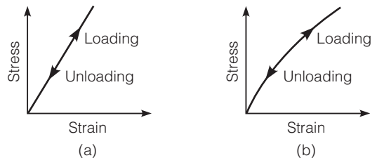
FIGURE 1.4 Elastic behavior: (a) linear and (b) nonlinear.
