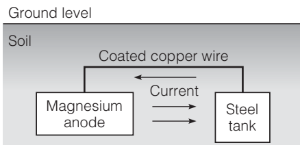
FIGURE 3.32 Cathodic protection of an underground pipeline using a magnesium sacrificial anode.
