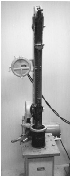
FIGURE 9.27 Marshall compactor.
