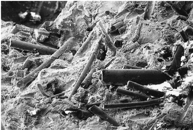
FIGURE 11.11 Scanning electron micrograph of concrete mortar mixed with carbon fibers.
