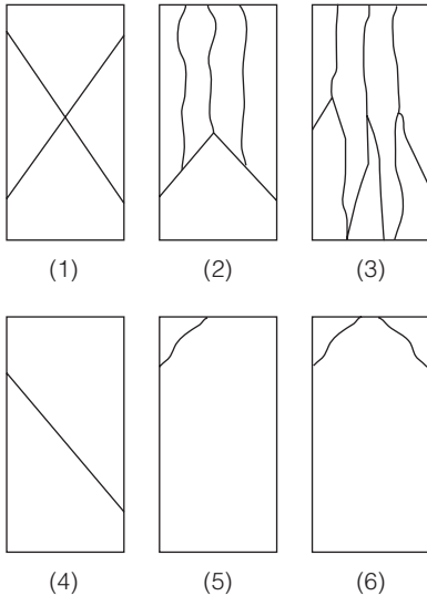
FIGURE A.40 Typical fracture patterns of concrete cylinders: (1) cones on both ends, (2) cone on one end and vertical cracks, (3) vertical cracks, (4) diagonal fracture, (5) side fracture, and (6) side fractures with pointed ends.
