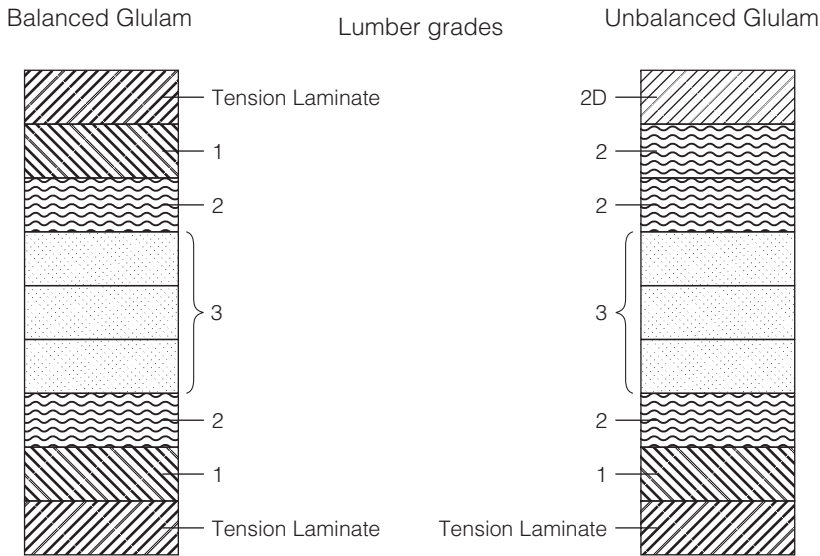
FIGURE 10.23 Layup arrangement for balanced and unbalanced glulams.
