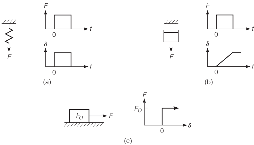
FIGURE 1.11 Basic elements used in rheology: (a) Hookean, (b) Newtonian, and (c) St. Venant's.
