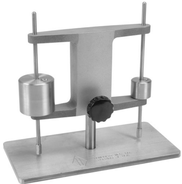
FIGURE 6.6 Gillmore set time apparatus. (Courtesy of Humboldt Mfg. Co.)
