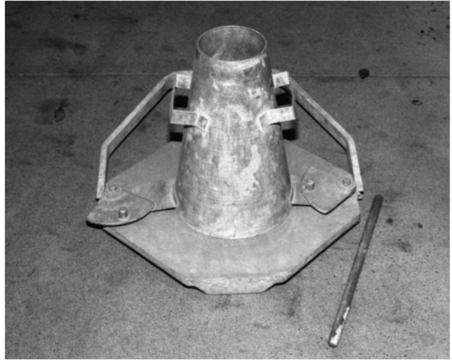
FIGURE 7.3 Slump test apparatus.
