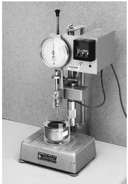
FIGURE A.52 Apparatus for penetration test of asphalt binder.
