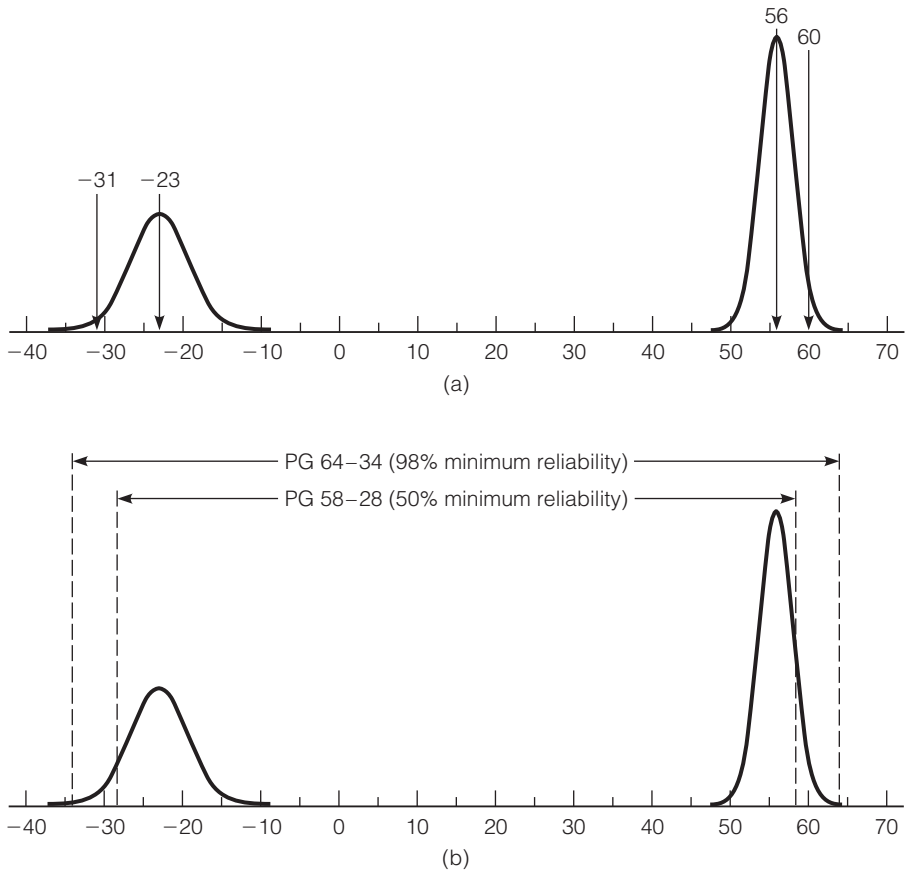
FIGURE 9.25 Example of the distribution of design pavement temperatures and selection of binder grades: (a) distribution of high and low design pavement temperatures, and (b) binder grade selection.
