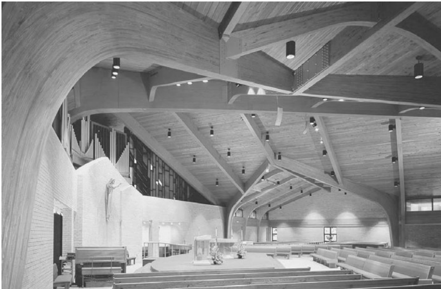
FIGURE 10.6 Frames made of structural glued laminated timber (glulam). (Courtesy of the American Institute of Timber Construction)
