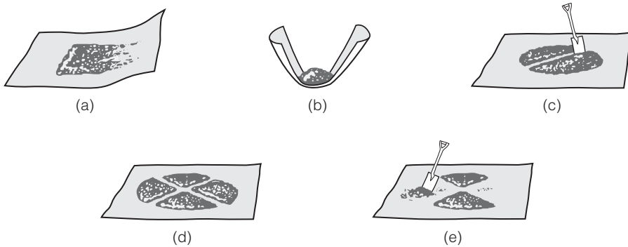
FIGURE 5.22 Steps for reducing the sample size by quartering: (a) mixing by rolling on blanket, (b) forming a cone after mixing, (c) flattening the cone and quartering, (d) finishing quartering, (e) retaining opposite quarters (the other two quarters are rejected). (ASTM C702). Copyright ASTM. Reprinted with permission.
