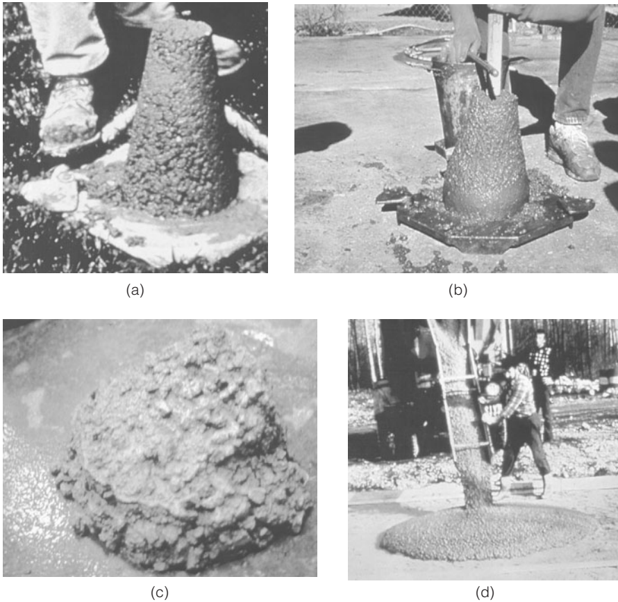
FIGURE 6.9 Slumps of concretes with the same water-cement ratio: (a) no water reducer, (b) conventional water reducer, (c) mid-range water reducer, (d) high-range water reducer (Superplasticizer).
