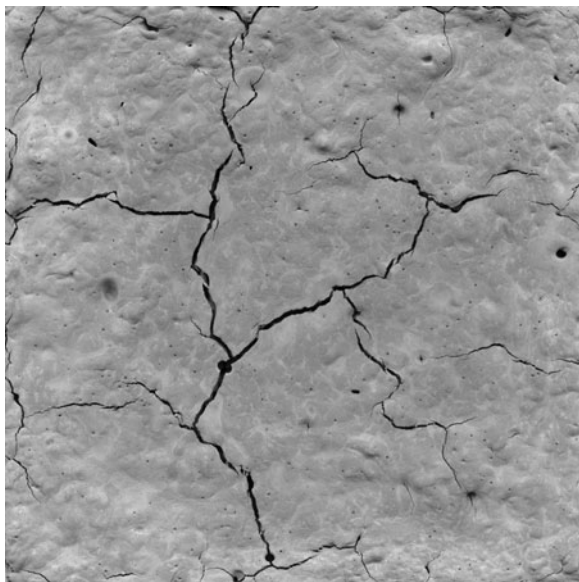
FIGURE 7.30 Plastic shrinkage cracking.
