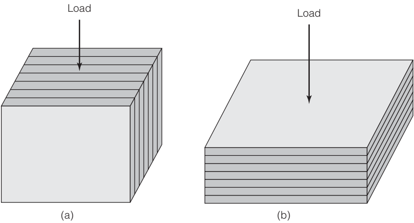
FIGURE 10.21 Axis convention used for defining loading conditions for Laminated Veneer Lumber: (a) edge use and (b) flat use.
