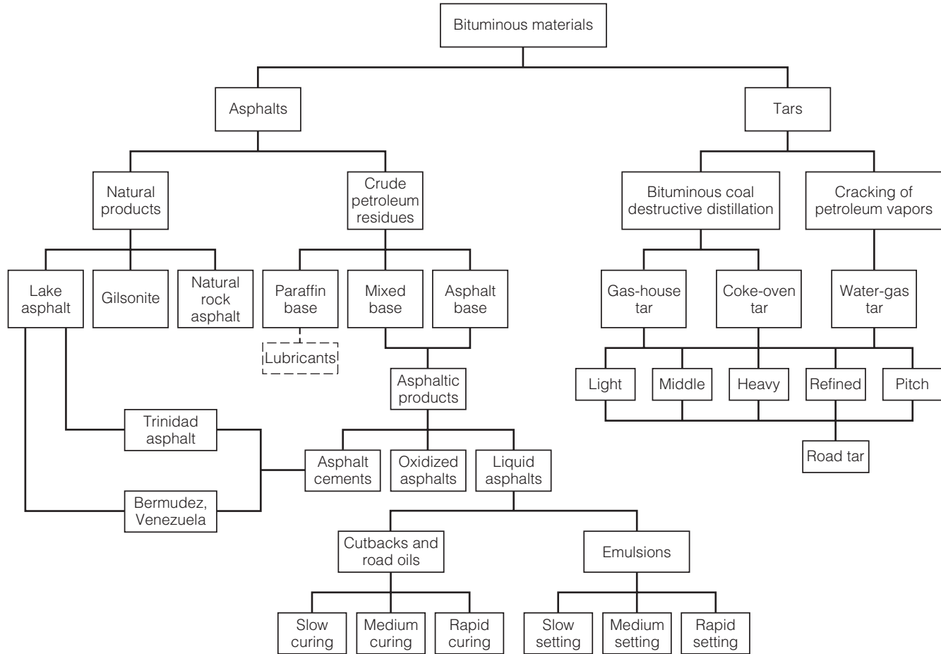
FIGURE 9.1 Classification of bituminous materials (Goetz and Wood, 1960).
