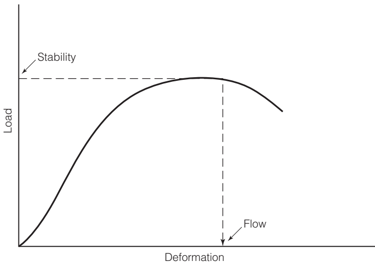
FIGURE A.65 Typical plot of load versus deformation during the Marshall stability test showing the stability and flow.
