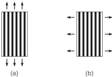
FIGURE 11.14 Patterns of loading continuously aligned fiber-reinforced composites: (a) loading parallel to fibers and (b) loading perpendicular to fibers.
