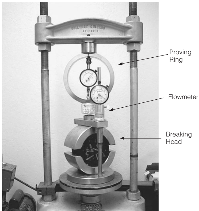
FIGURE A.64 Marshall stability machine.
