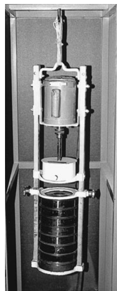
FIGURE A.18 Hanging-type sieve shaker and sieves for small samples of aggregates.
