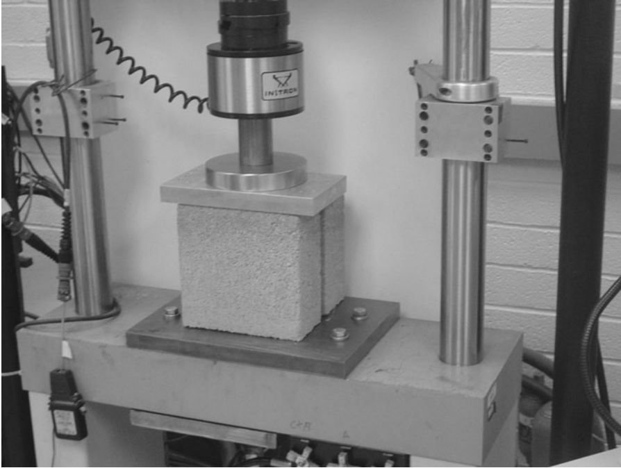
FIGURE A.48 Compression testing of a concrete masonry unit.
