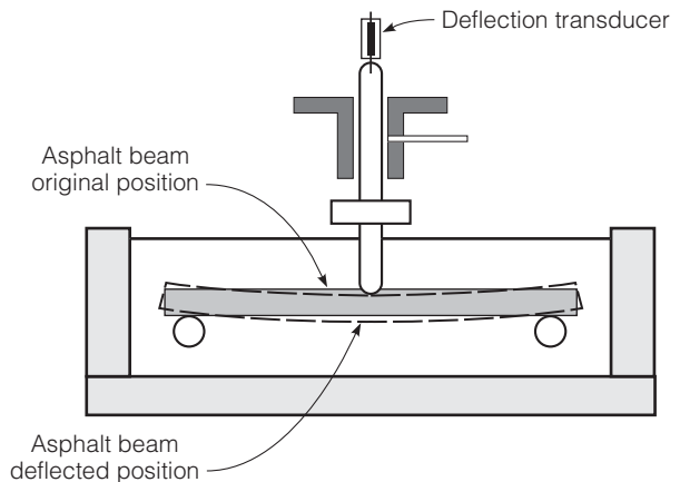
FIGURE 9.21 Schematic of the bending beam rheometer.
