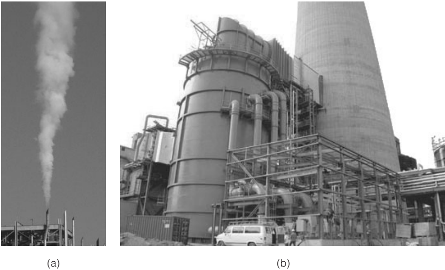
FIGURE 6.12 Fly ash resulting from the combustion of ground or powdered coal (a) being discharged from a smelter before environmental regulations were put into effect and (b) collected into a bag house.
