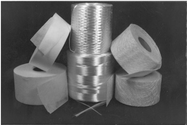
FIGURE 11.4 Common glass fibers (veil, roving, and mat). Photo courtesy of Creative Pultrusions, Inc.
