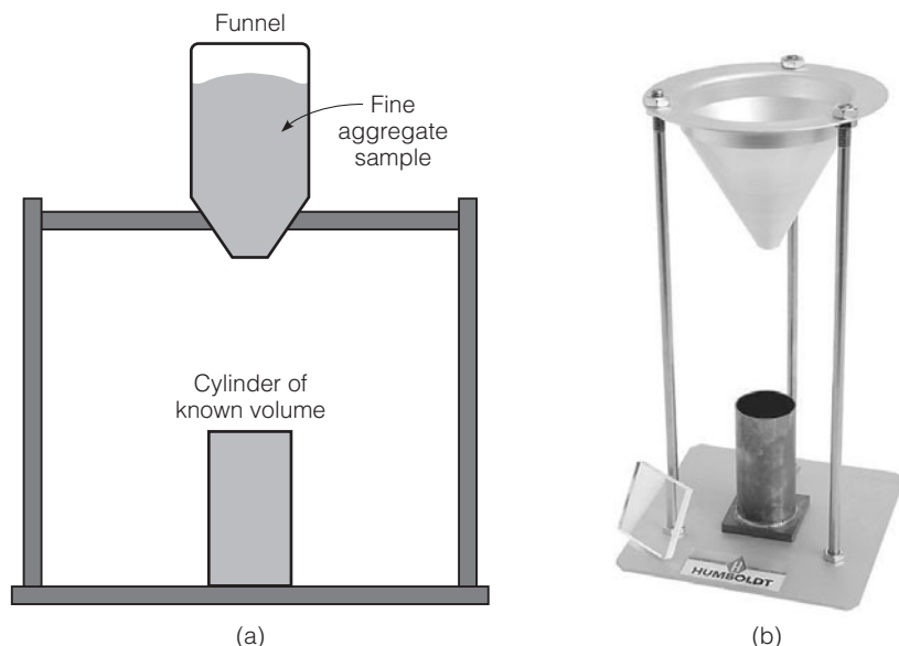
FIGURE 5.7 Apparatus used to measure angularity and surface texture of fine aggregate.
