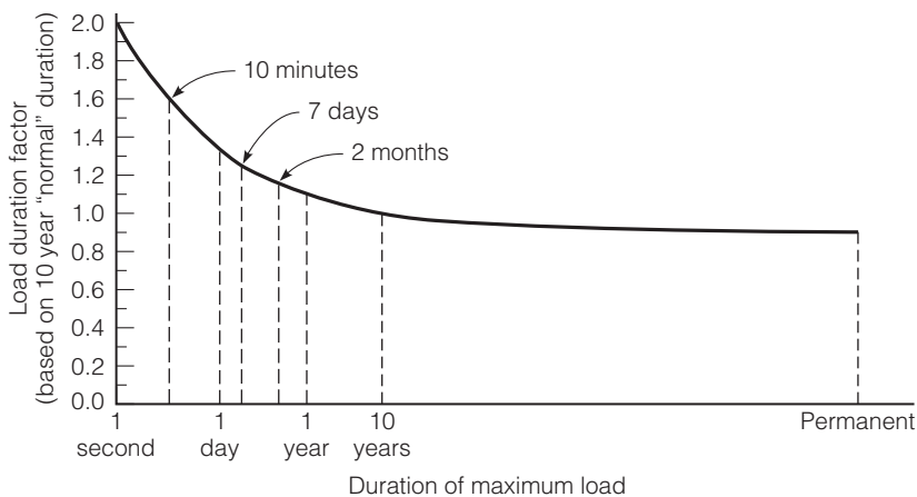
FIGURE 10.13 Adjustment factors for load duration working-stress for wood design based on 10-year nominal duration. Reprinted with permission of American Forest and Paper Association (1997).
