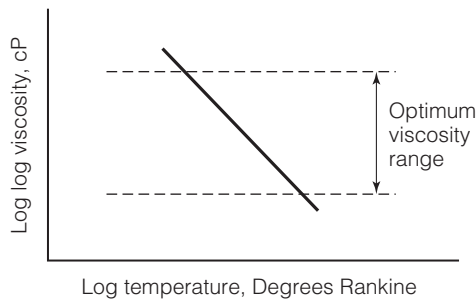
FIGURE 9.11 Typical relation between asphalt viscosity and temperature.
