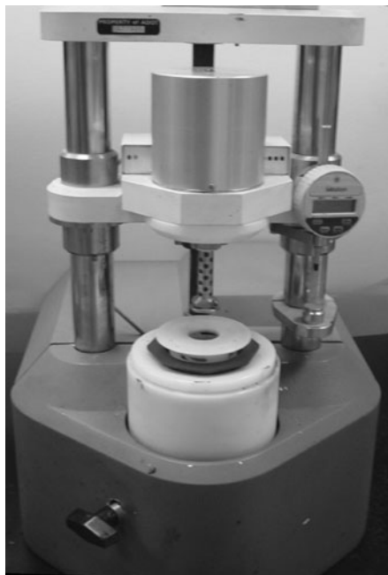
FIGURE A.50 Dynamic shear rheometer apparatus.
