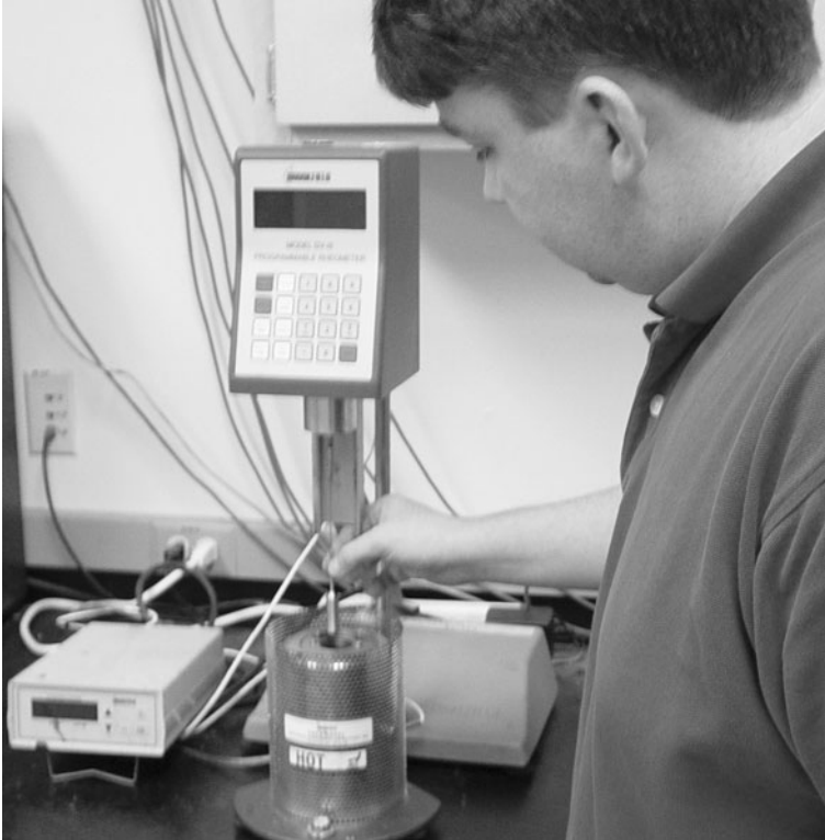
FIGURE A.49 Inserting the spindle into chamber during the rotational viscometer test.
