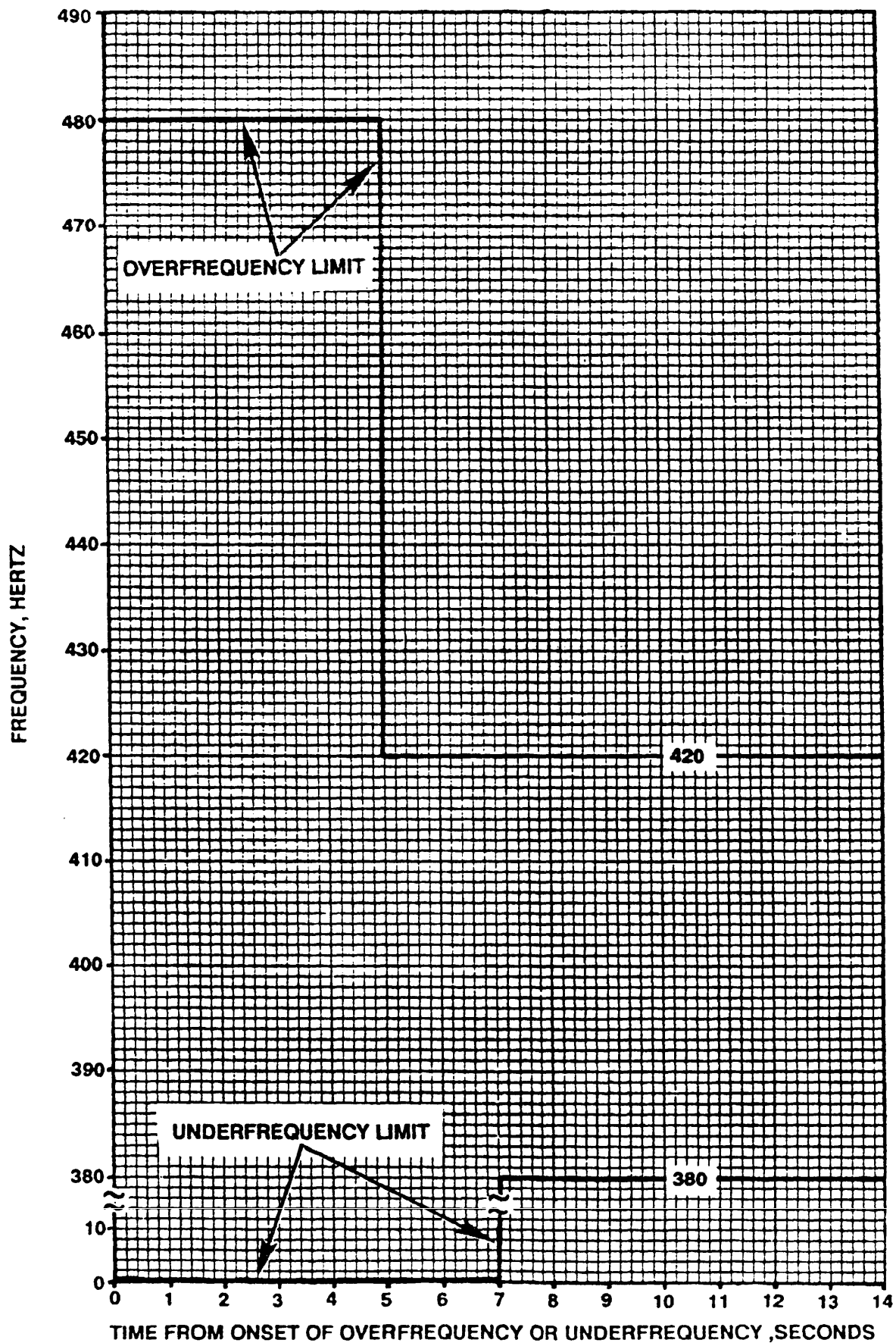
FIGURE 7. Limits for AC overfrequency or underfrequency.
