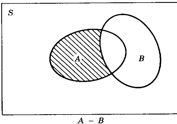
Figure 6.12. Difference, A - B .
