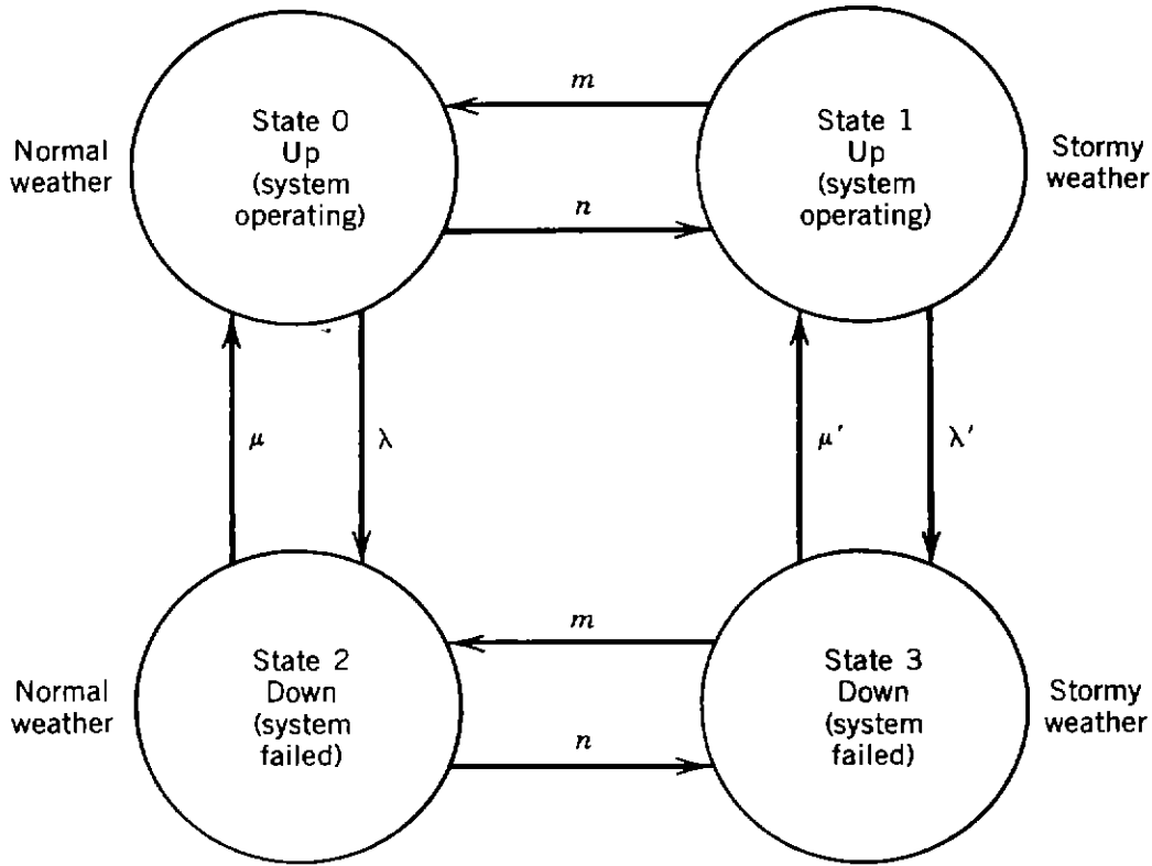
Figure 6.24. State space diagram for single component operating in two-weather environment.
