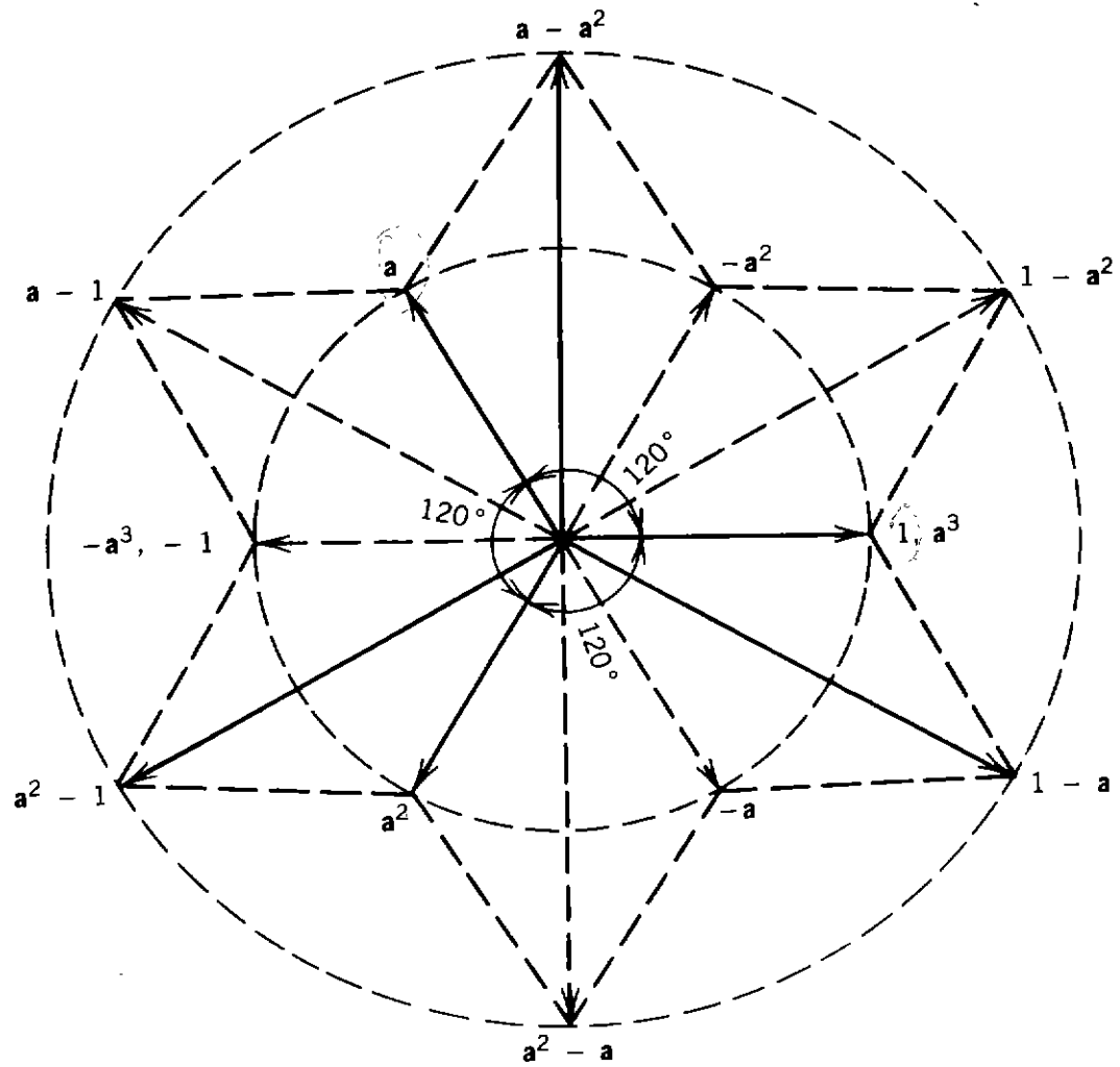
Figure 3.2. Phasor diagram of various powers and functions of operator a .
