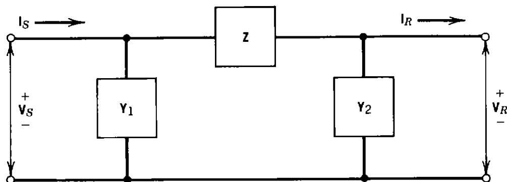
Figure 2.41. Asymmetrical- \Pi network.
