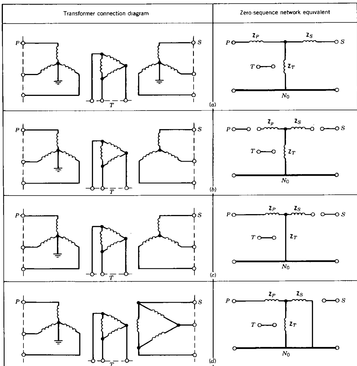
Figure 3.11. Zero-sequence network equivalents of three-phase transformer banks made of three identical single-phase transformers with three windings.
