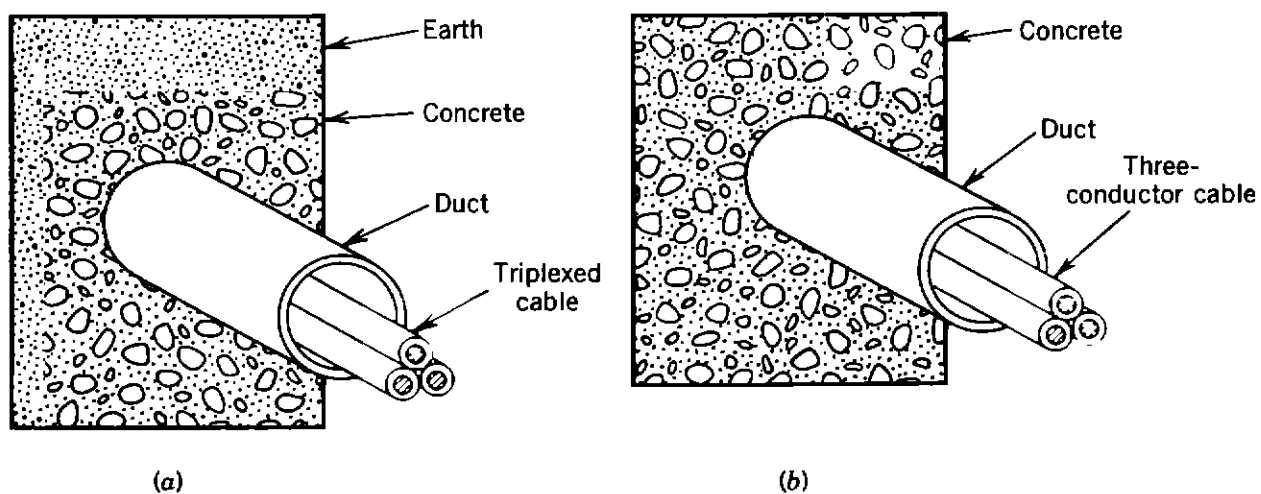
Figure 4.7. Burial in underground cuts (or duct bank): (a) for three single-conductor or triplexed, cables, (b) for three-conductor cable.
