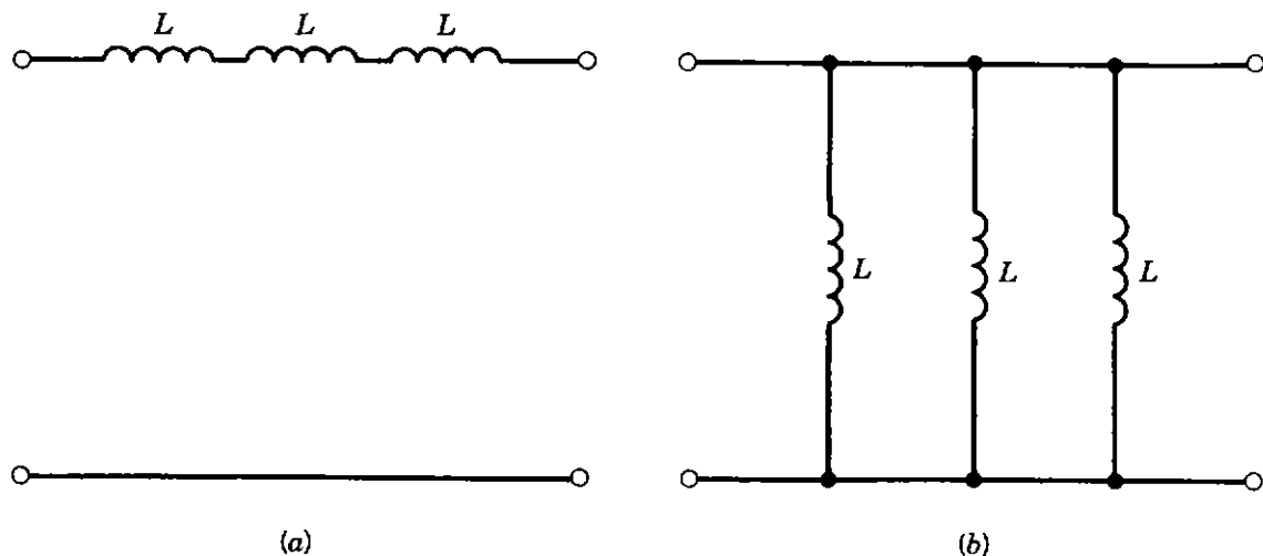
Figure 2.36. Transmission line compensation by adding lump inductances in: (a) series; (b) parallel (i.e., shunt).
