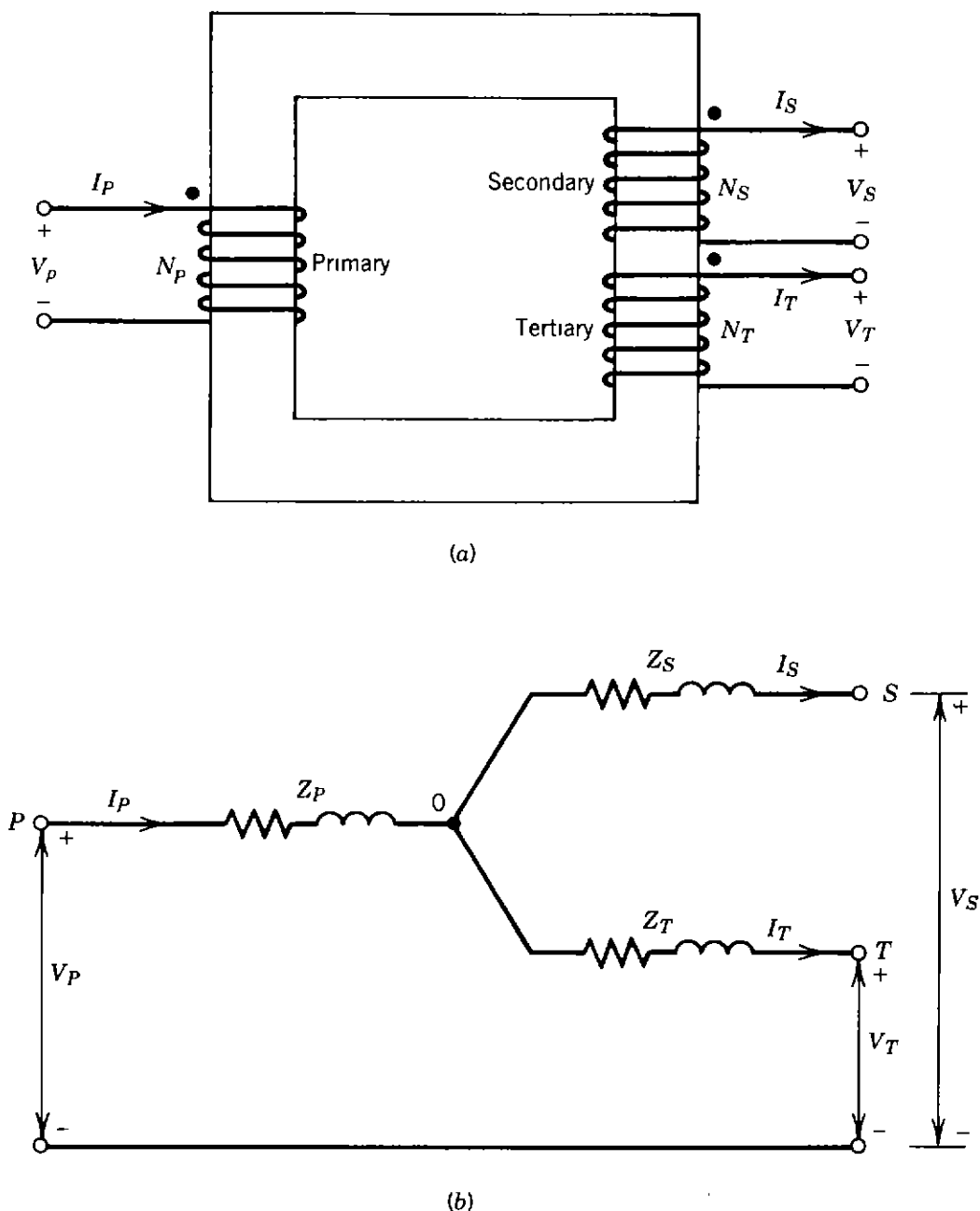
Figure 2.6. A single-phase three-winding transformer: (a) winding diagram; (b) equivalent circuit.
