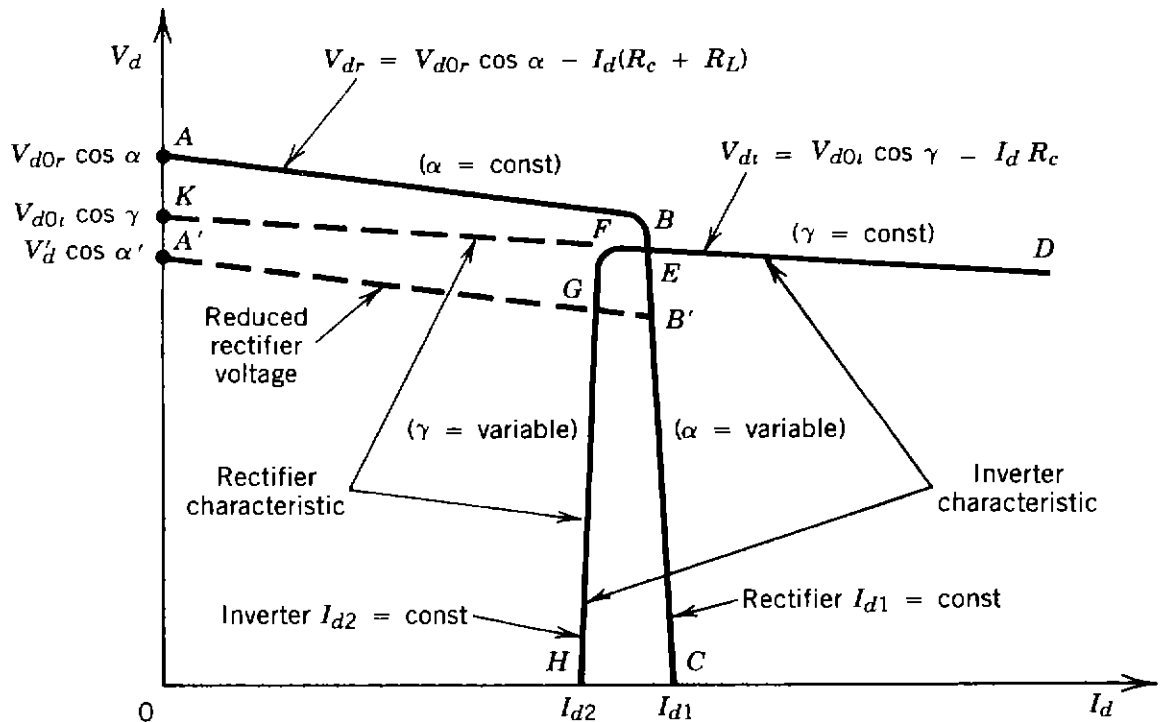
Figure 5.16. Inverter and rectifier operation characteristics with constant-current compounding.
