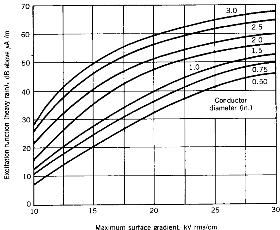
Figure 8.11. Radio interference excitation function in heavy rain of different bundles as function of maximum surface gradient (add 7 dB for n = 1 , 2 dB for n = 2 , and 0 dB for n = 3 , where n is number of subconductors). (From Ref. 27. Used with permission. © 1971 IEEE.)
