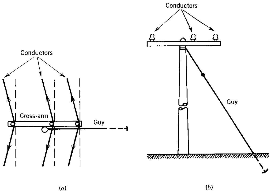
Figure 9.15. Guy installation at an angle: (a) plan; (b) elevation.
