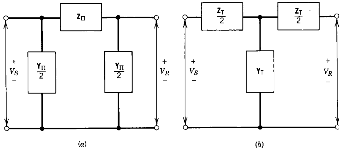
Figure 2.32. Equivalent and T circuits for long transmission line.
