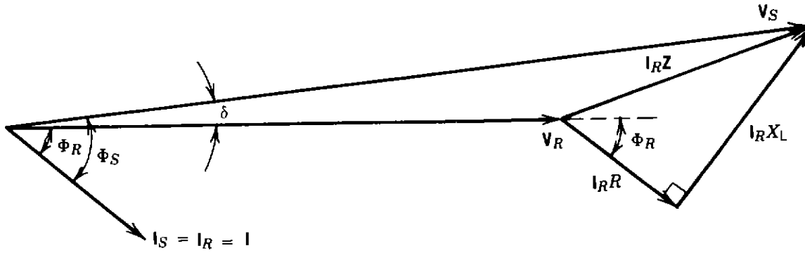
Figure 2.24. Phasor diagram of short transmission line to inductive load.
