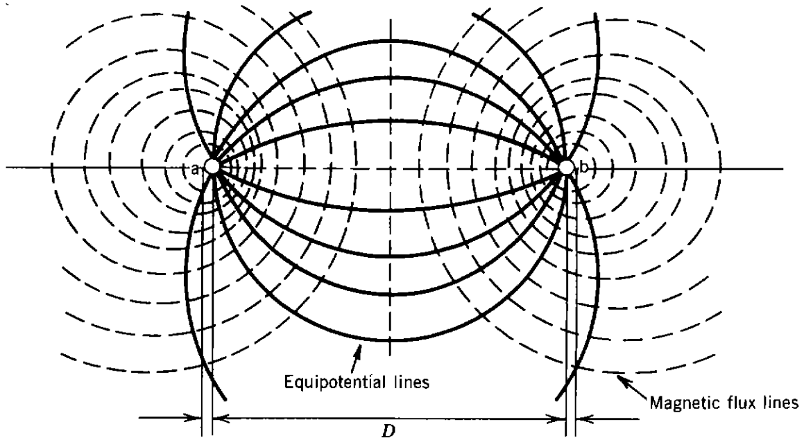
Figure 2.16. Magnetic field of single-phase line.
