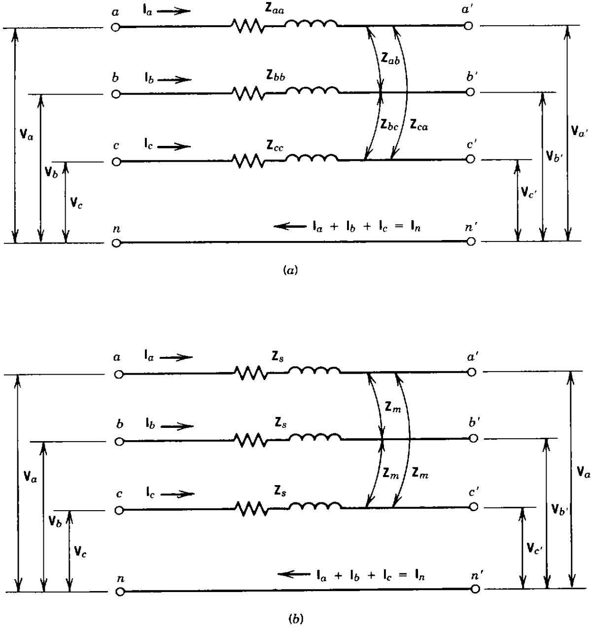
Figure 3.3. Transmission line circuit diagrams: (a) with unequal series and unequal impedances; (b) with equal series and equal mutual impedances.
