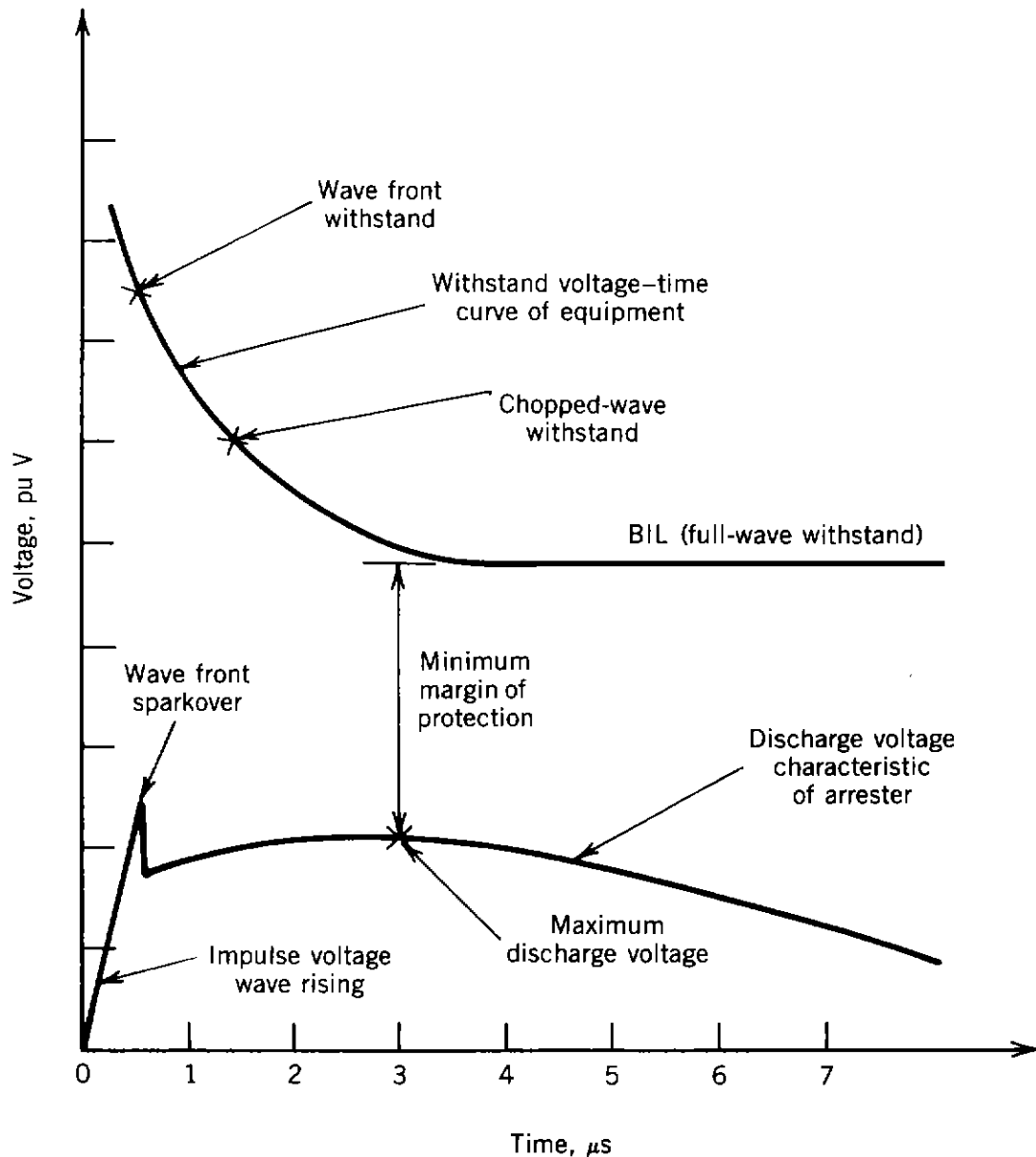
Figure 7.23. Illustration of insulation coordination between oil-filled equipment and surge arrester.
