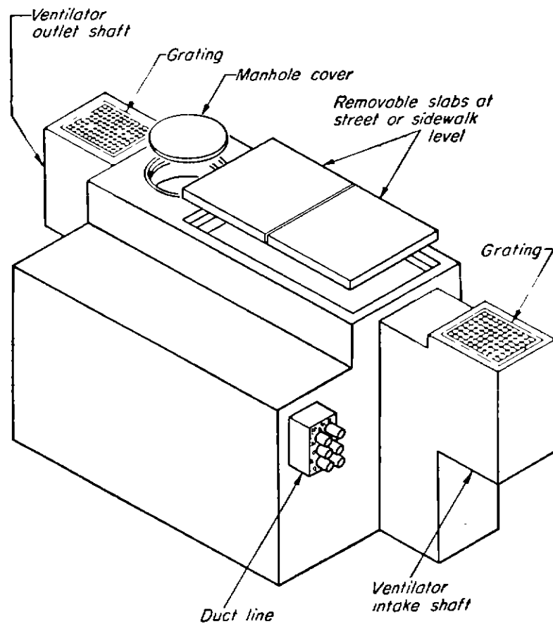
Figure 4.9. Street cable manhole [8].
