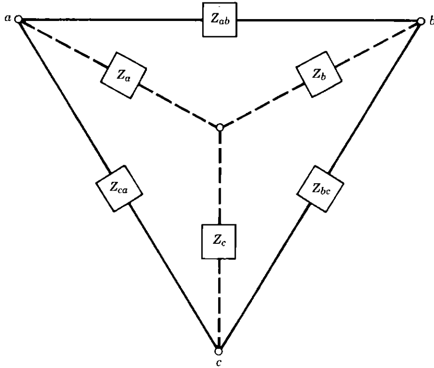
Figure 2.8. Delta-to-wye or wye-to-delta transformations.
