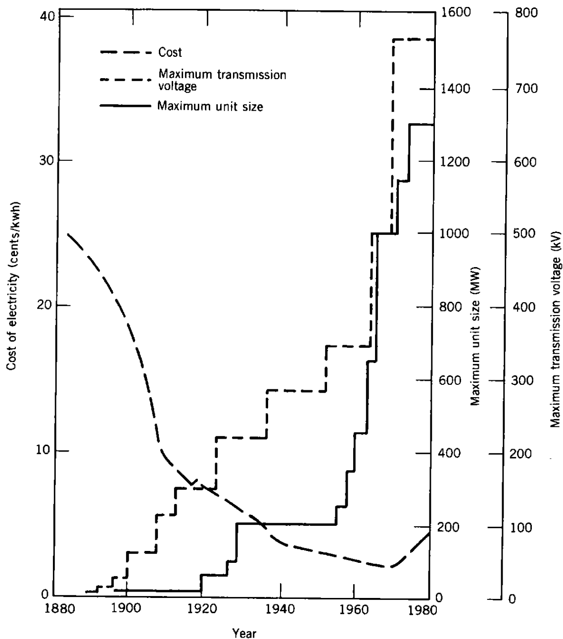
Figure 1.2. Historical trends in technology and cost of electrical energy. (From Electric Power Research Institute, 1979. Used by permission. © 1979 Electric Power Research Institute.)
