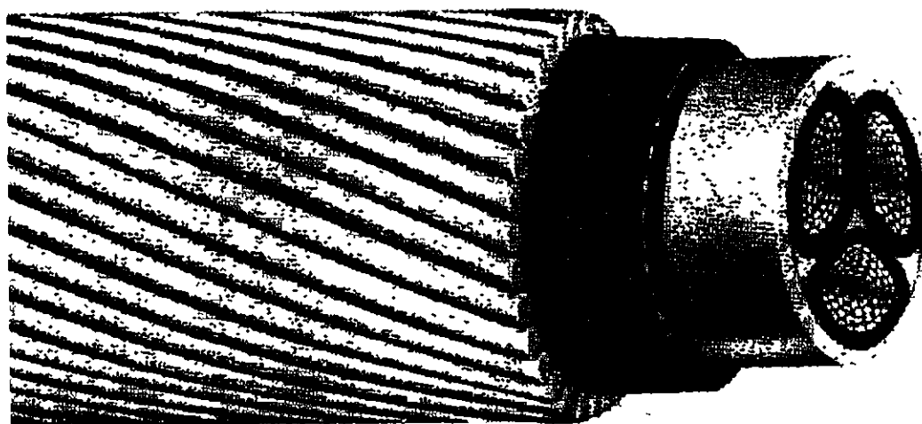
Figure 4.4. Various protective outer coverings for solid-type paper-insulated cables. (Courtesy of Okonite Company.)
