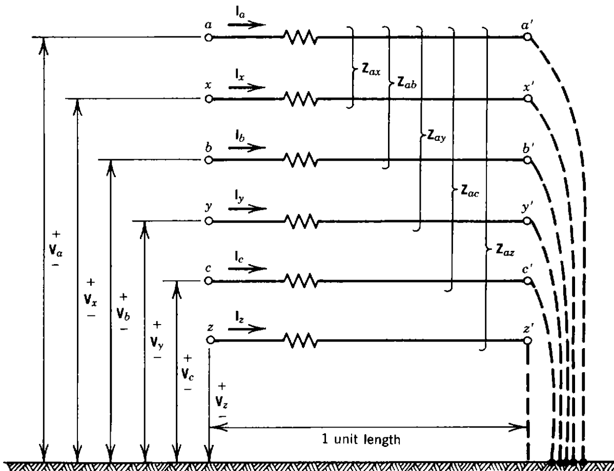
Figure 4.31. Three single-conductor cables with ground return.
