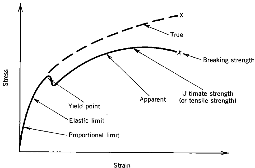
Figure 9.4. Stress-strain diagram.
