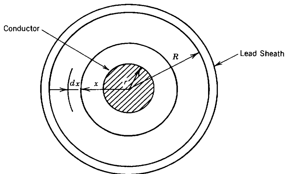
Figure 4.10. Cross section of single-conductor cable.
