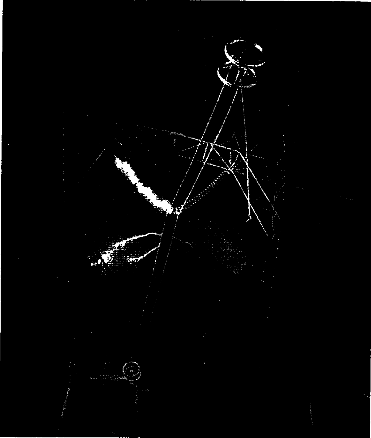
Figure 7.19. View of 500-kV line with two bundled conductors exposed to man-made lightning. (Courtesy of Ohio Brass Company.)
