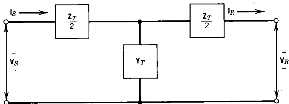
Figure 2.40. Transformer equivalent circuit at full load.
