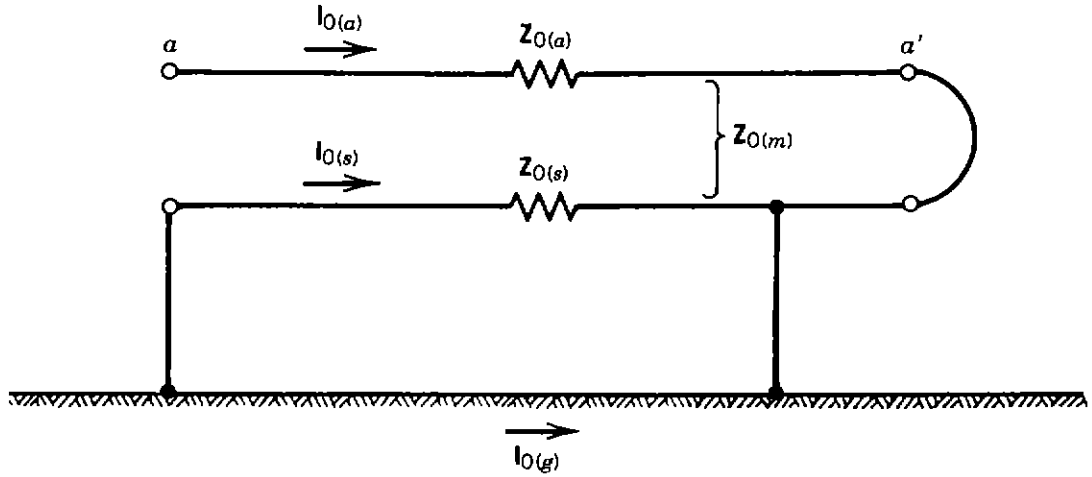
Figure 4.27. Equivalent circuit of three-conductor cable.
