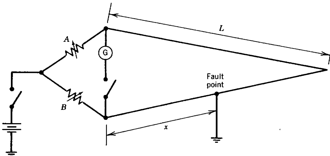
Figure 4.34. Murray loop.
