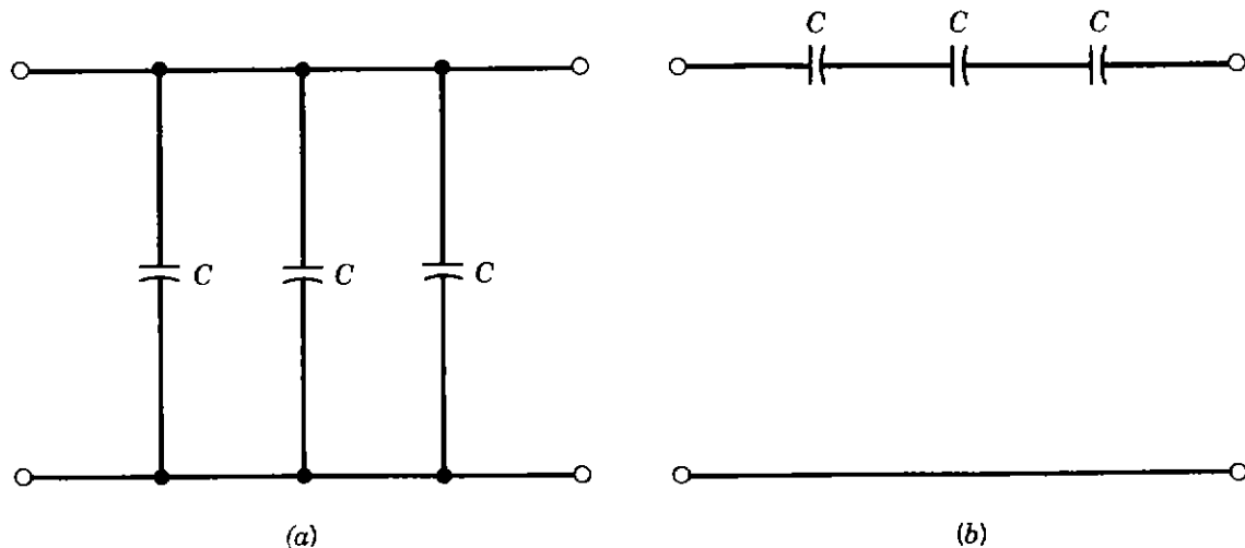
Figure 2.37. Transmission line compensation by adding capacitances in: (a) parallel (i.e., shunt); (b) series.
