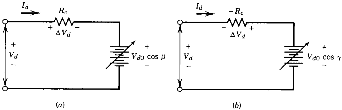
Figure 5.8. Equivalent circuits of inverter: (a) with constant \beta ; (b) with constant \gamma .
