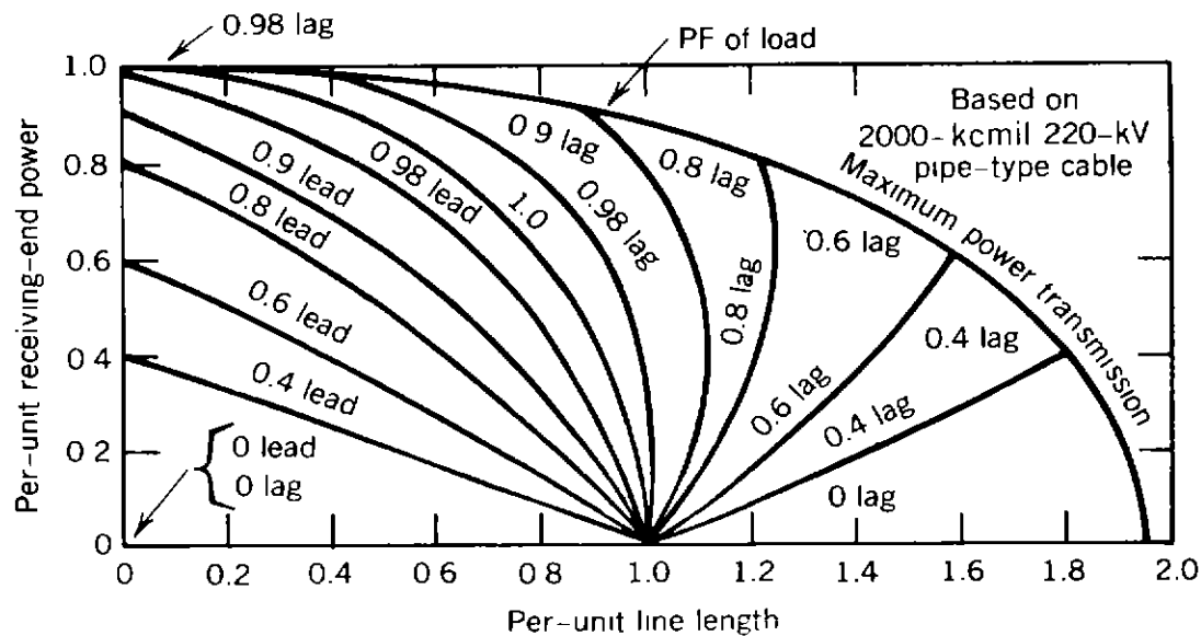
Figure 2.50. Power transmission limits of high-voltage ac cable lines. Curved lines: Sending-end current equal to rated or base current of cable. Horizontal lines: Receiving-end current equal to rated or base current of cable. (From Ref. 12. Used by permission. © 1956 IEEE.)
