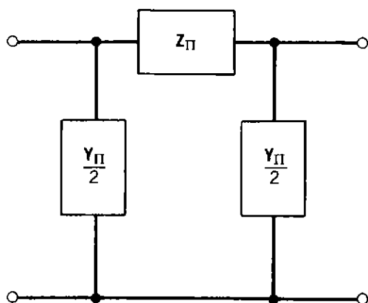
Figure 2.33. Equivalent- \Pi circuit.
