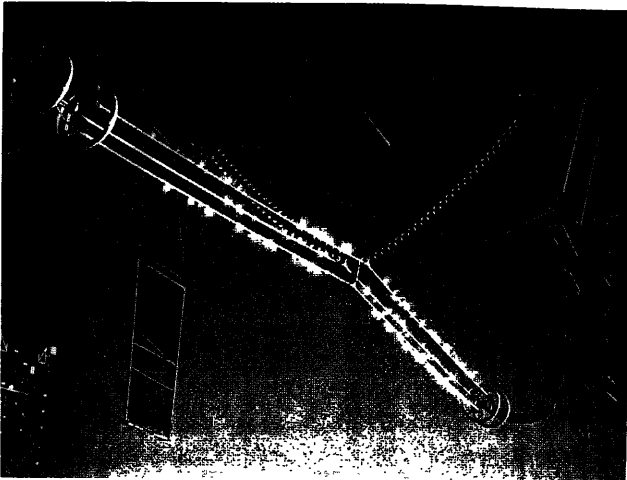
Figure 8.3. Corona testing on 500-kV triple-conductor support at elevated 60-Hz voltage for visual study of corona. (Courtesy of Ohio Brass Company.)
