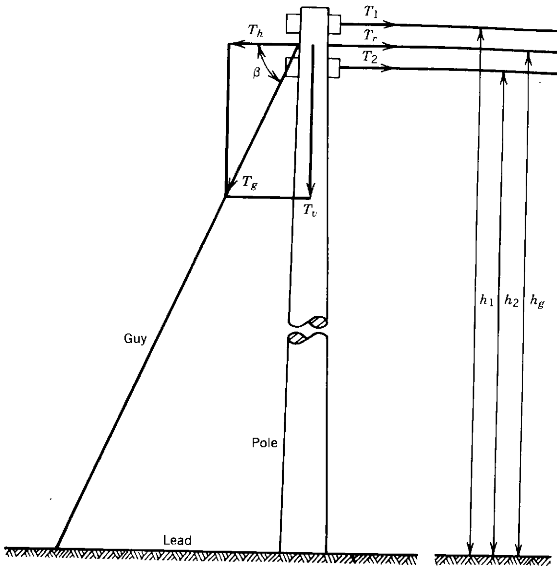
Figure 9.18. Guy-loading diagram.
