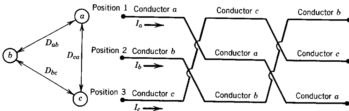
Figure 2.17. Transposition cycle of three-phase line.
