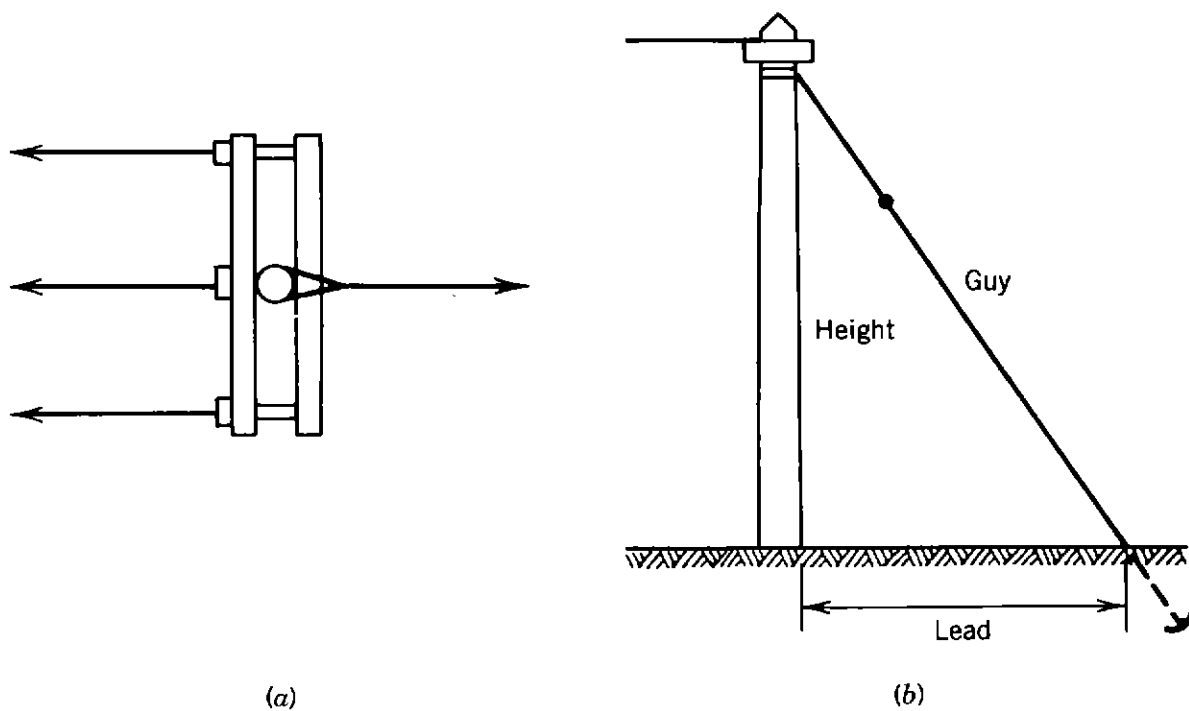
Figure 9.16. Dead-end guy installation: (a) plan; (b) elevation.
