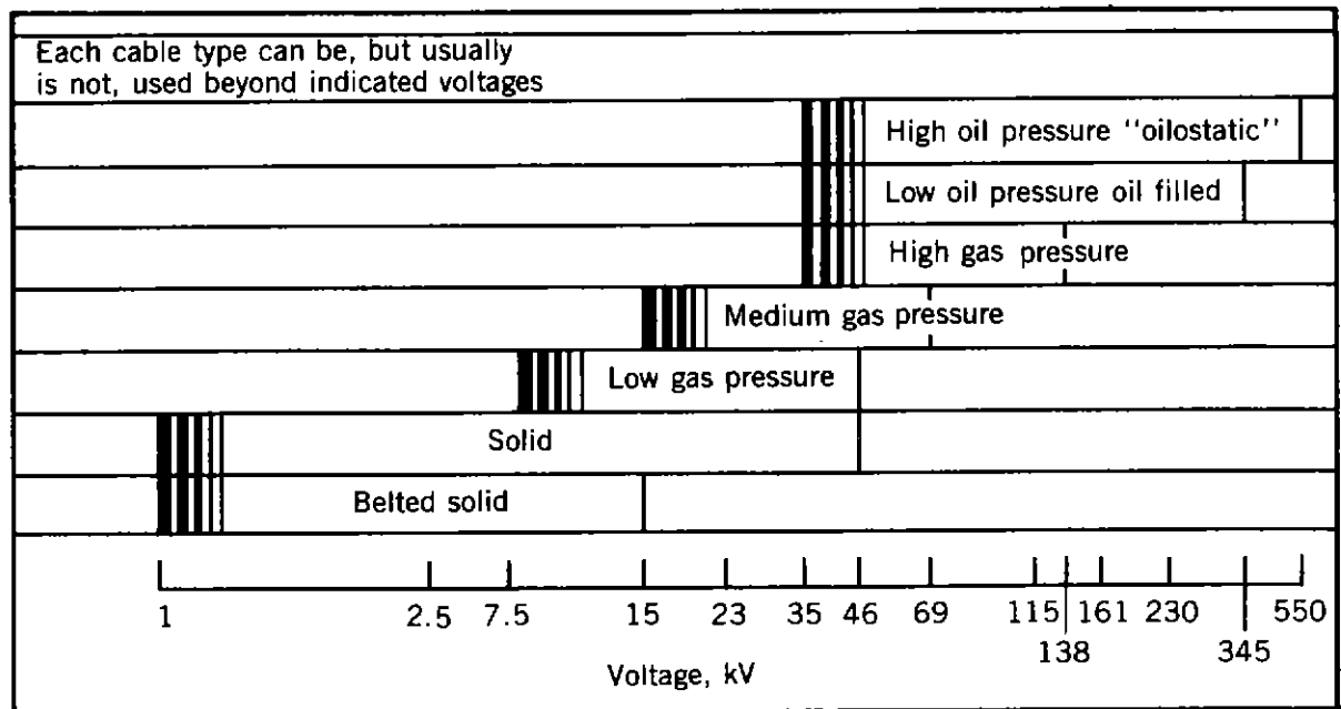
Figure 4.5. Recommended voltage ranges for various of paper-insulated paper cables. (Courtesy of Okonite Company.)
