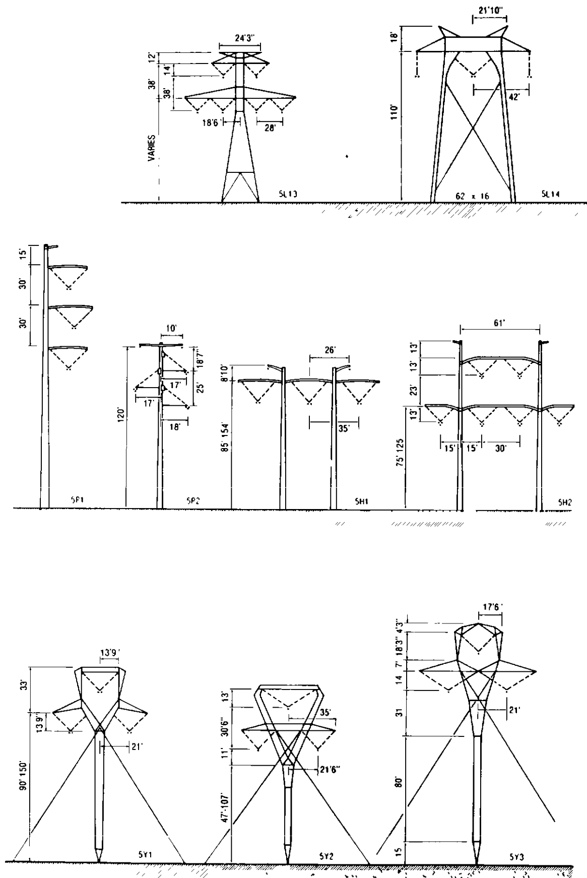
Figure 2.12. Typical 500-kV lattice, pole, guyed V- and Y-type structures (From Ref. 14. Used by permission. © 1979 Electric Power Research Institute.)
