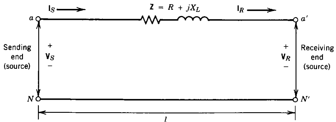
Figure 2.23. Equivalent circuit of short transmission line.
