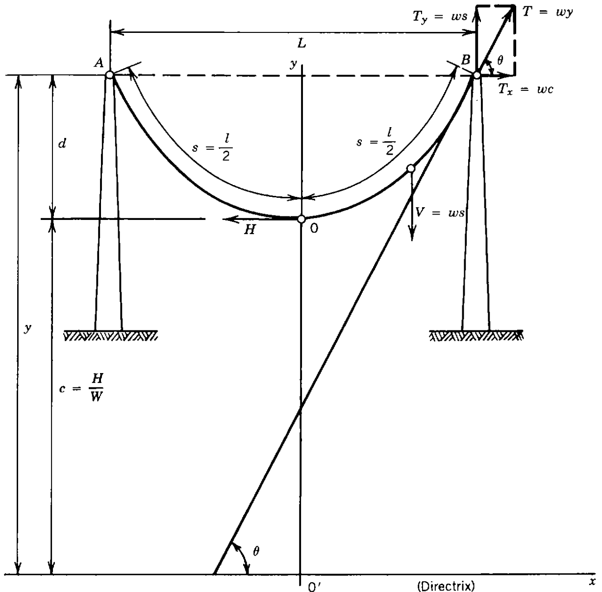
Figure 10.3. Parameters of catenary.
