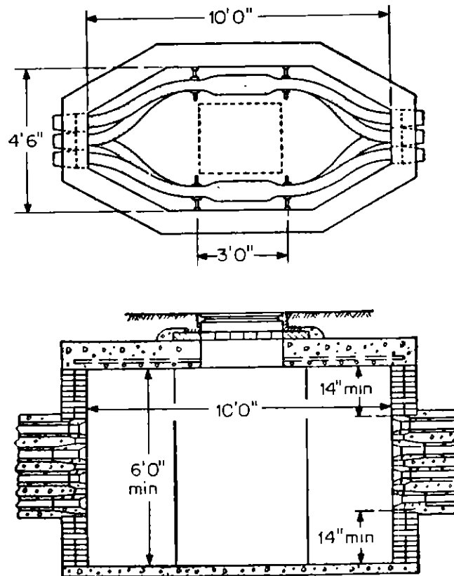
Figure 4.8. Straight-type manhole [4].
