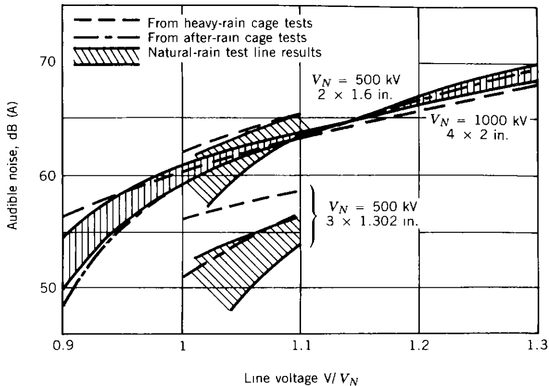
Figure 8.13. Comparison line between audible noise results with test lines under natural rain and computed values from cage tests with artificial rain. Line results are from two 500-kV lines of BPA (measuring point under outside phase) and from single-phase test line of Project UHV (measuring point at 100 ft from line). (From Ref. 27. Used by permission. © 1971 IEEE.)
