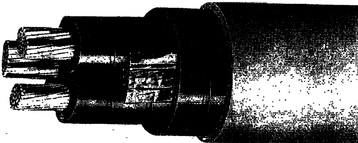
Figure 4.2. Three-conductor, belted, compact-sector, paper-insulated cable. (Courtesy of Okonite Company.)
