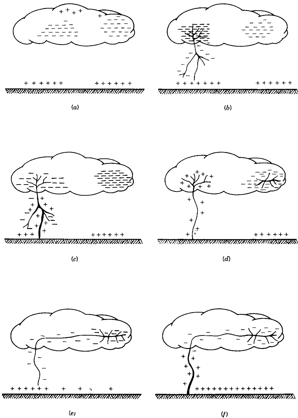
Figure 7.14. Charge distribution at various stages of lightning discharge: (a) charge centers in cloud and induced charge on ground; (b) leader stroke about to strike ground; (c) return stroke; (d) first charge center completely discharged; (e) dart leader; (f) return stroke.
