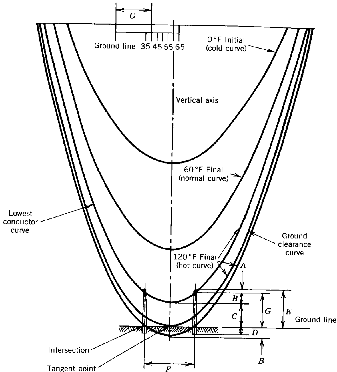
Figure 10.15. Sag template based on values given in Table 10.3: A , dimension from top of pole to point of attachment of lowest conductor; B , sag in level ground; C , ground clearance; D , setting depth of pole; E , length of pole; F , level ground span; G , dimension from ground to point of attachment of lowest conductor.
