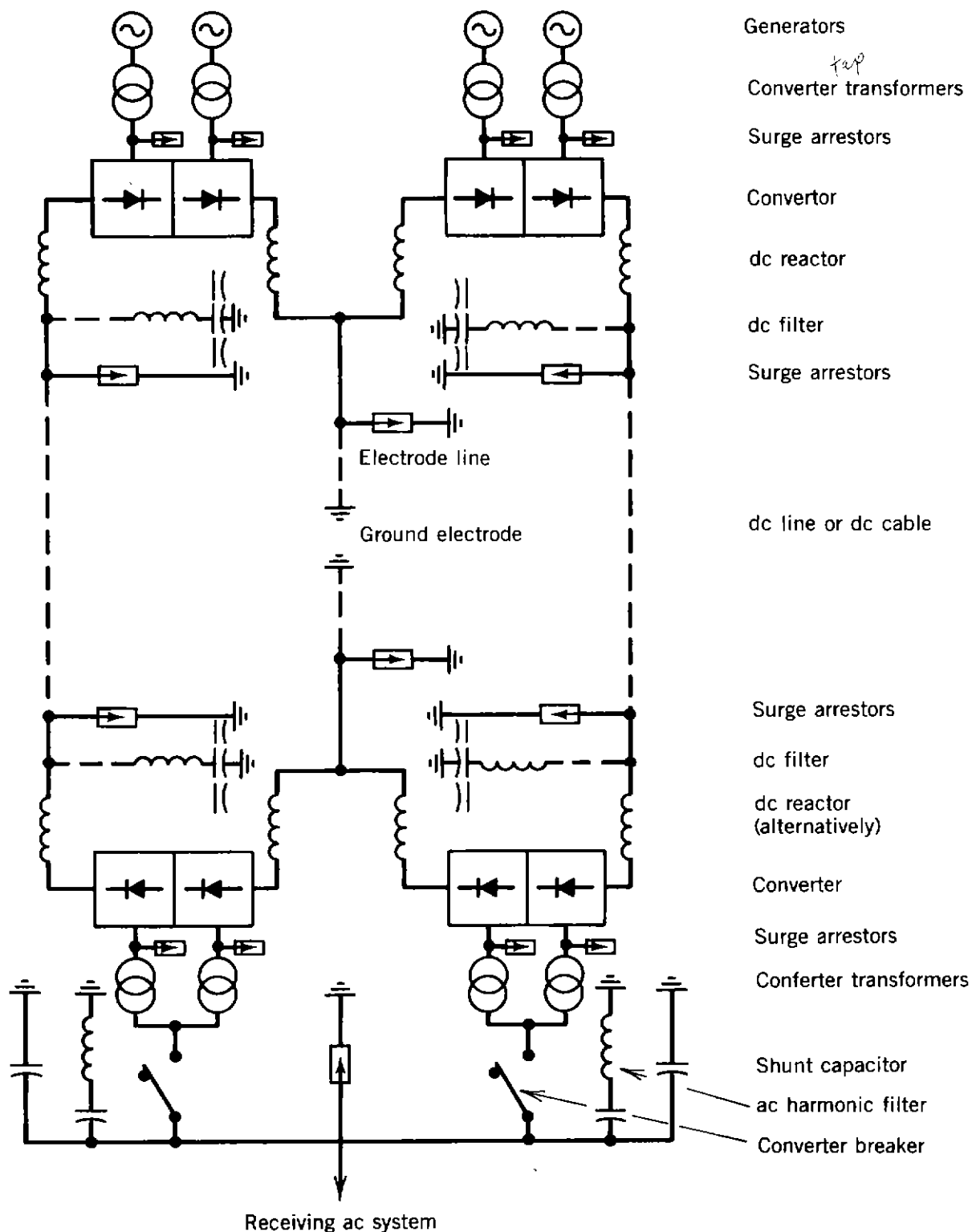
Figure 5.2. A dc transmission system operating in bipolar mode [2].
