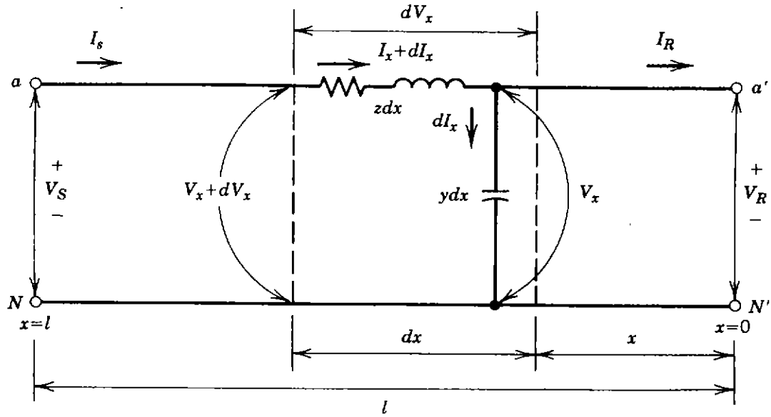
Figure 2.31. One phase and neutral connection of three-phase transmission line.
