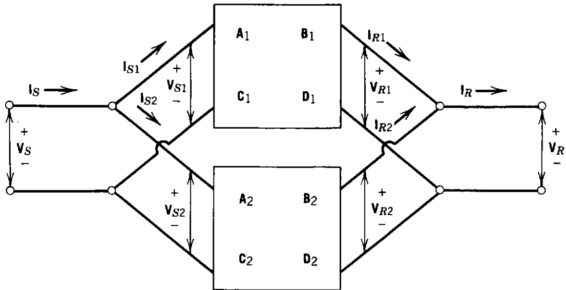
Figure 2.45. Transmission networks in parallel.
