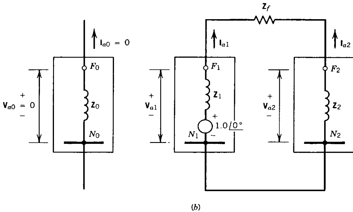
Figure 3.20. Line-to-line fault: (a) general representation; (b) interconnection of sequence networks.
