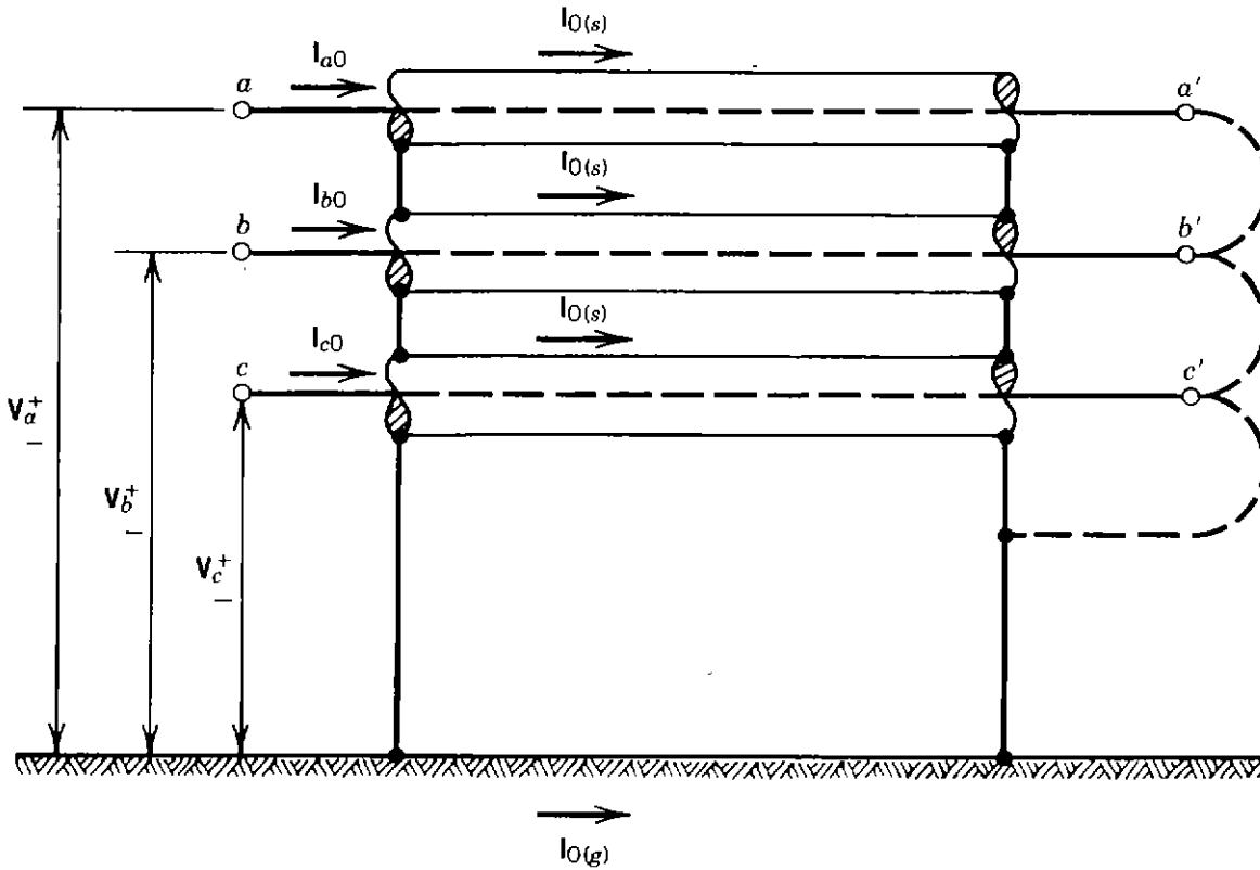
Figure 4.29. Actual circuit of three single-conductor lead-sheathed cables.
