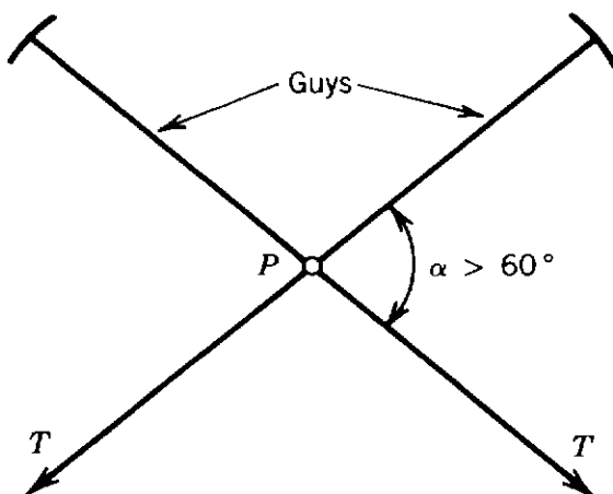
Figure 9.13. Installment of two guys when angle of departure of line is larger than 60^\circ .
