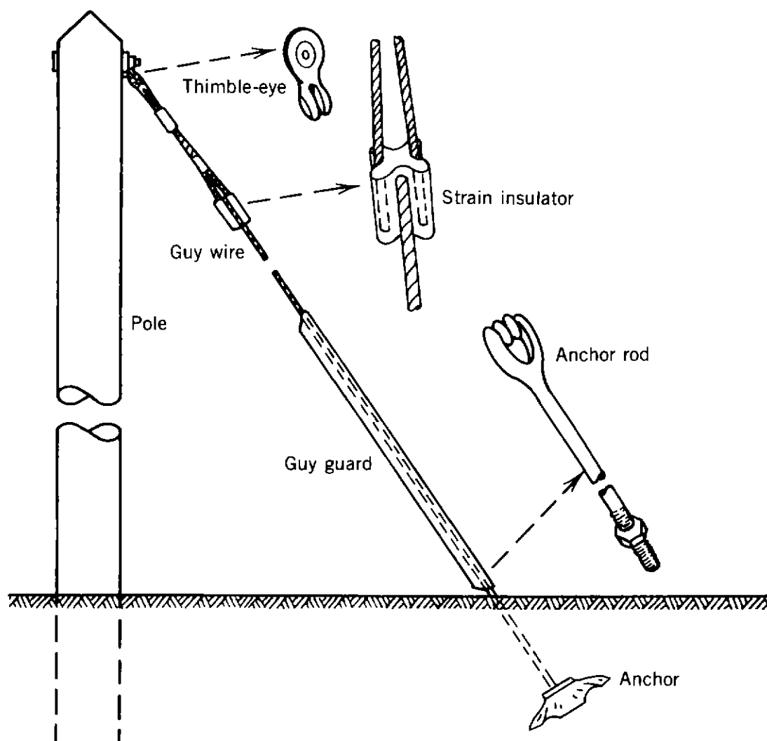
Figure 9.17. Components of anchor guy installation.
