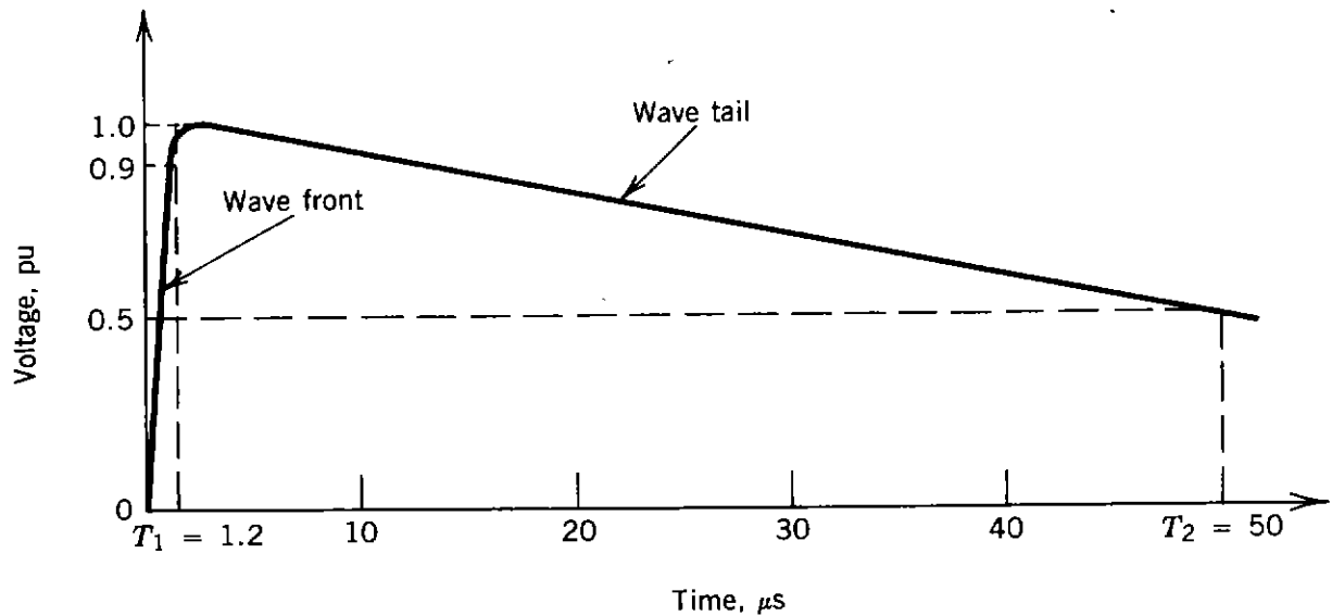
Figure 7.1. Standard impulse voltage waveform.
