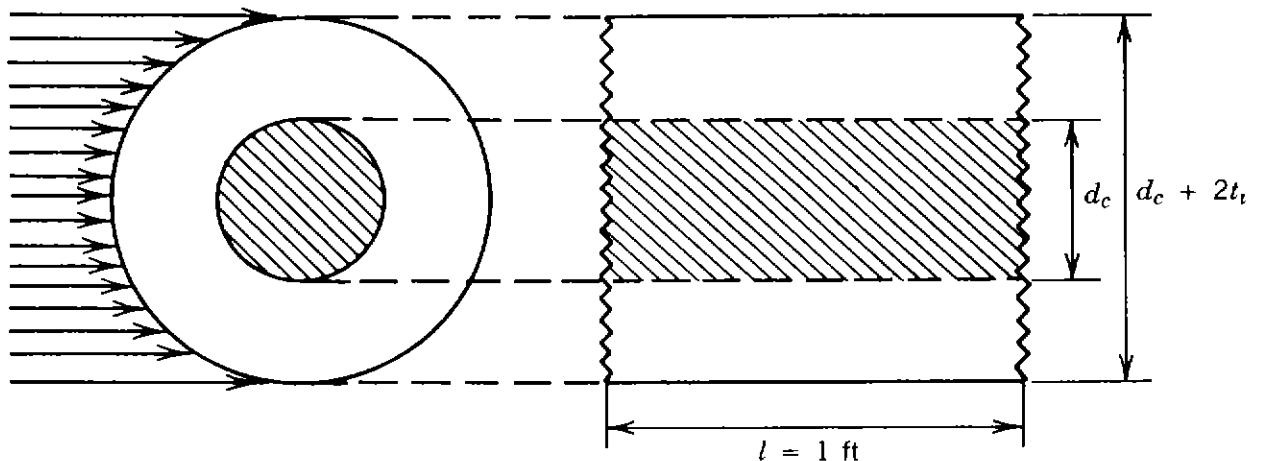
Figure 10.10. Force of wind on conductor covered with ice.
