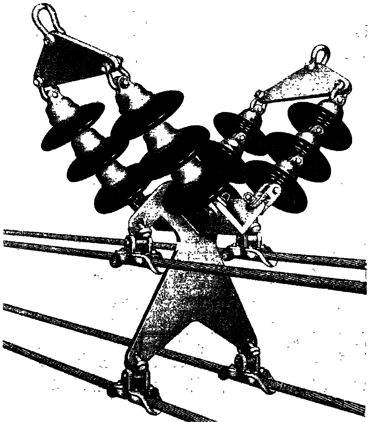
Figure 9.19. Vee arrangement of suspension insulator strings carrying four bundled conductors per phase. (Courtesy of Ohio Brass Company.)
