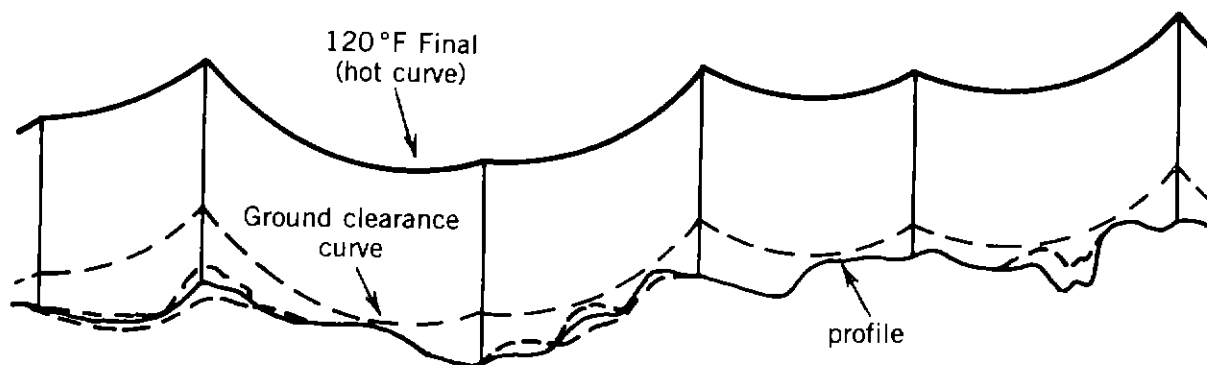
Figure 10.16. Locating structures by templates.
