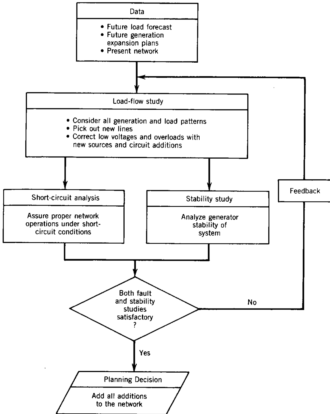
Figure 1.4. Logic diagram for transmission expansion study.
