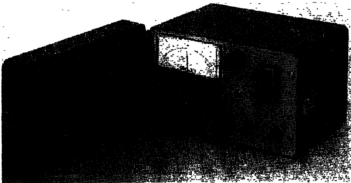
Figure 4.36. Portable Murray loop resistance bridge for cable fault-locating work (Courtesy of James G. Biddle Company.)
