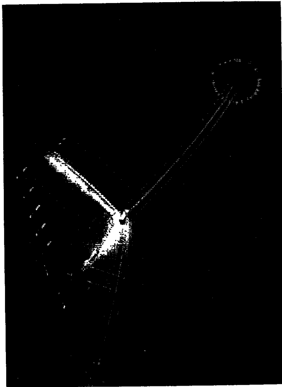
Figure 7.20. View of 500-kV line with three bundled conductors under corona and lightning impulse flashover test. (Courtesy of Ohio Brass Company.)
