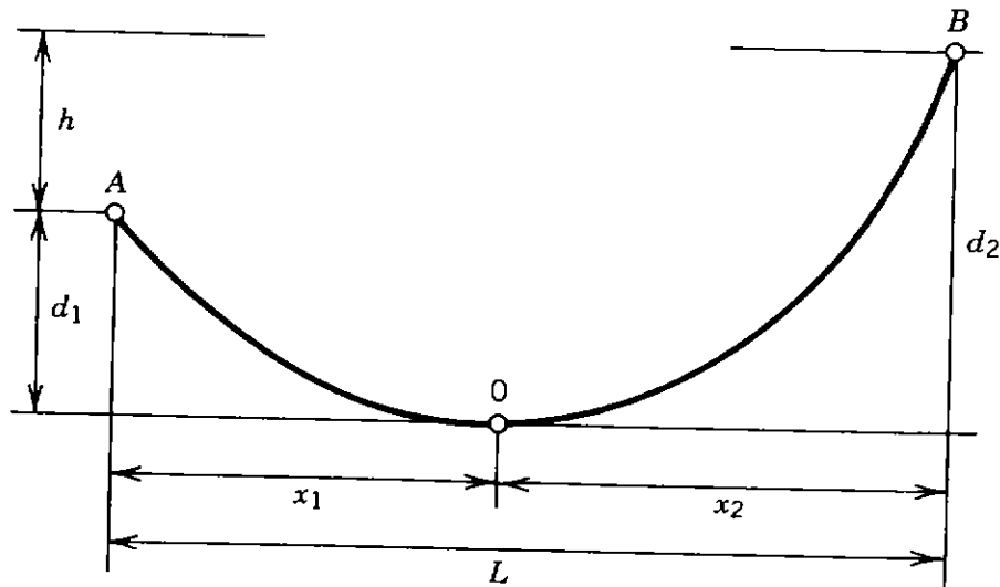
Figure 10.5. Supports at different levels.
