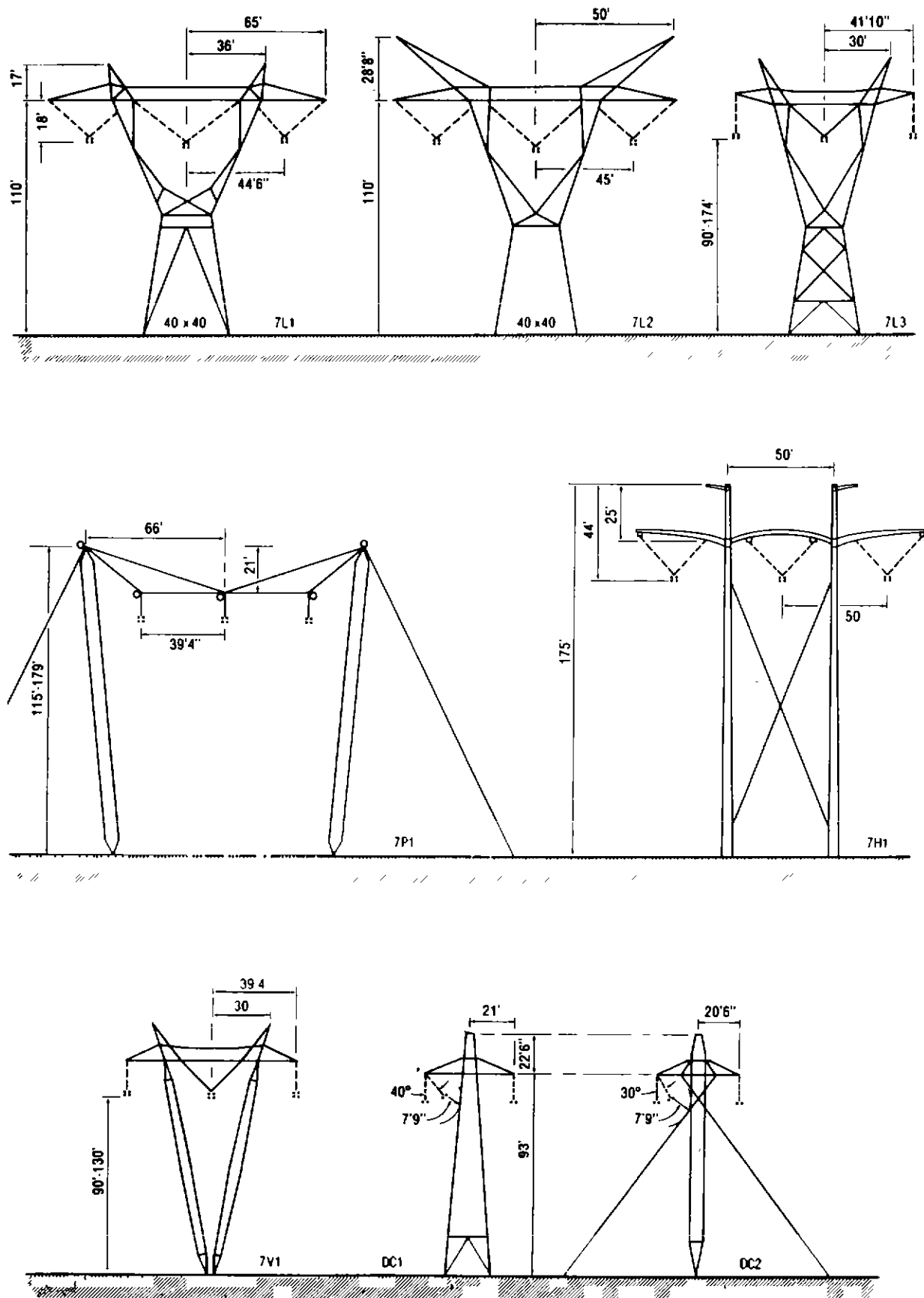
Figure 2.13. Typical 735–800-kV ac designs and dc structures (From Ref. 14. Used by permission: © 1979 Electric Power Research Institute.)
