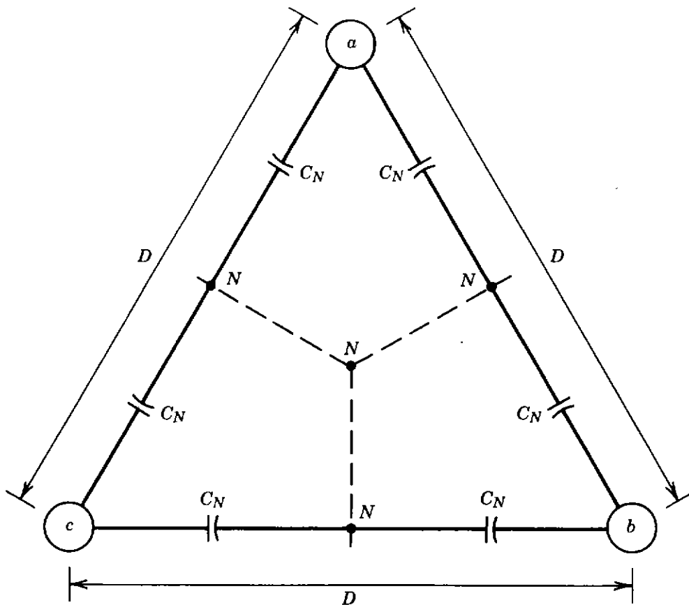
Figure 2.21. Three-phase line with equilateral spacing.
