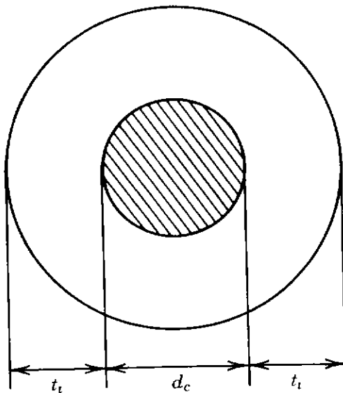
Figure 10.8. Assumed configuration of ice-covered conductor cross-sectional area.
