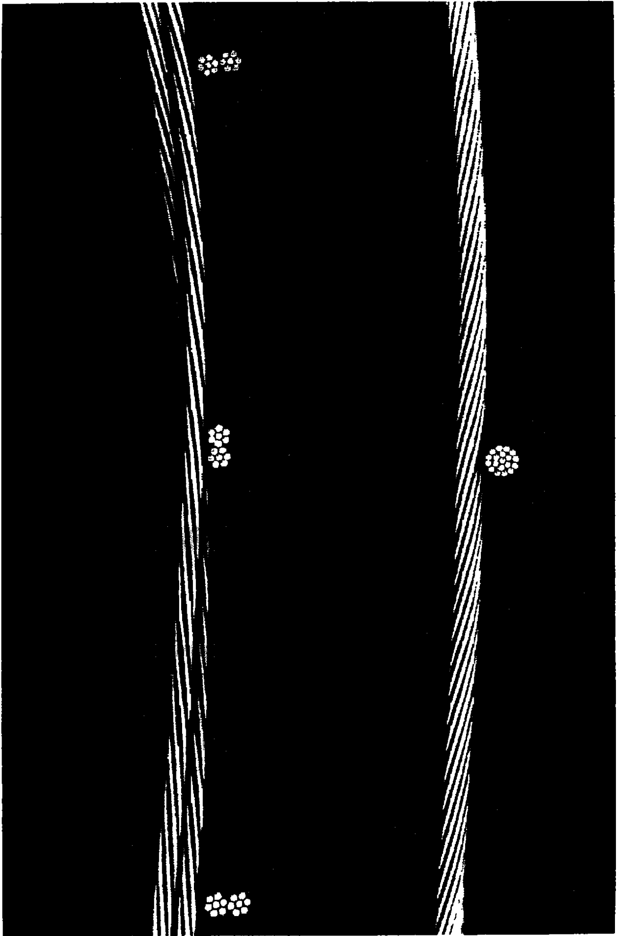
Figure 9.22. Cross-sectional comparison of round conductor and equivalent T_2 conductor, showing continually changing profile of T_2 . (Courtesy of Kaiser Aluminum.)
