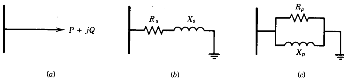
Figure 2.5. Load representations as: (a) real and reactive powers; (b) constant impedance in terms of series combination; (c) constant impedance in terms of parallel combination.
