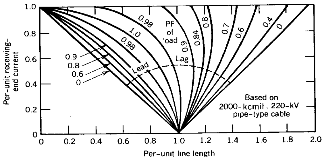
Figure 2.51. Receiving-end current limits of high-voltage ac cable lines. Curved lines: Sending-end current equal to rated or base current of cable. (From Ref. 12. Used by permission. © 1956 IEEE.)
