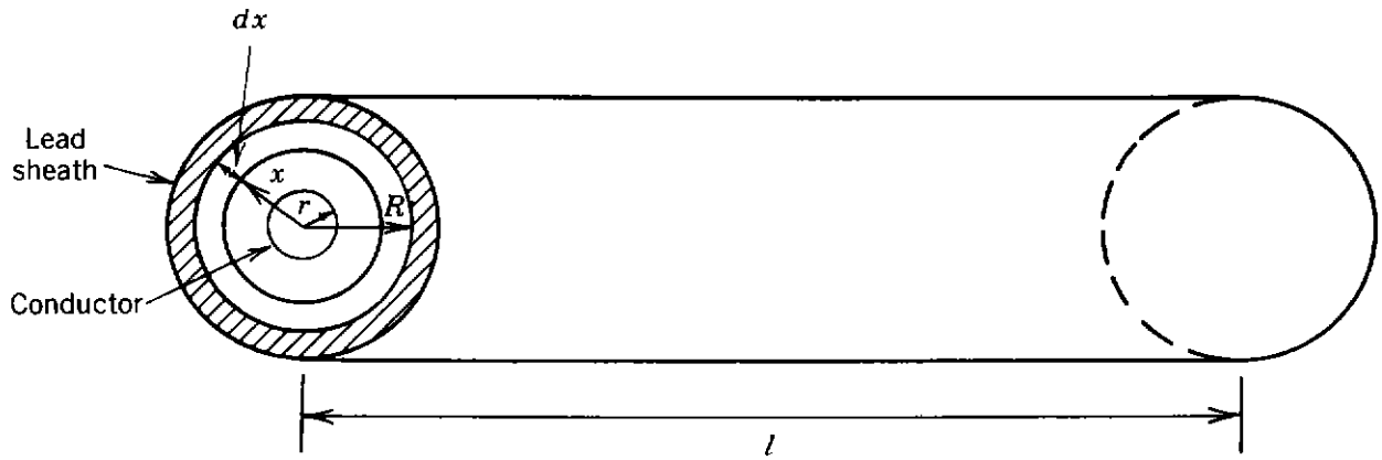
Figure 4.12. Cross section of single-conductor cable.
