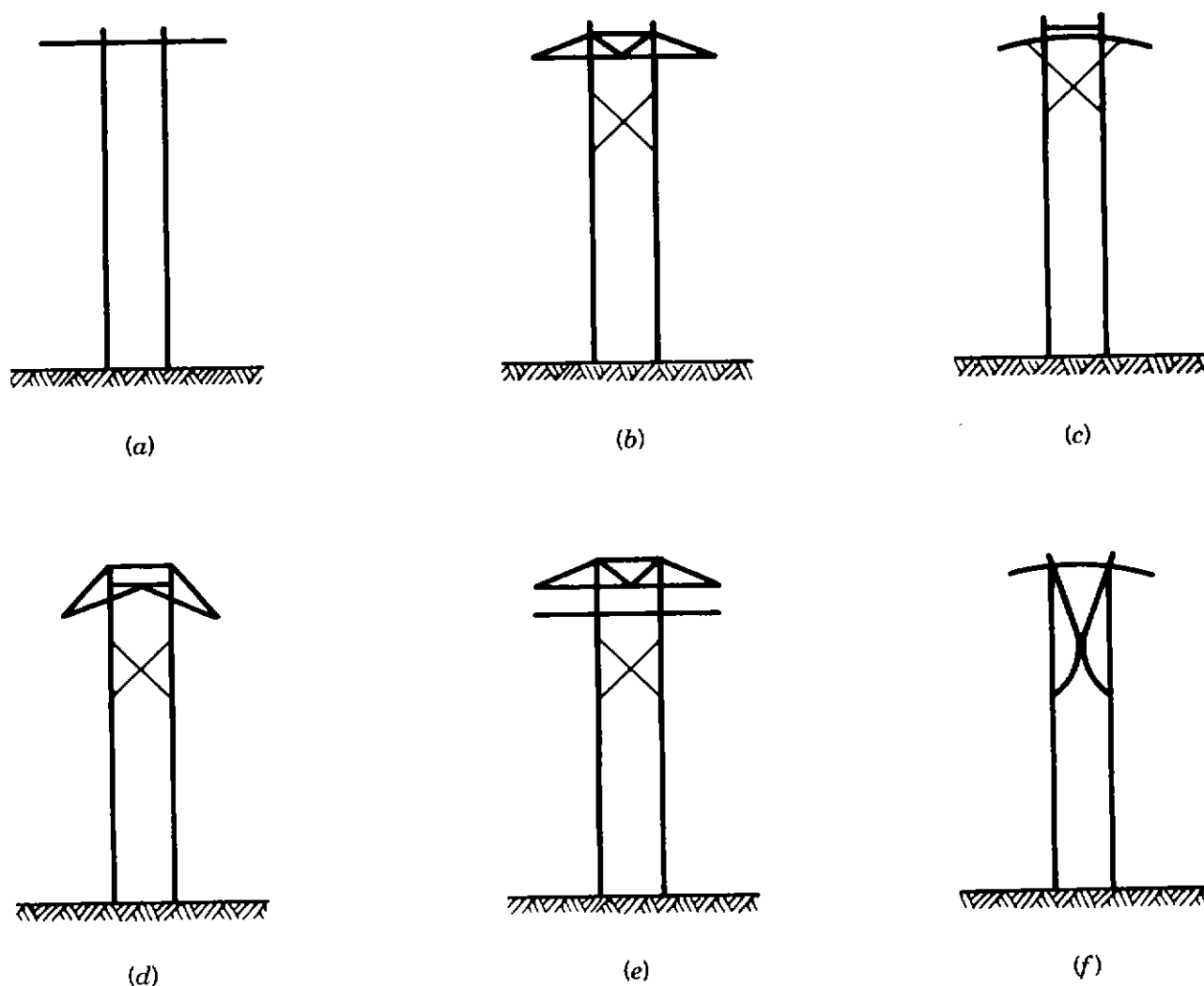
Figure 9.8. Typical two-column designs: (a) unbraced H-frame; (b) H-frame with wood (solid or laminated) cross-arm; (c) H-frame with curved laminated cross-arm; (d) K-frame; (e) double-circuit H-frame; (f) Dreyfus design.
