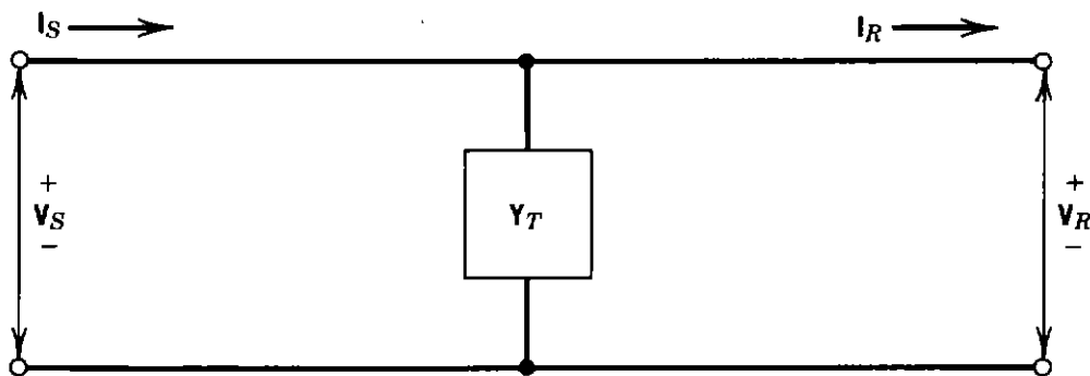
Figure 2.39. Transformer equivalent circuit at no load.
