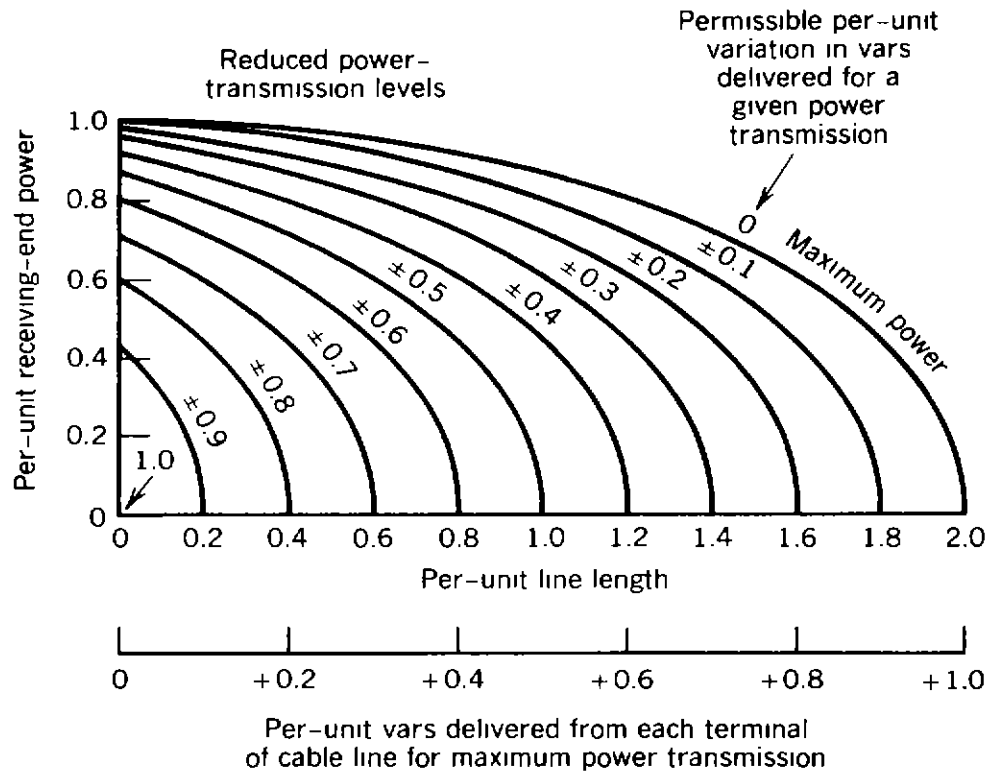
Figure 2.52. Permissible variations in per-unit vars delivered to electric system at each terminal of ac cable line for given power transmission. (From Ref. 12. Used by permission. © 1956 IEEE.)
