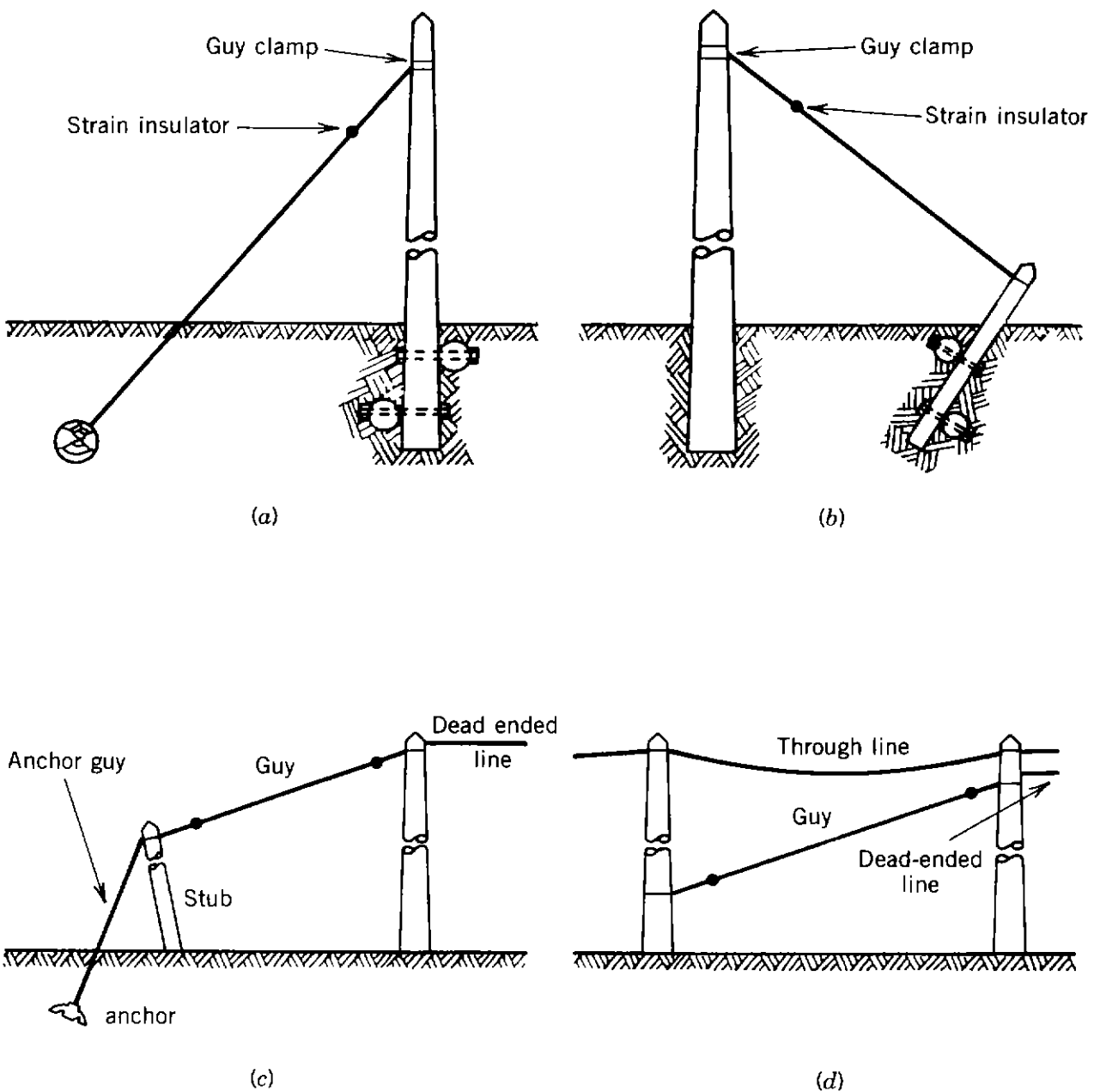
Figure 9.14. Various guying techniques: (a) anchor guy; (b) stub guy; (c) pole-to-stub-to-anchor guy; (d) pole-to-pole guy.
