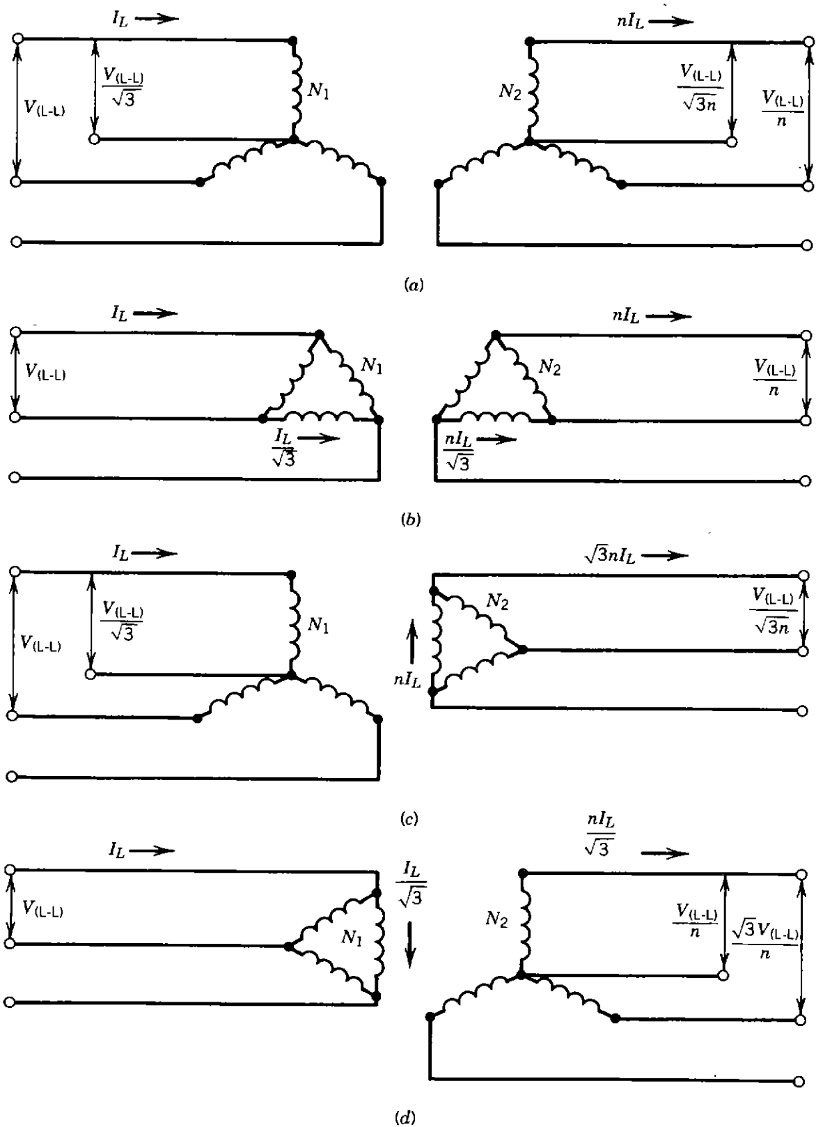
Figure 2.3. Conventional three-phase transformer connections: (a) wye-wye connection; (b) delta-delta connection; (c) wye-delta connection; (d) delta-wye connection.
