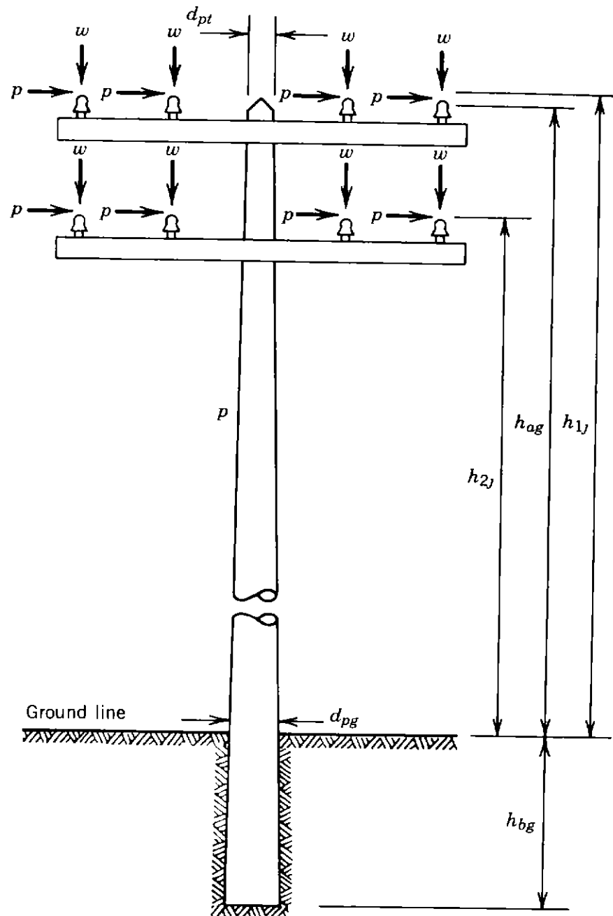
Figure 9.10. Schematic of pole with two cross-arms (not to scale).
