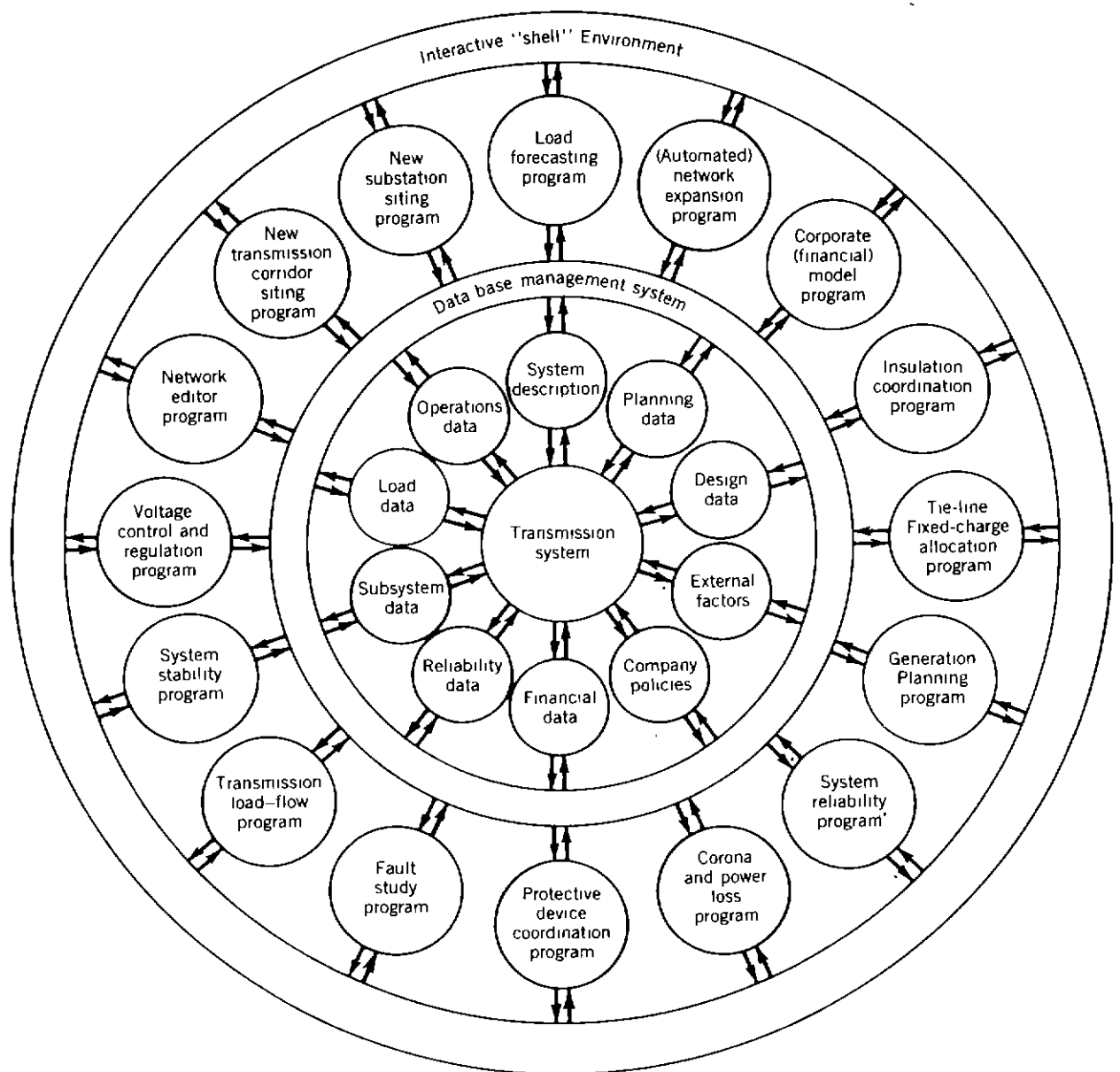
Figure 1.7. Block diagram of transmission system planning process in future.
