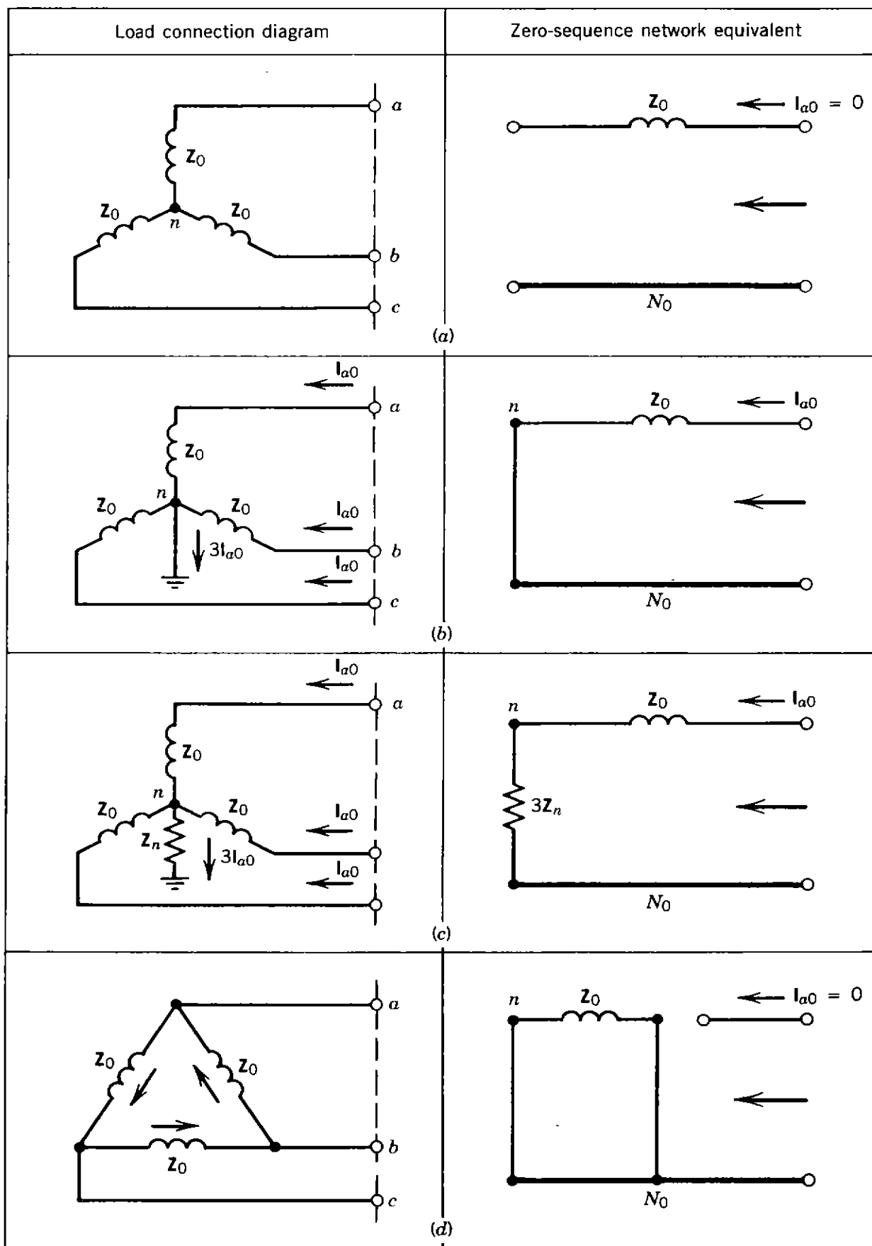
Figure 3.9. Zero-sequence network for wye- and delta-connected three-phase loads: (a) wye-connected load with undergrounded neutral; (b) wye-connected load with grounded neutral; (c) wye-connected load grounded through neutral impedance; (d) delta-connected load.
