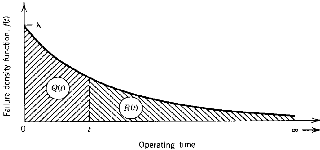
Figure 6.19. Relationship between reliability and unreliability.
