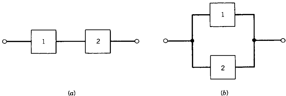
Figure 6.20. Block diagrams of system with two components: (a) connected in series; (b) connected in parallel.
