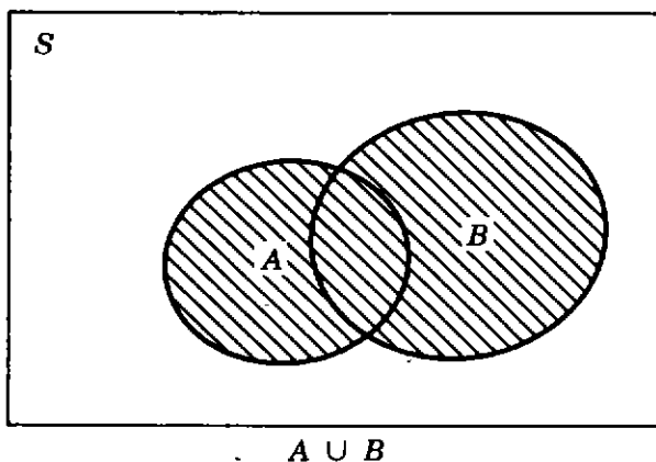
Figure 6.9. Union, A \cup B .
