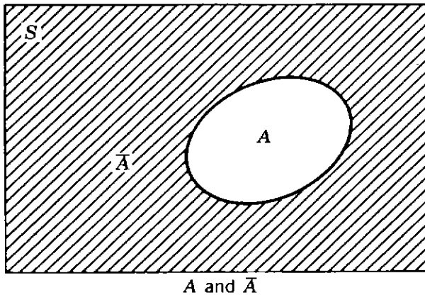
Figure 6.11. Complement set, \bar{A} .
