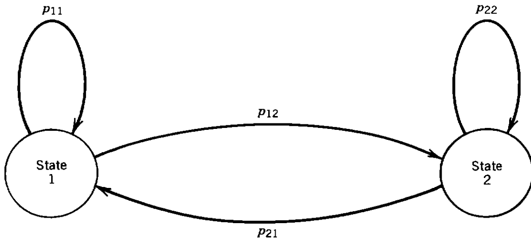
Figure 6.23. Transition diagram for two-state system.
