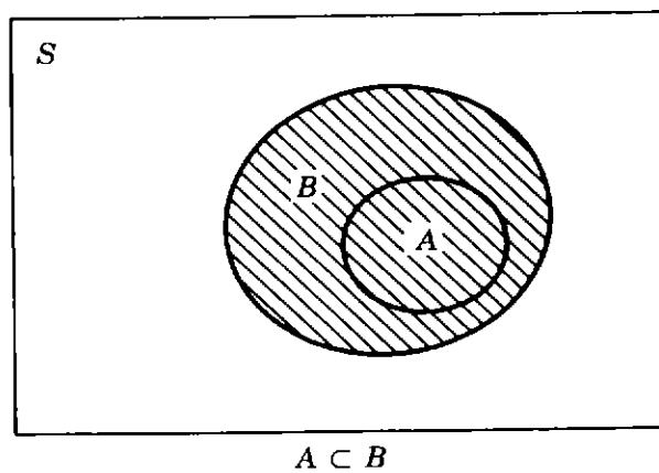
Figure 6.8. Set–subset relationship.
