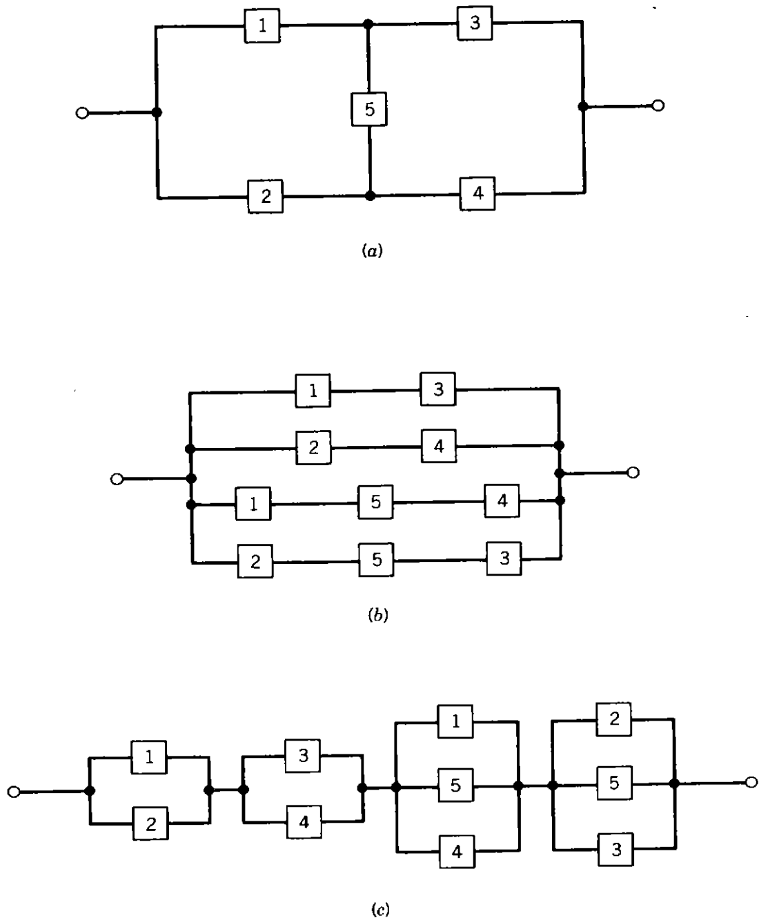
Figure 6.22. Reliability block diagrams showing bridge arrangement and its equivalents: (a) bridge-type network; (b) equivalent minimal-tie diagram; (c) equivalent minimal-cut diagram.
