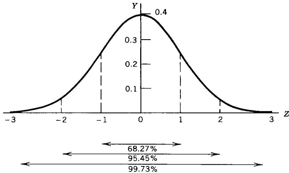
Figure 6.16. Standardized normal curve.
