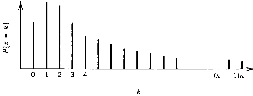
Figure 6.13. Binomial probability distribution with fixed n and p .
