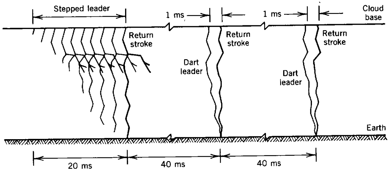
Figure 7.15. Mechanism of lightning flash.
