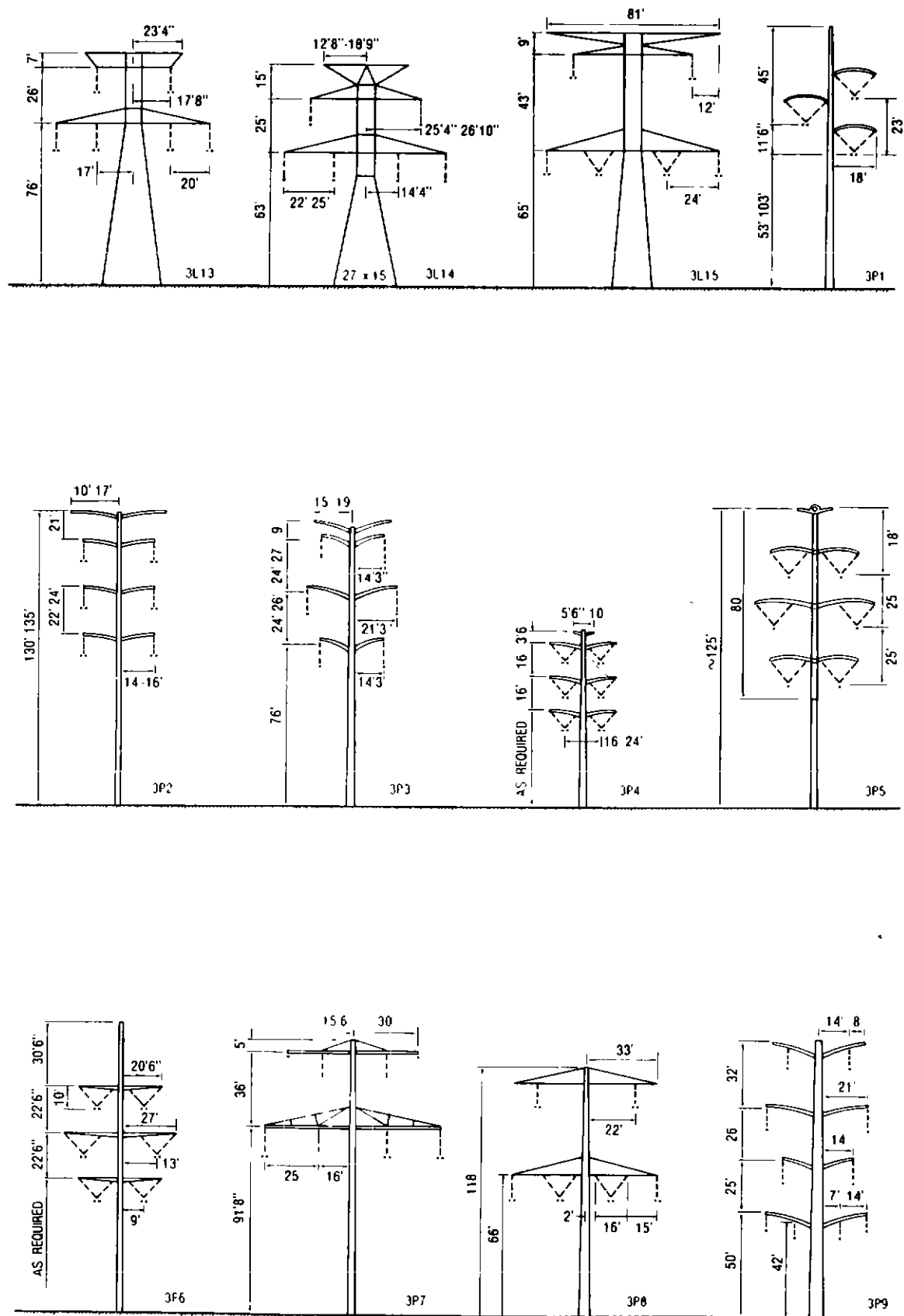
Figure 2.10. Typical pole- and lattice-type structures for 345-kV transmission systems. (Used by permission. © 1979 Electric Power Research Institute.)
