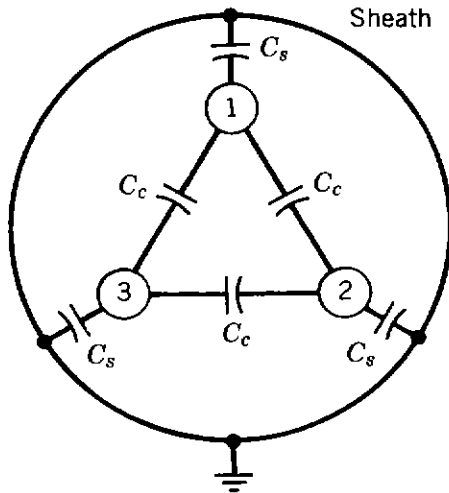
Figure 4.14. Effective capacitances.
