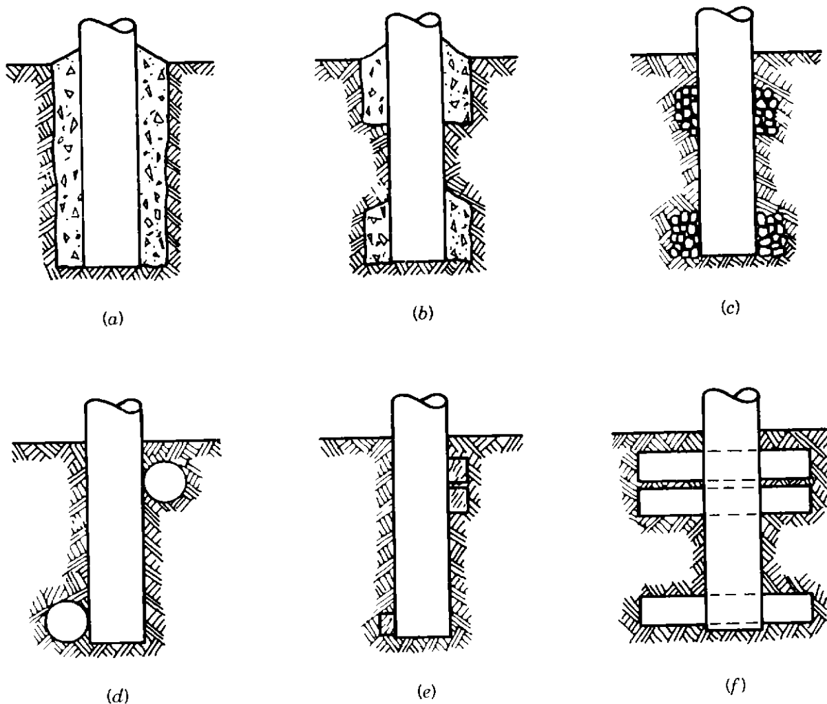
Figure 9.9. Setting techniques: (a) full-concrete setting; (b) concrete setting; (c) crushed stone setting; (d) plain earth setting; (e) heel-and-breast concrete blocks setting; (f) bolted-timber setting.
