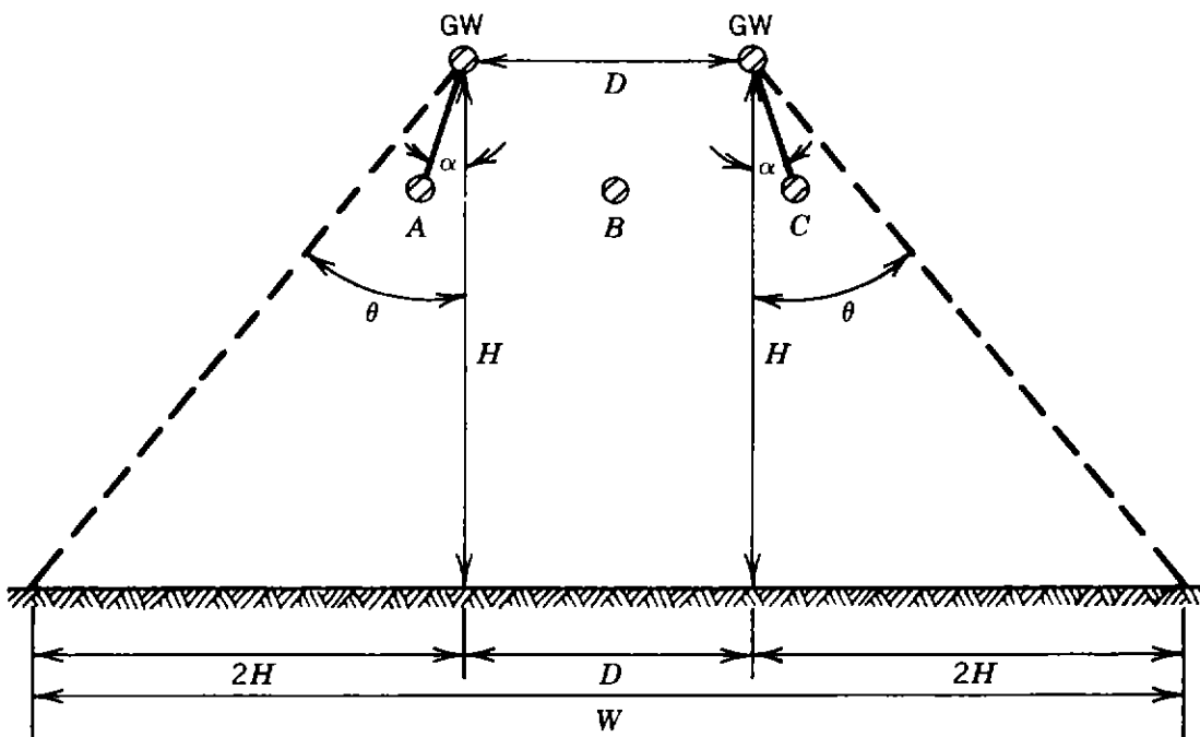
Figure 7.18. Width of right-of-way shielded from lightning strokes.
