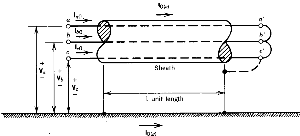
Figure 4.26. Actual circuit of three-conductor lead-sheathed cable.
