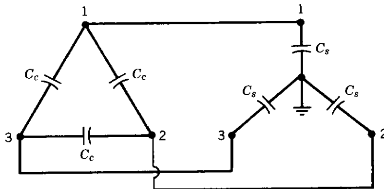
Figure 4.15. Equivalent circuit.
