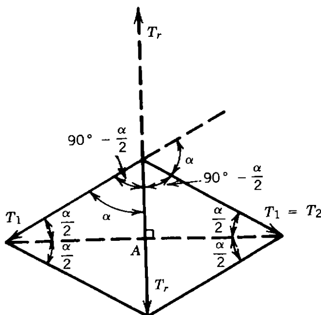
Figure 9.12. Plan view of angle pole and diagram of forces.
