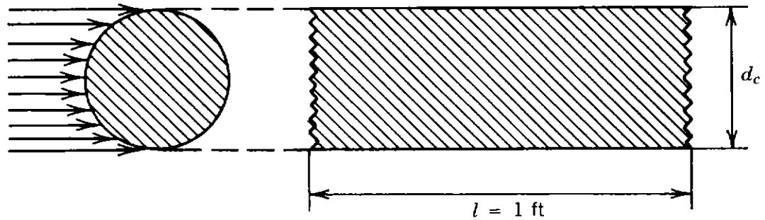
Figure 10.9. Force of wind on conductor covered with no ice.
