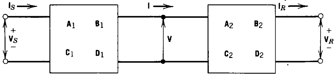
Figure 2.43. Transmission networks in series.
