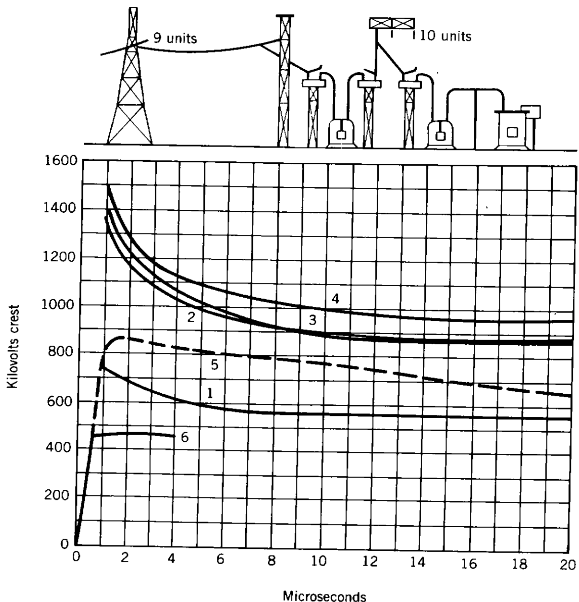
Figure 7.24. Insulation coordination in 138-kV substation for 1.5 \times 40\text{-}\mu\text{s} wave: (1) transformer with 550-kV BIL; (2) line insulation of 9 suspension units; (3) disconnect switches on 4 apparatus insulators; (4) bus insulation of 10 suspension units; (5) maximum 1.5 \times 40\text{-}\mu\text{s} wave permitted by line insulation; (6) discharge of 121-kV arrester for maximum 1.2 \times 40\text{-}\mu\text{s} full wave [16].
