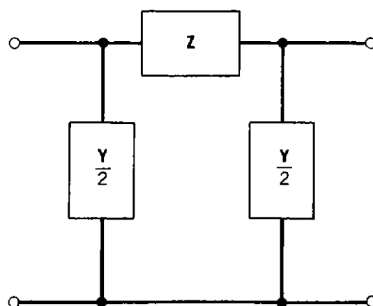
Figure 2.34. Nominal- \Pi circuit.
