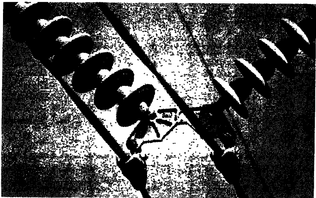
Figure 9.23. Installation of T_2 conductors. (a) clipping crew installing suspension clamp; (b) typical 345-kV two-conductor suspension clamp and yoke plate arrangement; (c) rigged used to dead end T_2 conductor; (d) strain clamp dead ends. (Courtesy of Kaiser Aluminum.)
