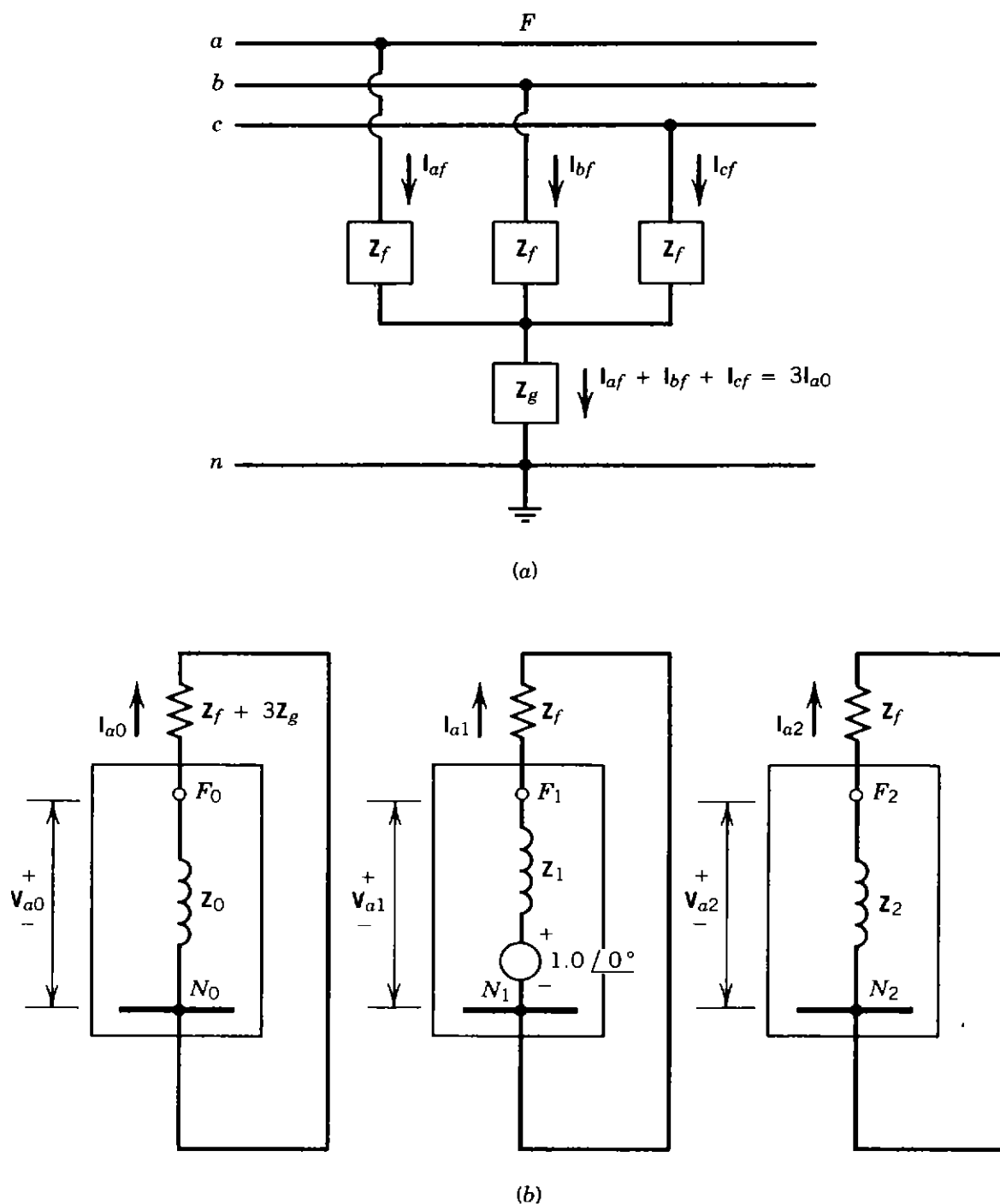
Figure 3.24. Three-phase fault: (a) general representation; (b) interconnection of sequence networks.
