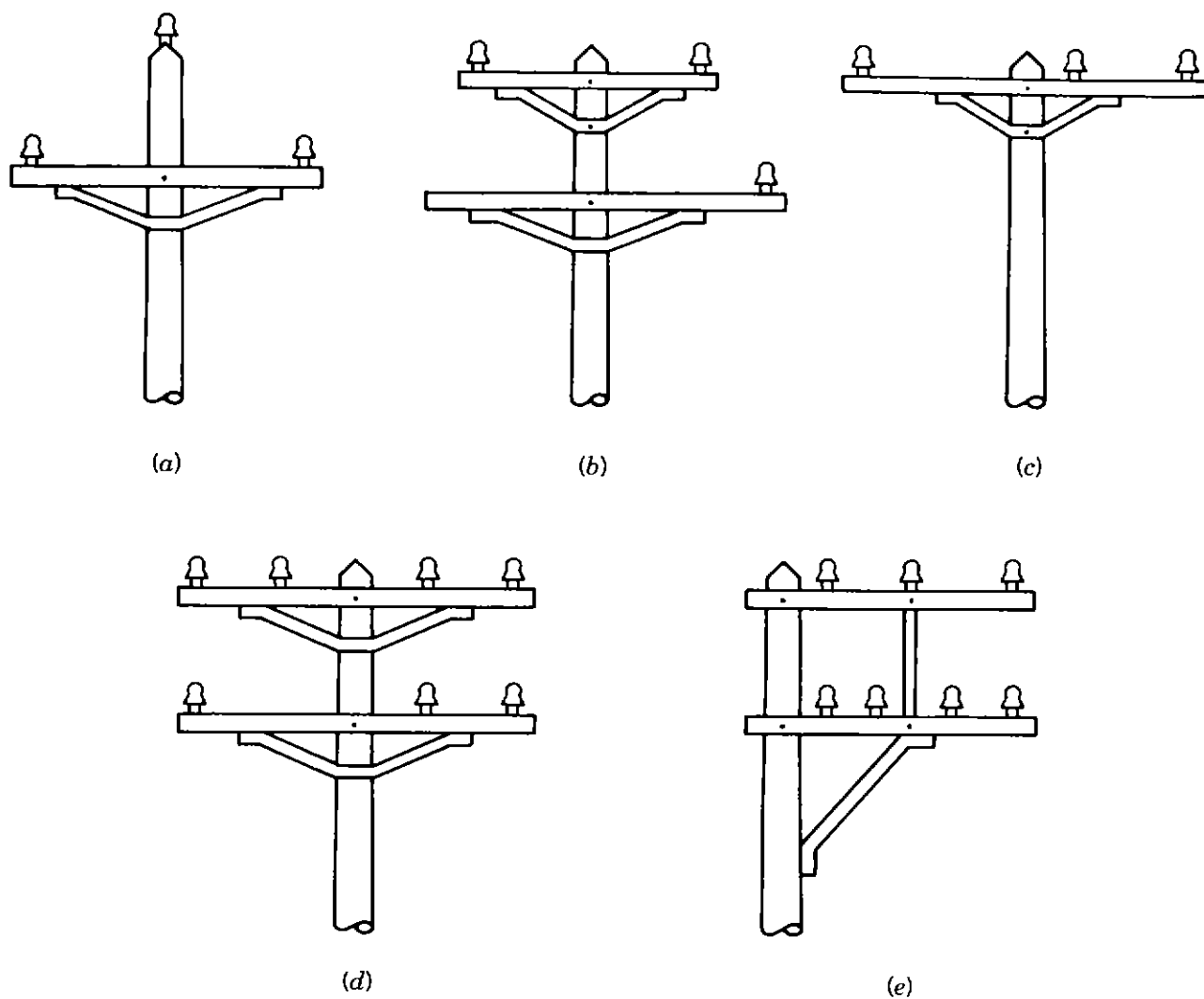
Figure 9.6. Typical single-pole designs used in distribution systems: (a) pole top; (b) two arms; (c) single arm; (d) line arms; (e) side arms.
