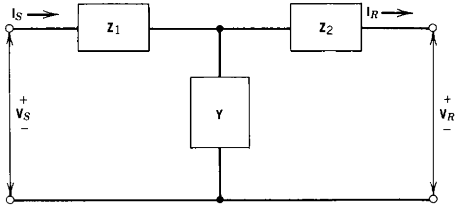
Figure 2.42. Asymmetrical-T network.
