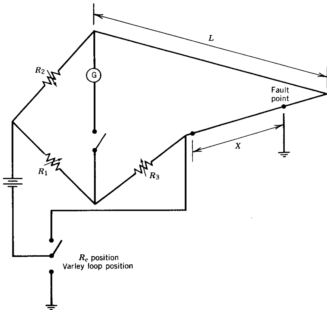
Figure 4.35. Varley loop.
