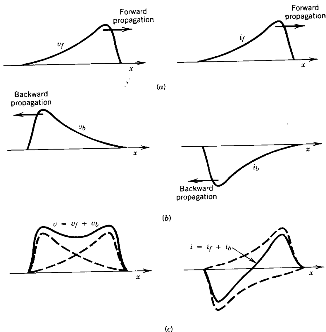
Figure 7.3. Representation of voltage and current waves: (a) in forward direction; (b) in backward direction; (c) superposition of waves.
