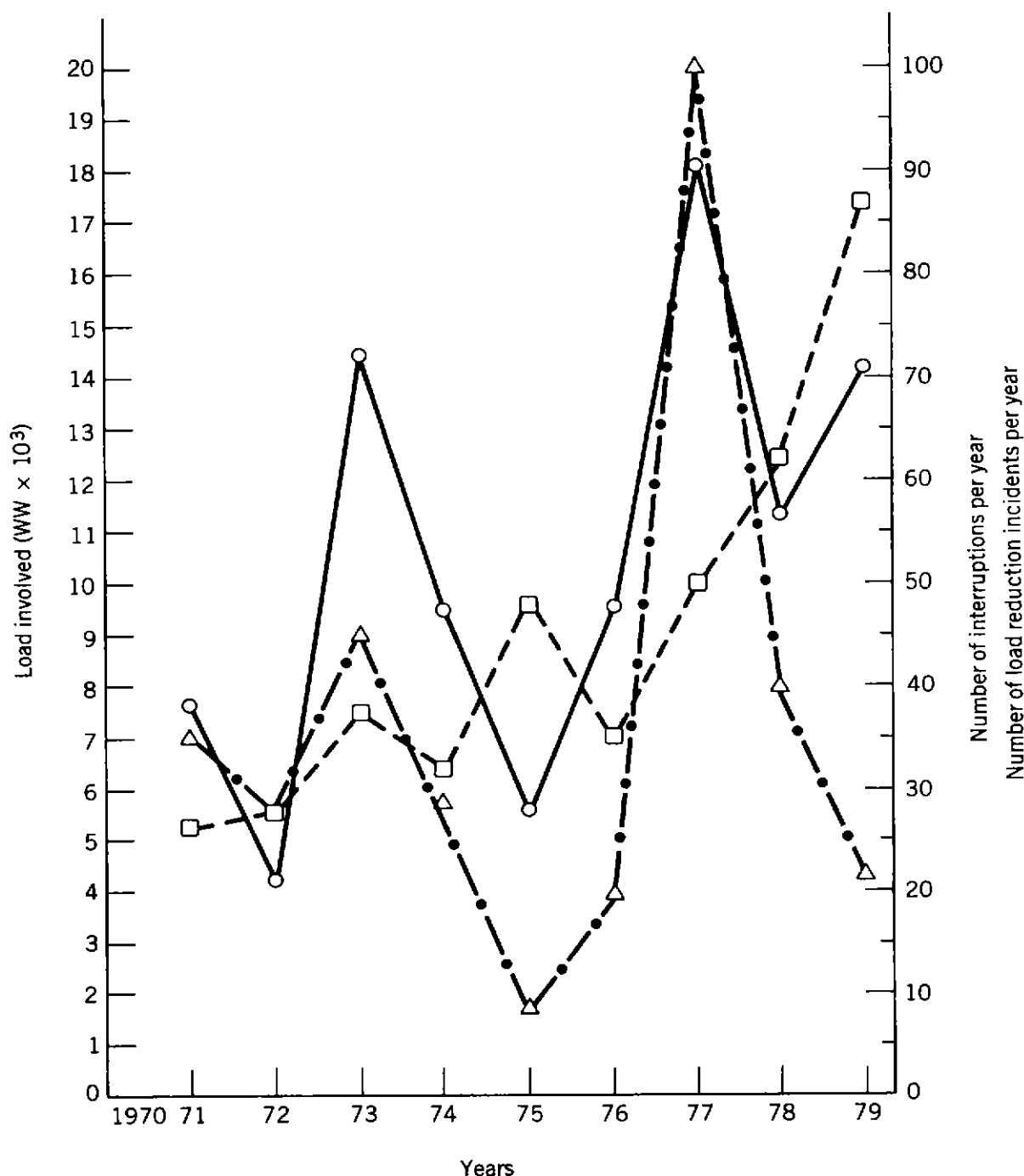
Figure 6.2. Bulk power system interruption data, 1971-1979 [3]: ○—○, load involved ( \times 10^3 MW); □-----□, interruptions per year; \Delta \cdots \cdots \Delta , load reduction incidents per year.
