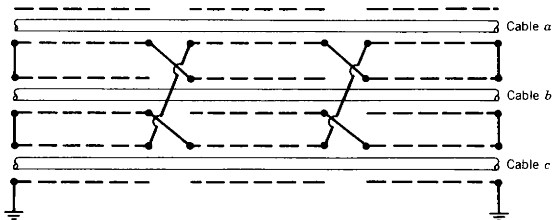
Figure 4.25. Cross bonding of single-conductor cables.
