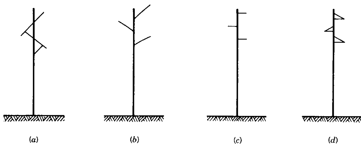
Figure 9.7. Typical single-column designs: (a) wishbone design; (b) unbraced up-swept arms; (c) horizontal line post; (d) braced horizontal arms.
