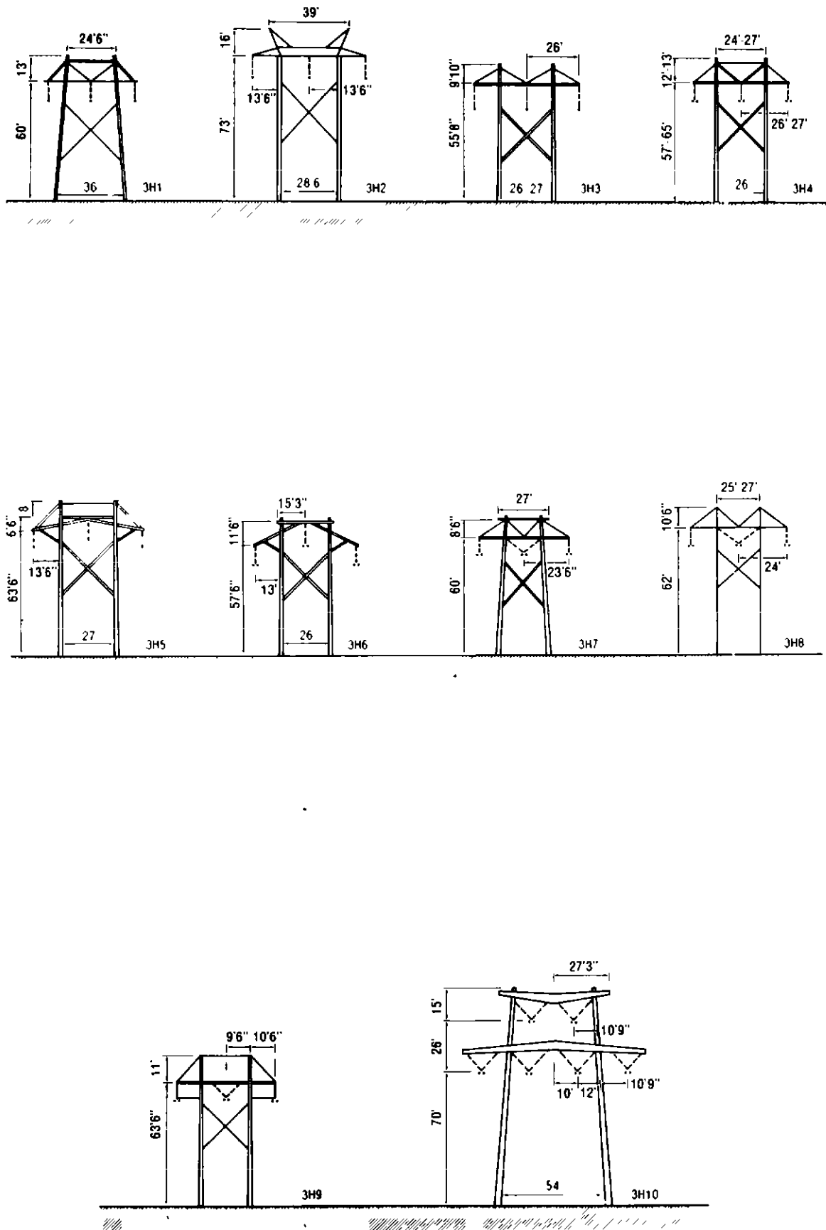
Figure 2.11. Typical wood H-frame-type structures for 345-kV system (From Ref. 14. Used by permission. © 1979 Electric Power Research Institute.)
