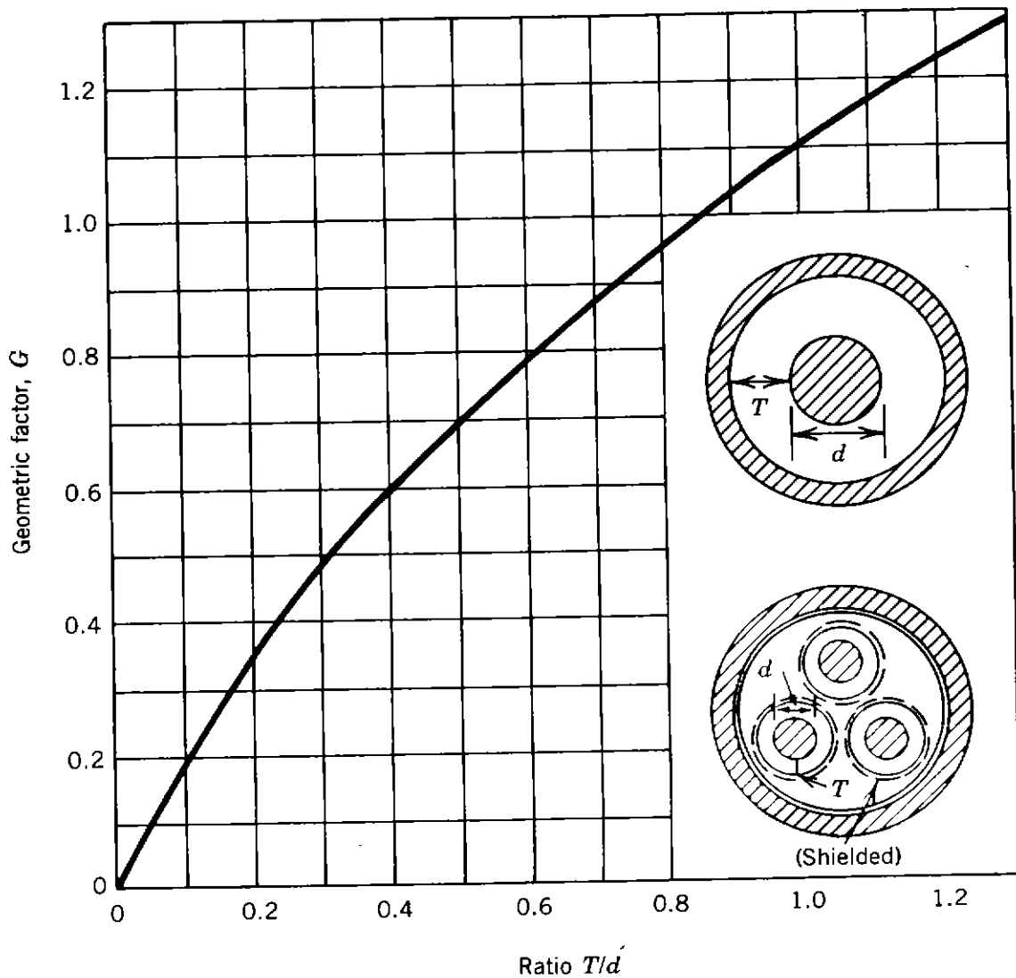
Figure 4.22. Geometric factor for single-conductor cables, or three-conductor shielded cables having round conductors [2].
