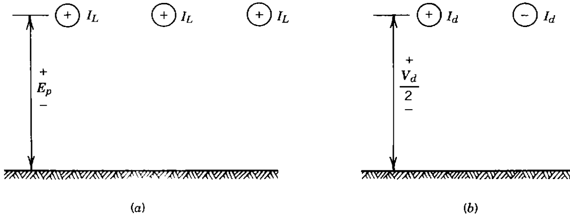
Figure 5.3. Transmission line conductor configuration for high voltage: (a) ac system; (b) dc system.
