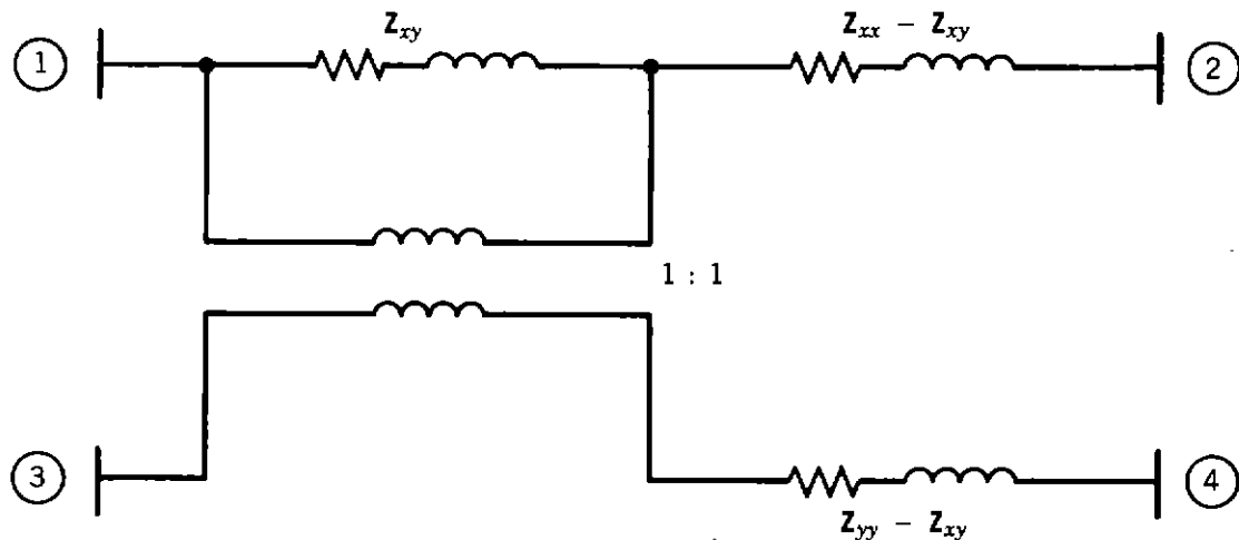
Figure 2.27. Representation of mutual impedance between two circuits by means of 1:1 transformer.
