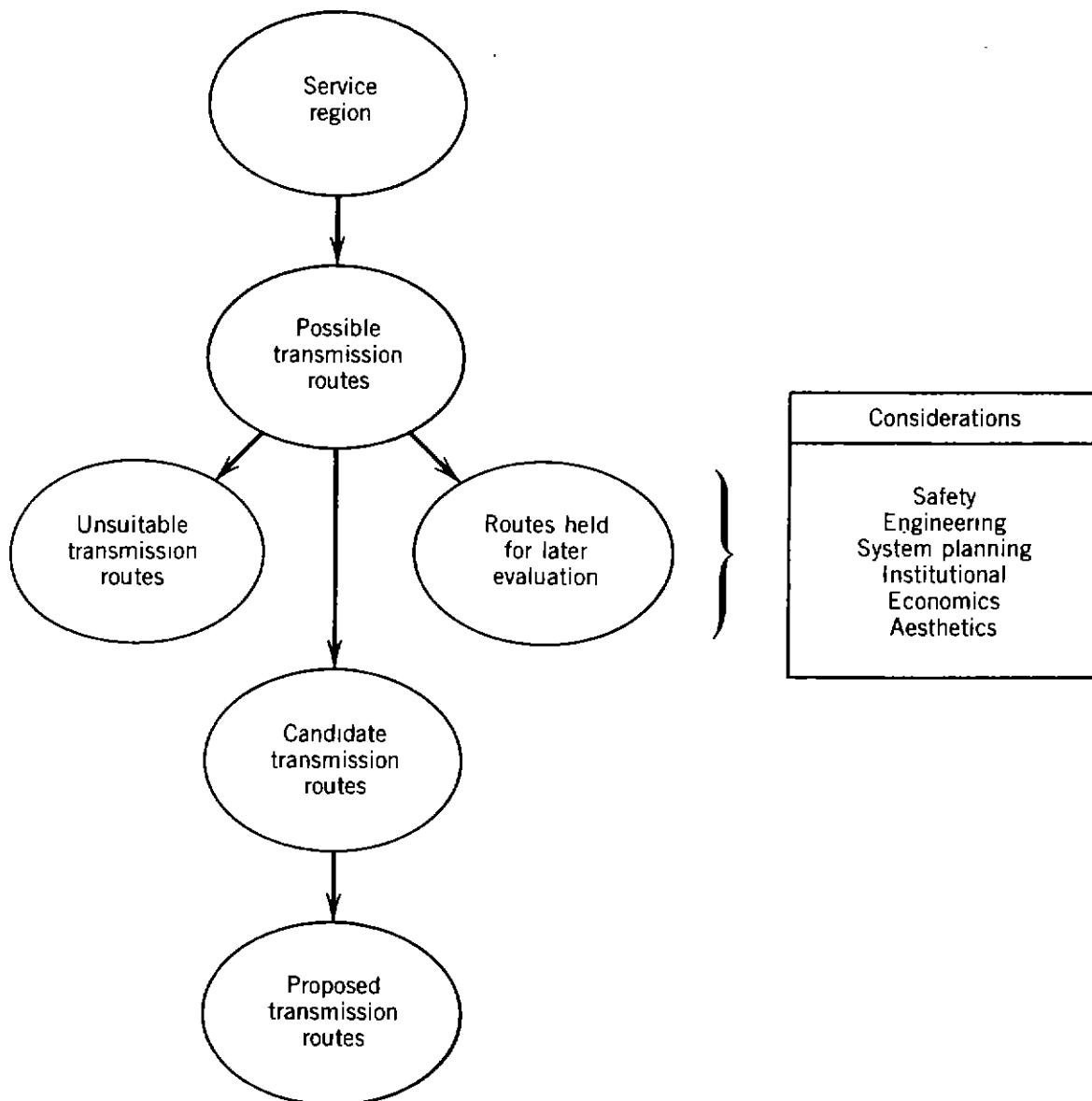
Figure 1.5. Transmission route selection procedure.
