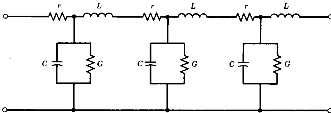
Figure 2.22. Distributed constant equivalent circuit of line.
