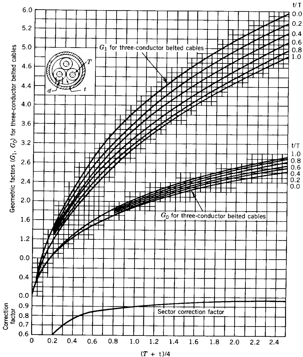
Figure 4.23. Geometric factor for three-conductor belted cables having round or sector conductors.
