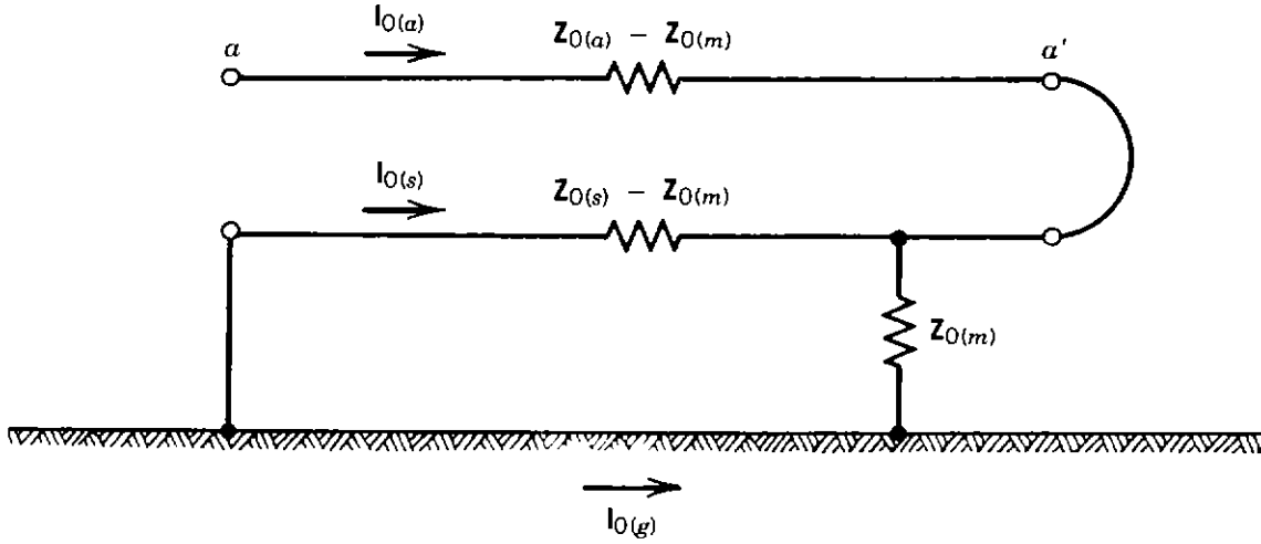
Figure 4.28. Modified equivalent circuit.
