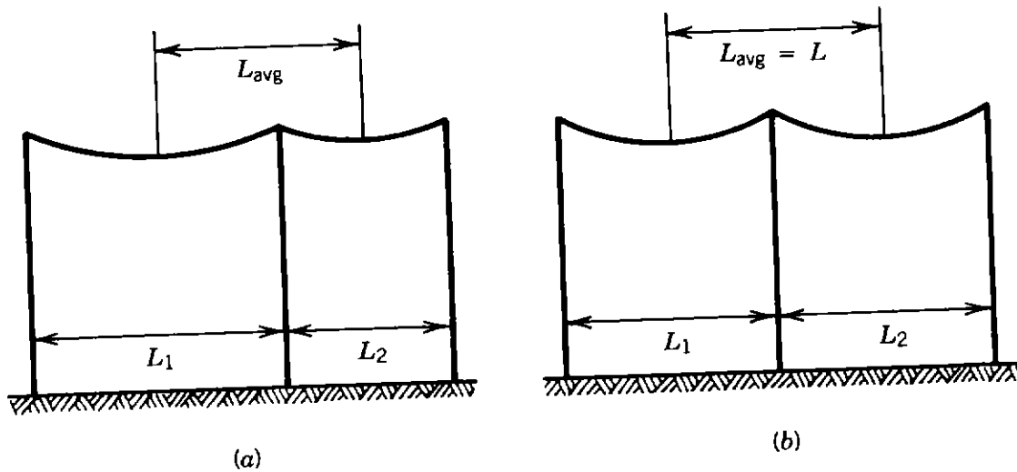
Figure 9.11. Pole-loading diagrams: (a) when two adjacent spans are not equal to each other; (b) when two adjacent spans are equal to each other.
