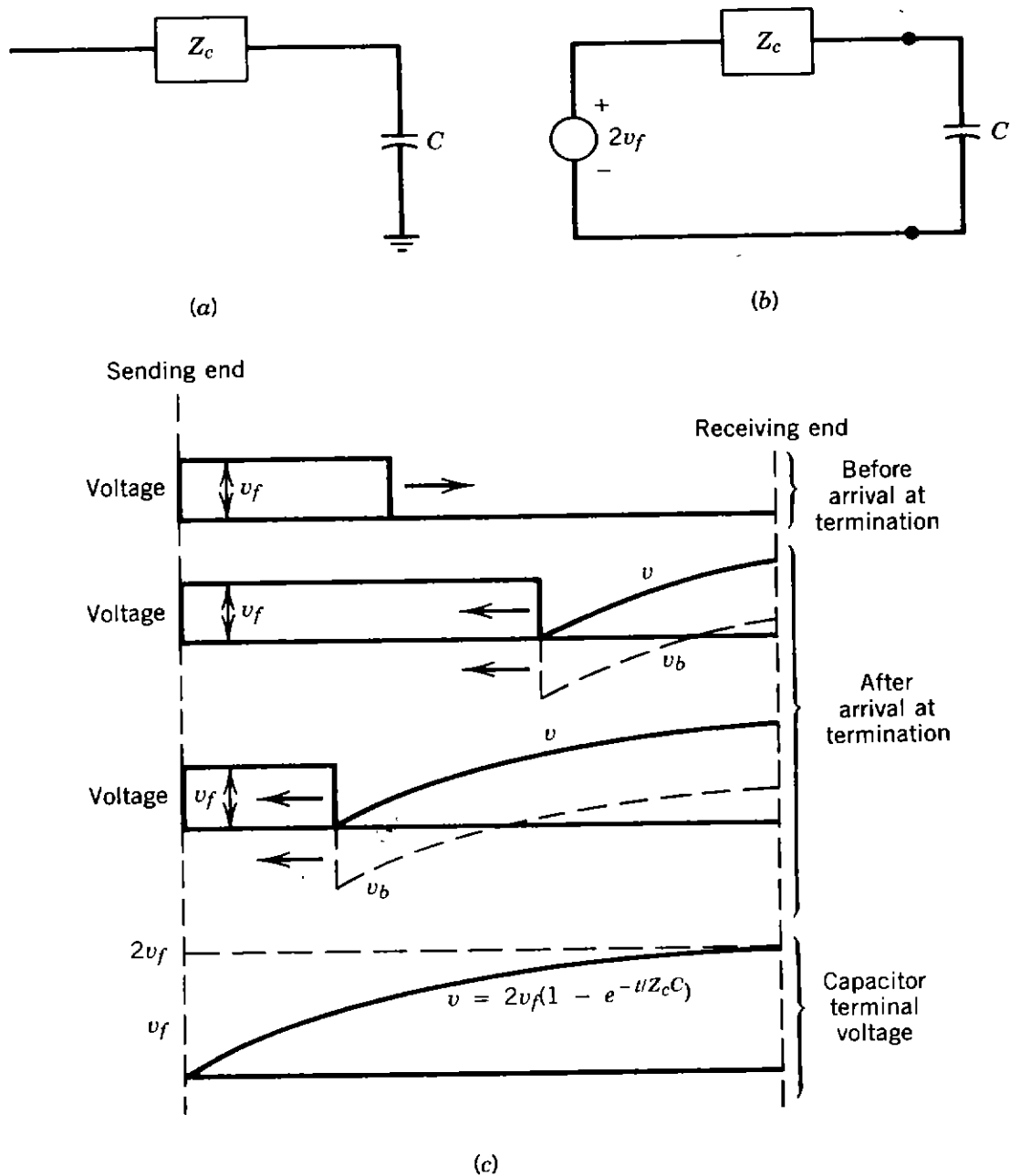
Figure 7.10. Traveling voltage wave on line with capacitive termination: (a) system; (b) equivalent circuit; (c) disposition of wave at various instants.
