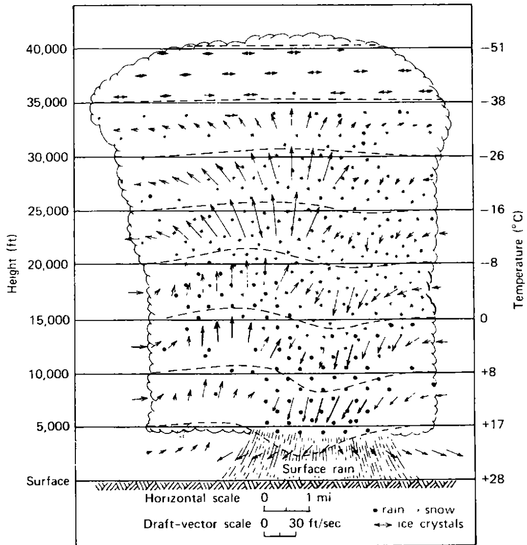
Figure 7.13. Idealized thunderstorm cloud cell in its mature state [20].
