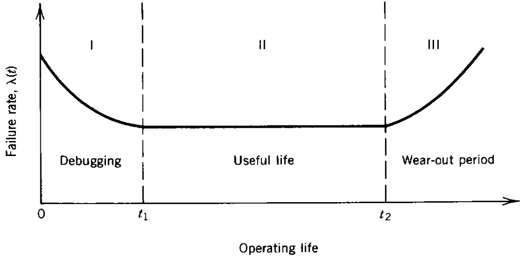
Figure 6.18. Bathtub hazard function.
