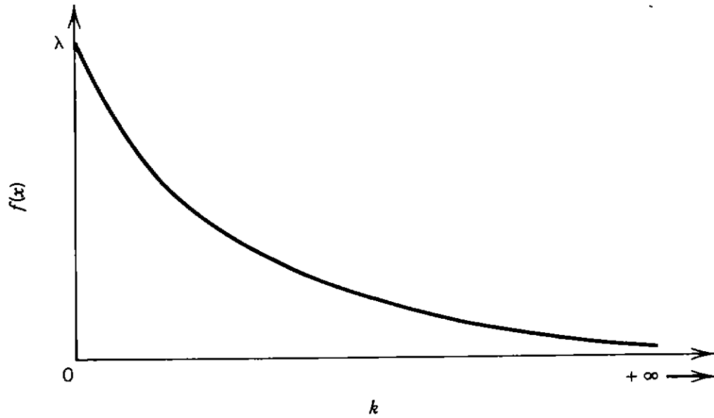
Figure 6.17. Exponential distribution.
