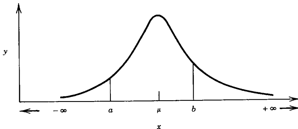
Figure 6.15. Normal probability distribution.
