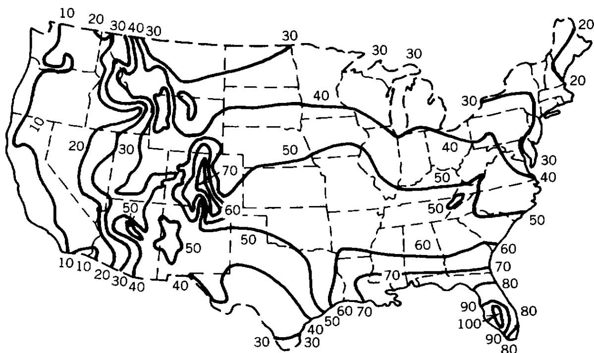
Figure 7.17. Isokeraunic map of United States showing average number of thunderstorm days per year. (U.S. Weather Bureau.)
