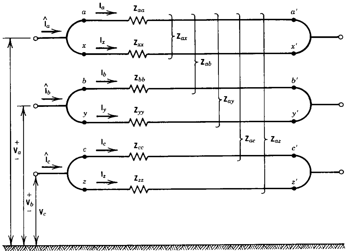
Figure 4.32. Equivalent circuit for bundled parallel cables.
