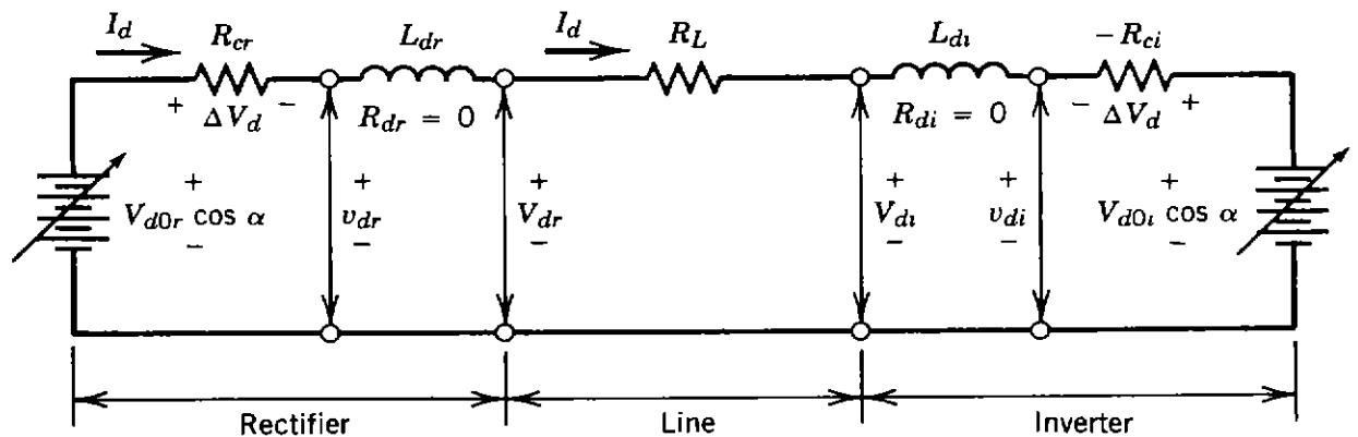
Figure 5.14. Equivalent circuit of dc link.
