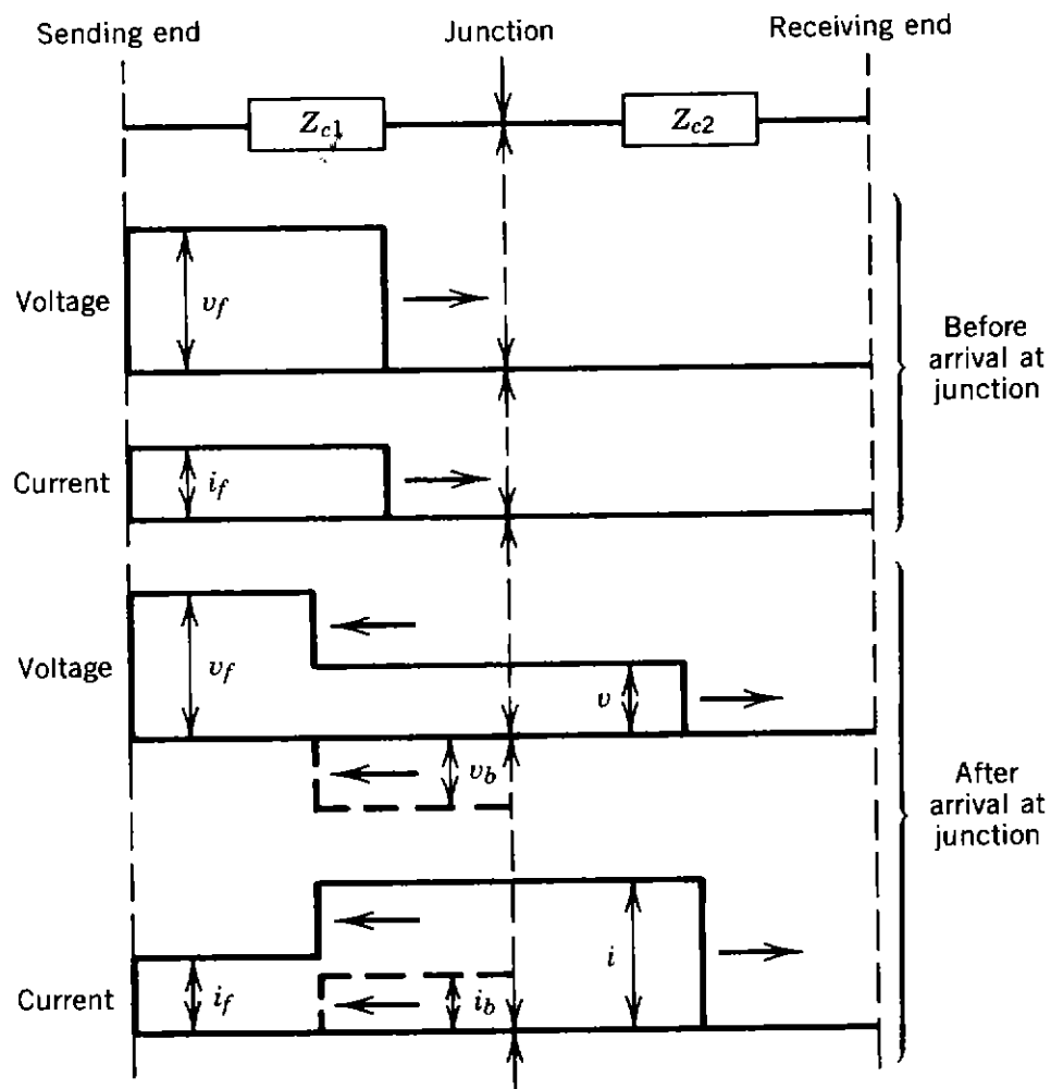
Figure 7.7. Traveling voltage and current waves being reflected and transmitted at junction between two lines.
