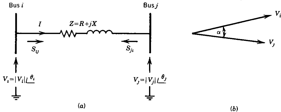
Figure 2.1. Per-phase representation of short transmission line.
