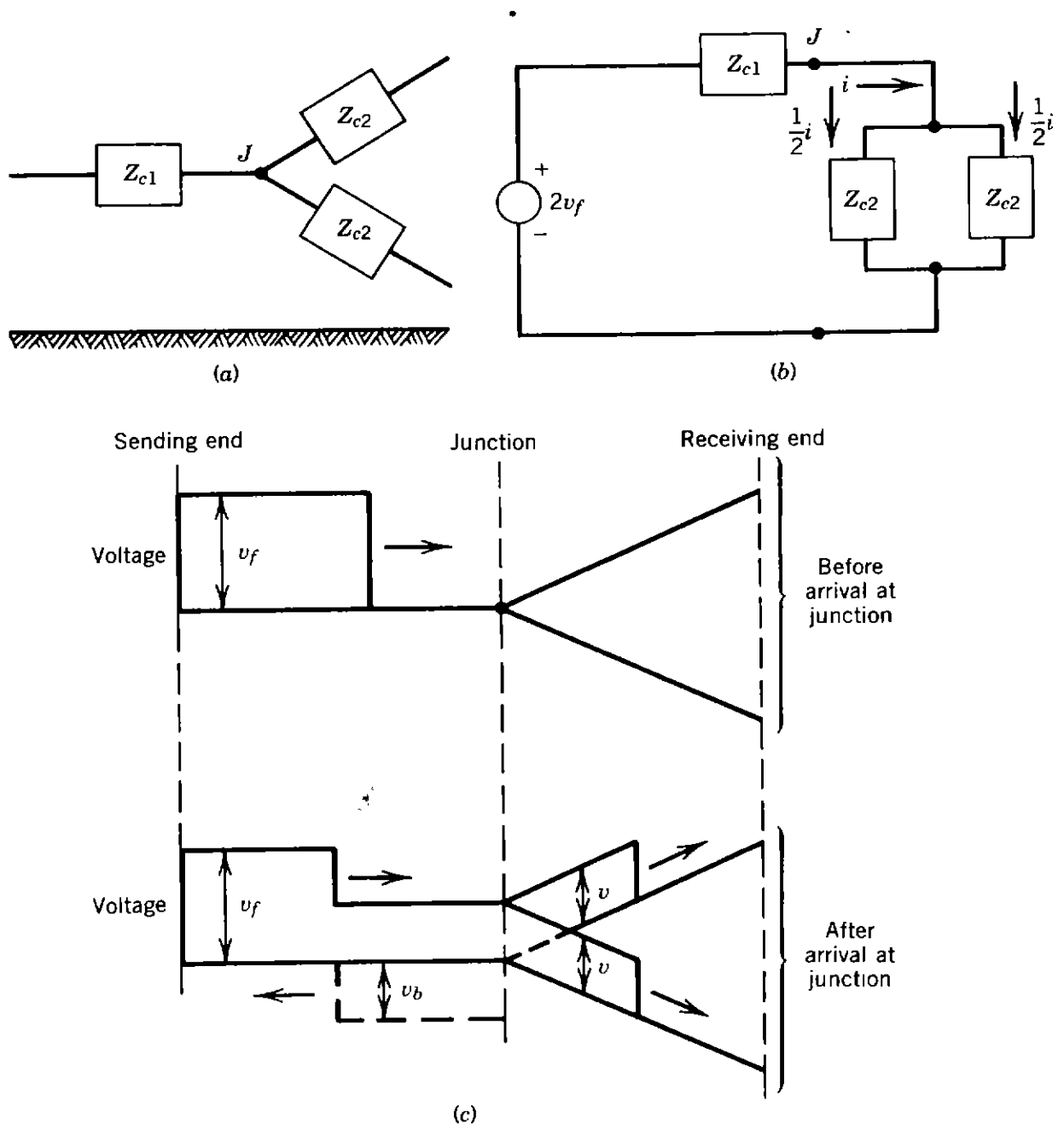
Figure 7.9. Traveling voltage wave encountering line bifurcation: (a) system; (b) equivalent circuit; (c) traveling voltage wave reflected and transmitted at junction of three lines.
