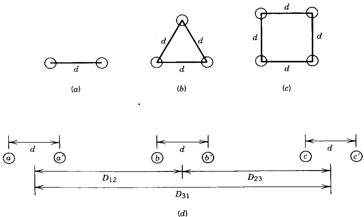
Figure 2.56. Bundle arrangements: (a) two-conductor bundle; (b) three-conductor bundle; (c) four-conductor bundle; (d) cross section of bundled-conductor three-phase line with horizontal tower configuration.
