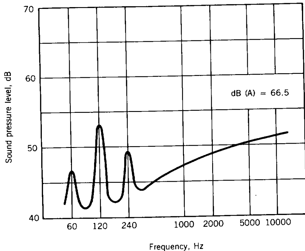
Figure 8.12. Audible noise frequency spectrum during rain (1/10 octave bandwidth dB above 0.0002 \mu bar General Radio meter) of a UHV line 4 \times 2 -in. bundle. (From Ref. 27. Used with permission. © 1971 IEEE.)
