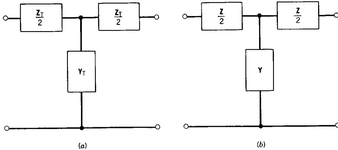
Figure 2.35. The T circuits: (a) equivalent T; (b) nominal T.
