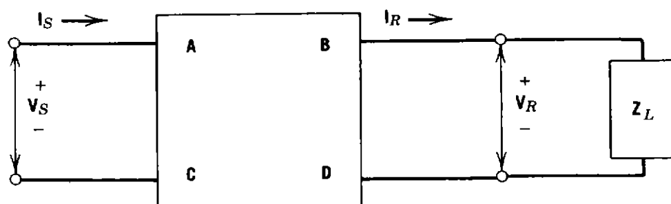
Figure 2.47. Terminated transmission line.
