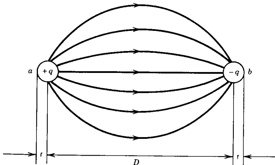
Figure 2.18. Capacitance of single-phase line.
