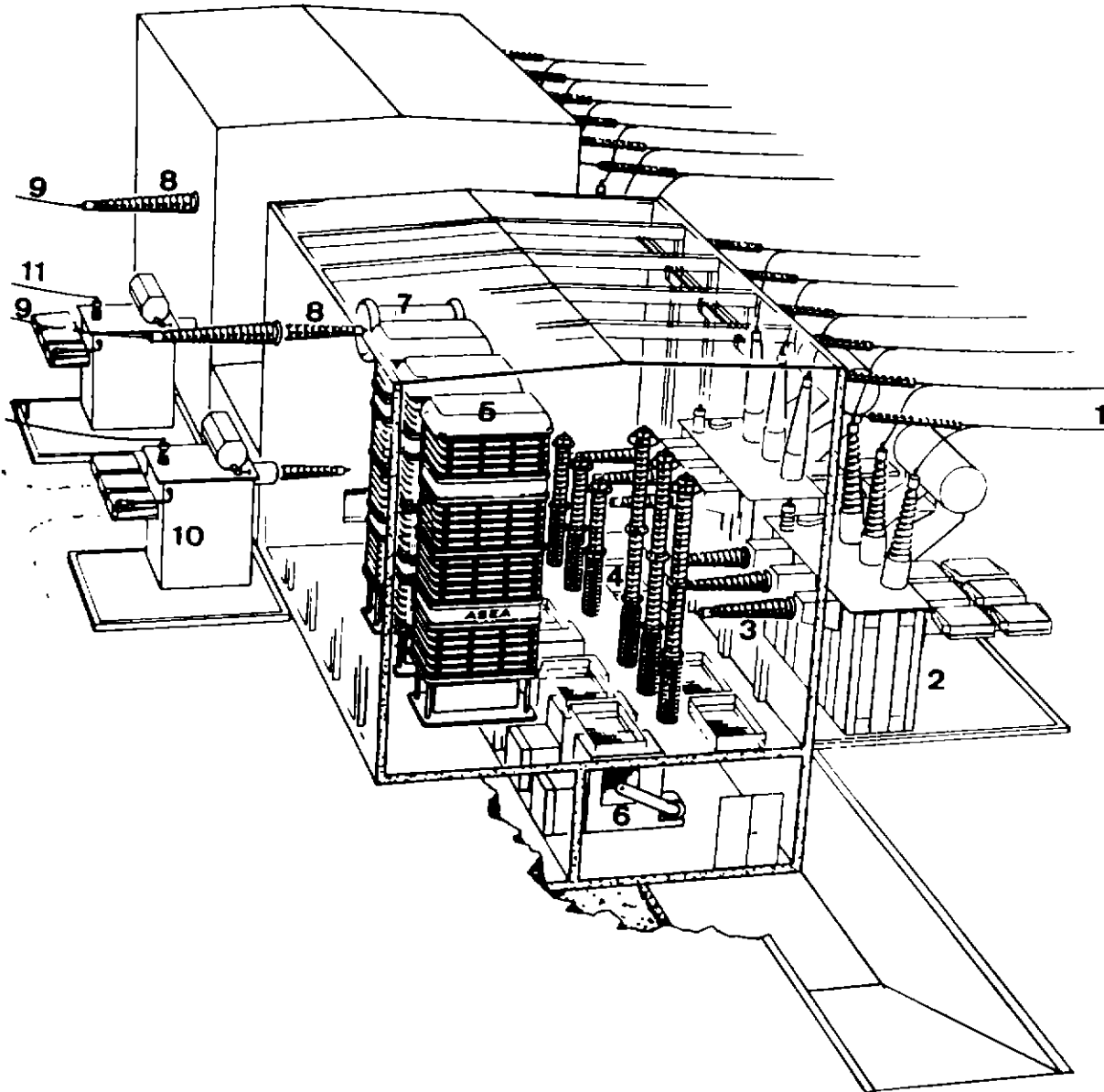
Figure 5.11. General arrangement of converter station with 12-pulse converters: (1) ac busbar; (2) converter transformer; (3) valve-side bushing of converter transformer; (4) surge arresters; (5) quadruple valves; (6) valve-cooling fans; (7) air core reactor; (8) wall bushing; (9) outgoing dc buswork; (10) smoothing reactor; (11) outgoing electrode line connection [2].
