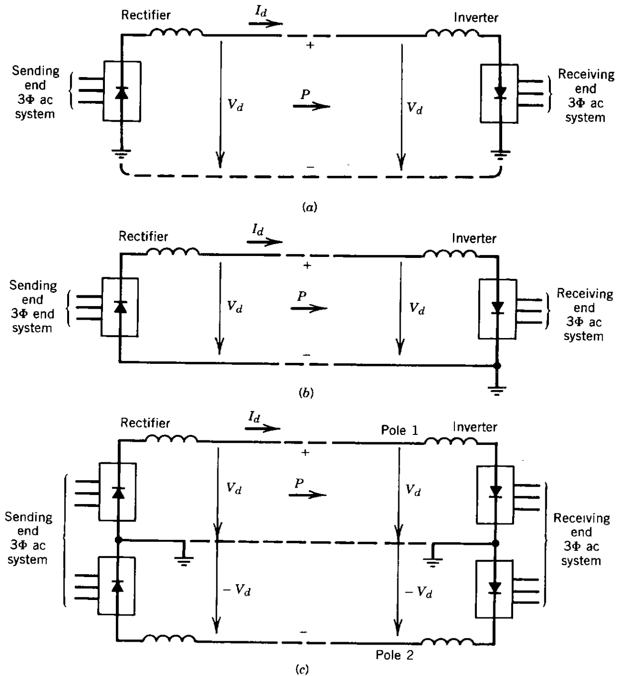
Figure 5.1. Typical circuit arrangements for high-voltage dc transmissions: (a) monopolar arrangement with ground return; (b) monopolar arrangement with metallic return grounded at one end; (c) bipolar arrangement.
