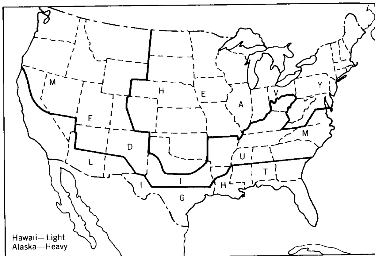
Figure 10.13. NESC's general loading map of United States with respect to loading of overhead lines.
