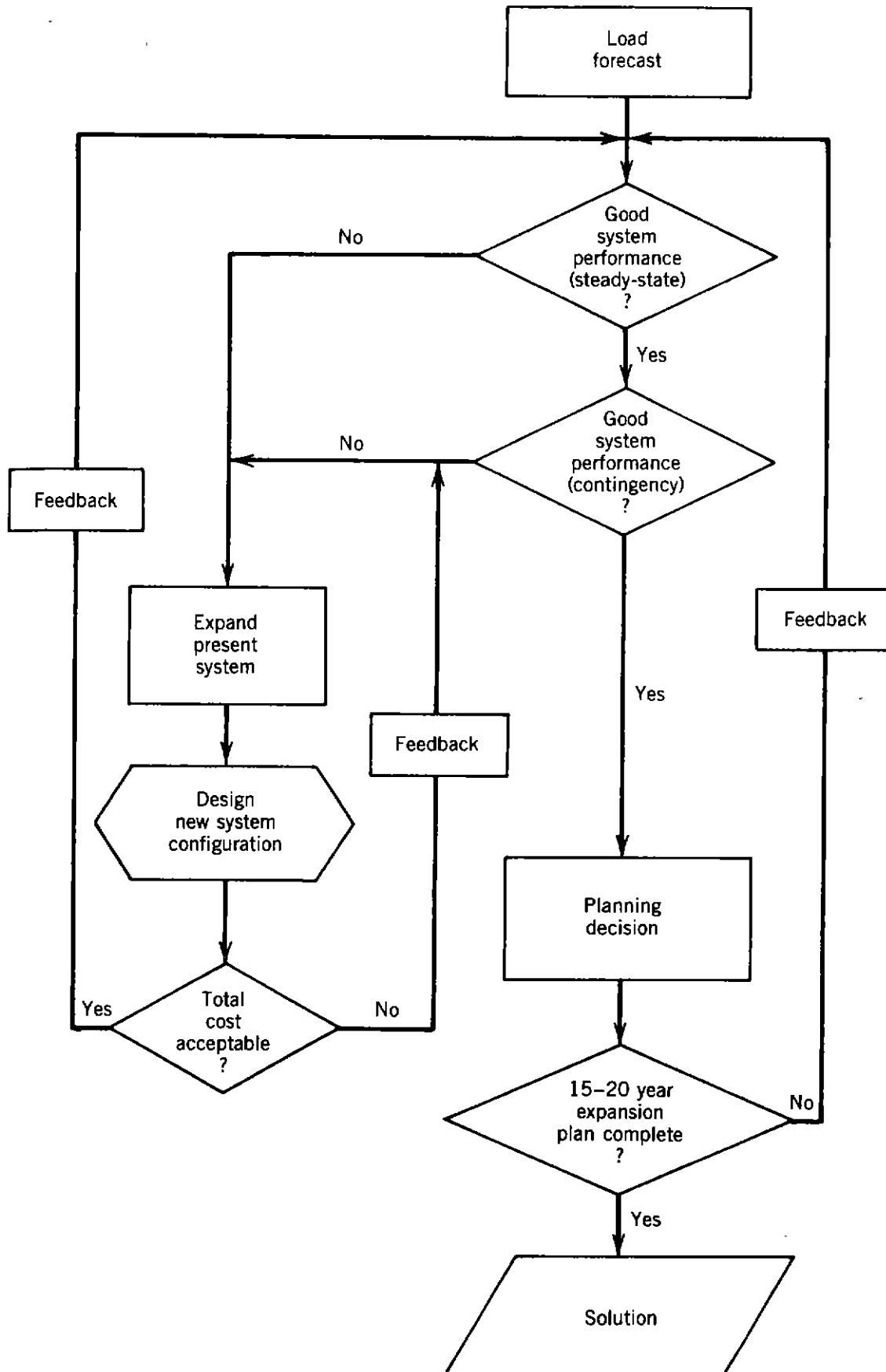
Figure 1.3. Block diagram of typical transmission system planning process.
