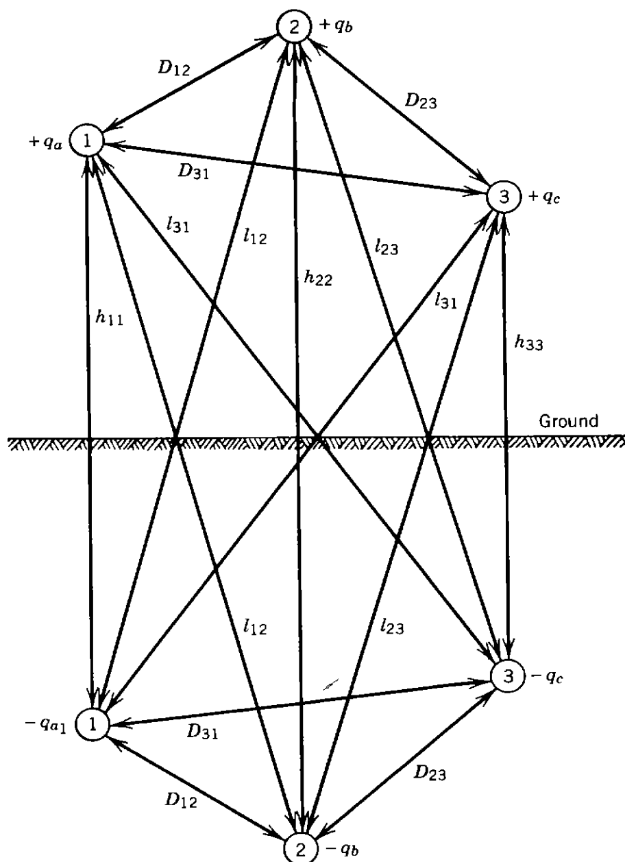
Figure 2.57. Three-phase line conductors and their images.
