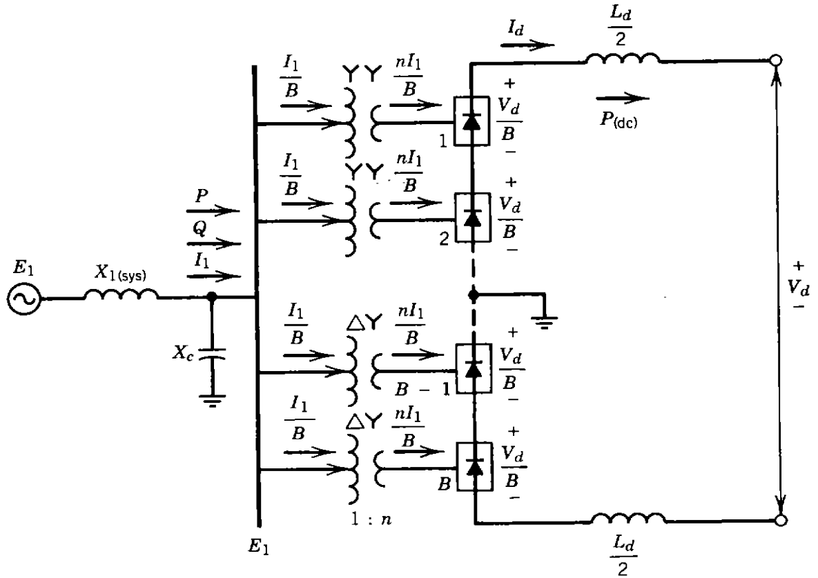
Figure 5.12. One-line diagram for B-bridge converter (rectifier) station.
