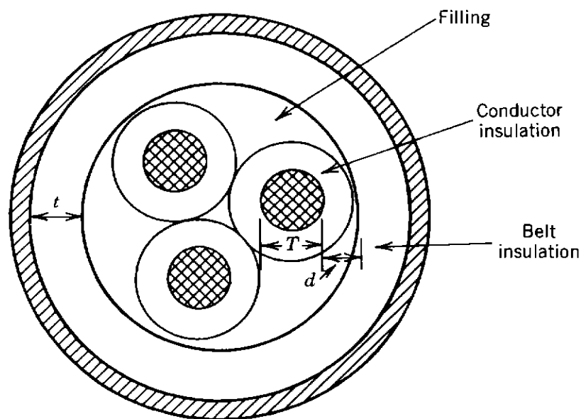
Figure 4.13. Three-conductor belted cable cross section.
