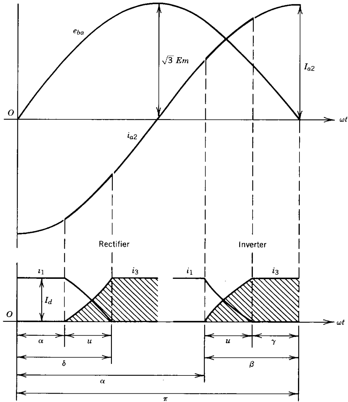
Figure 5.7. Relations among angles used in converter theory [1].
