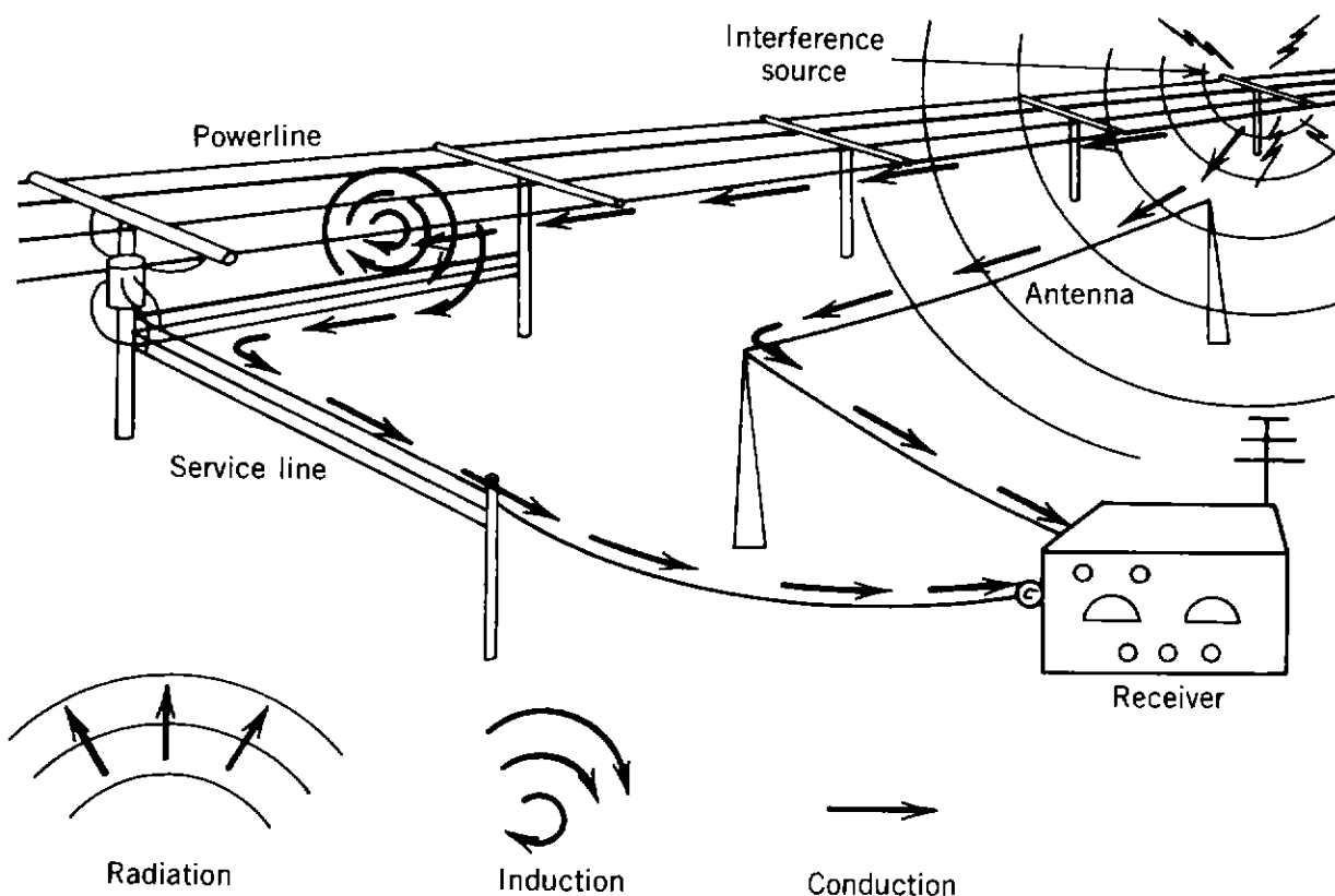
Figure 8.7. Paths by which interference energy travels from source to radio receiver. (From Ref. 17. Used with permission. © 1976 IEEE.)
