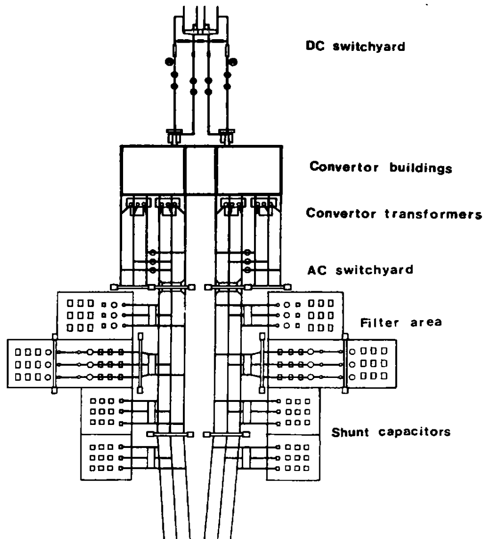
Figure 5.10. Typical converter station layout [2].
