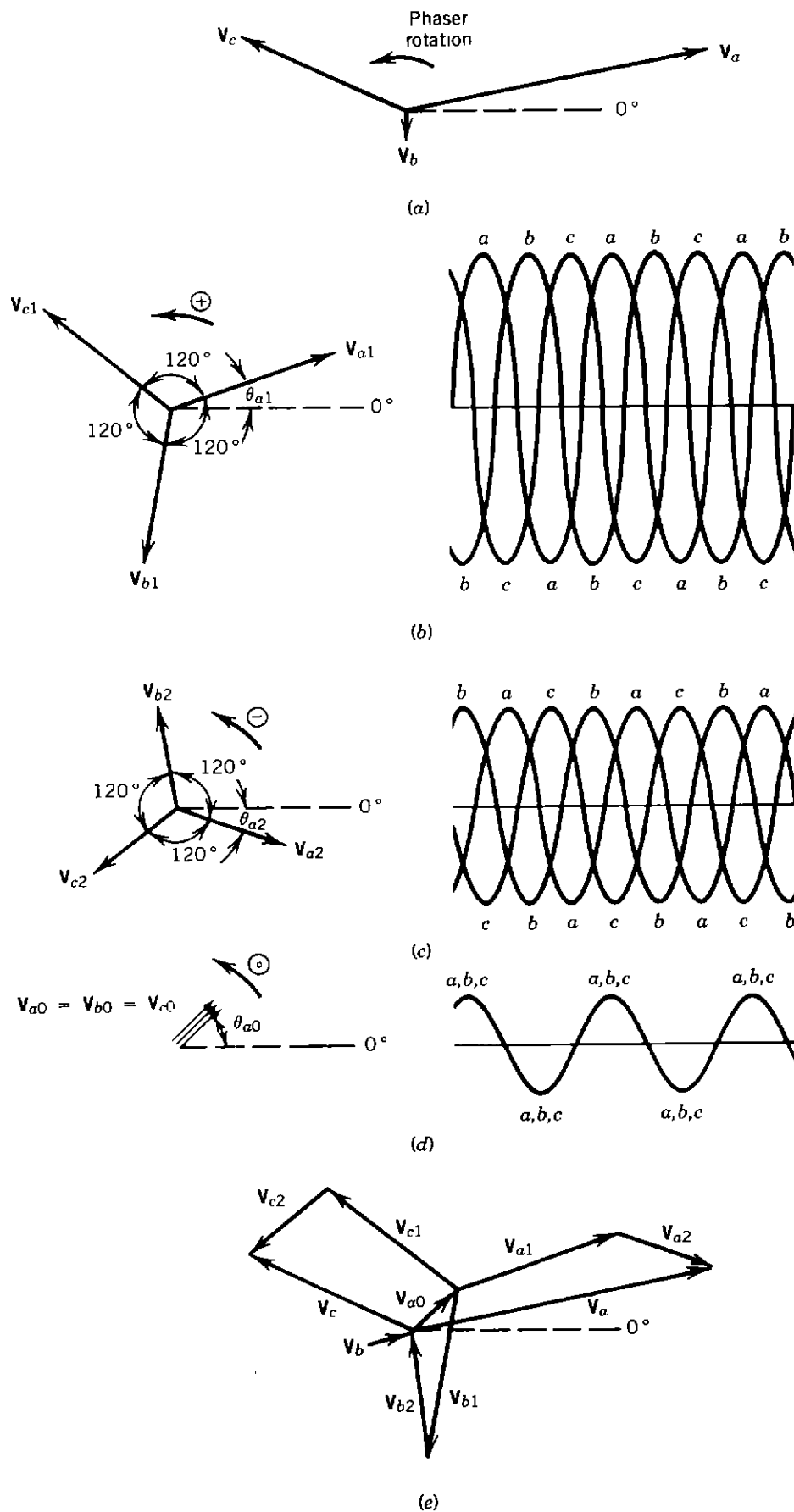
Figure 3.1. Analysis and synthesis of set of three unbalanced voltage phasors: (a) original system of unbalanced phasors; (b) positive-sequence components; (c) negative-sequence components; (d) zero-sequence components; (e) graphical addition of phasors to get original unbalanced phasors.
