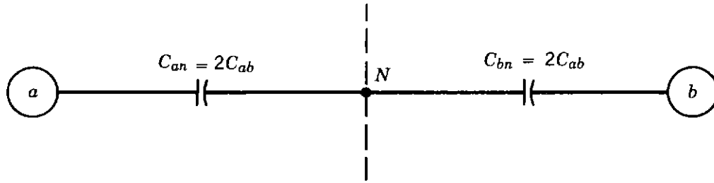
Figure 2.20. Line-to-neutral capacitance.
