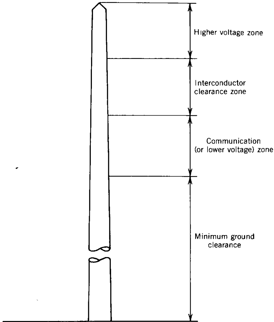
Figure 9.21. Allotment of pole space.
