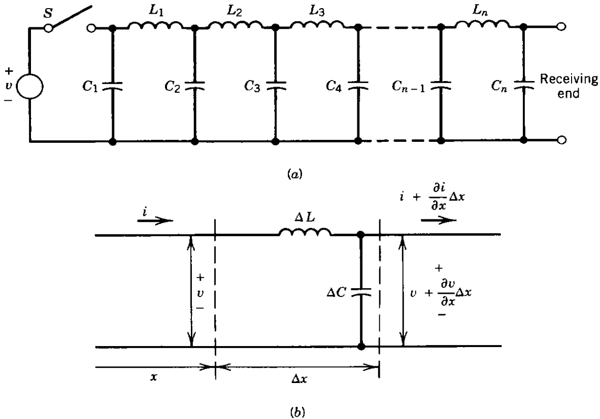
Figure 7.2. Representation of two-wire transmission line for application of traveling waves: (a) lumpy representation; (b) elemental section of line.
