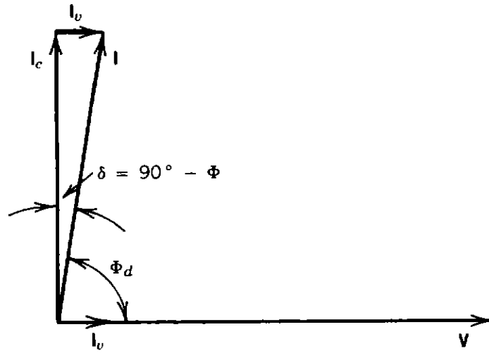
Figure 4.24. Phasor diagram for cable dielectric.
