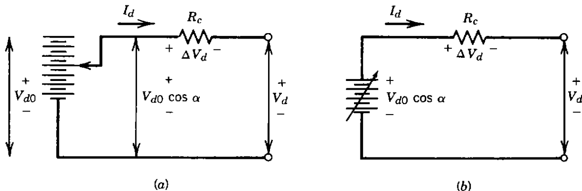
Figure 5.4. Equivalent circuit representations of bridge rectifier.
