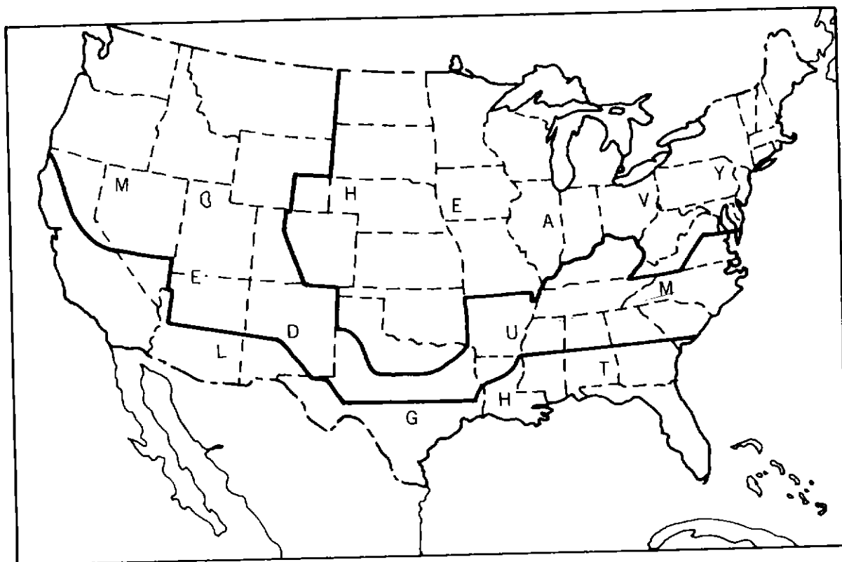
Figure 9.5. NESC's mechanical loading map for overhead lines.
