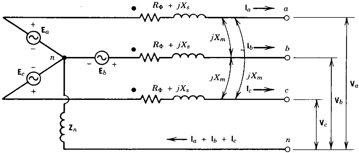
Figure 3.7. Equivalent circuit of cylindrical-rotor synchronous machine.
