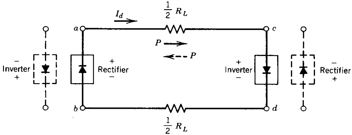
Figure 5.15. Illustration of reversion in power flow direction.
