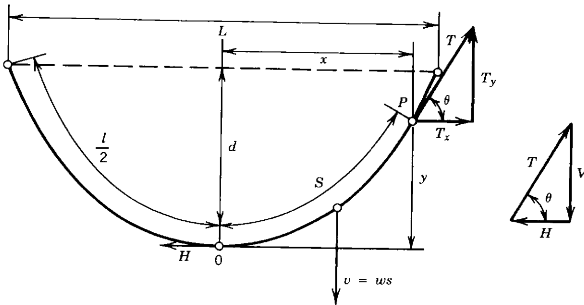
Figure 10.1. Conductor suspended between supports at same elevation.
