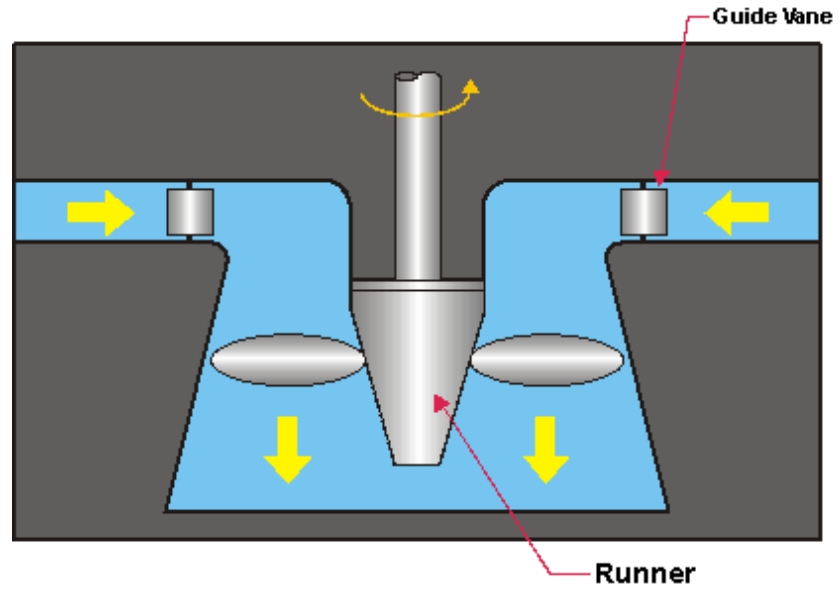
Figure 5.3: Kaplan Turbine
