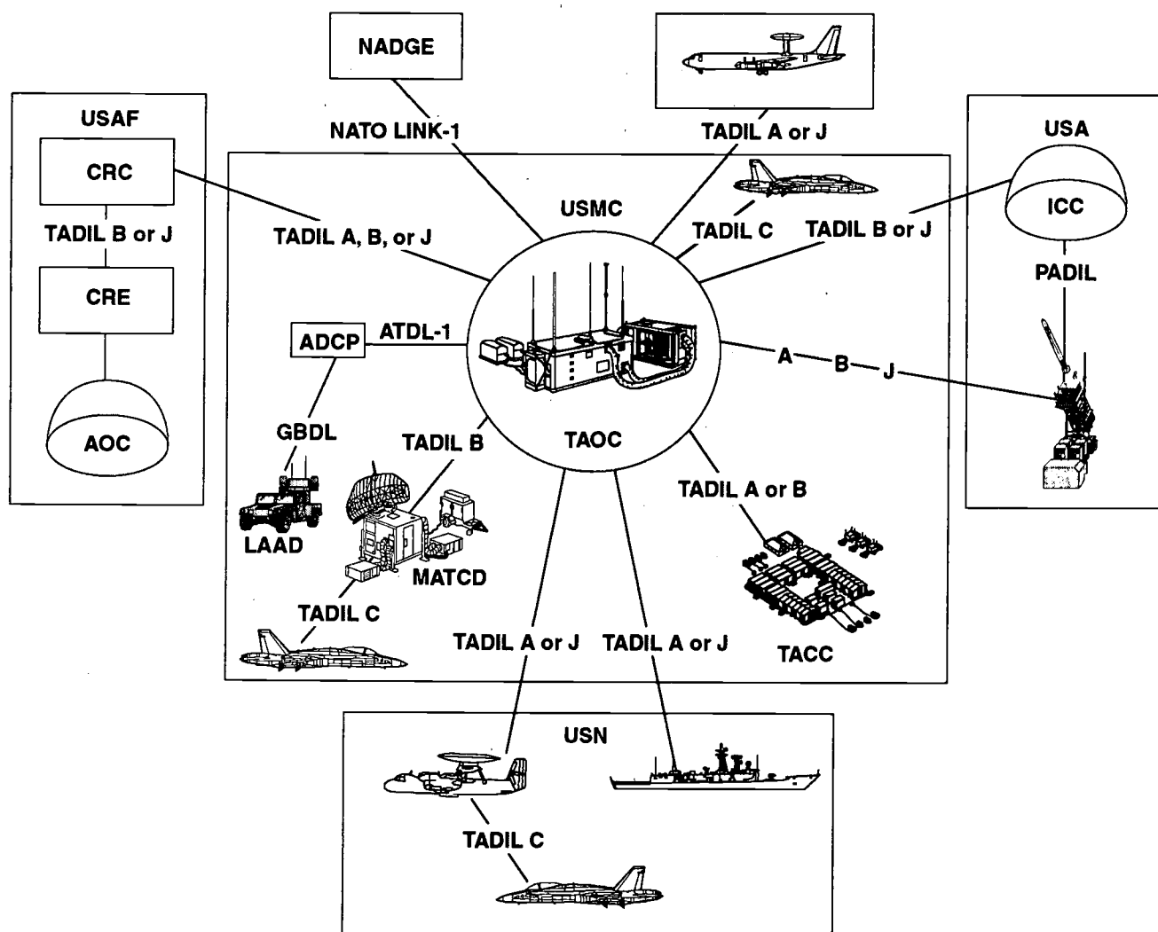
Figure A-2. Data Link Interfaces (TAOC-Emphasis).
