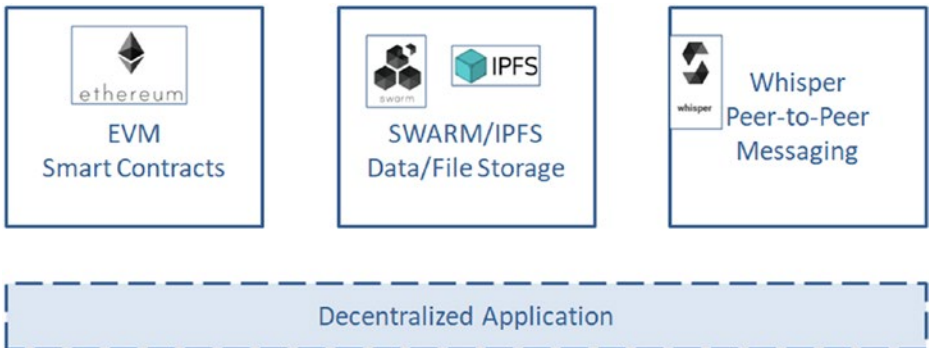
Figure 2-3. Ethereum ecosystem
