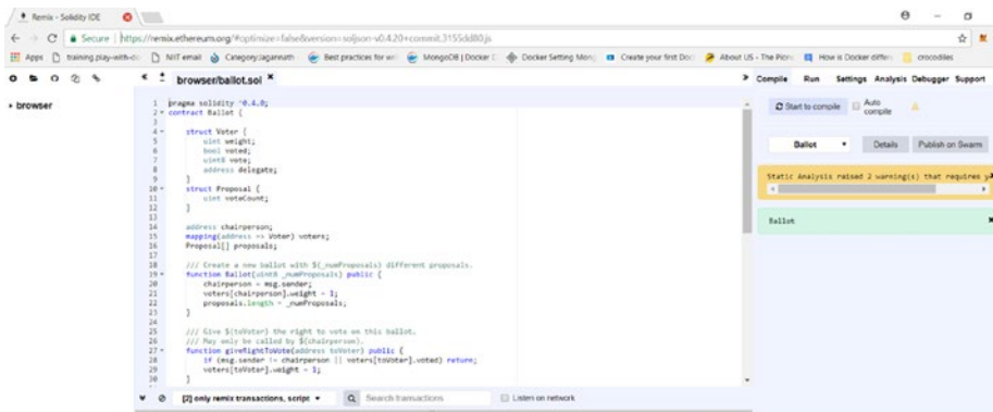
Figure 9-3. Remix browser
