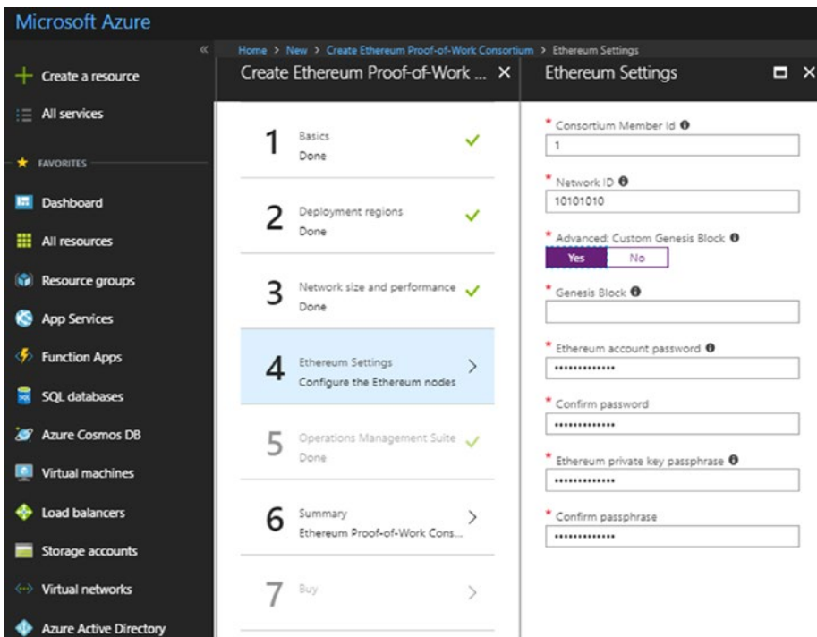
Figure 4-24. Ethereum settings
