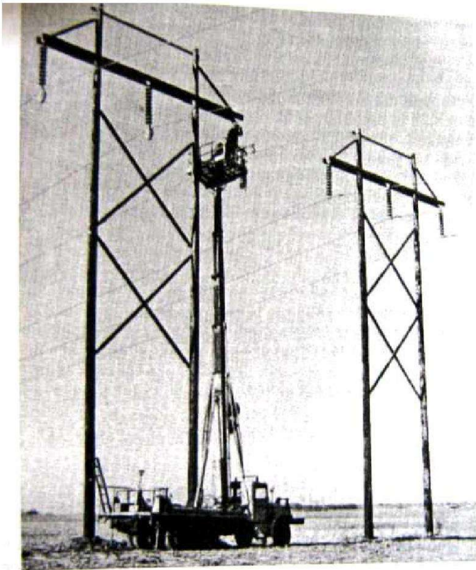
FIGURE 11.17 Conductor clipping with a high-reach
