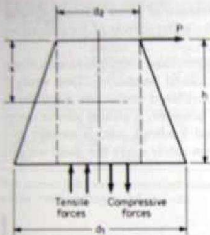
FIG. 5-2 Diagram of stresses on pole.
