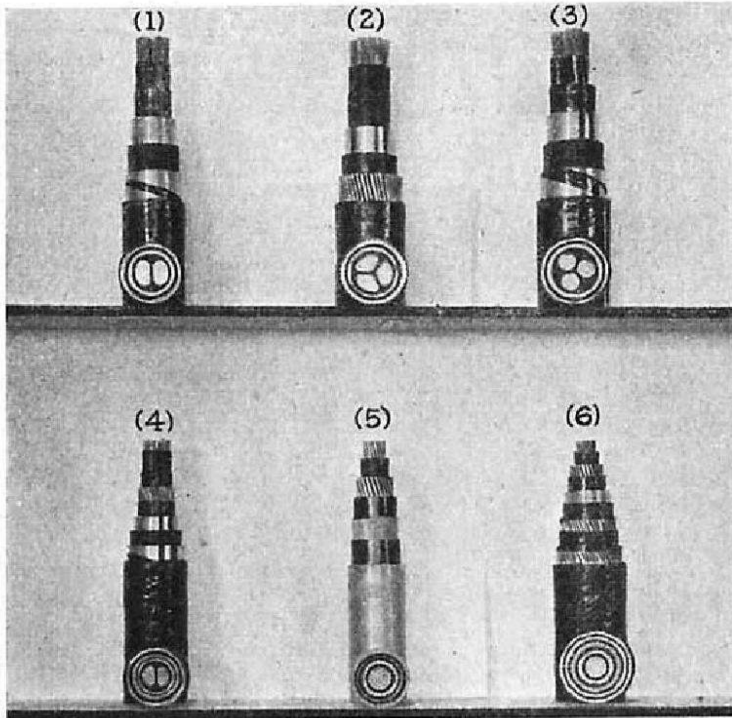
FIG. 70 PAPER-INSULATED POWER CABLES
