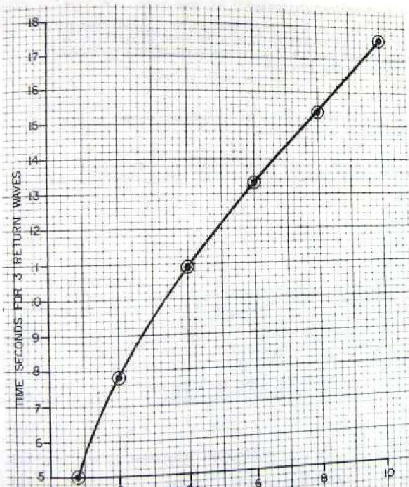
Wave Timing Chart Based on Formula
