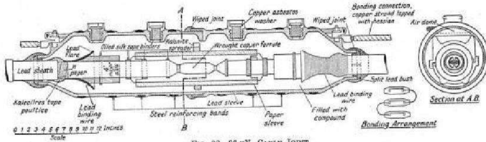
FIG. 82. 66 kV. CABLE JOINT (Cattinder's Cable and Construction Co.)
