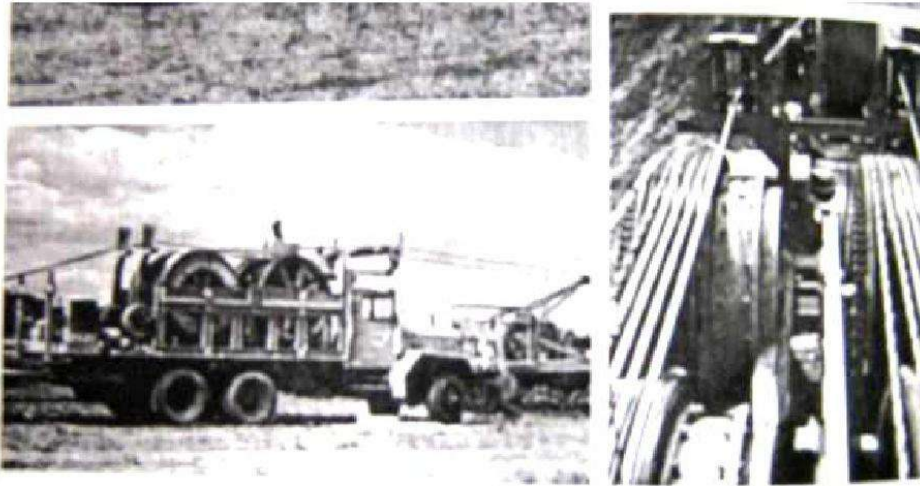
FIGURE 11.13 Views of a tensioner for bundles of two stringing
