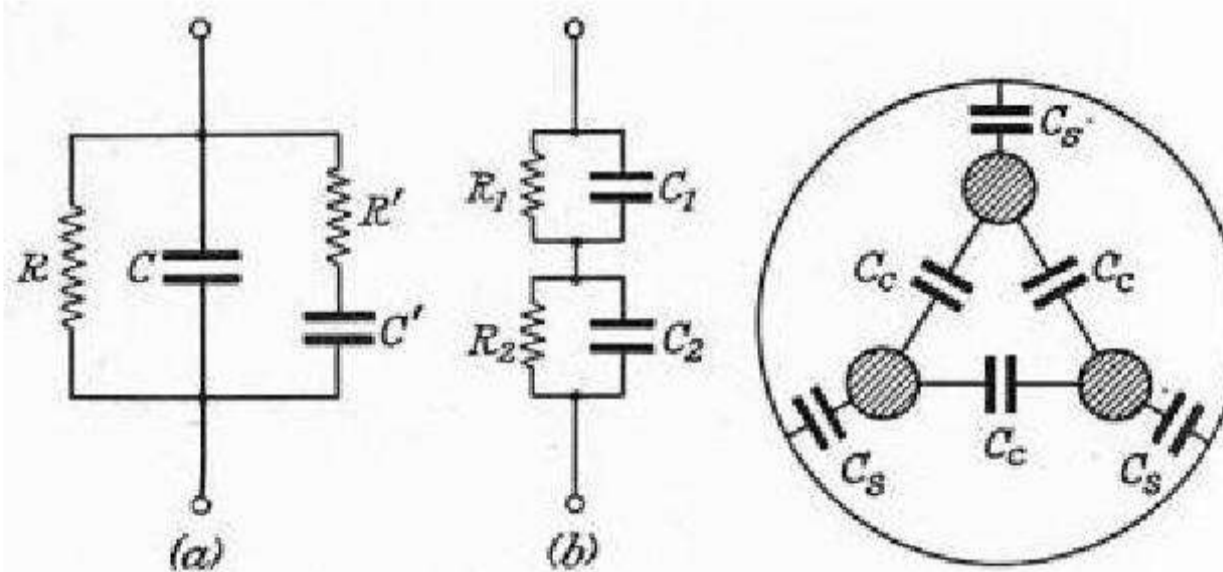
FIG. 93 REPRESENTATIONS OF IMPERFECT DIELECTRIC
