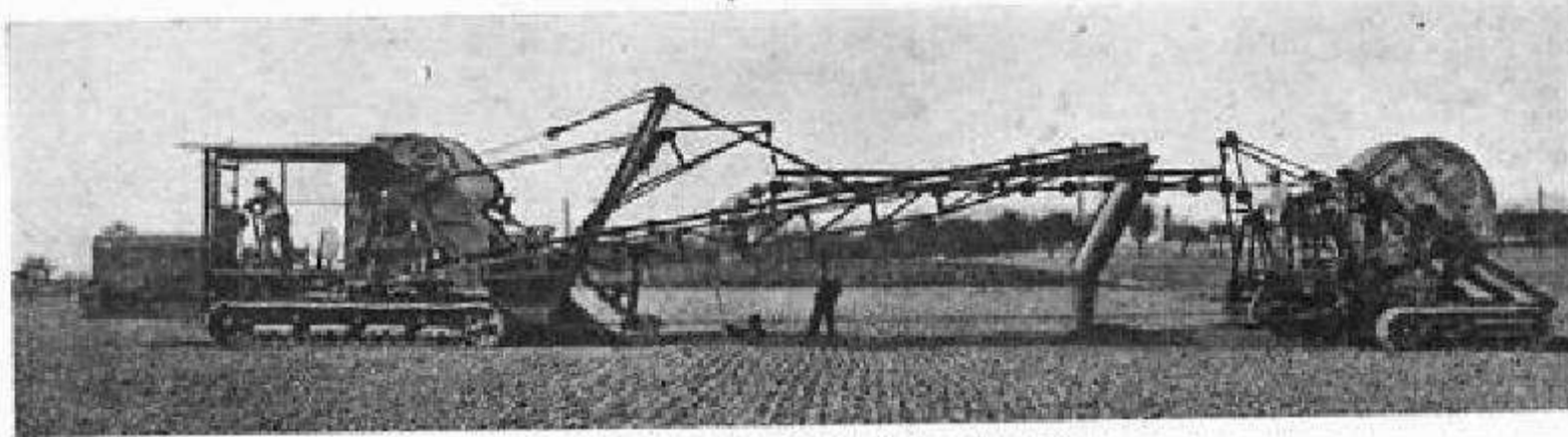
FIG. 78. MACHINE LAYING OF CABLES (Wasserhutte A.-G.)
