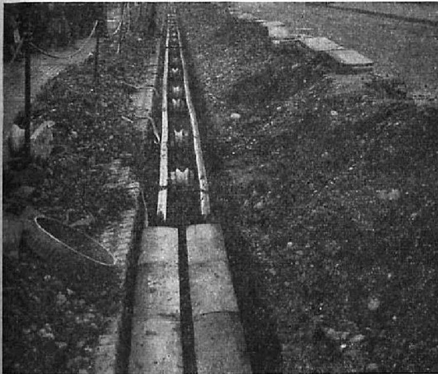
FIG. 79. CABLES IN TRENCH PROTECTED BY CONCRETE COVERS
