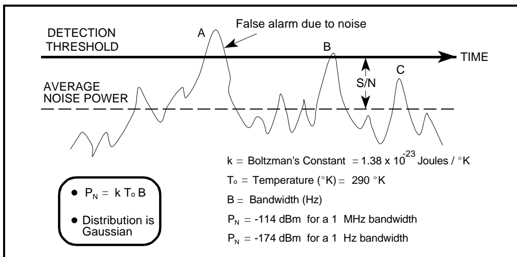
Figure 1. Receiver Noise Power at Room Temperature
