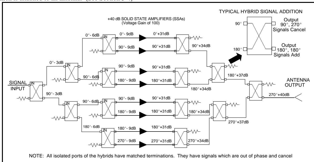
Figure 6. Combiner Network
