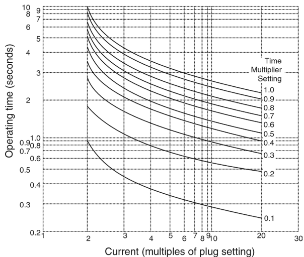
Figure 2.4 Time/Current Characteristic.
