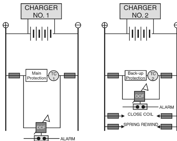
Figure 2.1 Arrangement of D. C. Supplies with Two Trip Coils for Each Circuit Breaker
