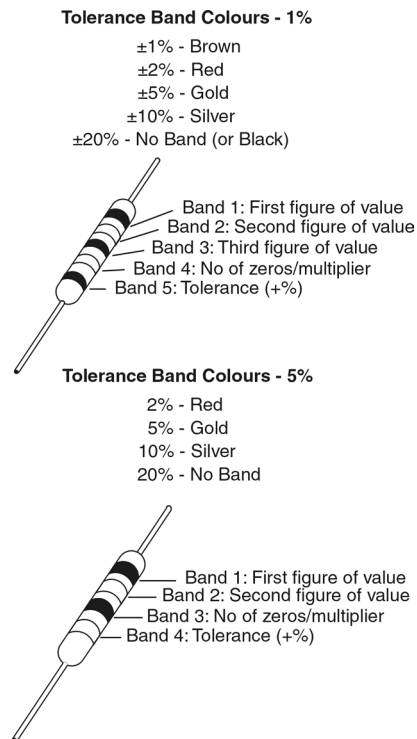
Figure D.1 Color coding for tolerance resistors
