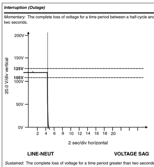
Figure 1.5 Interruption - Momentary/Sustained
