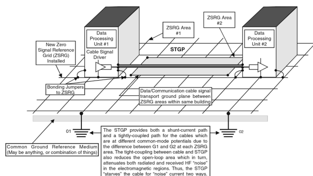
Figure 1.11 Data/Communication Signal Referencing
