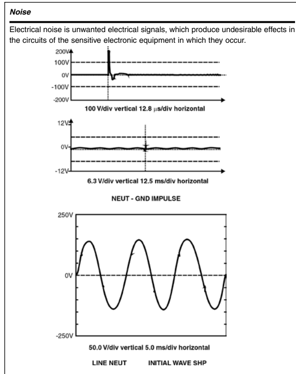
Figure 1.6 Noise
