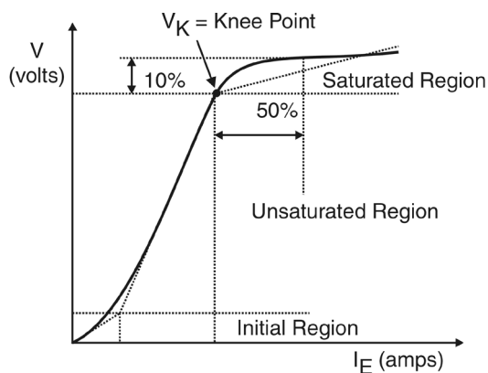
Figure 2.2 Typical CT Magnetization Curve.
