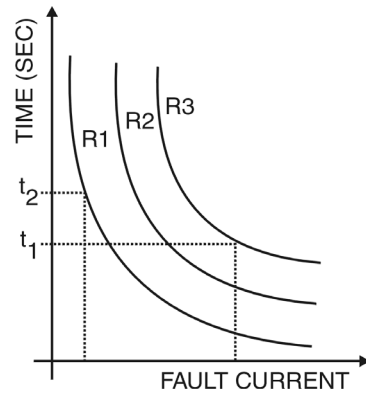
Figure 2.7 Inverse Definite Minimum Time.
