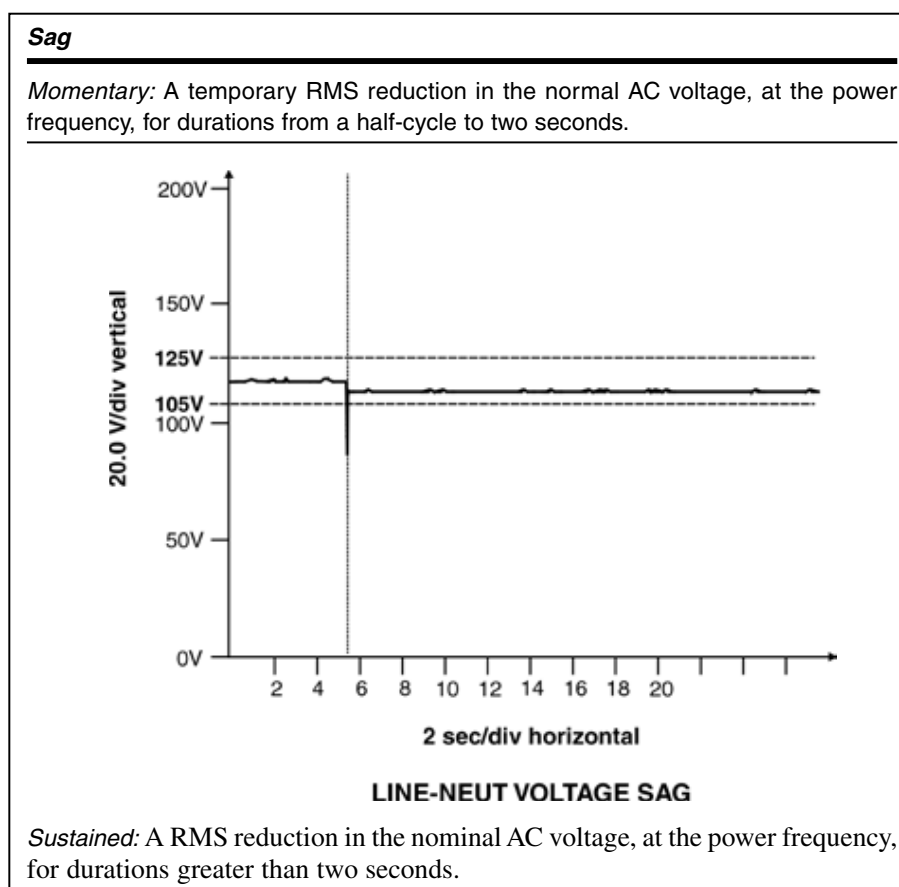
Figure 1.1 Sag
