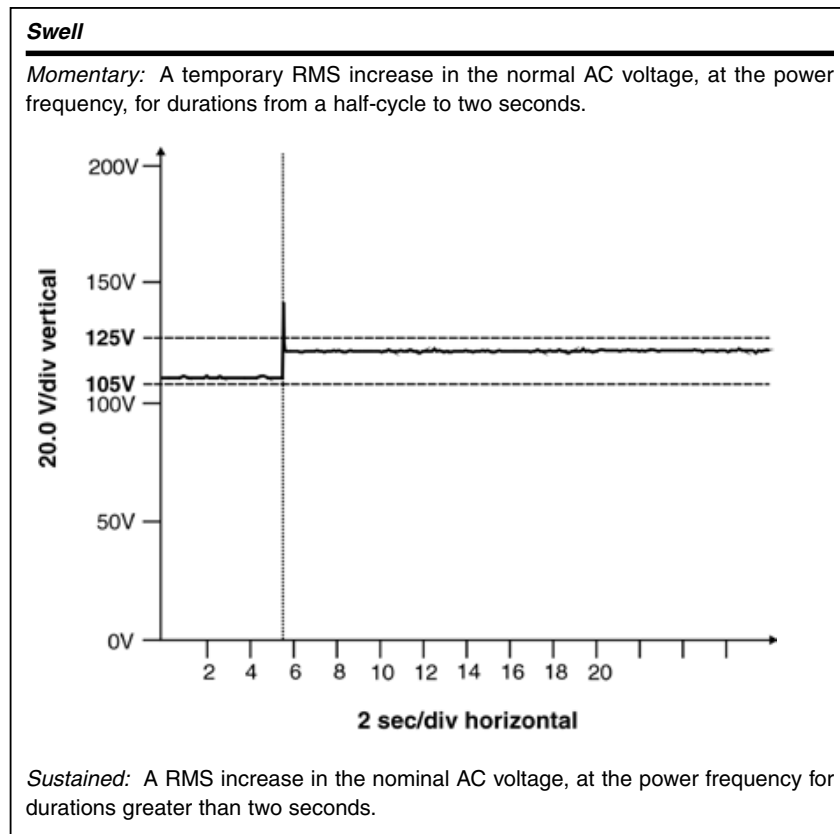
Figure 1.2 Swell
