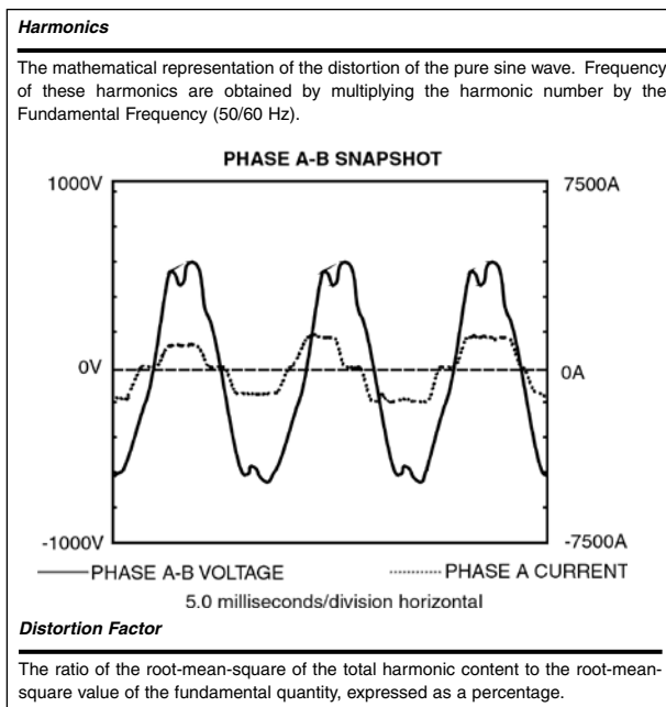
Figure 1.4 Harmonics/Distortion Factor
