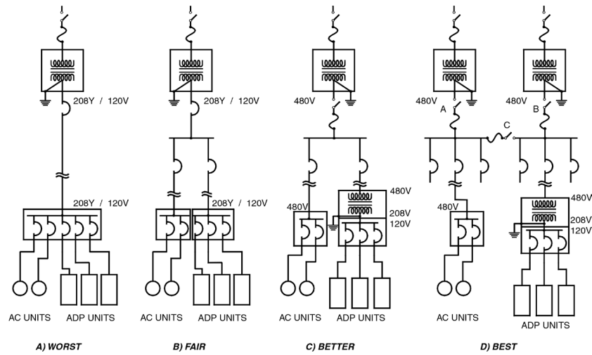
Figure 1.9 Four Wiring Diagrams
