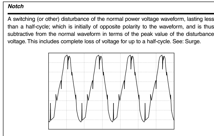
Figure 1.7 Notch
