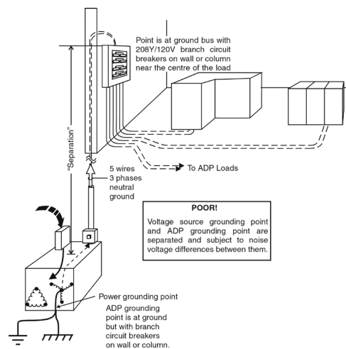
Figure 1.10 Poor and Better - Two Transformer Installation Diagrams
