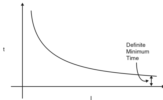
Figure 2.3 IDMT Relays
