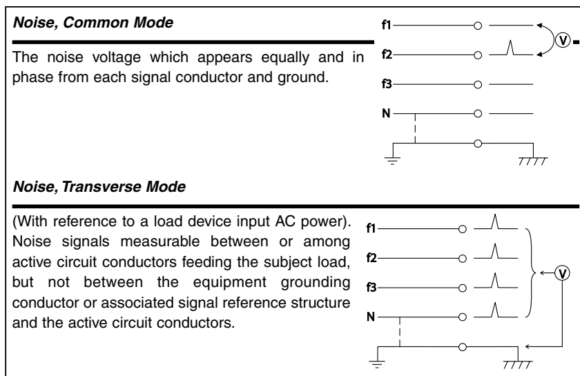
Figure 1.8 Noise - Common Mode/Transverse Mode
