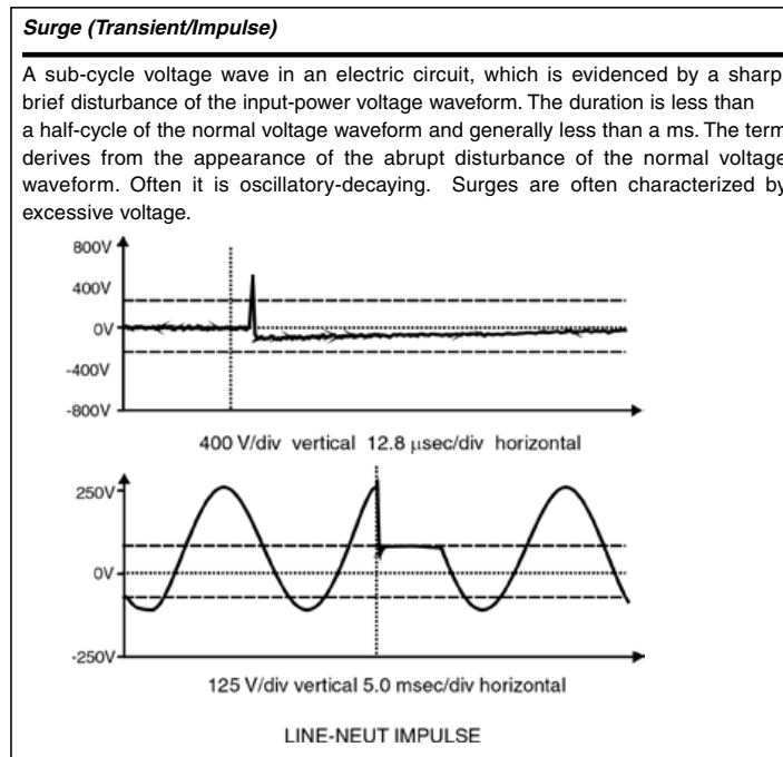
Figure 1.3 Surge/Transient
