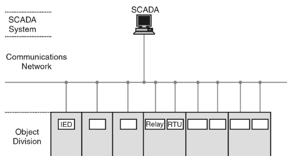
Figure 3.2 Basic Architecture of Substation Automation
