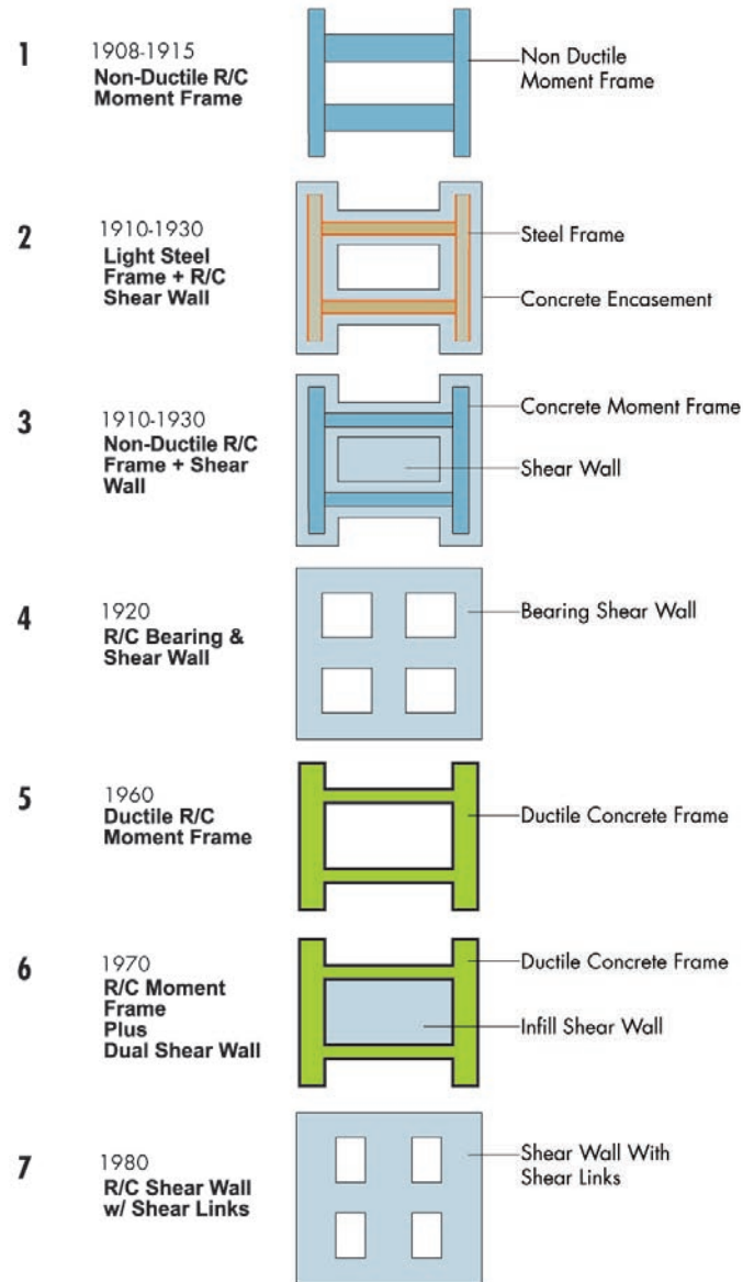
Figure 7-3: Concrete building frameworks
