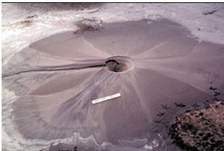
Figure 3-11: Sand Boil.
