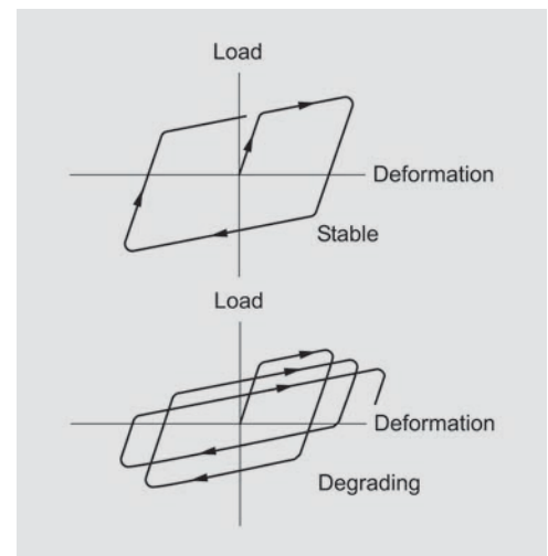
Figure 7-6: Cyclic behavior.
