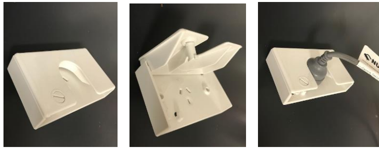
Figure 2 Standard GPO with the “FLIP TOP” cover for fridges and freezers- Clipsal- type 10PL.
