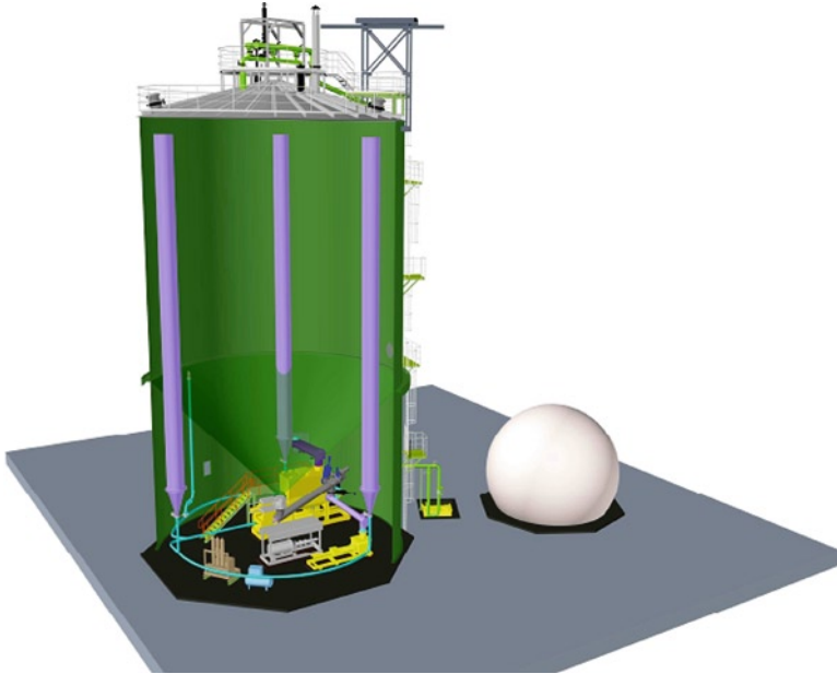
Fig. 7.15 Sectional view of a Dranco digester showing internal feeding tubes and the feeding pump under the digestion tank (photo courtesy: Organic waste systems n.v.)
