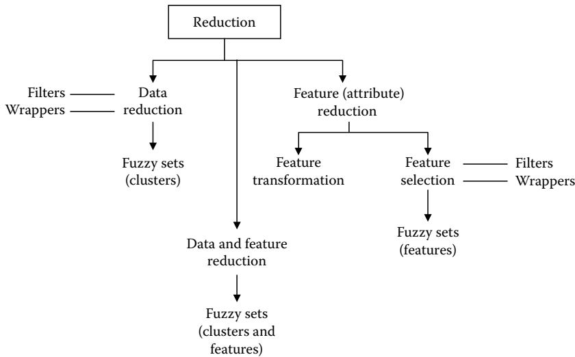
FIGURE 22.11 Categories of reduction problems in pattern recognition: feature and data reduction, use of filters, and wrappers criteria.
