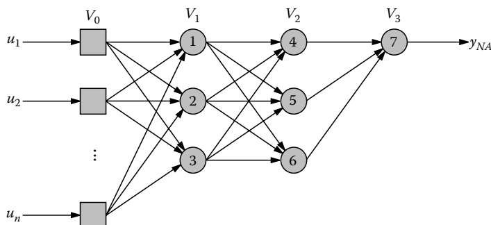
FIGURE 9.2 Order of node adding to the network in the tiling algorithm.
