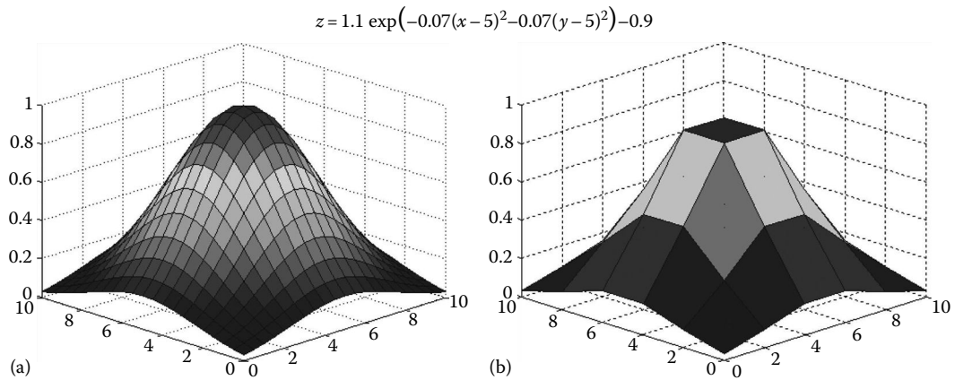
FIGURE 20.1 Required surface obtained from Equation 20.1: (a) 21 \times 21 = 441 points and (b) 6 \times 6 = 36 points.
