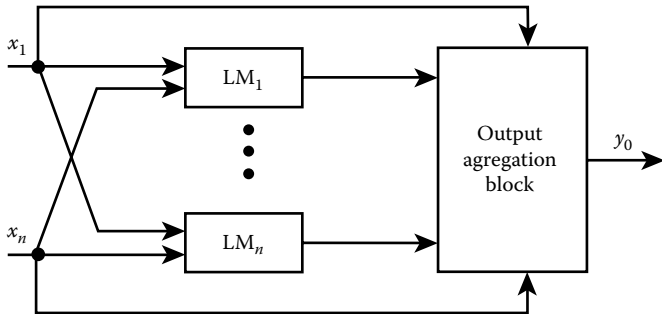
FIGURE 19.28 Aggregation block of the local fuzzy systems.
