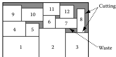
FIGURE 27.2 An example of three-stage guillotine cutting.
