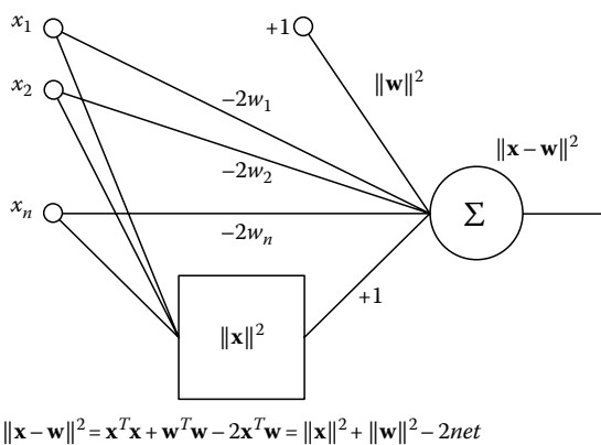
FIGURE 6.6 Sarajedini and Hecht-Nielsen neural network.
