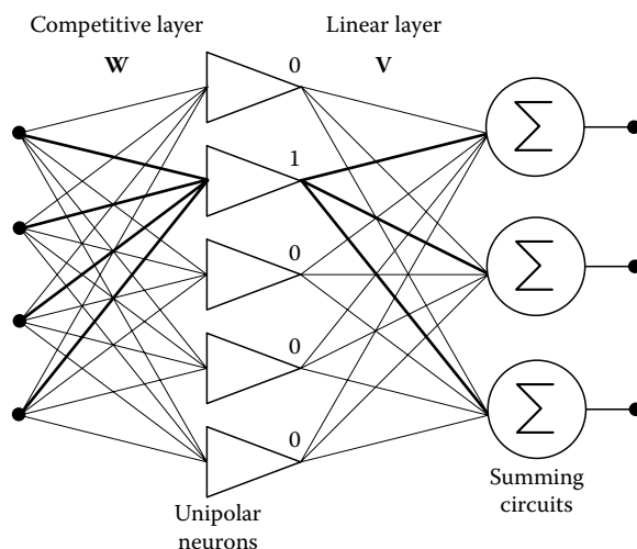
FIGURE 6.10 Learning vector quantization.
