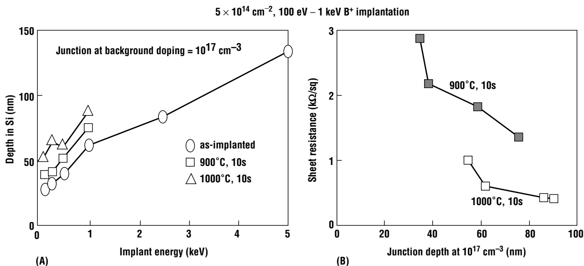
Figure 16.20 Very shallow junction results using low energy implantation and RTA. Increasing the anneal temperature increases the junction depth (A), but produces lower sheet resistance (B).
