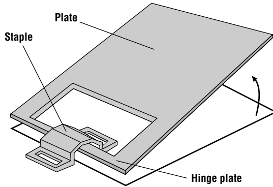
Figure 19.29 Basic hinge structure allowing out-of-plane motion of the plate (after Pister [59]).
