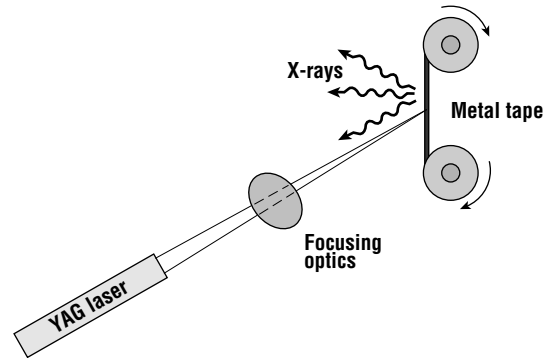
Figure 9.15 Laser plasma-heated x-ray source uses a focused high intensity pulsed laser to ablate a metal film. The superheated metal atoms radiate x-rays.
