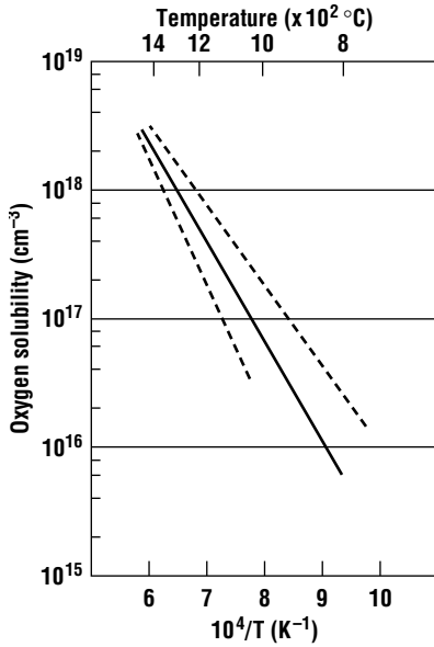
Figure 2.10 The solubility of oxygen in silicon. The dashed lines correspond to the highest and lowest variations (after Shimura).
