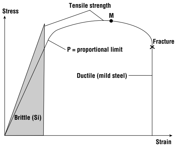
Figure 19.2 Stress–strain curve for a typical metal as well as for a brittle material like silicon (high Young’s modulus and no plastic deformation region) ( reprinted with permission from Madou [7]. Copyright CRC Press ).
