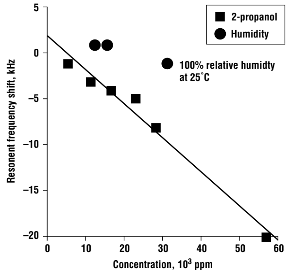
Figure 19.22 Change in cantilever beam resonant frequency as a function of concentration for isopropanol and water (after Baltes et al. [47], © 1998 IEEE).
