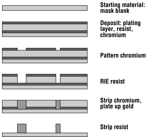
Figure 9.22 Additive process for x-ray mask fabrication.
