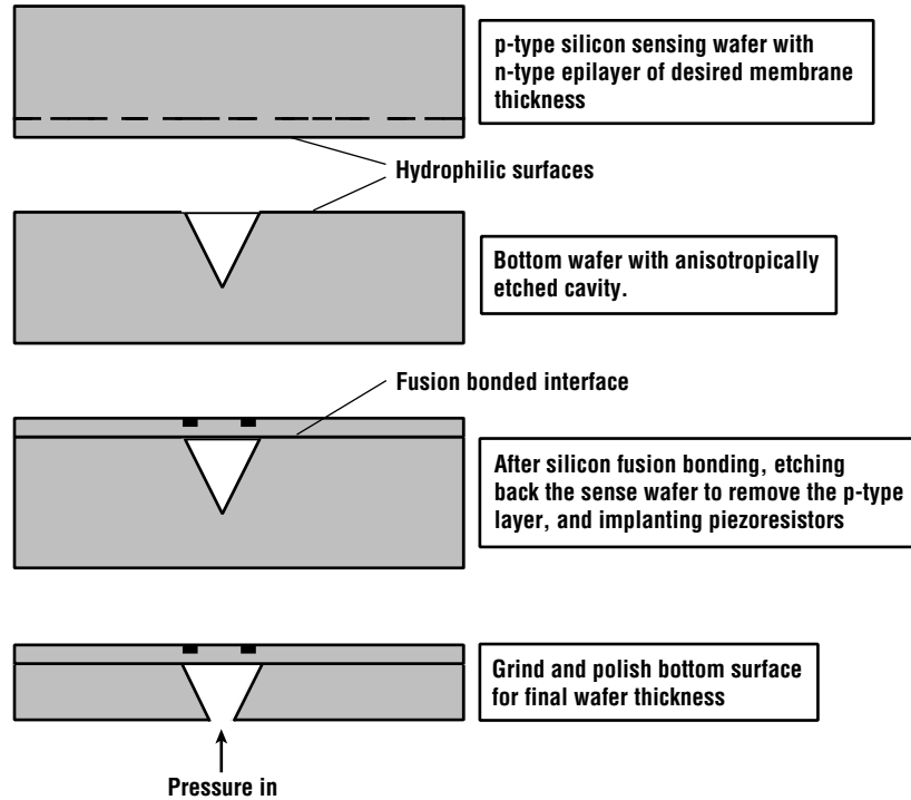
Figure 19.20 Fabrication process for silicon fusion bonded, low pressure sensor (after Petersen [3], © 1982 IEEE).
