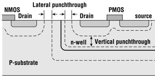
Figure 16.5 The minimum well depth must be chosen to prevent punchthrough from the reverse-biased source/well and source/substrate junctions.
