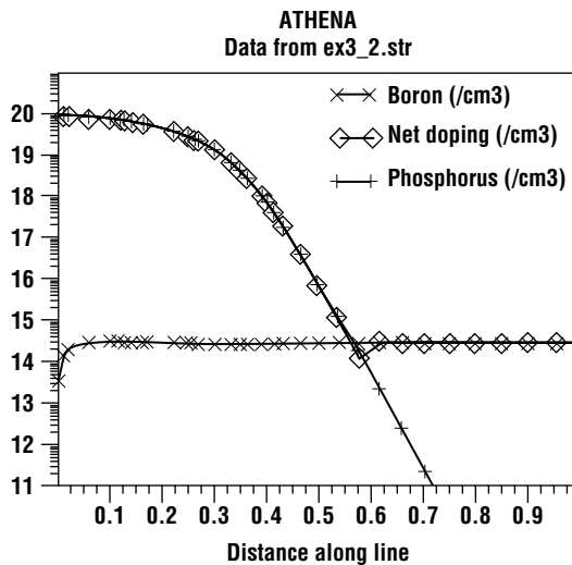
Figure 3.18 Plot of impurity as a function of depth for phosphorus drive-in.
