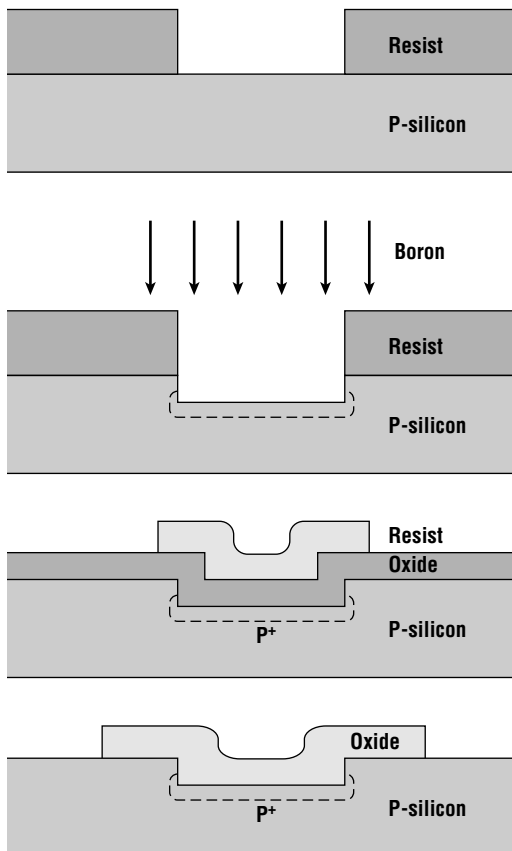
Figure 15.9 Simple shallow trench isolation process.
