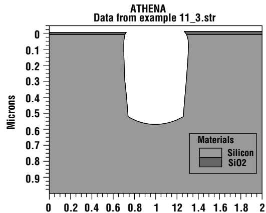
Figure 11.22 Etching a trench 0.5 \mu\text{m} wide.
