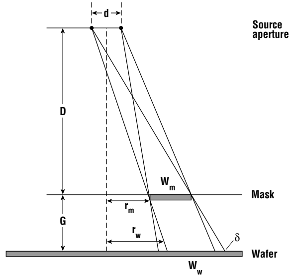
Figure 9.19 Geometry of the exposure system shown in Figure 9.18.
