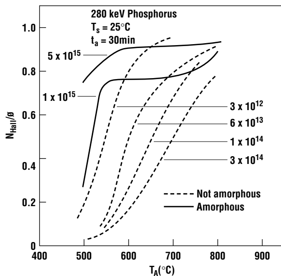
Figure 5.17 Isochronal annealing of phosphorus in silicon, with dose as a parameter. The solid lines correspond to implants that amorphized the substrate (reprinted by permission, AIP, after Crowder and Morehead).
