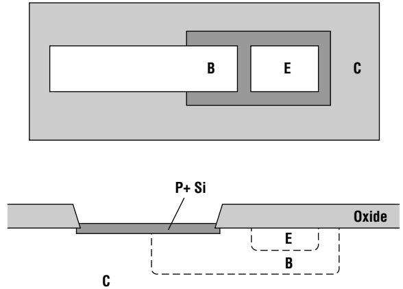
Figure 15.20 A PtSi Schottky used to shunt the base and collector of a bipolar transistor.
