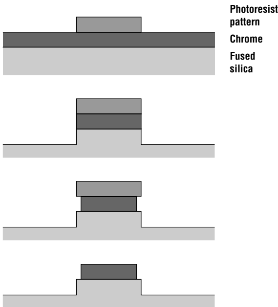
Figure 7.28 Self-aligned method of phase shifting the radiation at the edges of a pattern.
