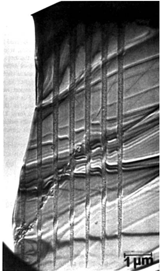
Figure 15.11 Cross-sectional scanning electron micrograph of an extreme aspect ratio deep isolation process (after Rajeevakumar et al., ©1991 IEEE).
