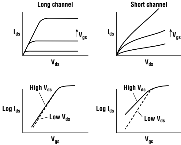
Figure 16.10 Current-voltage characteristics of MOSFETs comparing long- and short-channel behavior; typical threshold voltage dependence on gate length.
