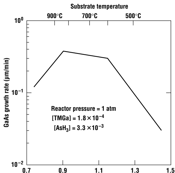
Figure 14.24 Growth rate of GaAs during MOCVD as a function of temperature (after Tischler [75], ©1990 IBM).
