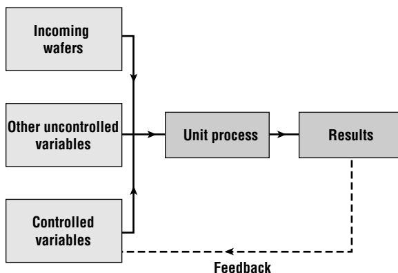
Figure 20.9 A schematic of a semiconductor process. Both controlled and uncontrolled variables must be considered.
