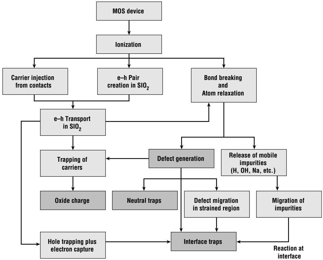
Figure 9.28 Radiation damage flow path (after Ma and Dressendorfer, reprinted by permission, Wiley).
