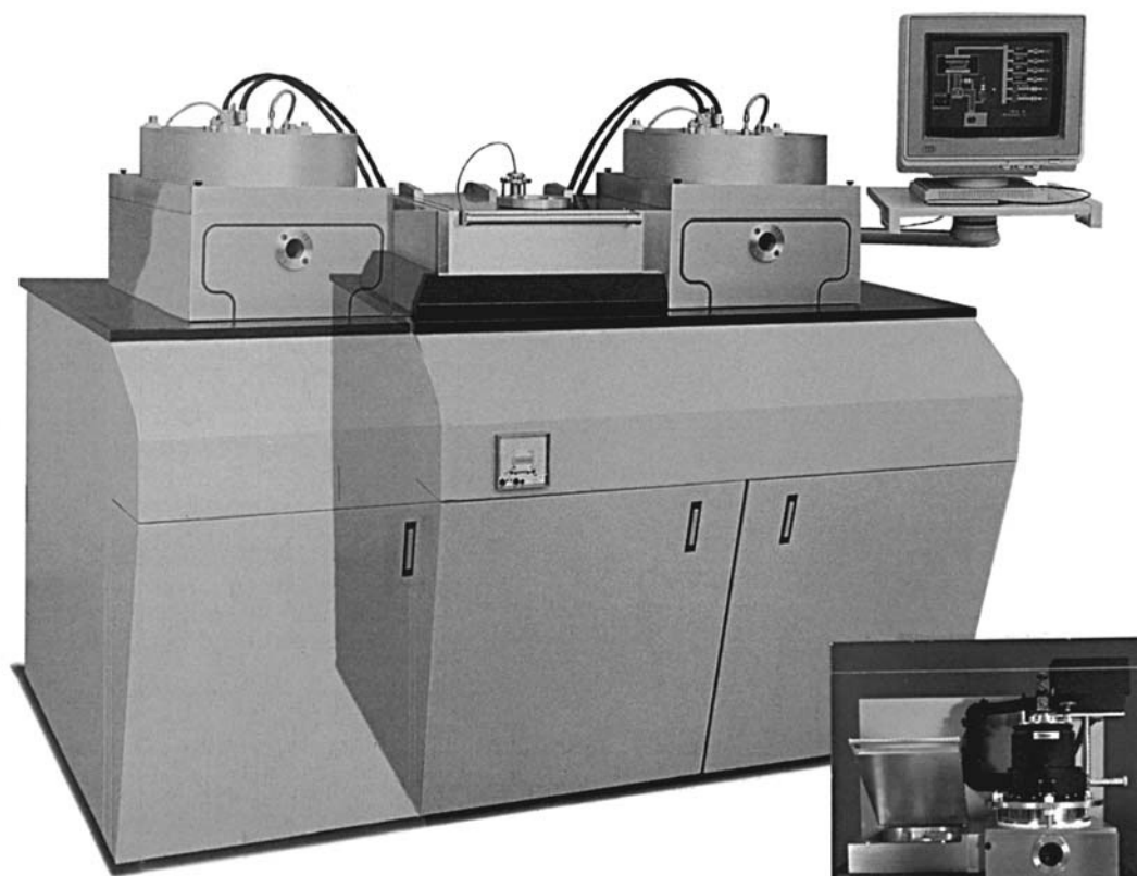
Figure 11.14 A computer-controlled, dual-chamber, parallel-plate plasma etch system ( courtesy Plasma Therm ).
