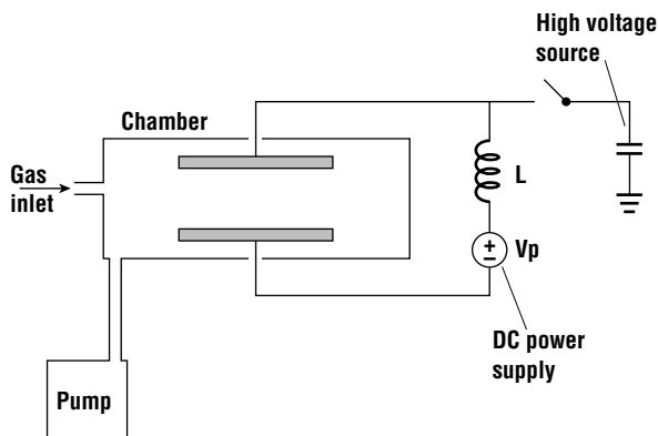
Figure 10.14 A simple parallel-plate plasma reactor.
