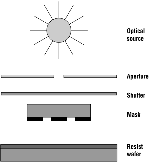
Figure 7.5 Schematic of a simple lithographic exposure system.
