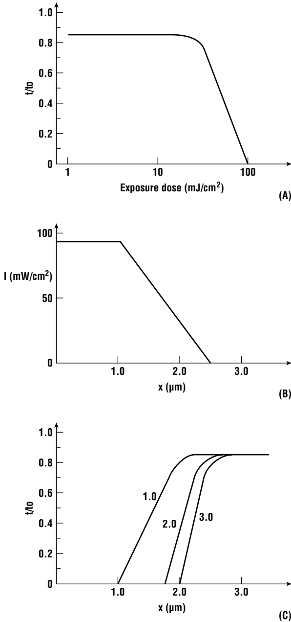
Figure 8.8 (A) Measured contrast curve for a commercial DQN resist. (B) Simple areal image. (C) Approximate profiles for 1-, 2-, and 3-sec exposures.
