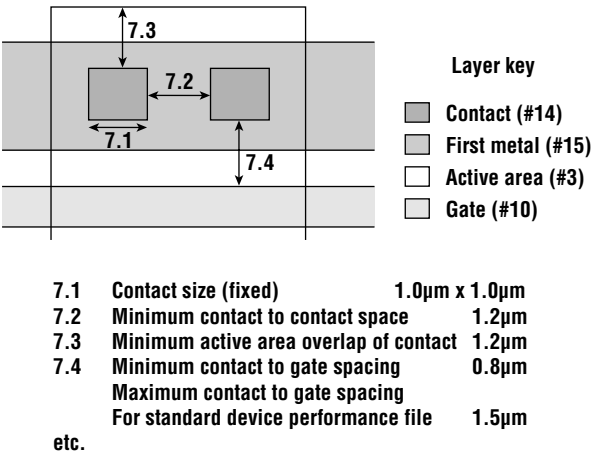
Figure 7.2 Excerpt of typical design rule set. This portion deals with first metal rules for a particular technology.
