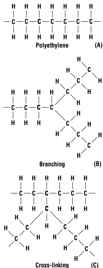
Figure 8.3 (A) Polyethylene, an example of a simple polymer. (B) Branched-chain polymers. (C) Cross-linking.
