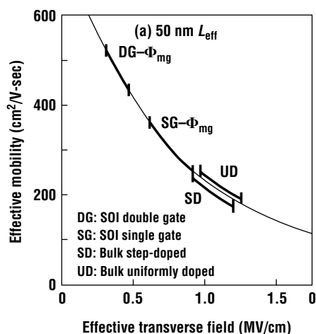
Figure 16.23 Effective transverse electric field ranges one can expect from bulk devices either uniformly doped or with a step profile, SOI single gate, and double gate devices (from Lochtefeld and Antoniadis, reprinted with by permission from IBM J. Res. Dev, Copyright 2000, IBM).
