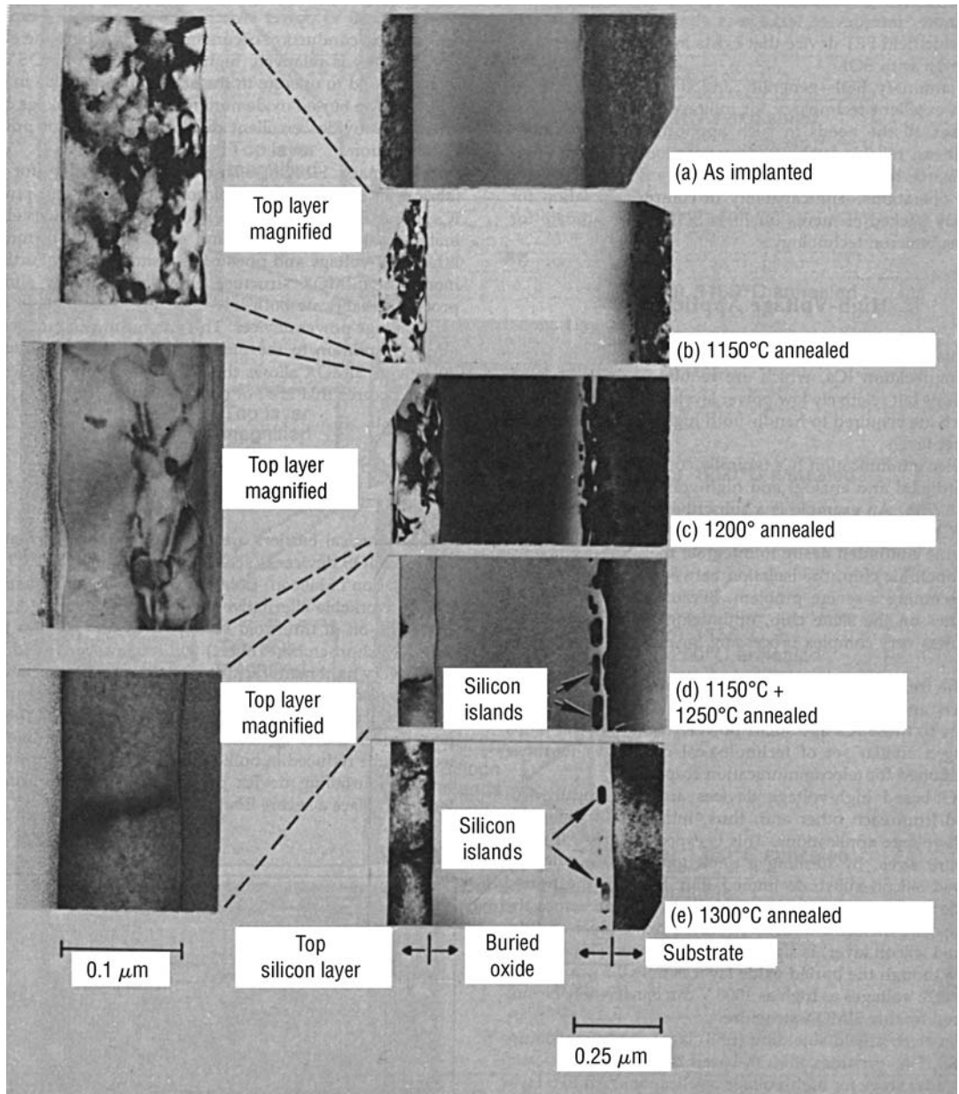
Figure 5.19 Cross-sectional TEMs of SIMOX layers for different anneal conditions. Samples were implanted at 150 keV with an oxygen dose of 2.25 \times 10^{18} \text{ cm}^{-2} (after Lam, reprinted by permission, © 1987 IEEE).
