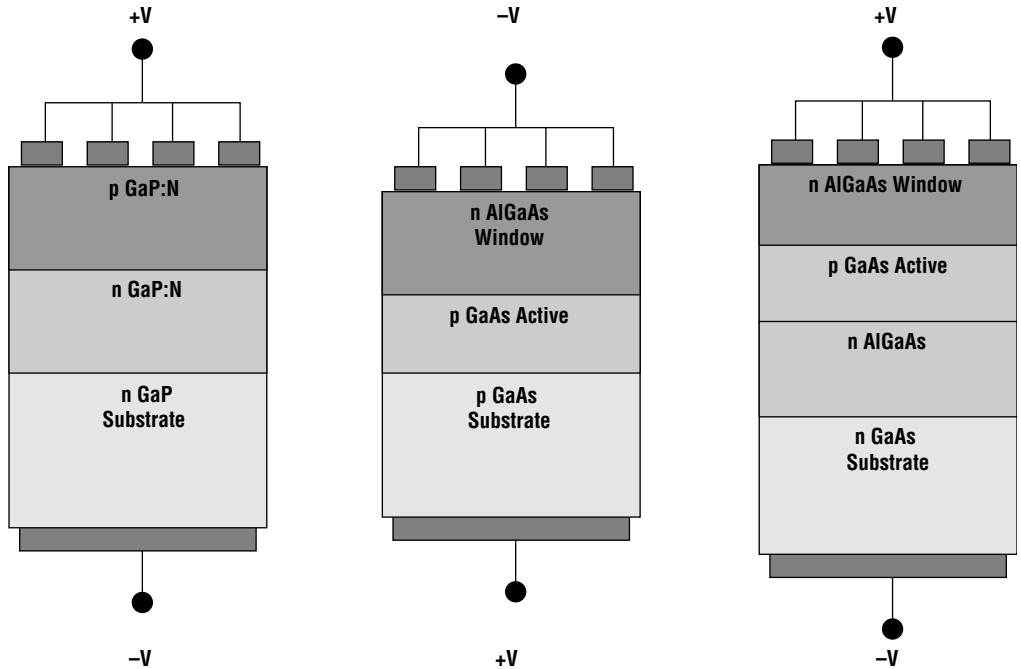
Figure 18.1 Typical LED structures: (A) homojunction, (B) single barrier, and (C) double barrier. If backside contact is not desired, the stack can be etched down to the substrate and a top-side substrate contact added.
