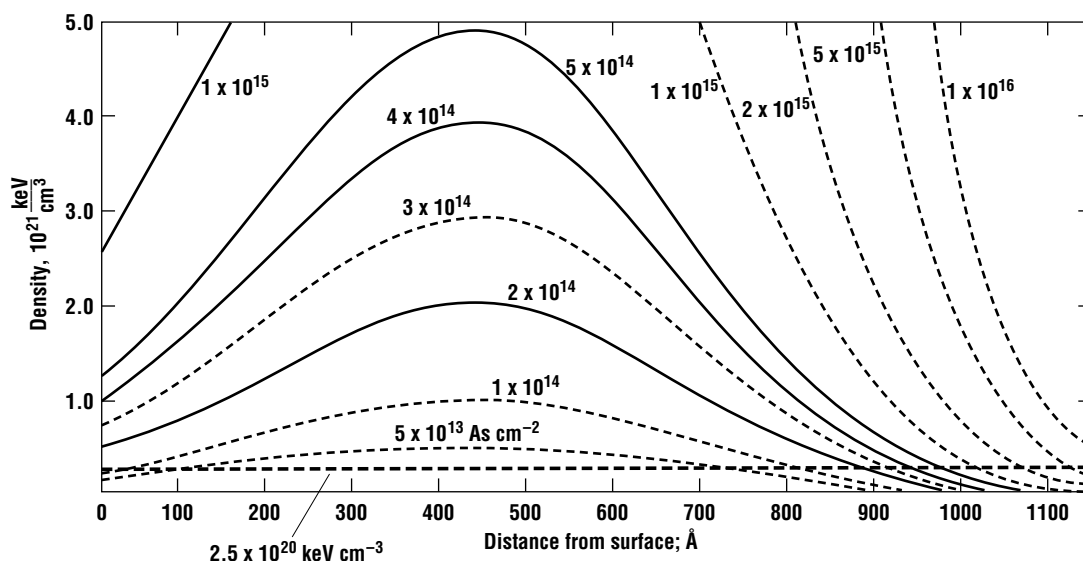
Figure 5.16 Damage density distribution for 100 keV arsenic implanted into silicon with dose as a parameter (reprinted by permission, AIP).
