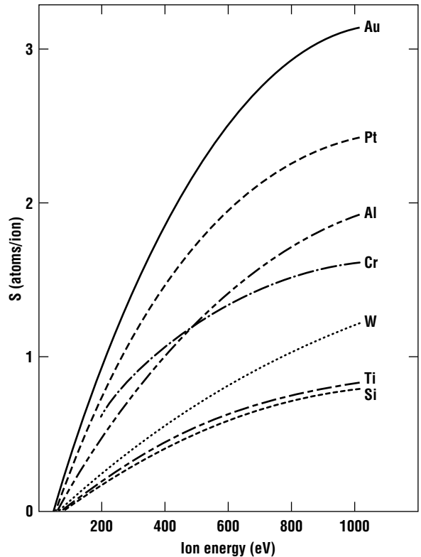
Figure 12.14 Sputter yield as a function of ion energy for normal incidence argon ions for a variety of materials (after Anderson and Bay, reprinted by permission).
