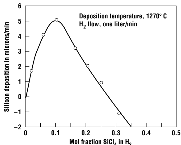
Figure 14.6 Growth rate as a function of the \text{SiCl}_4 flow. At high concentrations, the chlorine in the chamber leads to etching (after Theuerer, reprinted by permission of the publisher, The Electrochemical Society).
