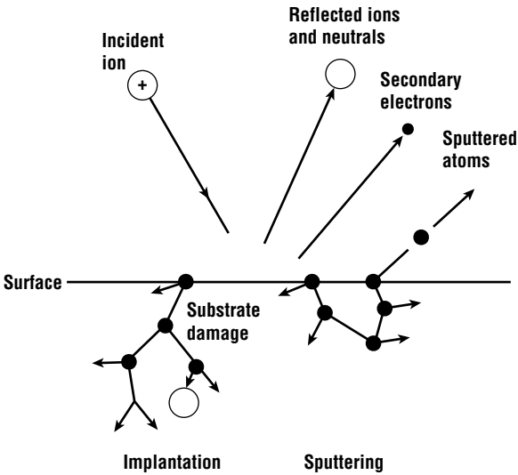
Figure 12.13 Possible outcomes for an ion incident on the surface of a wafer.
