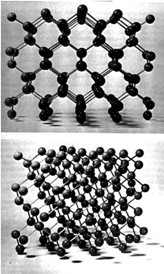
Figure 5.11 (A) Models of the diamond structure along a major crystal axis \langle 110 \rangle and along a random direction. (B) Schematics of channeling (reprinted by permission, Academic Press, after Mayer et al.).
