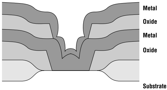
Figure 15.32 Nonplanarized plug structure consisting of a coincident contact and via.
