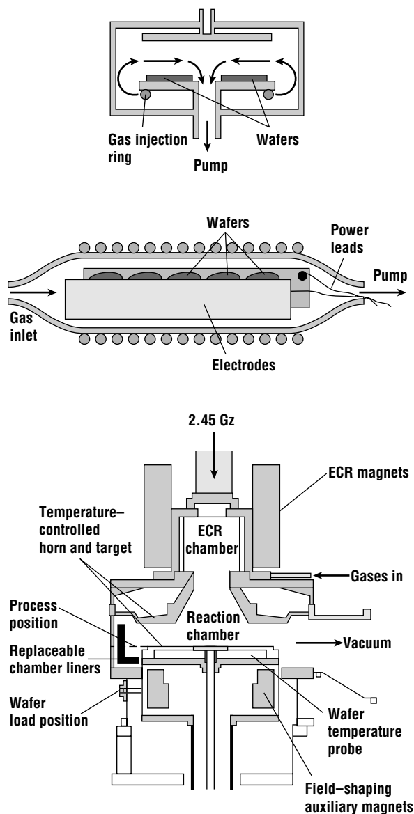
Figure 13.18 Basic PECVD geometries: cold wall parallel plate, hot wall parallel plate, and ECR.
