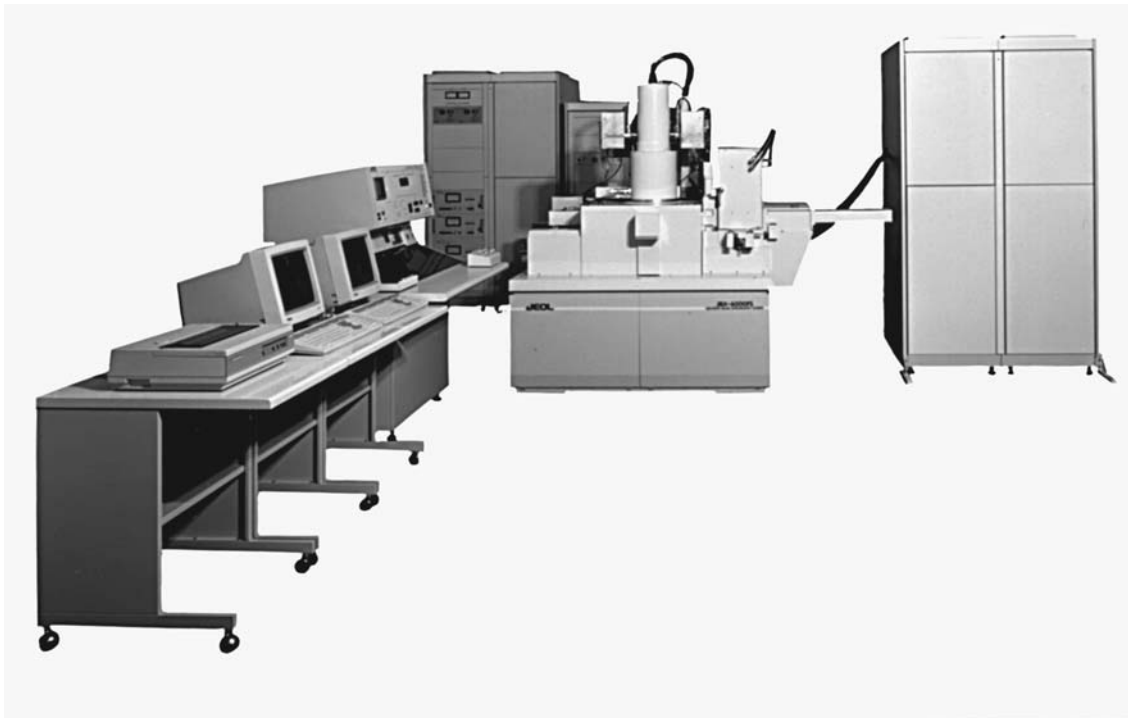
Figure 9.13 A JEOL-6000FS EBL system ( courtesy of JEOL Corporation ).
