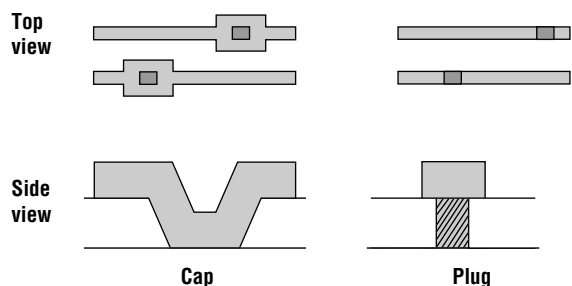
Figure 13.22 The use of caps versus plug-filled contacts.
