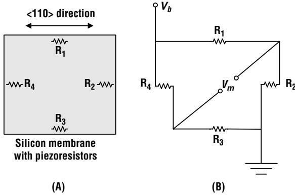
Figure 19.7 (A) Schematic drawing of the position and orientation of four piezoresistance elements on a silicon membrane with sides defined by anisotropic silicon etching of a (100) silicon wafer; (B) Wheatstone bridge configuration of the four piezoresistive elements.
