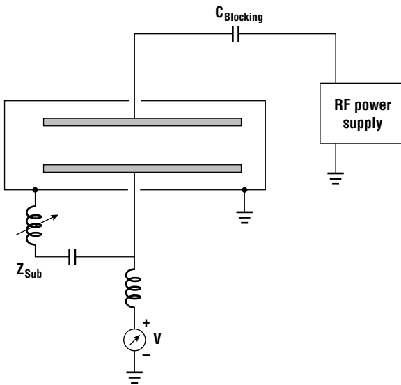
Figure 10.17 Schematic of an RF plasma system.
