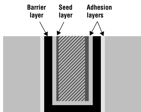
Figure 13.27 Most extreme stack in a contact, showing all of the needed layers. The crosshatched area is electroplated Cu.
