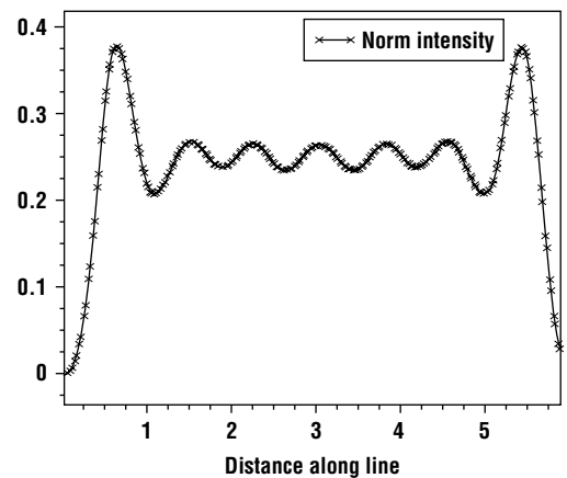
Figure 7.12 Same 1D plot for a grating with a pitch of 0.8 μm exposed on the same system.
