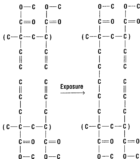
Figure 9.26 Cross-linking of an e-beam resist where the basic PMMA structure has been modified through the addition of a \text{C}=\text{C} side chain to promote cross-linking.
