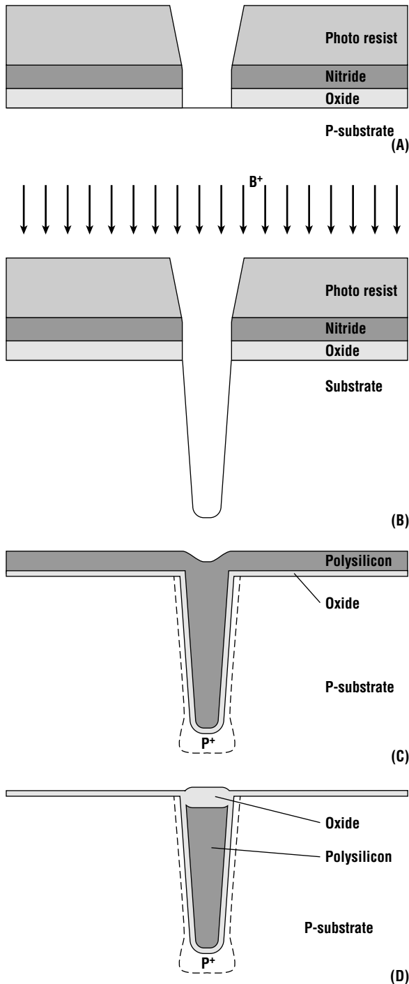
Figure 15.10 Deep trench isolation process schematic.
