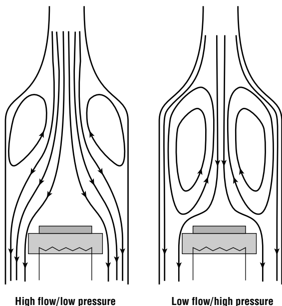
Figure 13.7 Buoyancy-driven recirculation cells.
