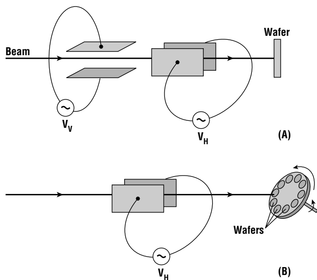
Figure 5.5 Typical scanning systems for ion implanters. (A) Electrostatic rastering commonly used in medium current machines. (B) Semelectrostatic scanning used on some high current machines.
