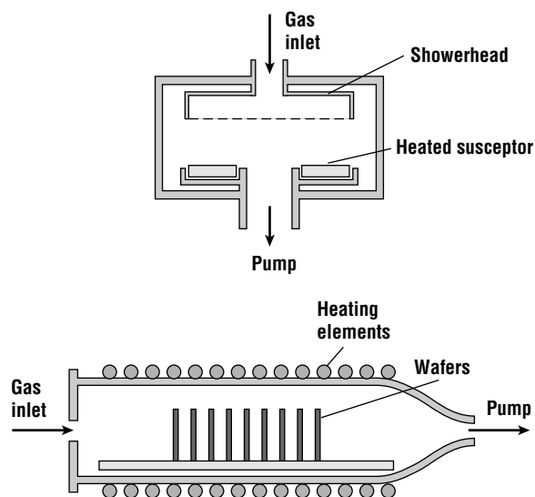
Figure 13.12 Common LPCVD reactor geometries.
