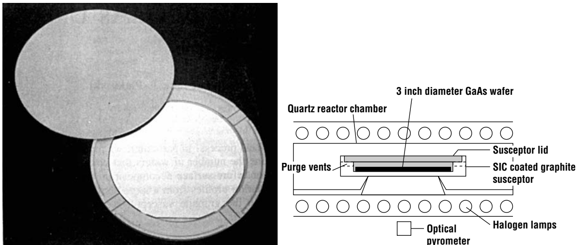
Figure 6.12 Photograph and schematic for capless arrangement for annealing GaAs (after Kazior et al. , © 1991 IEEE).
