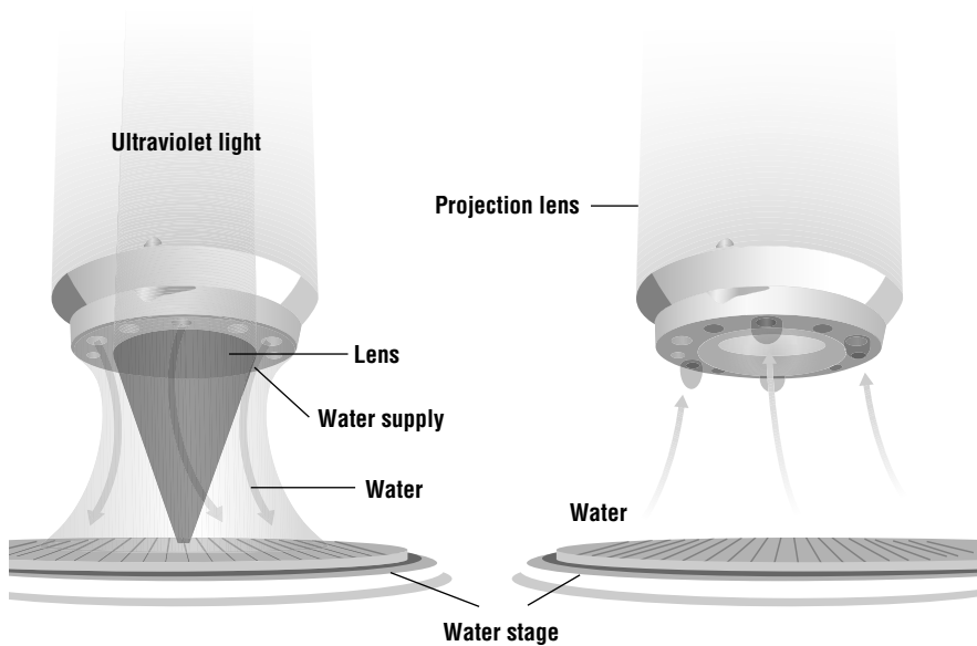
Figure 7.25 Nozzle system used by Nikon to put the water down and suction it up for each stage (from Geppert, reprinted by permission IEEE.)
