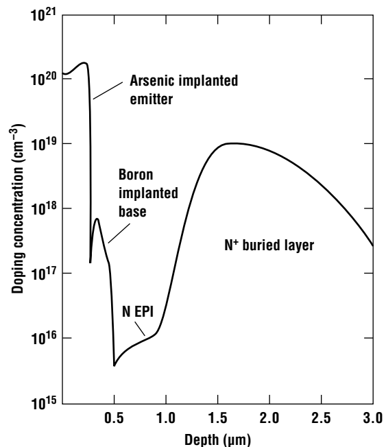
Figure 17.18 Doping profile of a typical buried collector BJT (after Ko et al., ©1983 IEEE).
