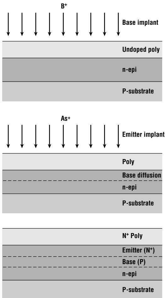
Figure 17.20 In the simple poly emitter technology, the poly is used to diffuse the emitter and intrinsic base layers.
