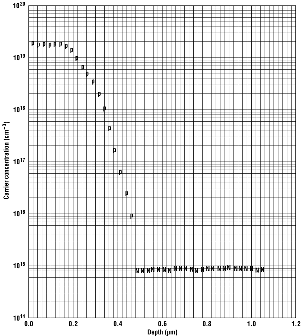
Figure 3.16 Typical spreading resistance profile showing measured carrier concentration as a function of depth ( used with permission, Solecon Labs ).
