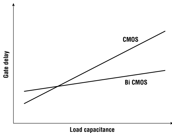
Figure 17.28 Relative gate delays for equal-area CMOS and BiCMOS technologies.
