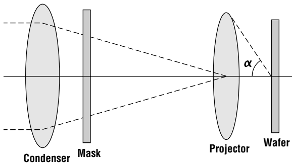
Figure 7.21 Schematic for the optical train of a simple projection printer.
