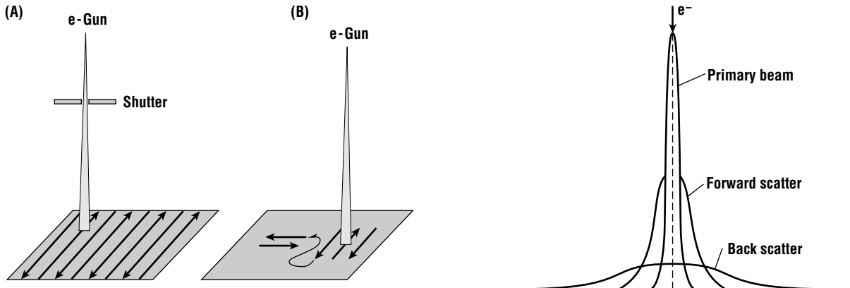
Figure 9.9 A comparison of scanning methodologies: raster scan (A) and vector scan (B).
