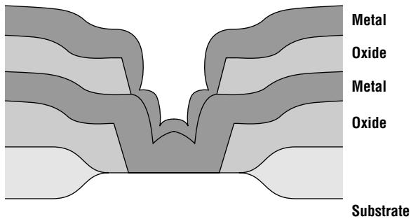
Figure 15.32 Nonplanarized plug structure consisting of a coincident contact and via.
