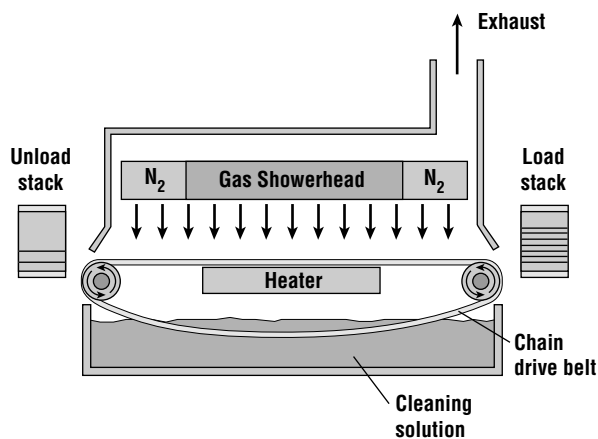
Figure 13.9 Simple continuous-feed atmospheric pressure reactor (APCVD).
