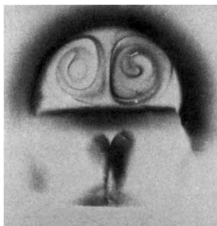
Figure 13.6 Flow field for a square cross section CVD reactor showing roll cells ( after Moffat ). Roll cells in hemispherical tubes at 760 torr (left) and 160 torr (right) ( after Takahashi et al. , reprinted by permission of the publisher, The Electrochemical Society ).
