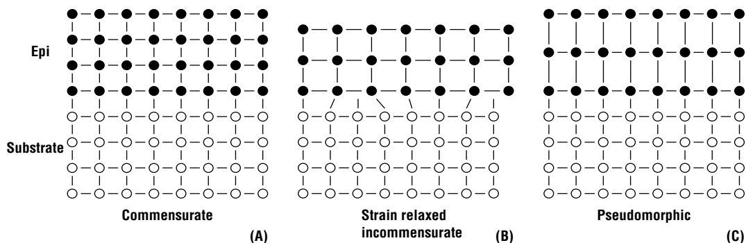
Figure 14.15 Epitaxial growth processes can be divided into (A) commensurate, (B) strain relaxed incommensurate, and (C) incommensurate but pseudomorphic.
