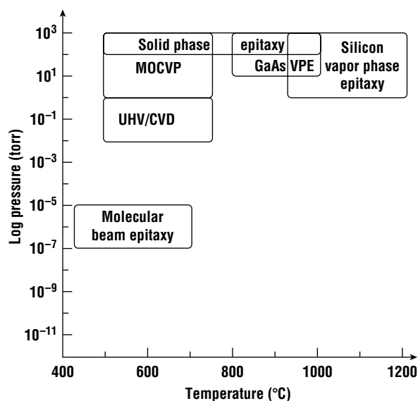
Figure 14.14 Temperature and pressure regimes of various epitaxial growth techniques.
