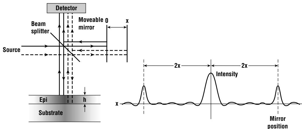
Figure 14.11 A Fourier transform infrared spectroscopy system. Infrared light is used, since silicon is nearly transparent in this region.
