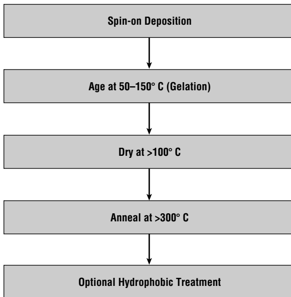
Figure 15.34 Process sequence for a typical aerogel film (after Ramos et al.).
