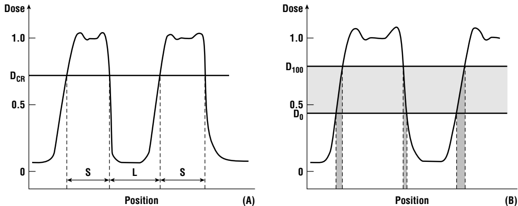
Figure 7.10 Plot of dose versus position on the wafer. Dose is given by the intensity of the light in the aerial image multiplied by the exposure time. Typical units are millijoules per centimeter squared ( \text{mJ}/\text{cm}^2 ).
