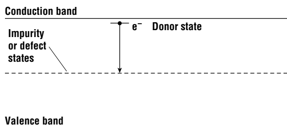
Figure 15.15 Deep levels necessary for forming a semi-insulating substrate.
