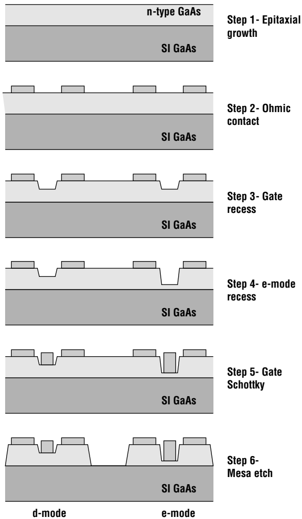
Figure 17.4 Process flow for an etched-channel E/D technology.
