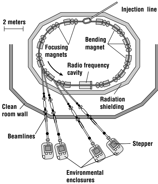
Figure 9.16 Basic schematic of an electron storage ring for XRL. Several exposure stations are indicated (after Glendenning and Cerrina, reprinted by permission, Noyes Publications).
