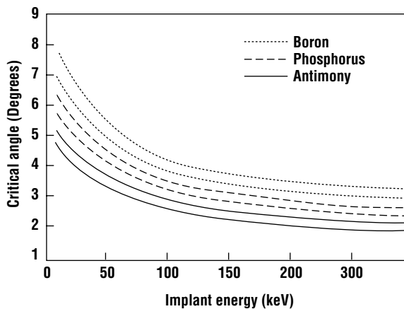
Figure 5.12 Critical angle at which channeling begins for common impurities in silicon. For each impurity, the upper curve is implanting into \langle 111 \rangle substrates. The lower curves correspond to \langle 100 \rangle substrates.
