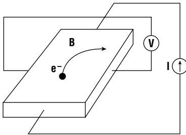
Figure 3.15 The Hall effect is able to simultaneously measure the carrier type, mobility, and sheet concentration.
