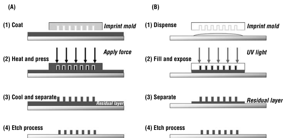
Figure 9.32 Process diagrams for (A) thermal nanoimprint lithography (NIL) and (B) ultraviolet-assisted NIL. In both processes, a mold is pressed into a soft material to form a physical relief image of the mold ( reproduced by permission of the MRS bulletin, from Ref. 103 ).
