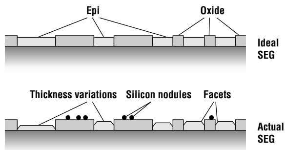
Figure 14.12 A cross-sectional view of selective epitaxial growth.
