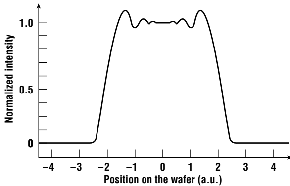
Figure 7.7 Typical near field (Fresnel) diffraction pattern.
