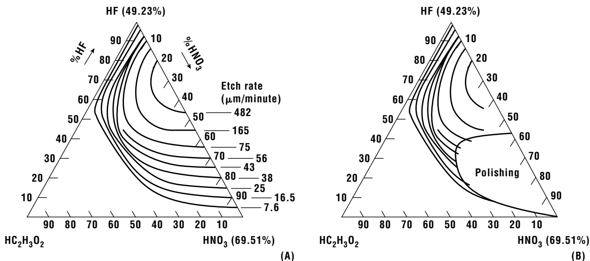
Figure 11.4 The etch rate of silicon in HF and \text{HNO}_3 (after Schwarz and Robbins, reprinted by permission of the publisher, The Electrochemical Society Inc.).
