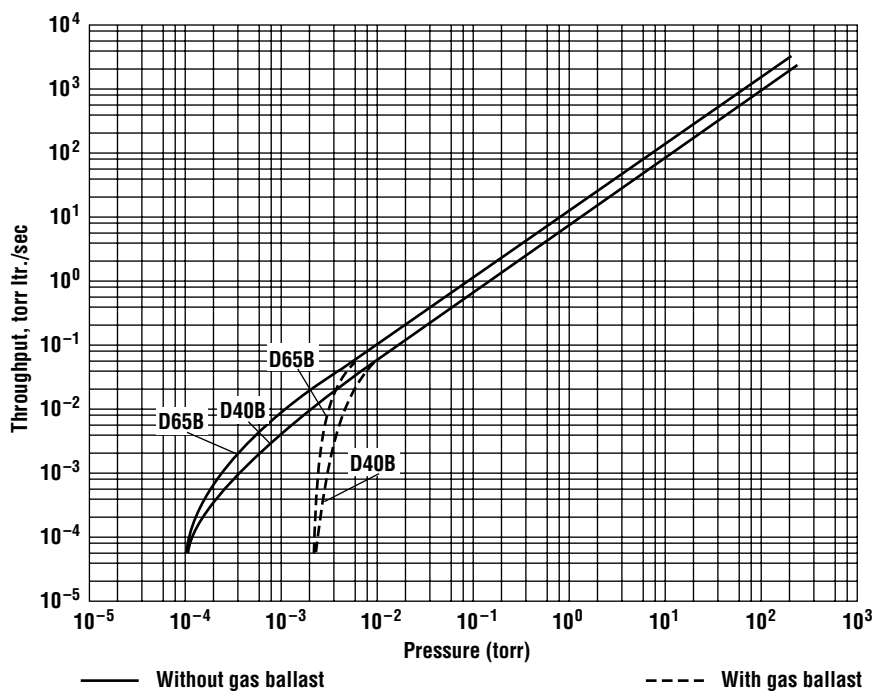
Figure 10.6 The pumping characteristics of Leybold D65® and D40® two-stage rotary vane vacuum pumps with and without gas ballasting (courtesy Leybold).
