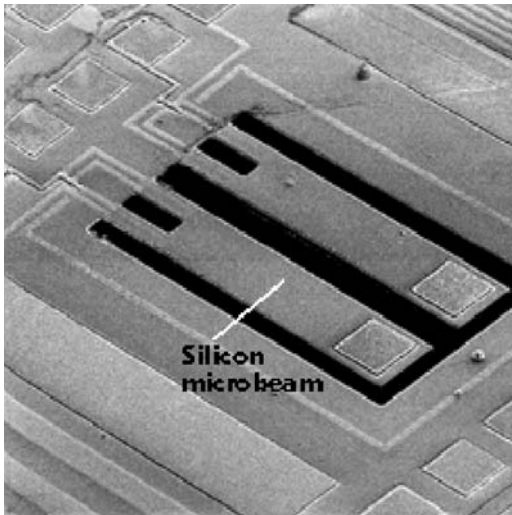
Figure 19.21 A pair of silicon cantilever beams used to detect airborne contaminants prior to deposition of the polymer layer (after Baltes et al. [47], © 1998 IEEE).
