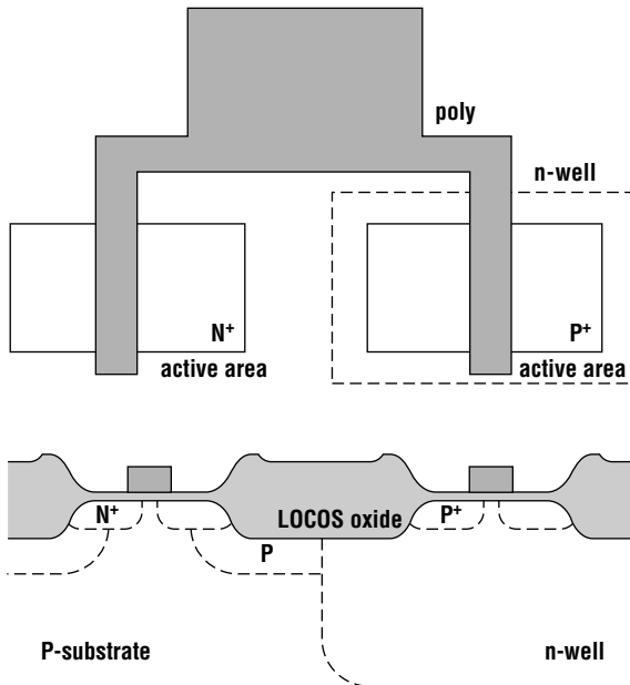
Figure 16.8 Top and cross-sectional views of a CMOS inverter after source/drain implants.
