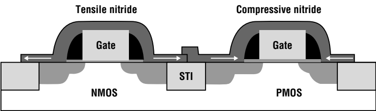
Figure 16.24 Example of uniaxial strained technology using nitrides with different stoichiometries to induce stress in the channel (from Thompson et al., reprinted by permission at IEEE).
