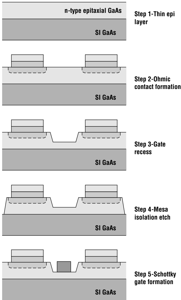
Figure 17.2 Process flow for a simple mesa-isolated MESFET. The first step can be replaced with an Si implant and anneal as discussed.
