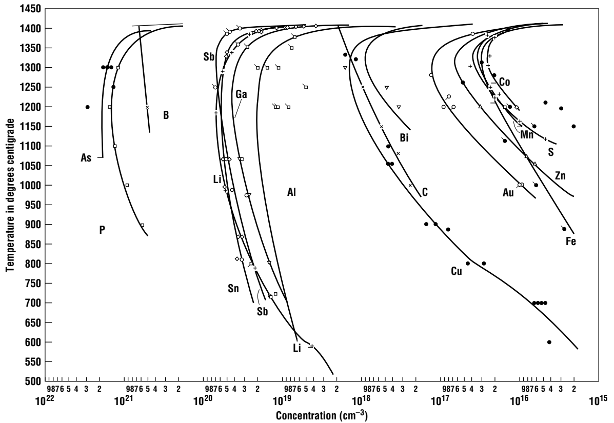
Figure 2.4 Solid solubility of common silicon impurities: note that concentration increases to the left ( all rights reserved, reprinted with permission, © 1960 AT & T ).
