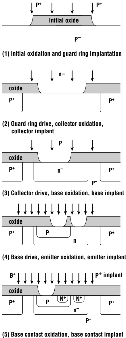
Figure 17.17 Process flow for a simple junction-isolated, triple-diffused bipolar technology.
