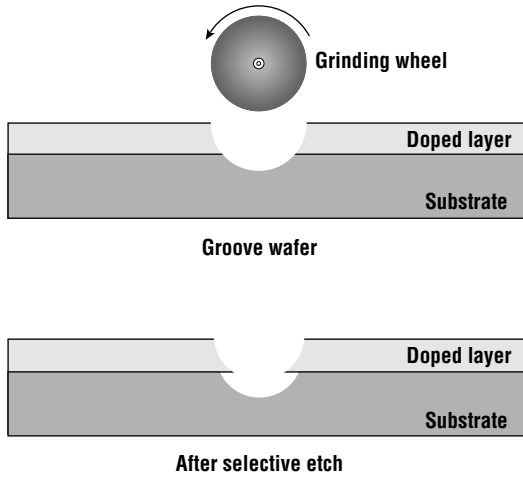
Figure 3.14 In junction staining, a cylinder is used to groove the wafer. A doping-sensitive etch then removes part of the top layer. The junction depth can be found from the known diameter of the cylinder and the measured width of the lower abraded groove.
