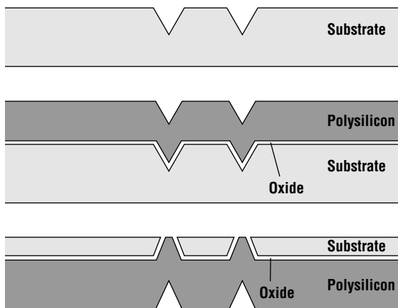
Figure 15.13 Dielectric isolation (DI) process for forming silicon on insulator.
