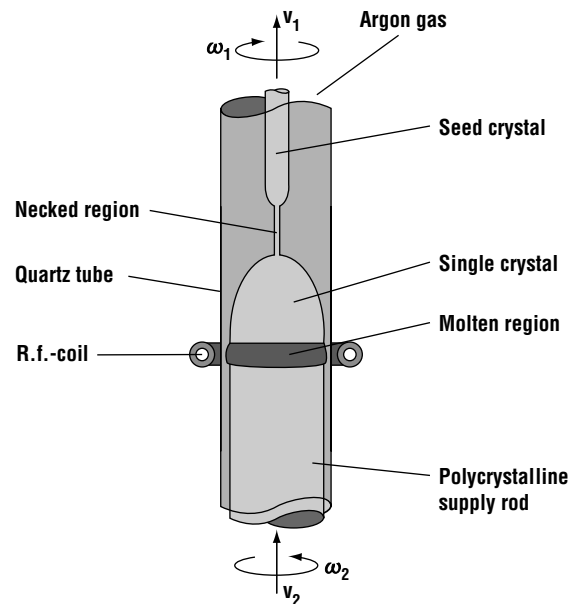
Figure 2.21 Schematic of a float zone refining system.
