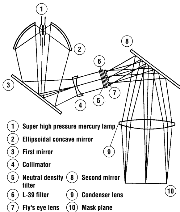
Figure 7.15 Schematic of a typical source assembly for a contact/proximity printer (after Jain).
