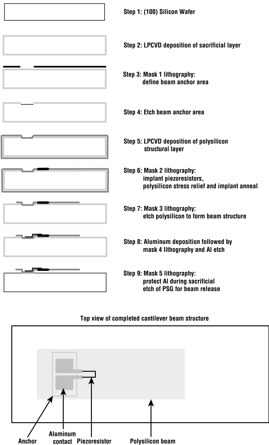
Figure 19.26 Surface micromachining process flow for a cantilever beam structure with a piezoresistor.
