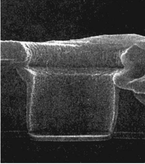
Figure 12.29 Cross section electron micrograph of a moderately high aspect ratio contact that has been sputter-deposited with TiN (after Kohlhasse, Mändl, and Pamler, reprinted by permission, AIP).
