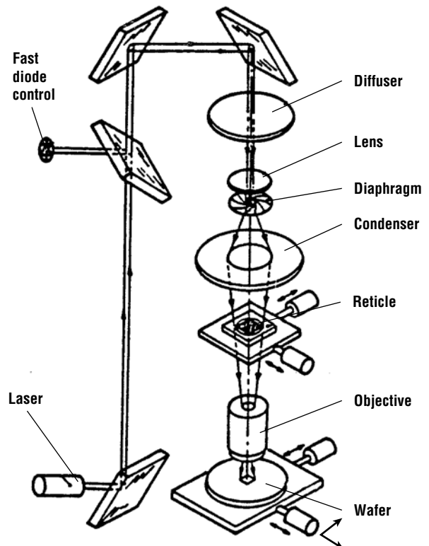
Figure 7.17 Optical train for an excimer laser stepper (after Jain).
