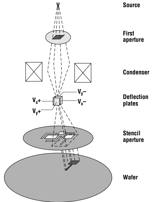
Figure 9.6 The use of stencil masks with EBL to improve system throughput. This type of exposure is useful only for exposing highly repetitive designs.
