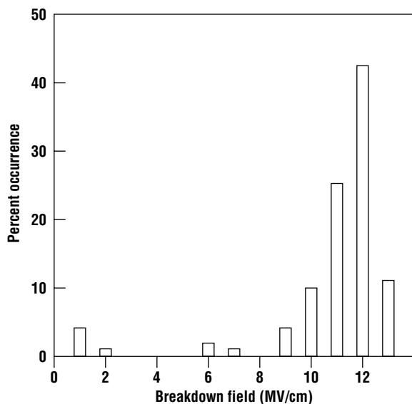
Figure 4.9 Typical breakdown histogram for an oxide.
