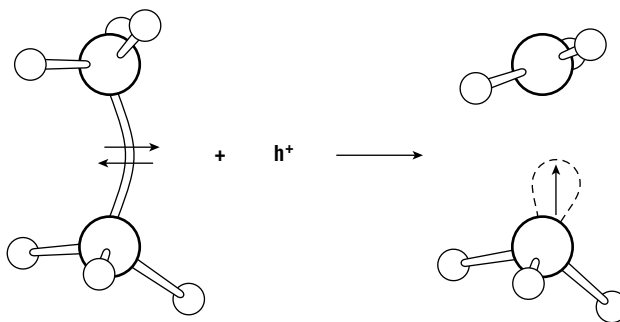
Figure 9.29 An example of a trap creation process believed to occur upon x-ray irradiation of MOS structures. The larger atoms are silicon, the smaller are oxygen. Due to an oxygen vacancy, the two silicon atoms are initially bonded together.
