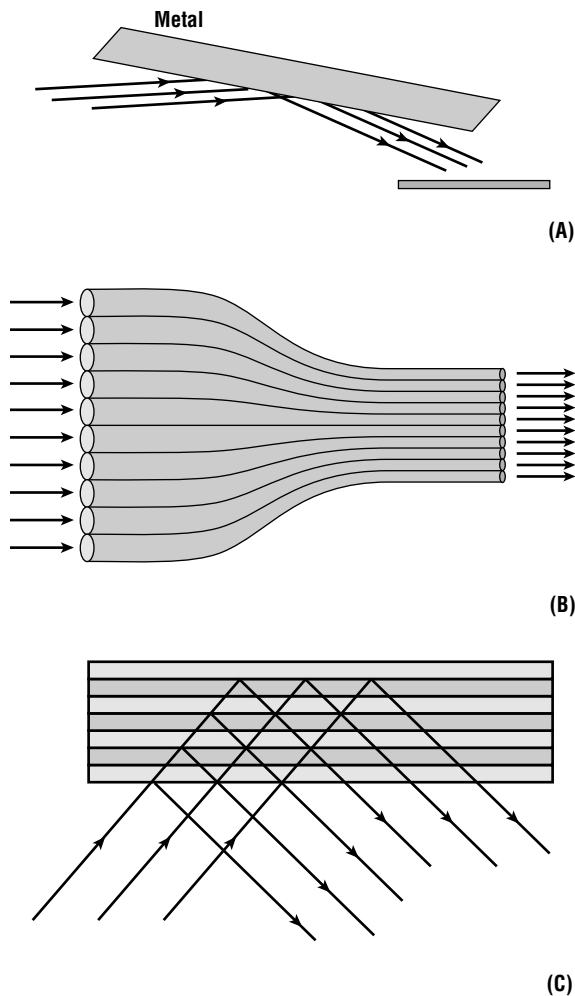
Figure 9.20 Possible choices for x-ray optics systems include glancing angle metal mirrors (A), Kumakhov lenses (B), and multilayer mirrors (C).
