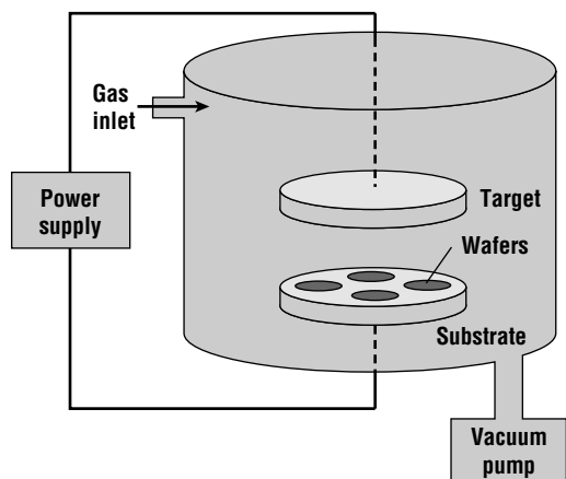
Figure 12.12 Chamber for a simple parallel-plate sputtering system.
