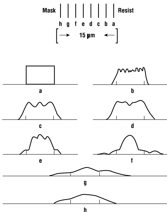
Figure 7.20 Intensity as a function of position on the wafer for a proximity printing system where the gap increases linearly from g = 0 to g = 15 \text{ }\mu\text{m} (after Geikas and Ables).
