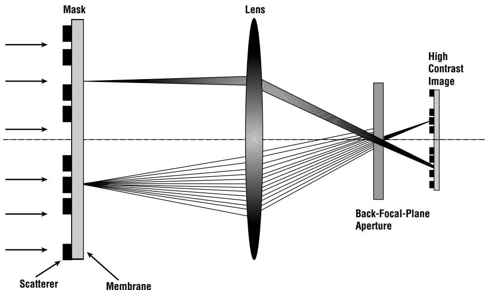
Figure 9.25 SCALPEL principle of operation.
