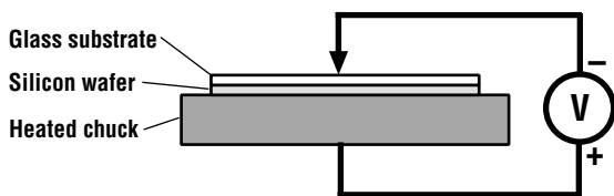
Figure 19.19 Typical electrostatic (anodic) bonding setup.
