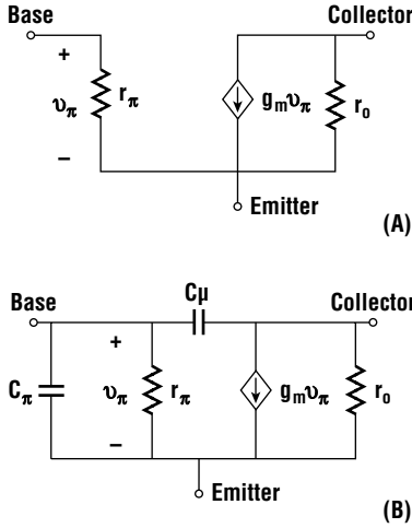
Figure 17.14 Small-signal models of the bipolar transistor at (A) low frequency and (B) high frequency.
