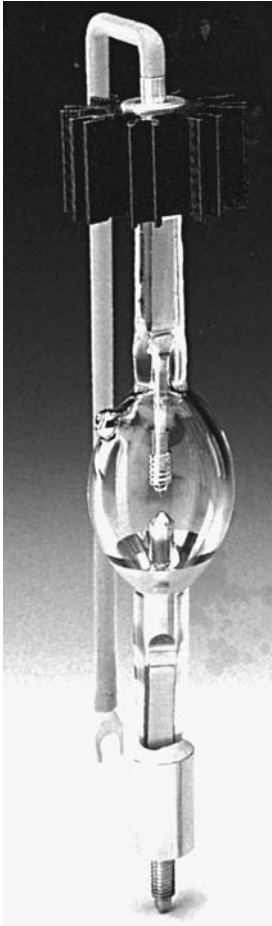
Figure 7.13 Typical high pressure, short arc mercury lamp (courtesy Osram Sylvania).
