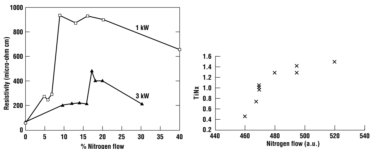
Figure 12.28 Resistivity and composition of reactively sputtered TiN as a function of the \text{N}_2 flow in the sputtering chamber (after Tsai, Fair, and Hodul, reprinted by permission, The Electrochemical Society , and Molarius and Orpana, reprinted by permission, Kluwer Academic Publishing ).
