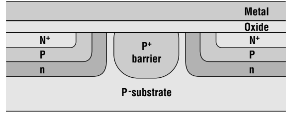
Figure 15.5 Guard ring isolation for the bipolar technology from Figure 15.3.
