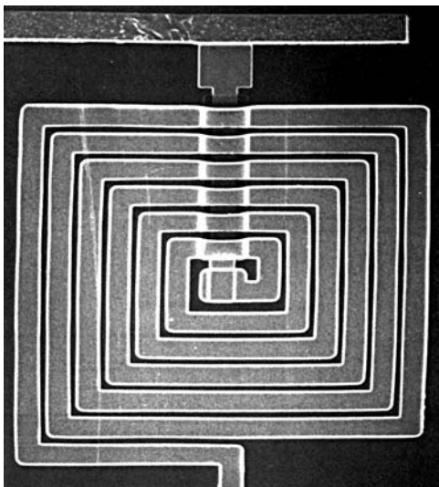
Figure 17.10 Completed spiral inductor using an air bridge crossover (after Sciater, reprinted by permission, TAB Books, Inc.).
