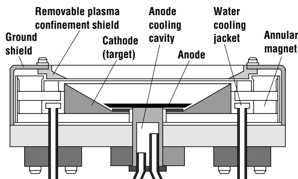
Figure 12.19 Cross-sectional diagram of an S-Gun® sputtering source (courtesy Varian Associates).
