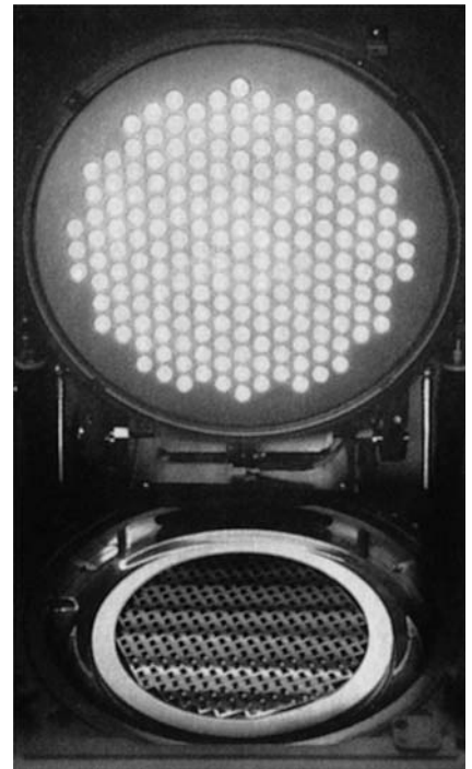
Figure 6.16 The Applied Materials Centura RTP Honeycomb source in the lifted position. The wafer is in the lower part of the photograph (courtesy Applied Materials).
