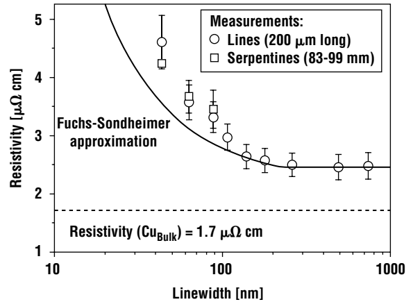
Figure 15.37 Example of the effect of linewidth on the measured resistivity of copper lines (from Steinhogel et al., reprinted with permission from Journal of Applied Physics. Copyright 2005, American Institute of Physics).
