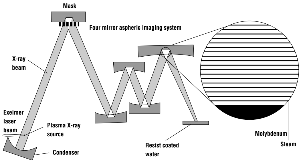
Figure 9.24 An x-ray projection lithography system using x-ray mirrors and a reflective mask (after Zorpette, reprinted by permission, © 1992 IEEE).
