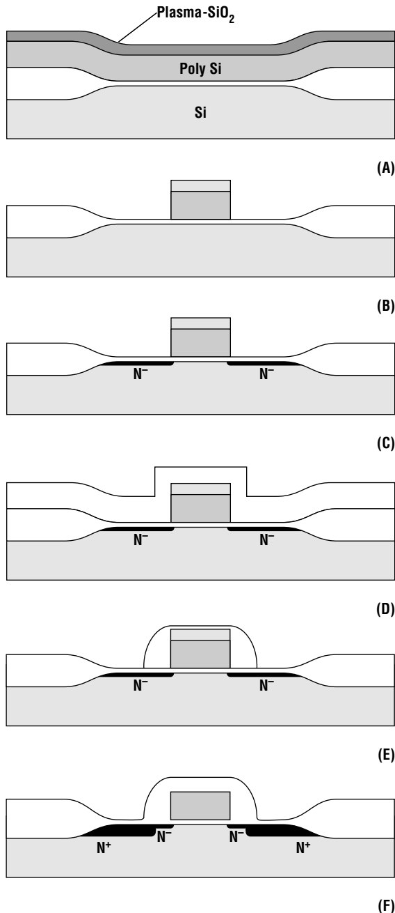
Figure 16.17 Common lightly doped drain (LDD) process sequence.
