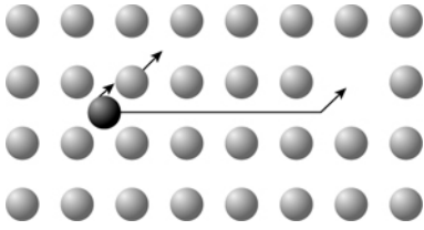
Figure 3.6 The kick-out (left) and Frank–Turnbull mechanisms (right).
