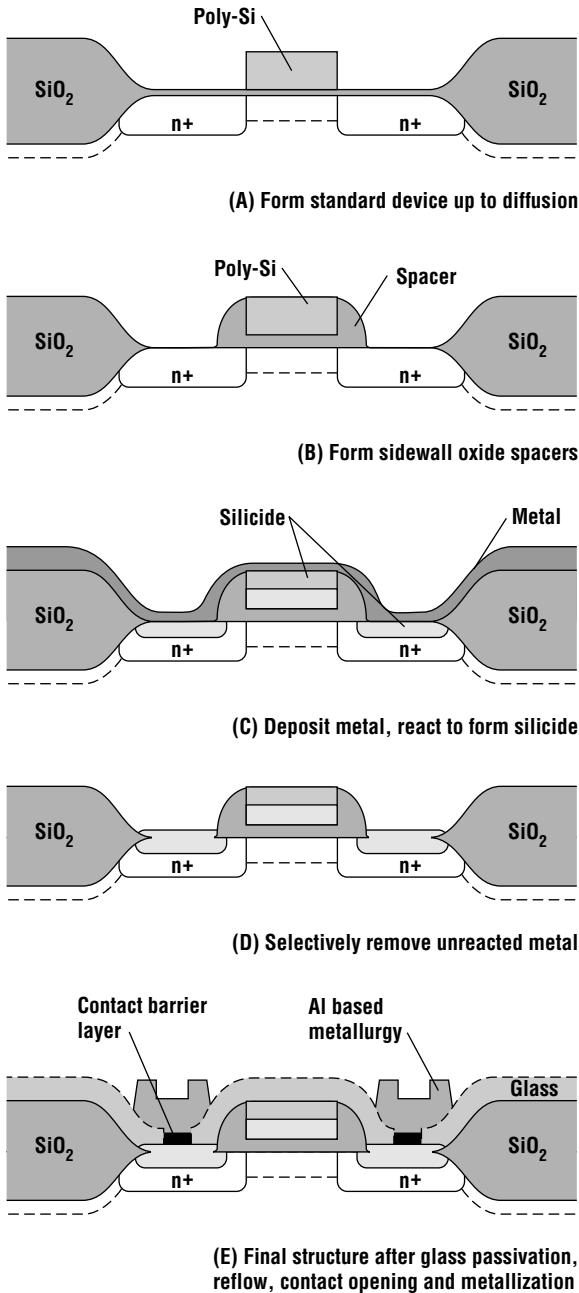
Figure 16.14 Common salicide process sequence (after Ting, © 1984 IEEE).
