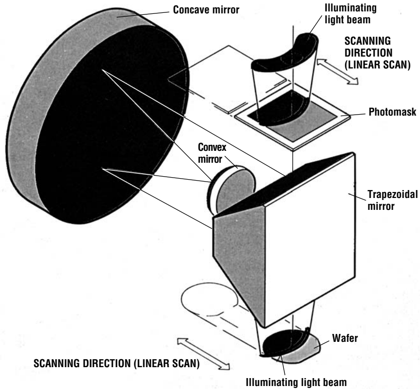
Figure 7.23 Schematic for the operation of a scanning mirror projection lithography system ( courtesy of Canon U.S.A. ).
