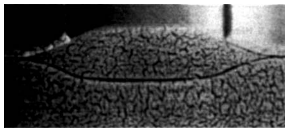
(A) Standard LOCOS—800Å Nitride/300Å Oxide
