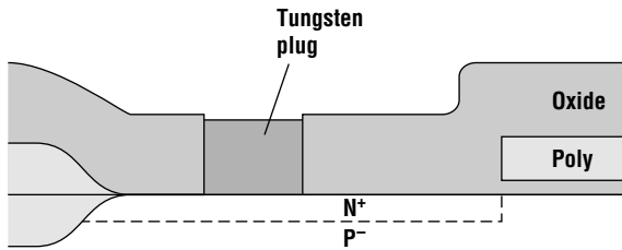
Figure 15.26 Tungsten plug structure.
