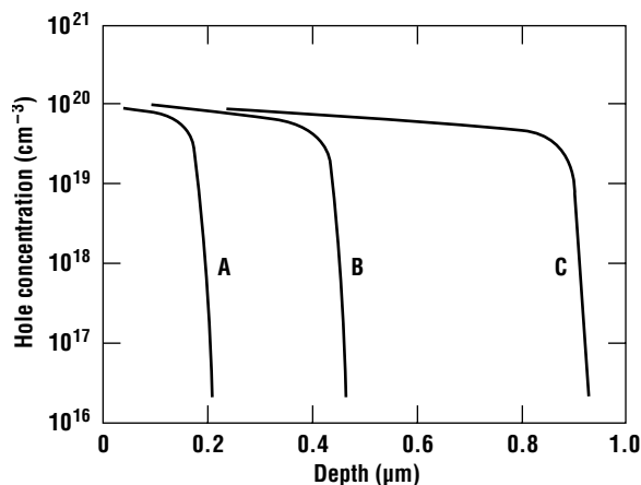
Figure 3.10 Predeposition diffusions of zinc into GaAs at 600°C for 5, 20, and 80 min (after Field and Ghandi, used with permission, Electrochemical Society).
