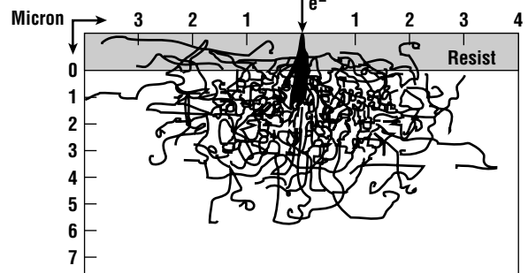
Figure 9.10 Monte Carlo simulation of electron trajectories during an EBL exposure. The upper curve indicates the forward- and backscattered components of the beam (after Hohn, reprinted by permission, SPIE).
