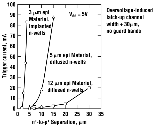
Figure 16.19 Effects of epitaxial layer thickness on latchup (from ref. 62).
