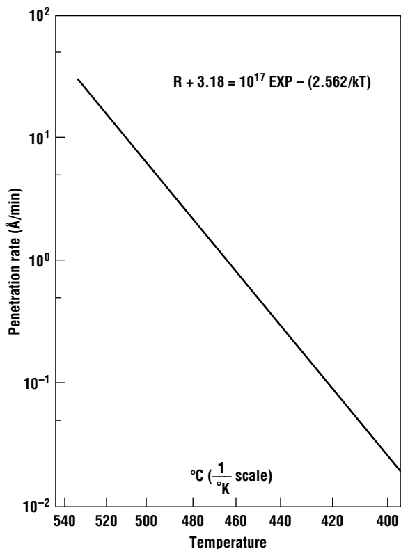
Figure 15.23 Aluminum penetration rate through aluminum oxide as a function of temperature (after Wolf [1], reprinted by permission, Lattice Press).
