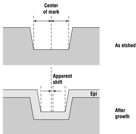
Figure 14.10 A schematic diagram of pattern shift. Alignment marks are etched into the wafer, but nonuniform growth rates cause the mark position to shift after growth.
