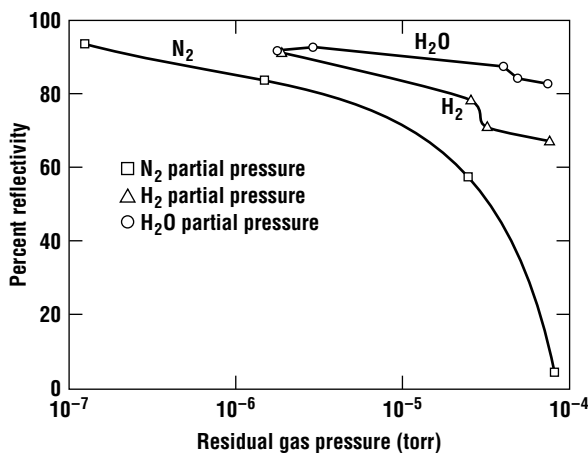
Figure 12.27 Reflectance of Al-Si layers at 400 nm as a function of the partial pressures of \text{N}_2 , \text{H}_2 , and \text{H}_2\text{O} (after McLeod and Hartsough, reprinted by permission, AIP).
