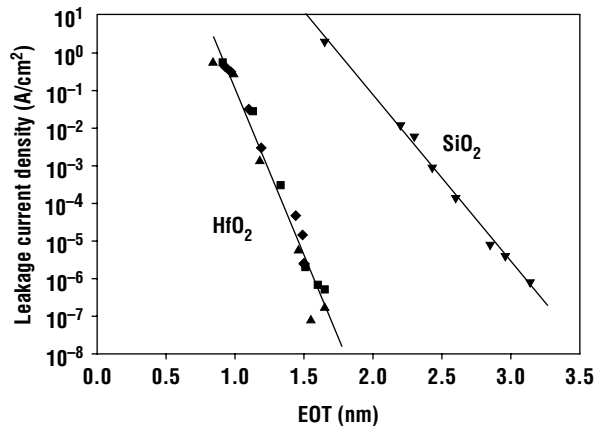
Figure 4.23 Leakage current density as a function of equivalent oxide thickness (EOT) \text{HfO}_2 and \text{SiO}_2 .
