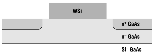
Figure 15.21 Typical GaAs MESFET structure.
