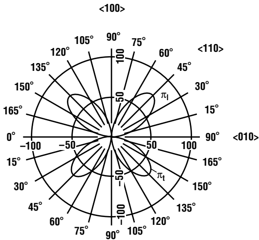
Figure 19.6 Piezoresistance coefficients \pi_t and \pi_l for the [100] plane of p-type single crystal silicon. \pi_l values are shown on the upper half and \pi_t values on the lower half. Units are 10^{-11} \text{ Pa}^{-1} . Note that the maximums are in the \langle 110 \rangle directions (after Kanda [29], © 1982 IEEE Press).
