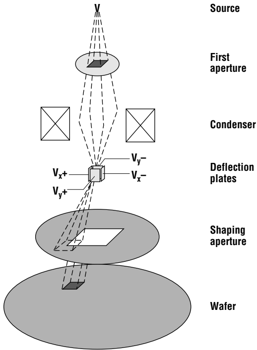
Figure 9.7 A variable shaped beam exposure system using mechanical beam stops for beam shaping. The broad beam exposes many pixels simultaneously, but dimensional control is not as reliable as in standard EBL.
