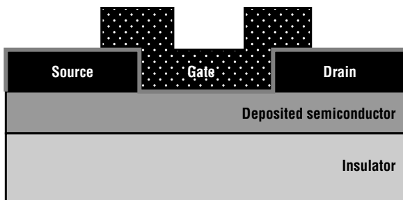
Figure 17.31 Schematic of a simple top-gate structure. Weimer's device had the source/drain contacts under the semiconductor in what is now called a staggered structure.
