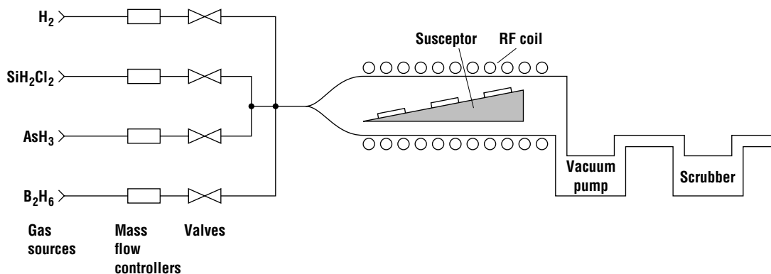
Figure 14.1 A simple VPE system. The susceptor in this chamber is inductively heated using RF power in the external coil.
