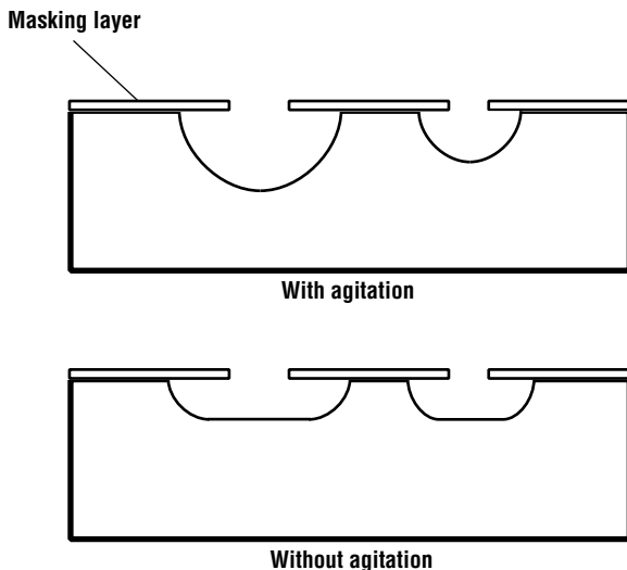
Figure 19.9 Isotropic etch cross sections showing undercutting of the etch mask and the effect of agitation on the etch profile.
