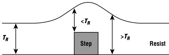
Figure 8.14 Cross-sectional view of resist as it covers a vertical step.
