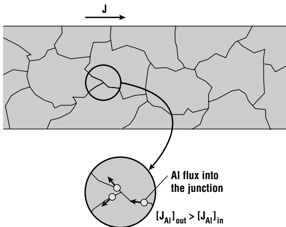
Figure 15.31 Typical point of flux divergence in an interconnect material.
