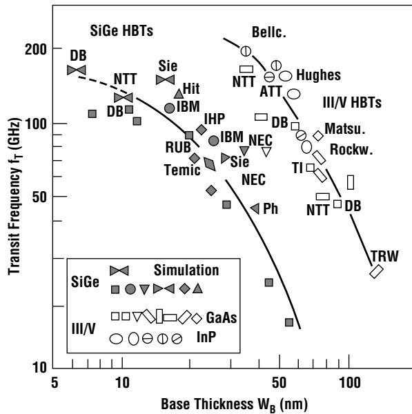
Figure 17.27 Transit frequency of GeSi, and III–V HBTs (after König, used by permission, IEEE, 1998).
