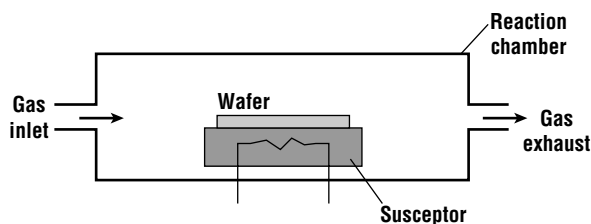
Figure 13.1 A simple prototype thermal CVD reactor.
