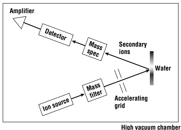
Figure 3.17 A typical SIMS arrangement. The sample is bombarded by high energy ions. The sputtered material is mass-analyzed to determine the composition of the substrate.
