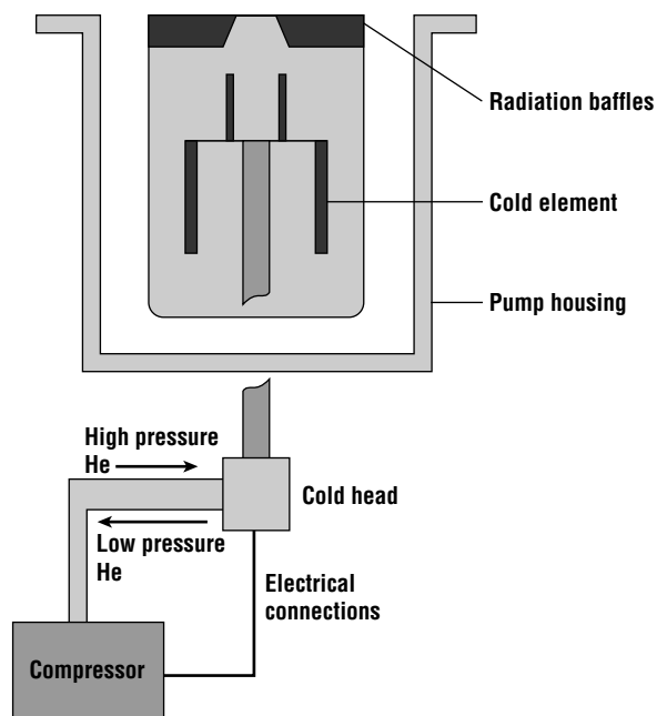
Figure 10.12 Schematic view of a typical cryopump.
