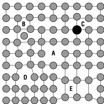
Figure 2.7 Simple 0- and 1-D semiconductor defects include: (A) vacancies, (B) self-interstitials, (C) substitutional impurities, (D) edge dislocations, and (E) dislocation loops.
