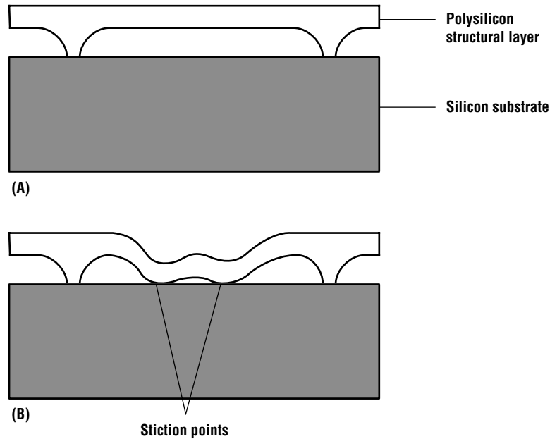
Figure 19.25 Side view of a released structure (A) without and (B) with stiction at two points.
