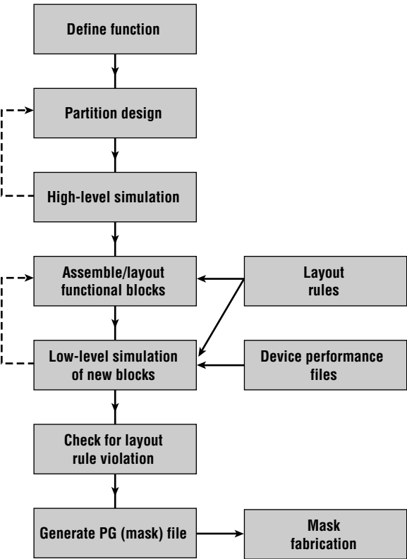
Figure 7.1 Simplified IC design process flow diagram.
