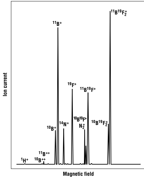
Figure 5.4 Typical mass spectrum for a BF_3 source gas (after Ryssel and Ruge, reprinted by permission Wiley).
