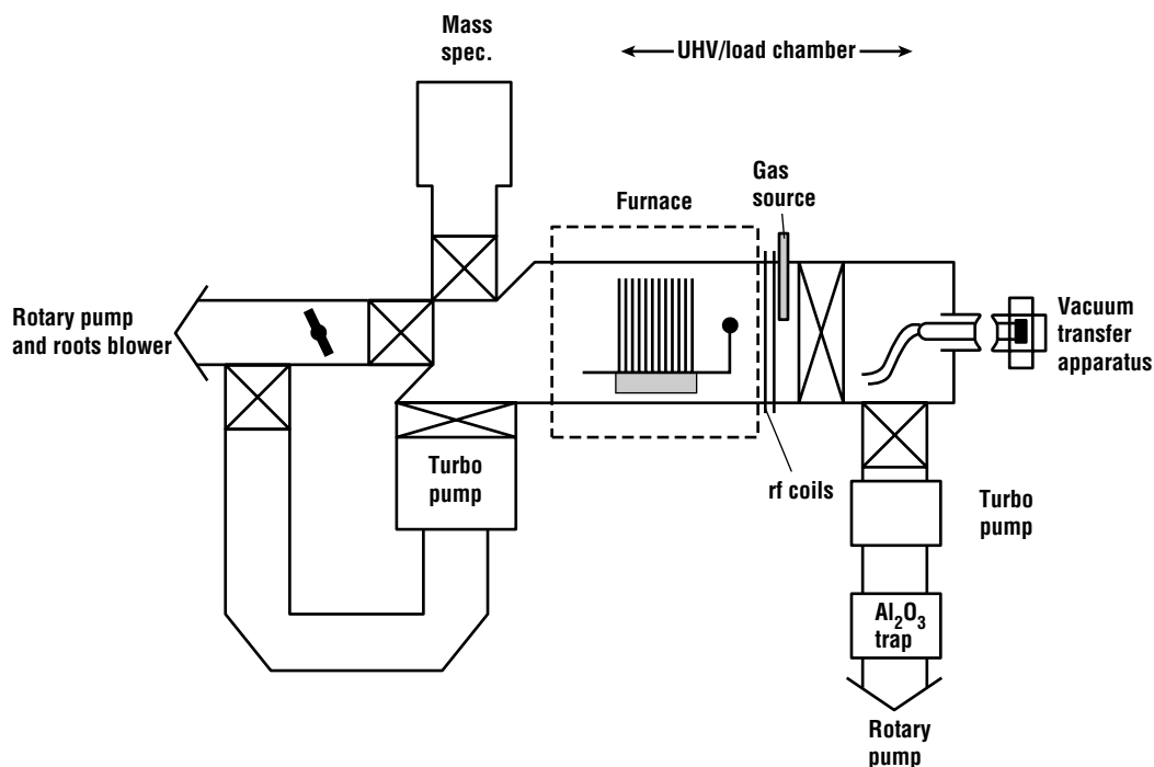
Figure 14.27 Schematic of an ultrahigh vacuum CVD epitaxial growth system (after Mayerson, ©1986 AIP).
