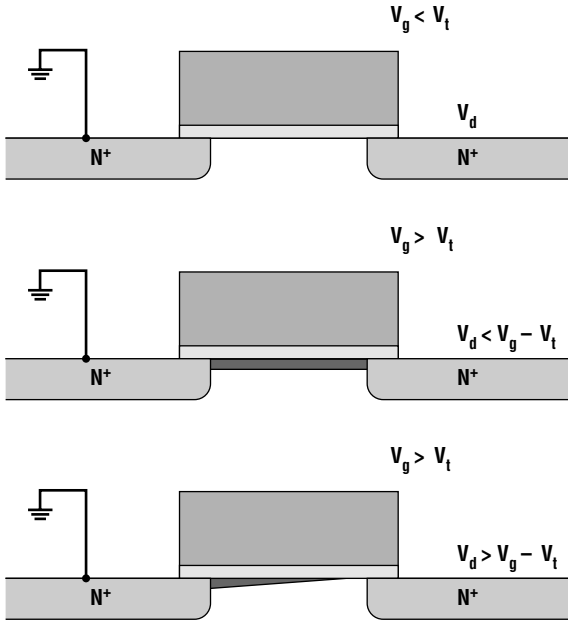
Figure 16.2 Three regions of n-channel MOSFET operation are subthreshold, linear, and saturation.
