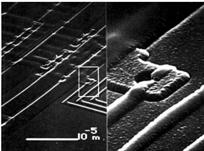
Figure 7.30 Resist lines for patterning the metal running diagonally from the lower left. On the right is an expanded view of the geometry described in Figure 7.31 (after Listvan et al.).
