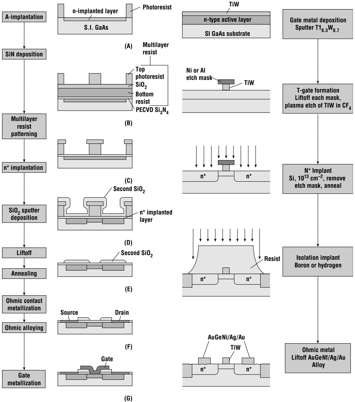
Figure 17.5 The self-aligned gate process implantation N + technology (SAINT) (after Yamaski et al. , ©1982 IEEE) and the T-gate process. The order of the last two steps of the T-gate may be reversed to reduce any isolation degradation.
