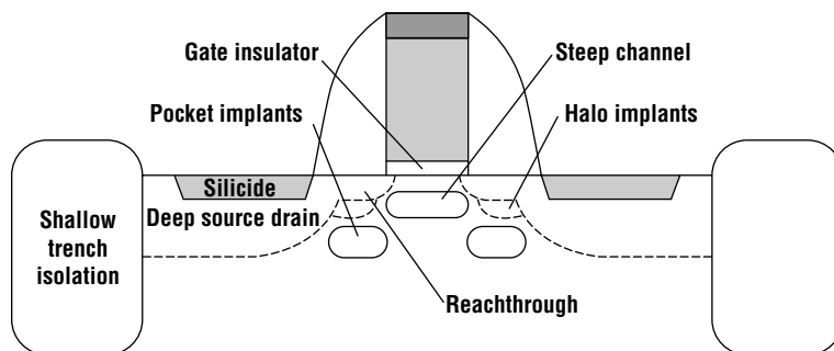
Figure 16.21 Cross section of deep submicron MOSFET showing optional channel engineering implants.
