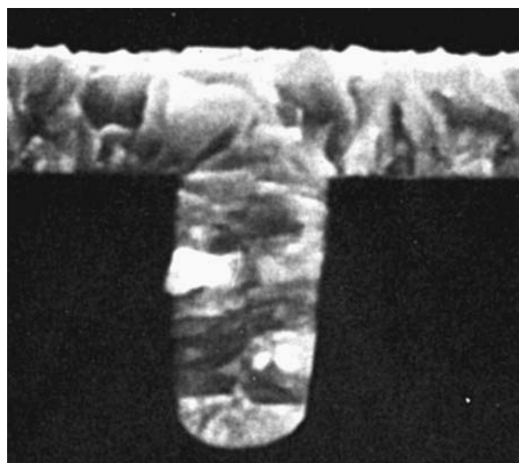
Figure 13.23 A filled contact showing the CVD tungsten morphology (after Schmitz, reprinted by permission, Noyes).
