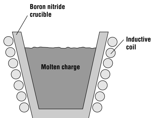
Figure 12.8 Example of an inductively heated crucible used to create moderately charged temperatures.
