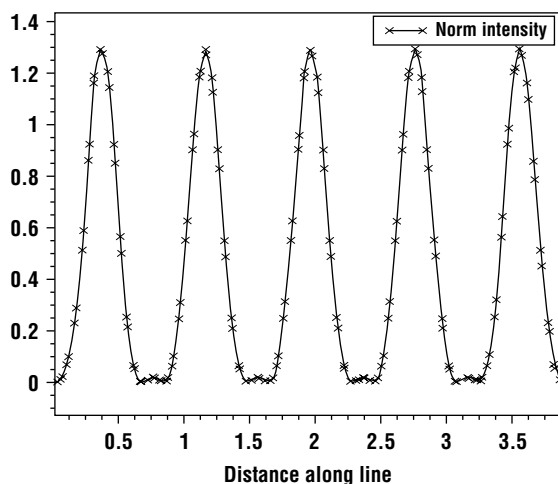
Figure 7.18 Intensity as a function of position for a 0.8\text{ }\mu\text{m} period grating ( 0.4\text{ }\mu\text{m} features) exposed at 193 nm with \text{NA} = 0.43 .
