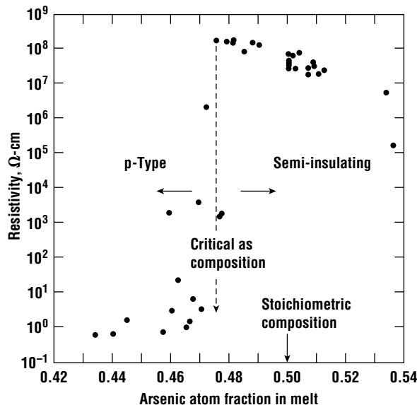
Figure 15.16 The resistivity of GaAs substrates as a function of the melt stoichiometry (after Ferry).
