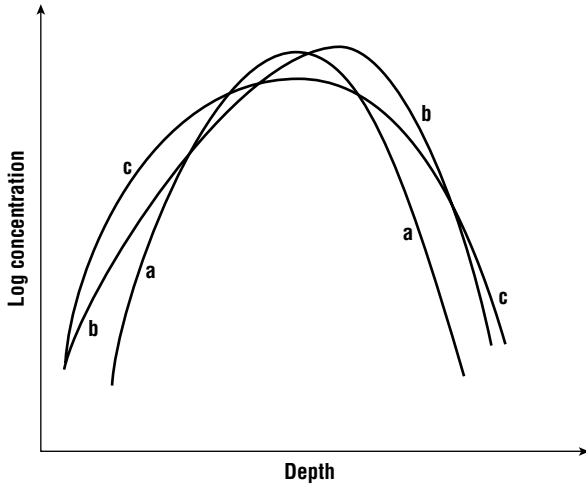
Figure 5.10 Curve (a) shows a standard Gaussian. (b) A negative skewness, which moves the peak slightly deeper and adds a tail extending toward the surface. (c) A large kurtosis flattens the peak of the distribution.
