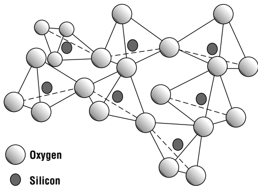
Figure 4.7 The physical structure of \text{SiO}_2 consists of silicon atoms sitting at the center of oxygen polyhedra.
