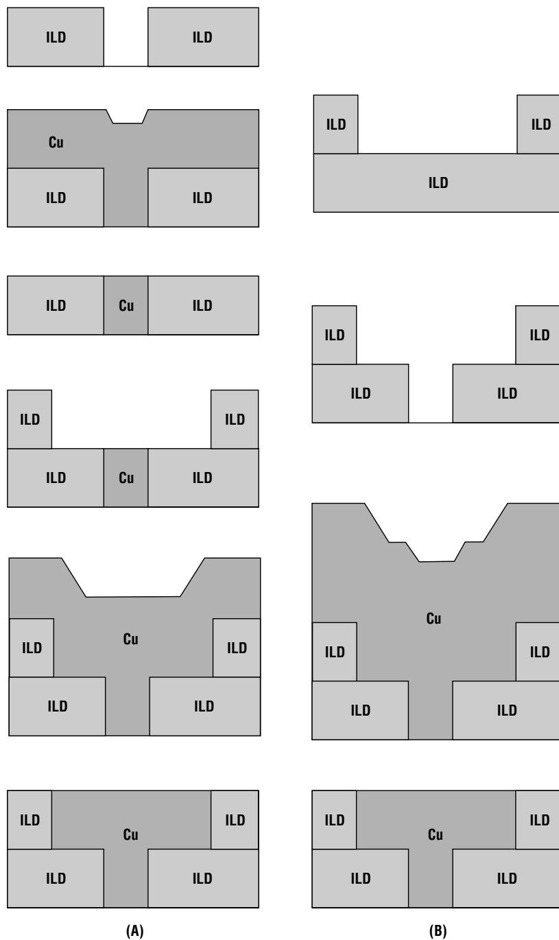
Figure 15.35 Two options for performing a dual damascene process: (A) single damascene; (B) dual damascene (after Price et al., Used with permission. Thin Solid Films , 1997).
