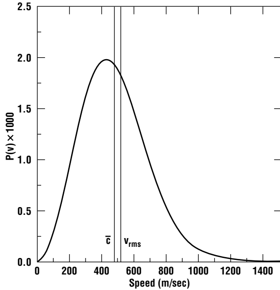
Figure 10.1 A Maxwellian speed distribution of particles; P(v) is the probability that a particular particle will have the target magnitude of velocity.
