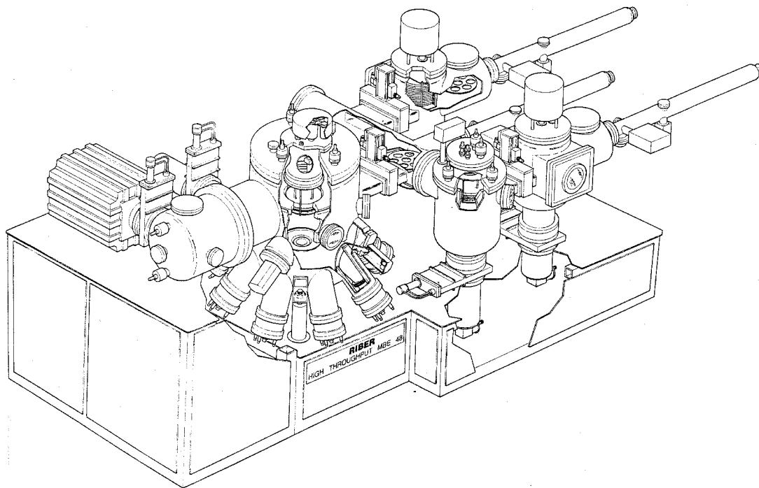
Figure 14.33 A high throughput automated MBE system includes load and unload locks, preparation, and growth chambers, all connected under UHV. Three 4-in. wafers are held on circular platens ( courtesy of RIBER S.A. ).
