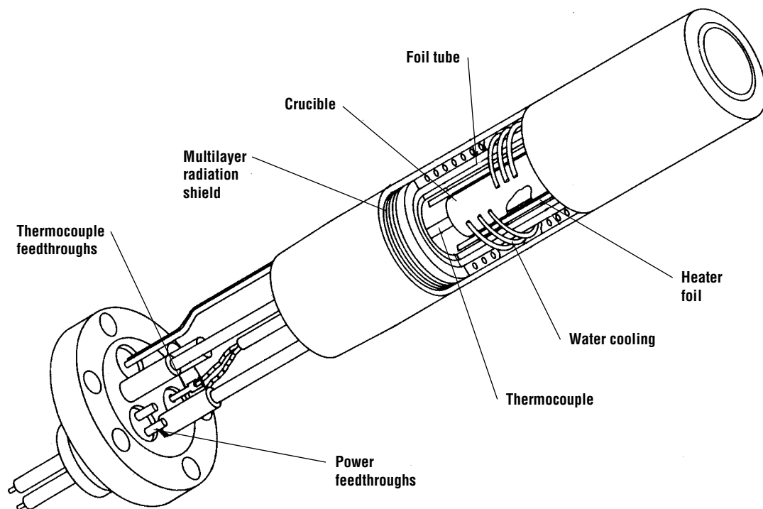
Figure 14.29 Cutaway of a simple Knudsen cell for producing thermal beam for MBE (after Davies and Williams).
