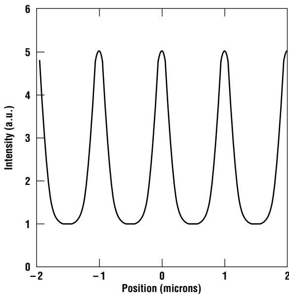
Figure 7.9 Far field image for a diffraction grating.
