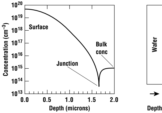
Figure 3.1 Typical concentration plot of impurities or carriers as a function of depth into the wafer. Note that these profiles are typically much less than 1% of the total wafer thickness.
