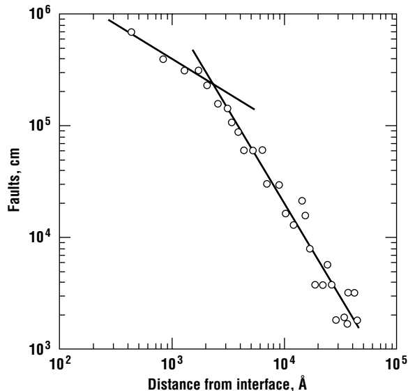
Figure 14.16 Defect density as a function of the epitaxial layer thickness for the growth of Si on sapphire ( \text{Al}_2\text{O}_3 ) (after Vasudev).
