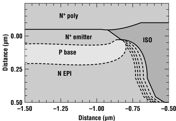
Figure 17.23 Walled transistors may have emitter–collector leakage along the isolation edge (after Ratnam et al., © 1992 IEEE).
