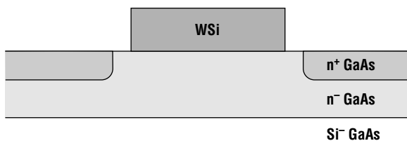
Figure 15.21 Typical GaAs MESFET structure.
