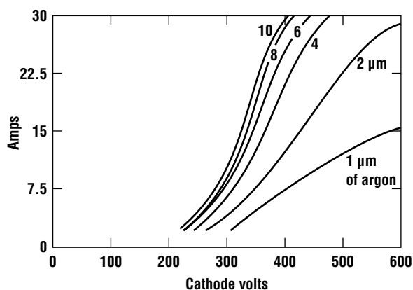
Figure 12.20 Current-voltage characteristics of a magnetron system with chamber pressure as a parameter. The lines are for 1, 2, 4, 6, 8, and 10 \mu\text{m} of Ar (after Van Vorous, reprinted by permission, Solid State Technology ).
