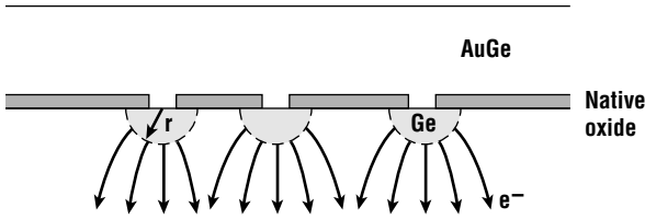
Figure 15.27 Schematic of ohmic contact to n-type GaAs showing the formation of small hemispherical contact regions and subsequent current crowding.
