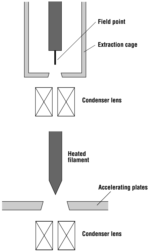
Figure 9.4 Simplified cross section schematics of field emission and thermionic emission electron guns.
