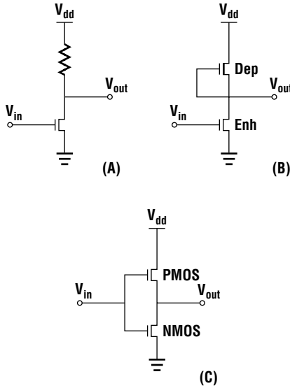
Figure 16.3 MOS inverters: (A) resistor load, (B) enhancement/depletion or E/D, and (C) CMOS.
