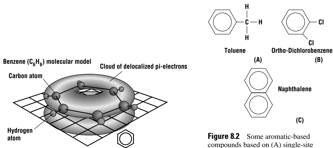
Figure 8.1 Diagram of simple benzene aromatic ring. The delocalized pi-bond electrons are in a ring that surrounds the nuclei. The symbol indicates the currently accepted ring notation.
