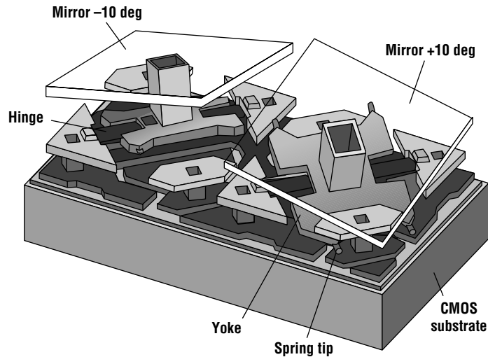
Figure 19.32 Two DMD pixels (mirrors shown as transparent) (after Van Kessel [63], © 1998 IEEE).
