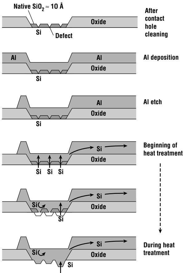
Figure 15.25 Cross-sectional diagrams of Al on Si contact formation process (after Wolf [1], reprinted by permission, Lattice Press).
