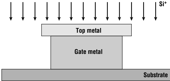
Figure 15.28 Cross-sectional schematic of a low resistance MESFET using ion implantation to reduce the contact resistance.
