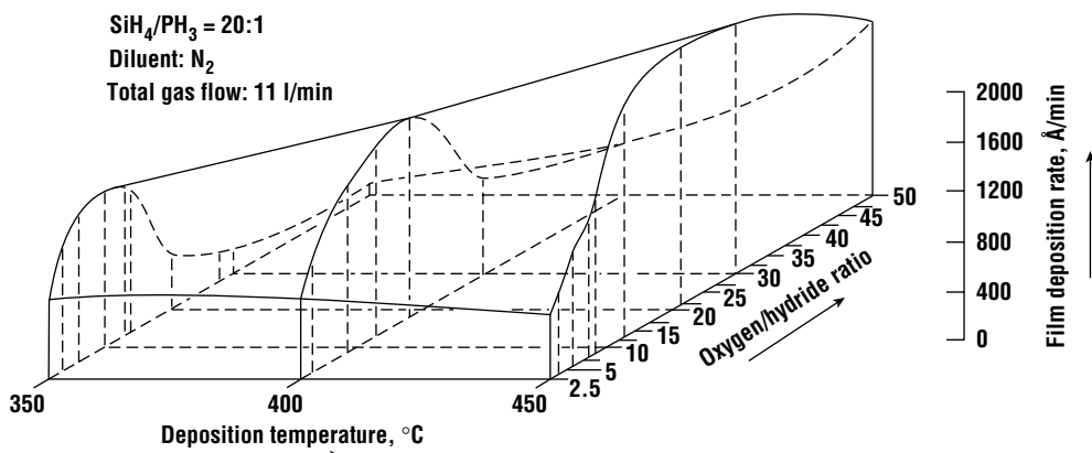
Figure 13.10 Deposition rate of PSG in an APCVD system (after Kern and Rosler, ©1977, AIP).
