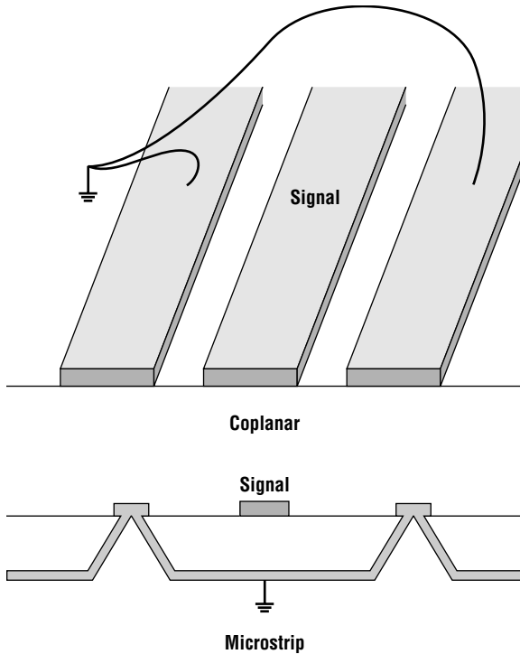
Figure 17.11 Coplanar and microstrip waveguides for MMIC interconnect.
