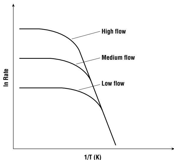
Figure 13.8 Typical deposition rates for CVD as a function of the temperature with flow rate as a parameter.
