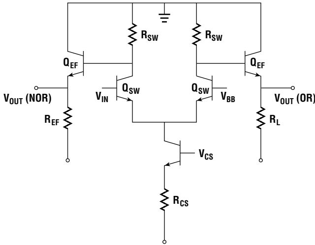
Figure 17.15 Basic ECL logic gate with inverting and noninverting output.
