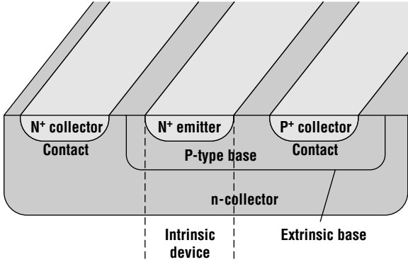
Figure 17.13 Cross-sectional view of a simple bipolar transistor showing the active or intrinsic device region and the parasitic or extrinsic regions.
