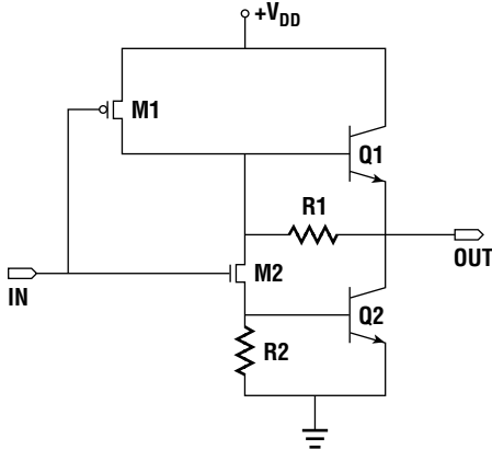
Figure 17.29 A common example of a merged gate BiCMOS structure.
