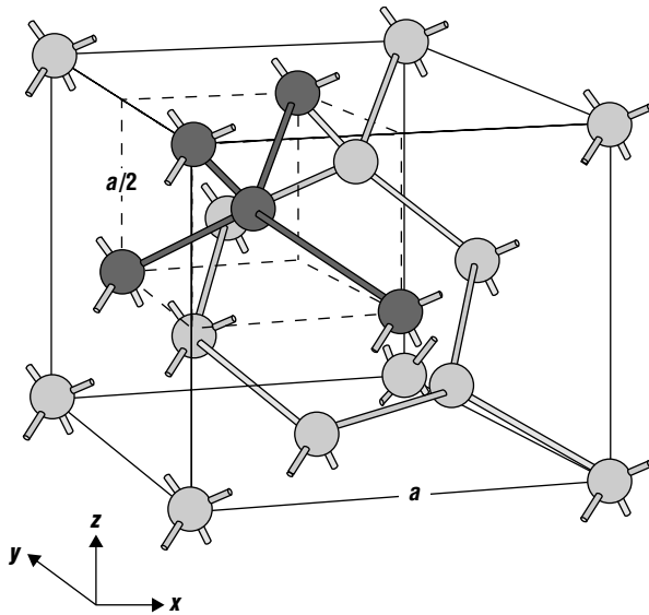
Figure 2.6 The diamond structure. The dark part of the diagram indicates the atom at (a/4, a/4, 3a/4) , and its four nearest neighbors (0, 0, a) , (a/2, a/2, a) , (0, a/2, a/2) , and (a/2, 0, a/2) .
