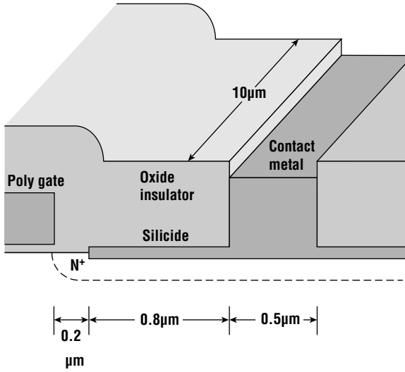
Figure 16.15 Cross section and dimensions of MOSFET example.
