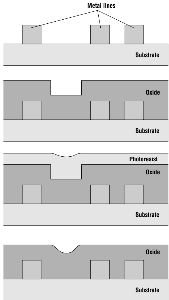
Figure 15.33 Etch-back planarization process.
