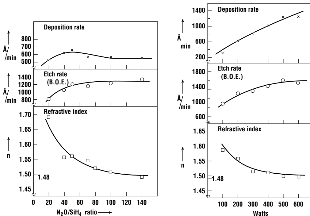
Figure 13.21 Results for the PECVD of SiO_2 (after Van de Ven, ©1981, Solid State Technology).
