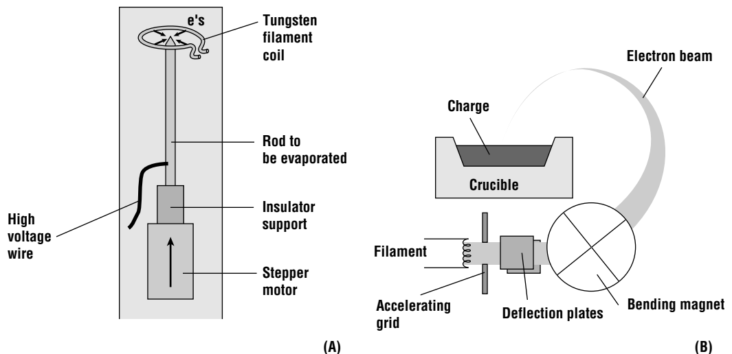
Figure 12.9 Electron beam evaporative sources. (A) A simple low flux source using a hot wire electron source and a thin movable rod. (B) A popular source using a 2707 source arc in which the beam can be rastered across the surface of the charge. The magnet must be much larger than shown to achieve the full 270° of arc.
