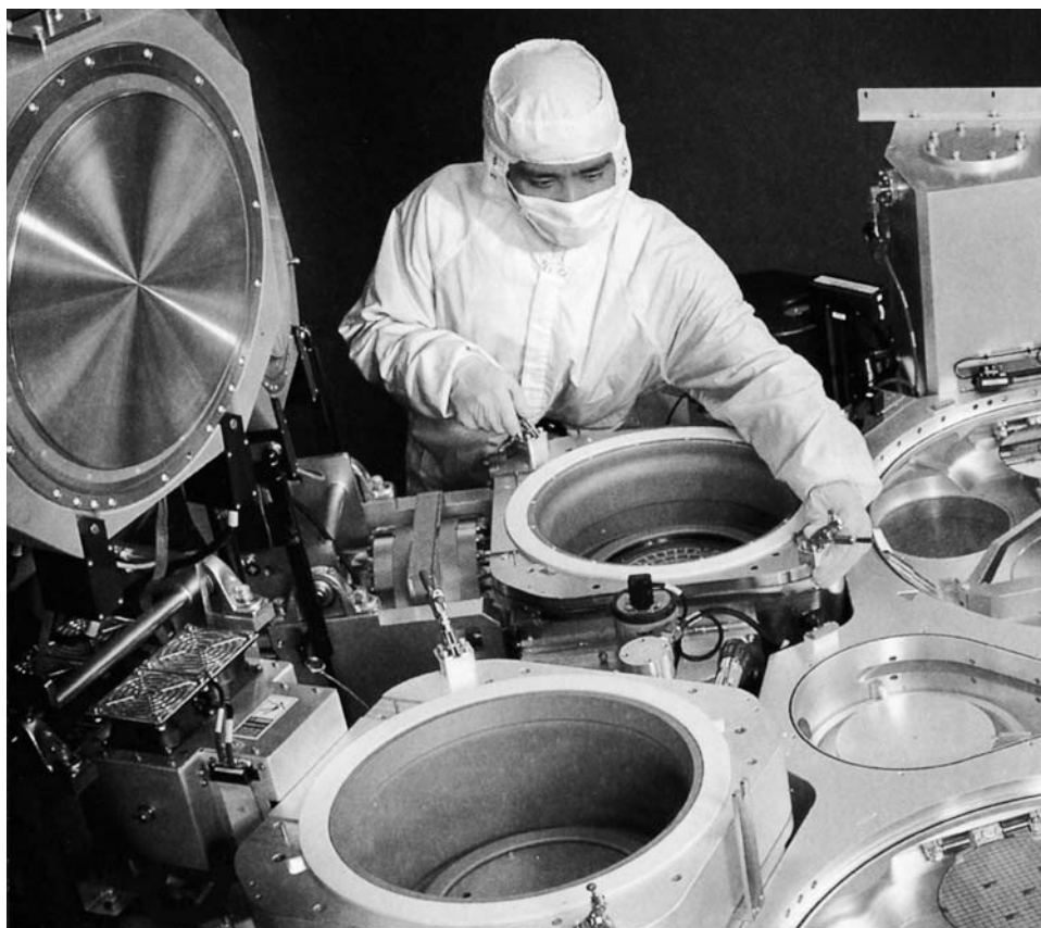
Figure 12.25 The Endura system by Applied Materials uses a number of PVD or CVD chambers fed by a central robot. For conventional and IMP sputtering, targets are hinged to open upward. Two open chambers are shown, along with the load lock ( from Applied Materials ).
