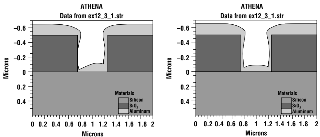
Figure 12.6 Athena simulation of the evaporation of aluminum in a 1:1 aspect ratio contact deposition conditions that reasonably approximate: simple evaporation (left) and evaporation onto a sample mounted in a rotating planetary (right).
