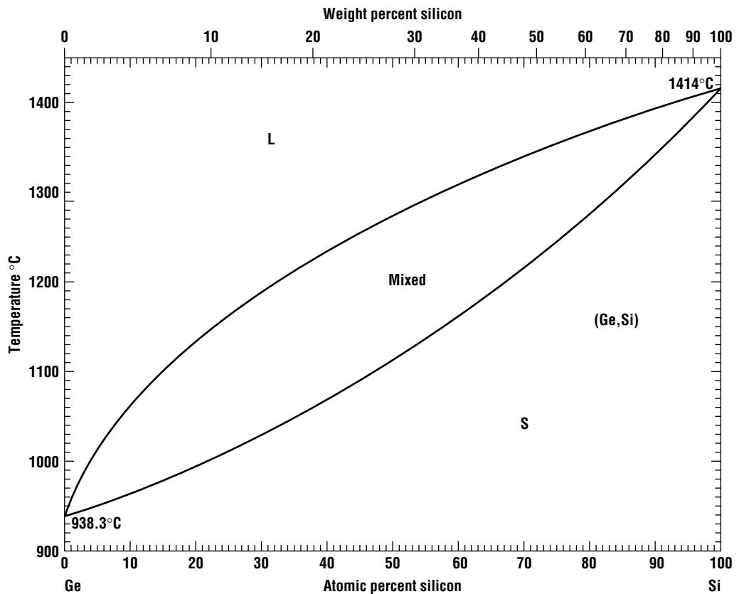
Figure 2.1 Phase diagram of Ge–Si ( courtesy of ASM International ).
