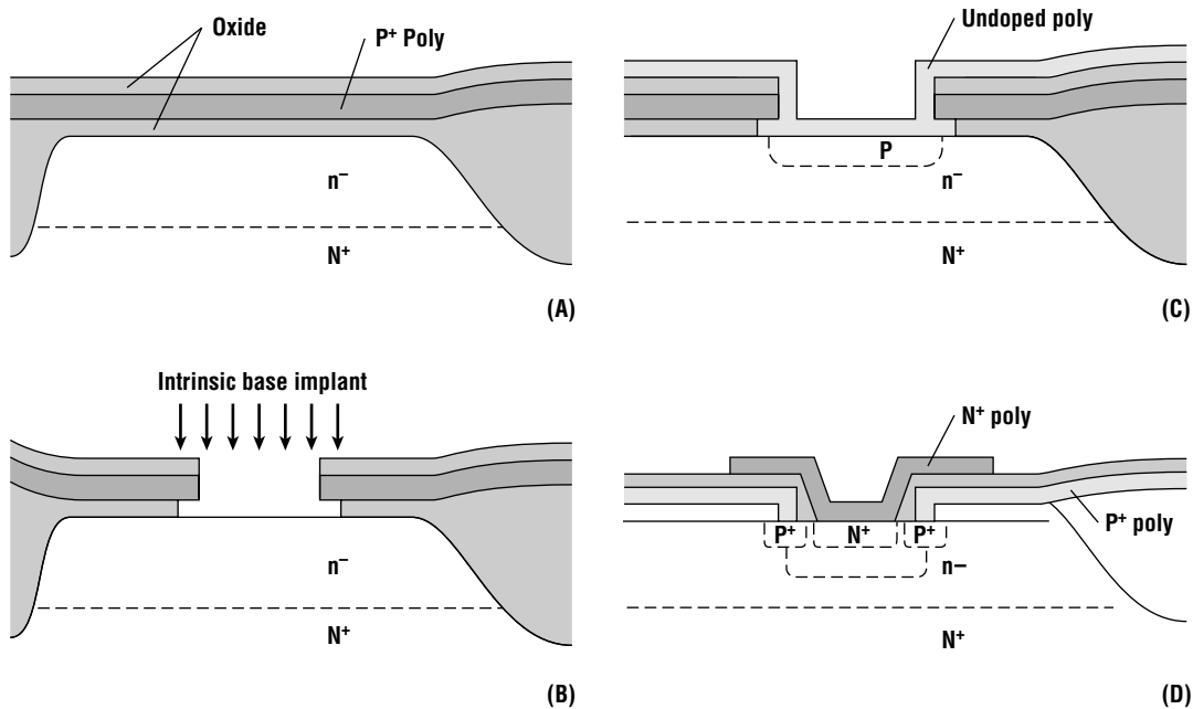
Figure 17.24 The super-self-aligned or Antipov emitter bipolar transistor.
