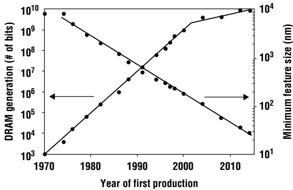
Figure 1.1 Memory and minimum feature sizes for dynamic random access memories as a function of time (data from IC knowledge and ITRS Roadmap, 2005 edition).
