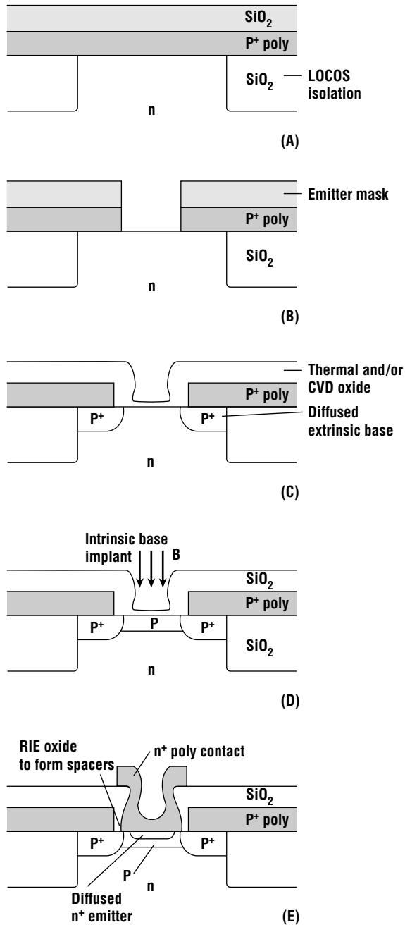
Figure 17.21 Simple process flow for a self-aligned double-poly bipolar technology.
