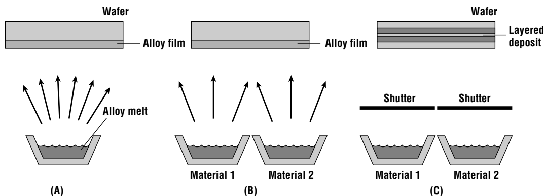
Figure 12.11 Methods for evaporating multicomponent films include (A) single-source evaporation, (B) multisource simultaneous evaporation, and (C) multisource sequential evaporation.
