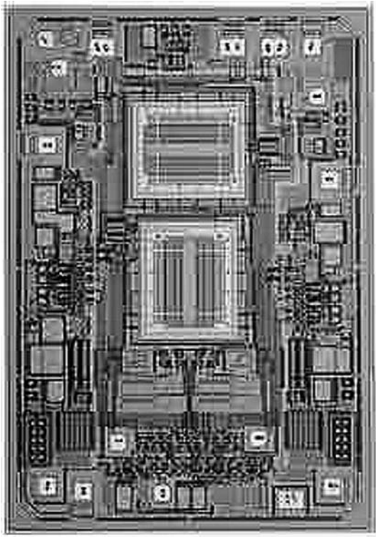
Figure 19.27 Photo of Analog Device's ADXL250 two-axis accelerometer chip. Acceleration measurement range of \pm 50\text{ g} , with resolution of 10 milli-g. The two MEMS devices are the large structures oriented 90^\circ to each other (photo courtesy of Analog Devices, Inc.).
