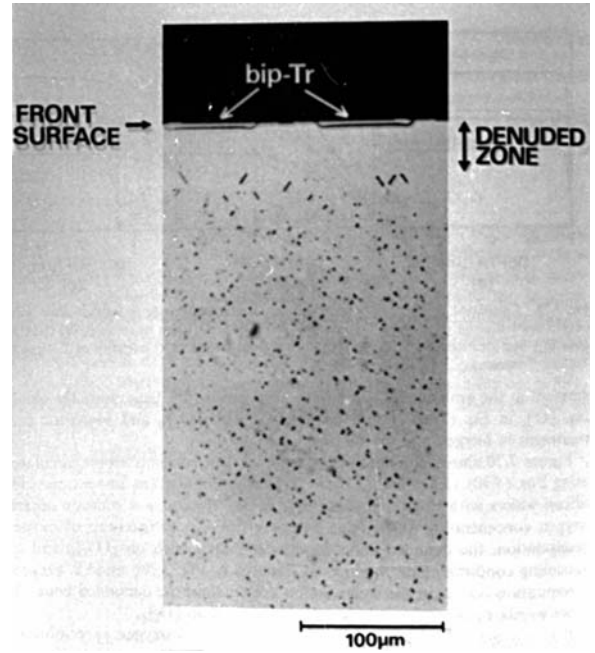
Figure 2.11 Cross-sectional view of denuded wafer with bipolar transistor (reprinted by permission, Academic Press, after Shimura).
