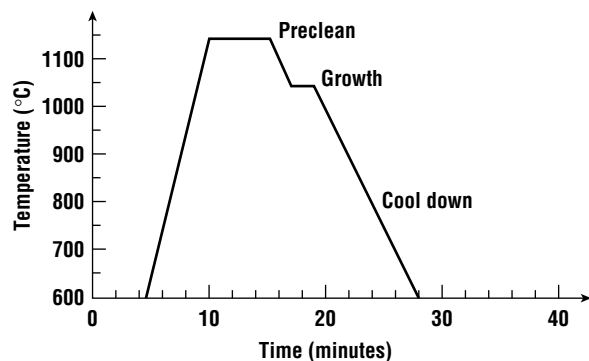
Figure 14.25 A typical time/temperature cycle for growing 1 \mu\text{m} of epitaxial silicon in a VPE reactor.
