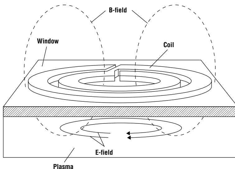
Figure 10.22 Schematic of ICP system showing the RF coil, the dielectric window, and the magnetic and electric fields (From Hopwood [13], reprinted with permission from Plasma Sources Science and Technology . Copyright 1992, IOP Publishing).
