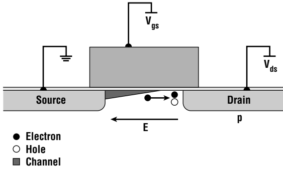
Figure 16.16 Impact ionization process in a MOSFET operated in pinchoff.
