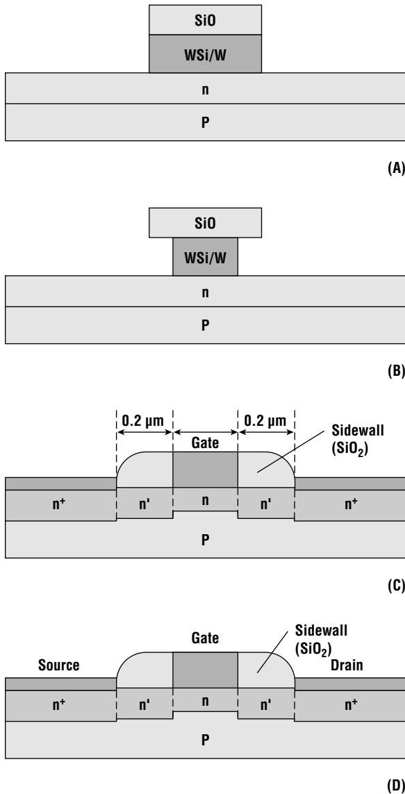
Figure 17.6 Process flow that employs both a buried p-layer and an LDD (after Shimura et al., ©1992 IEEE).
