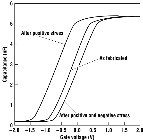
Figure 4.13 Typical C–V traces from temperature bias stress measurements of an oxide contaminated with a positive ion impurity.
