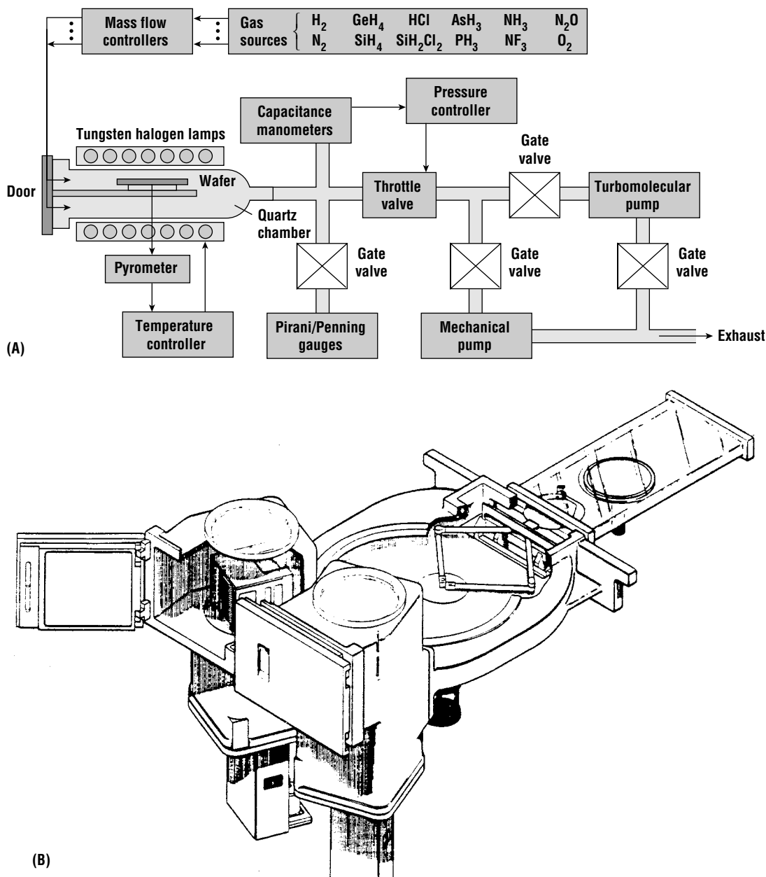
Figure 14.26 (A) Schematic of a rapid thermal epitaxial growth system (after Hsieh et al., reprinted by permission of the publisher, The Electrochemical Society). (B) Commercial rapid thermal epitaxial growth system showing load and unload stations, robot arm, and rapid thermal flow sleeve (courtesy of ASM Corp.).
