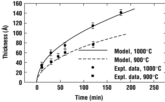
Figure 4.21 Growth of oxynitride in nitric oxide. Reprinted by permission from Journal of Applied Physics. Copyright 2003, American Institute of Physics.
