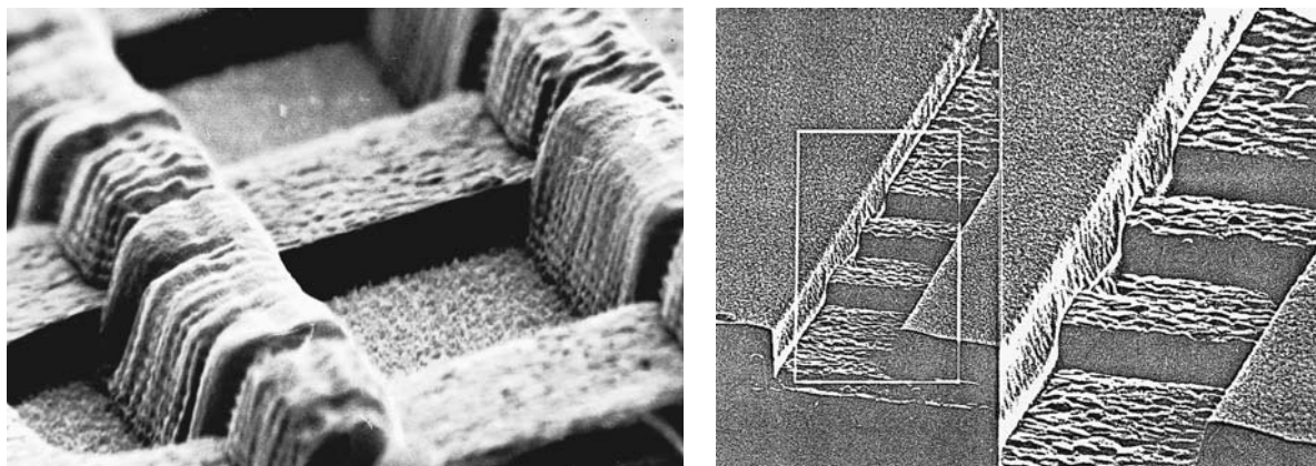
Figure 7.31 Micrographs of resist lines on reflective metal without and with a 2700-Å antireflecting layer under the resist (after Listvan et al.).
