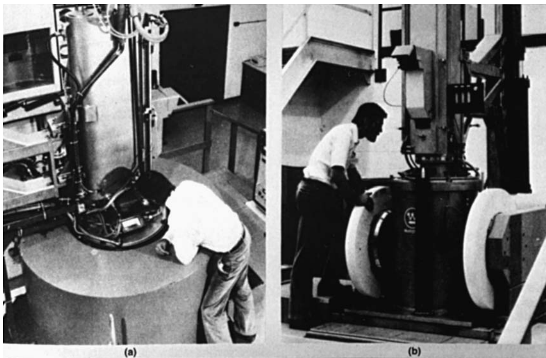
Figure 2.16 Photographs of a commercial magnetically confined Czochralski system ( Thomas et al. ).
