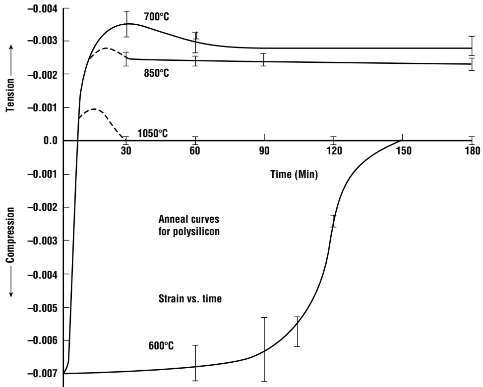
Figure 19.23 Change in strain level for low-stress polysilicon as a function of anneal temperature and time (after Guckel et al. [13], © 1988 IEEE).
