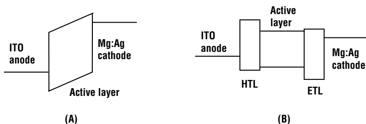
Figure 18.3 Band diagrams of (A) simple OLEDs and (B) OLEDs with electron transport layers (ETL) and hole transport layers (HTL).
