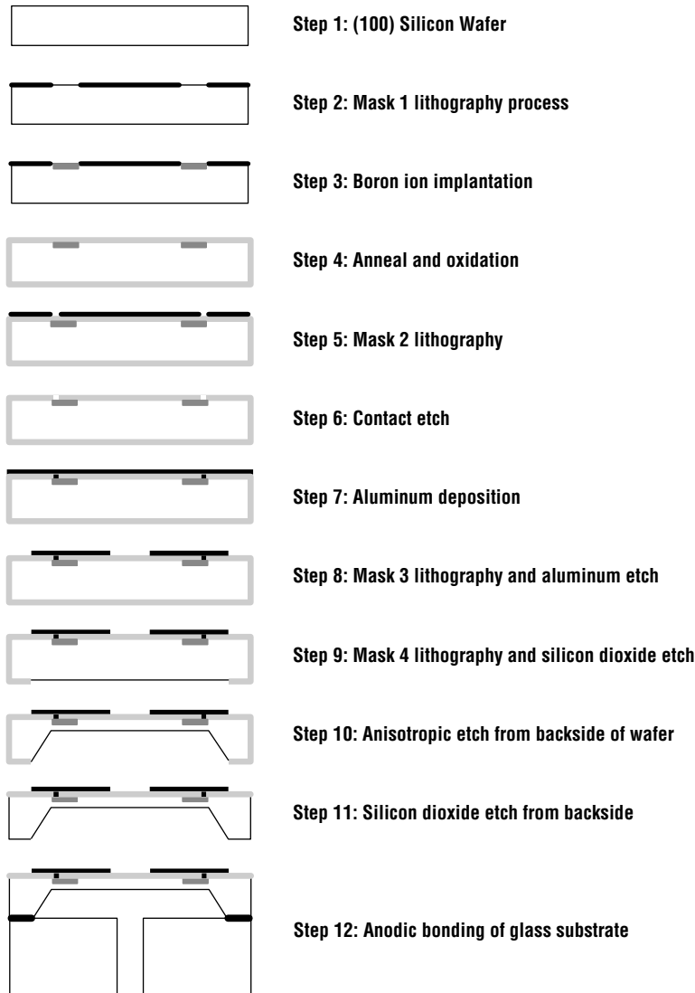
Figure 19.18 Bulk micromachining process for a piezoresistive pressure sensor.
