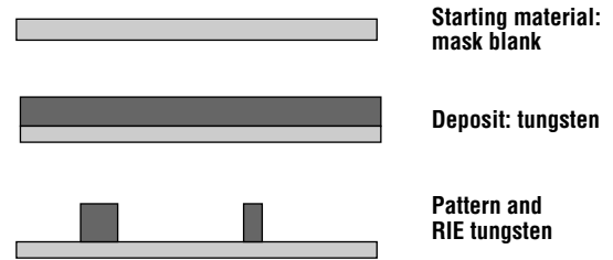
Figure 9.23 Subtractive process for x-ray mask fabrication.
