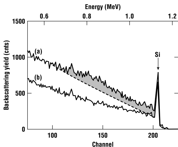
Figure 5.14 RBS spectra showing the backscattered He intensity as a function of energy. Curve (b) is an unimplanted wafer. The curve labeled (a) is a wafer after a 2 \times 10^{15} \text{ B} implant at 200 keV. The dashed line represents the component of the spectrum corresponding to the remaining crystalline silicon. The shaded area represents the contribution of displaced atoms ( reprinted by permission of Elsevier Science, after Schreutelkamp et al. ).
