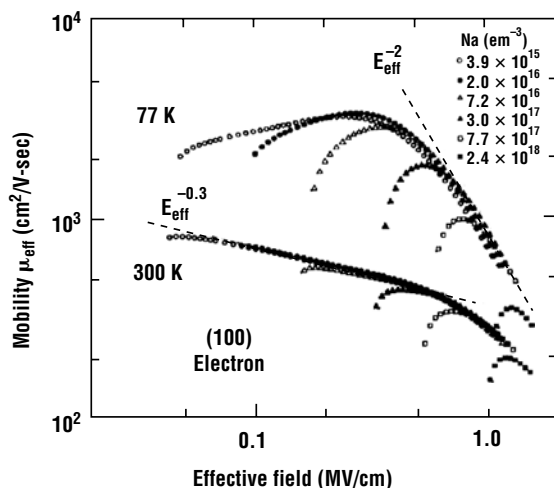
Figure 16.22 The universal curve for electrons at room temperature and at 77 K for electrons for various doping concentrations (Takagi et al., reprinted by permission of IEEE).
