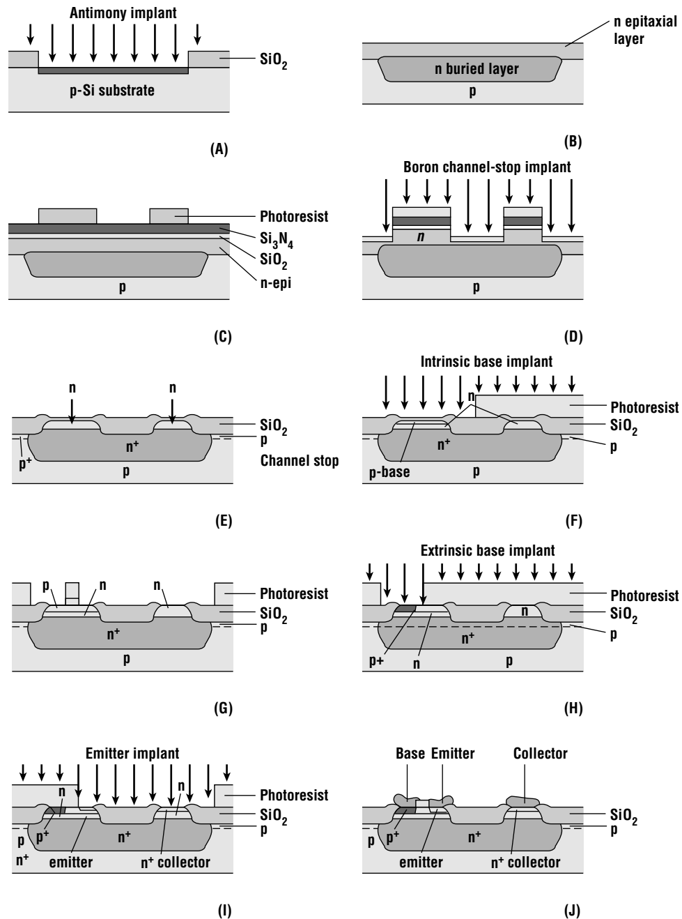
Figure 17.19 Process flow for an oxide-isolated, triple-diffused bipolar technology without sinks: (A) buried layer formation, (B) epitaxial growth, (C) LOCOS patterning, (D) silicon recessing and channel stop implants, (E) local oxidation, (F) intrinsic base implant, (G) contact mask, (H) extrinsic base implant, (I) emitter and collector contact implant, and (J) metallization (after Sze, reprinted by permission of John Wiley & Sons).
