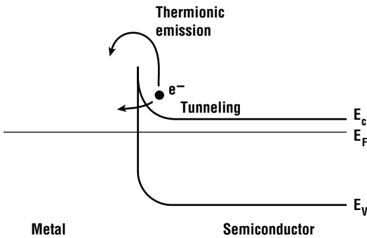
Figure 15.22 Two carrier transport mechanisms typically found in metal semiconductor contacts.
