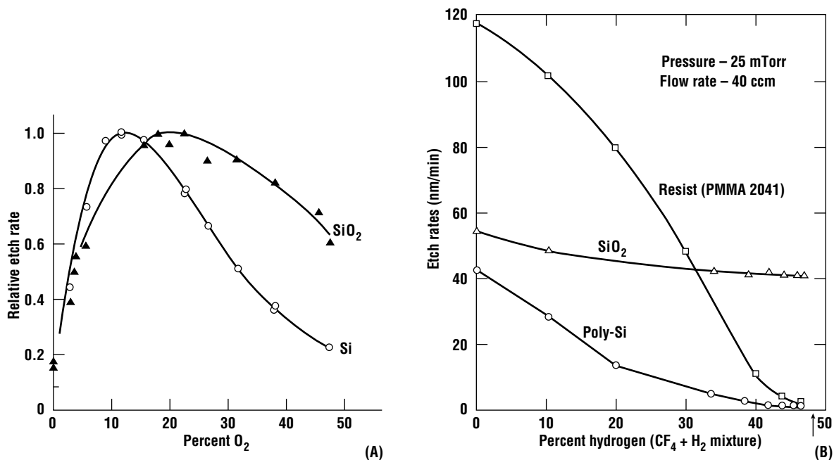
Figure 11.12 Etch rate of Si and \text{SiO}_2 in (A) \text{CF}_4/\text{O}_2 plasma (after Mogab et al. [59], reprinted by permission, AIP), and (B) \text{CF}_4/\text{H}_2 plasma (after Ephrath and Petrillo [100], reprinted by permission of the publisher, The Electrochemical Society Inc.).
