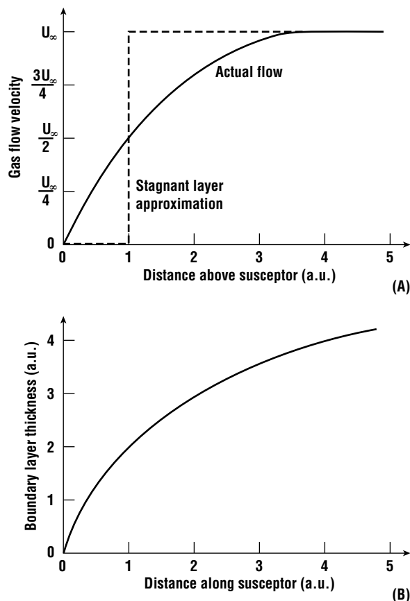
Figure 13.5 (A) Gas flow as predicted by a parabolic flow model and in the stagnant layer approximation. (B) Stagnant layer thickness versus position assuming a plug flow inlet.
