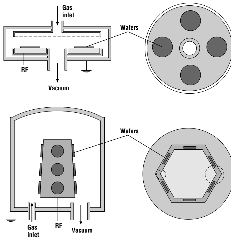
Figure 11.18 Top and side views of parallel-plate and hexode batch RIE systems. Typical conditions for either are 50 mtorr and 5 kW/m 2 . For larger wafers the exhaust in the upper figure is drawn from the periphery rather than the center.
