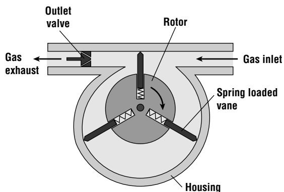
Figure 10.5 One of the most common types of pumps for microelectronic processing is the rotary vane vacuum pump.
