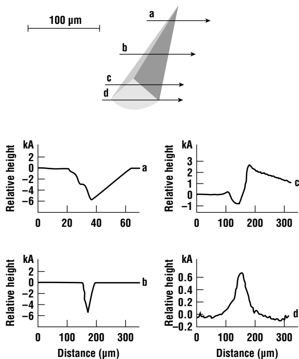
Figure 14.9 An electron micrograph of a stacking fault in an epitaxial layer grown on a (111) wafer. The lower plot shows mechanical scans of the surface topology at four sites on the fault (reprinted from Liaw and Rose by permission, Academic Press).
