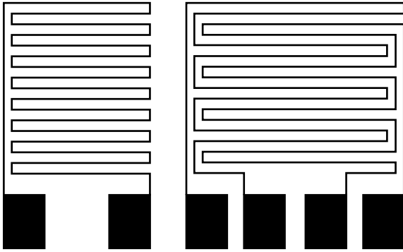
Figure 20.4 Meander lines and interdigitated comb structures used to determine a layer defect density.
