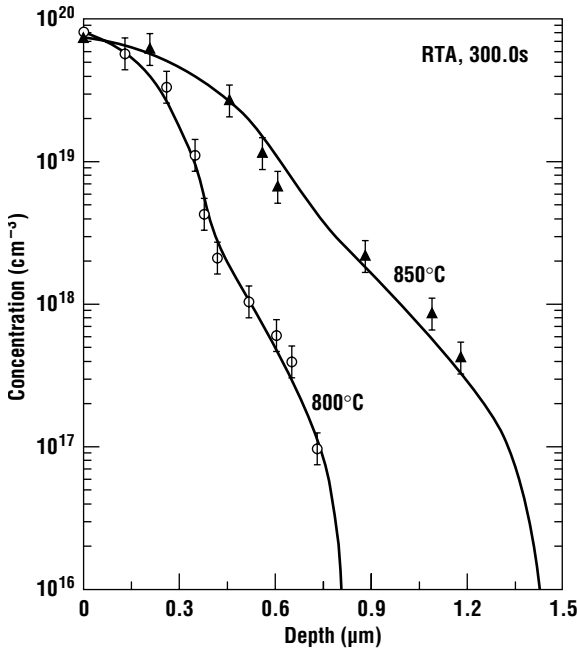
Figure 3.11 Comparison of the multiple charge model for zinc diffusion and experimental results (after Kahen, used with permission, Materials Research Society).
