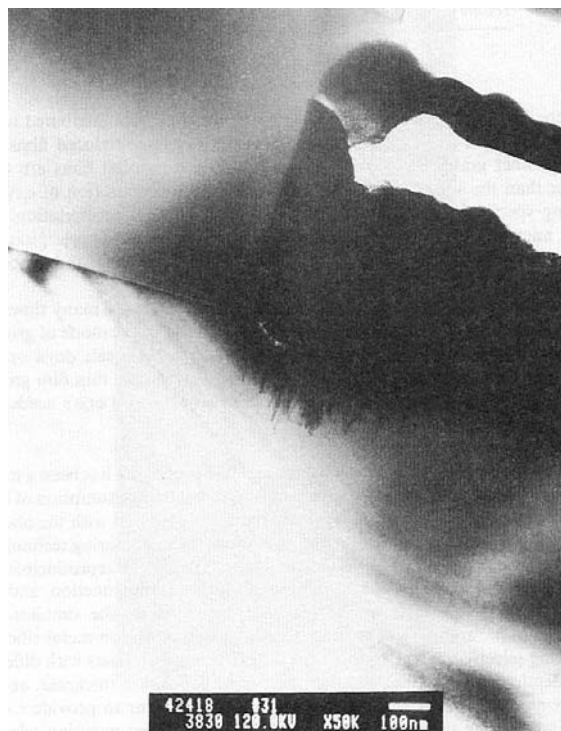
Figure 13.25 Damage to the substrate produced by selective tungsten.
