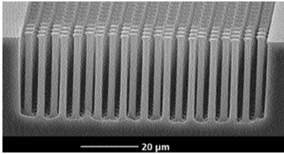
Figure 19.16 Example of structures formed using deep silicon etching with a high density plasma source (after Picraux and McWharther [40], © 1998 IEEE).
