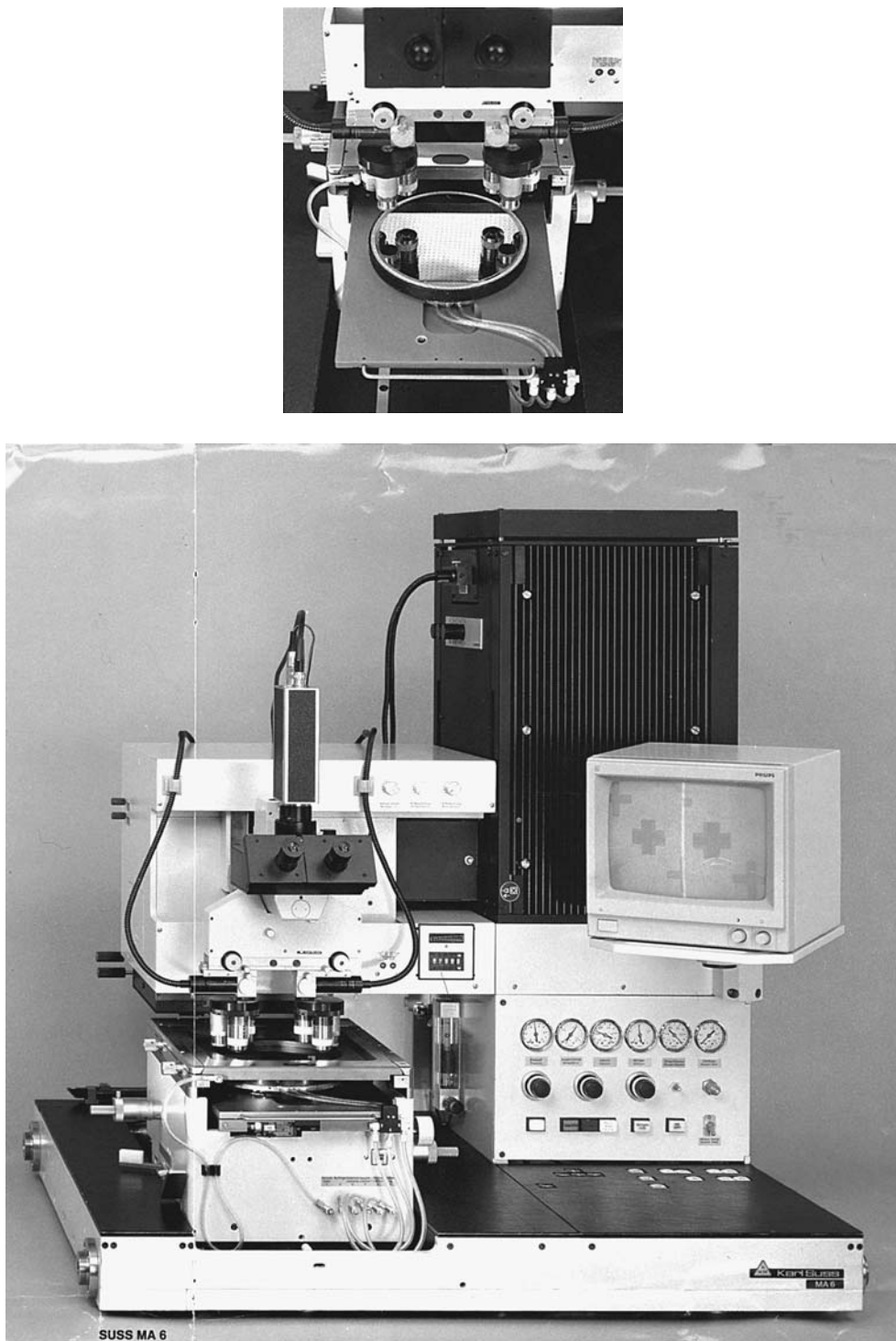
Figure 7.19 Typical contact exposure system ( courtesy of Karl Suss ).
