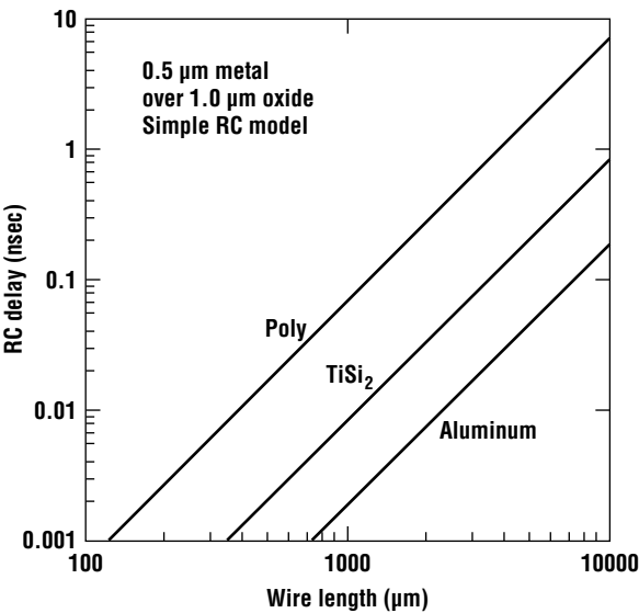
Figure 15.29 Simple lumped parameter model for the time constant of various interconnect materials.
