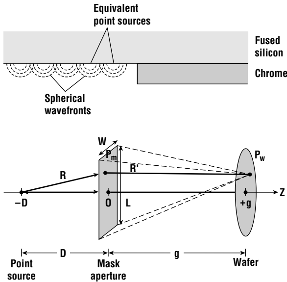
Figure 7.6 Huygens's principle applied to the optical system shown in Figure 7.5. A point source is used to expose an aperture in a dark field mask.
