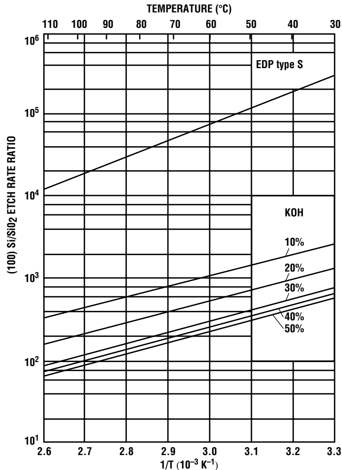
Figure 19.14 Etch rate ratio of (100) silicon to \text{SiO}_2 for EDP and KOH etch solutions (after Seidel [33], reproduced by permission of The Electrochemical Society, Inc.).
