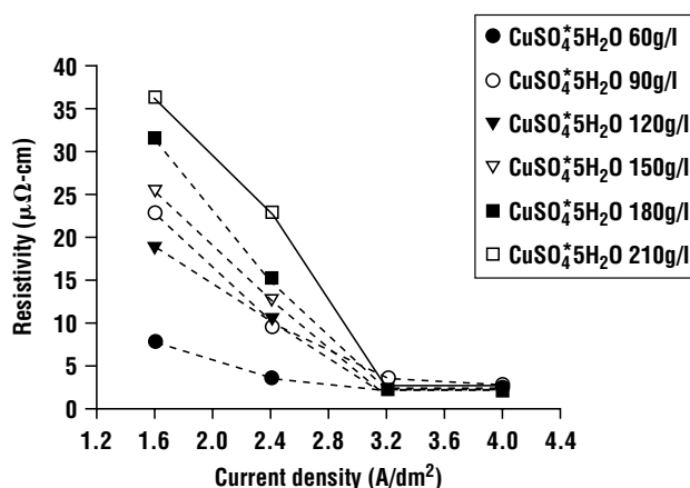
Figure 13.28 Copper resistivity as a function of the current density for various bath concentrations (After Gau, et al., reprinted with permission from Journal of Vacuum Science and Technology . Copyright 2000 IOP Publishing).
