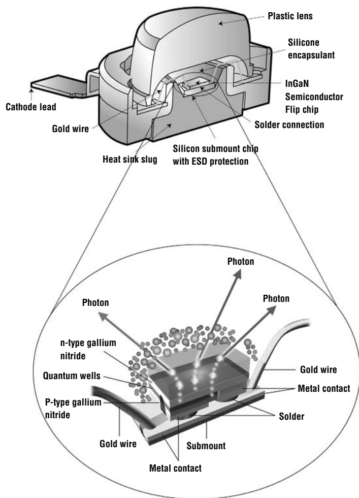
Figure 18.2 Cross section view of a LUXEON power LED. The active device is mounted upside down in the package. Considerable care is taken in heat sinking and encapsulation to allow high power density (used by permission, Philips Lumileds Lighting Company).
