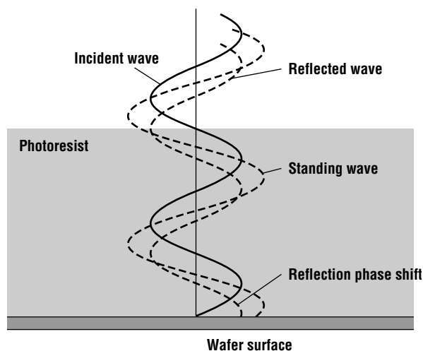
Figure 7.32 The formation of standing waves in the resist.
