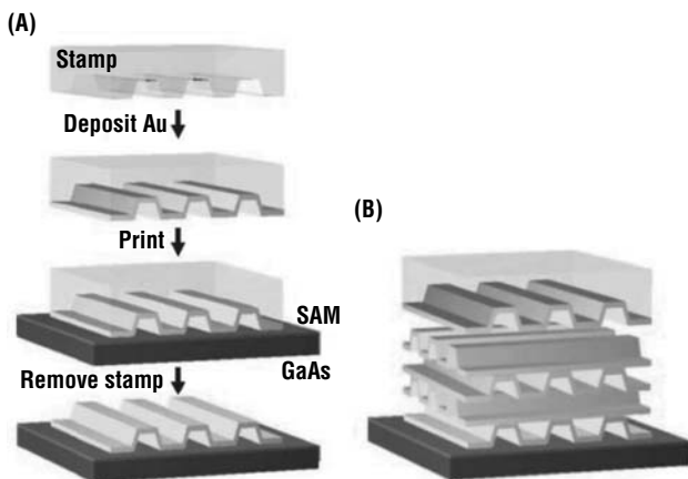
Figure 9.31 Schematic of a 3D micromolding process using a gold layer to form fluid flow channels ( reprinted with permission from Nanoletters, from Ref. 92. ) Copyright 2003, American Chemical Society.
