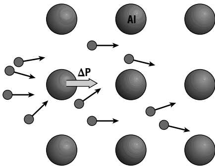
Figure 15.30 Momentum transfer between electrons and matrix atoms in an interconnect material.
