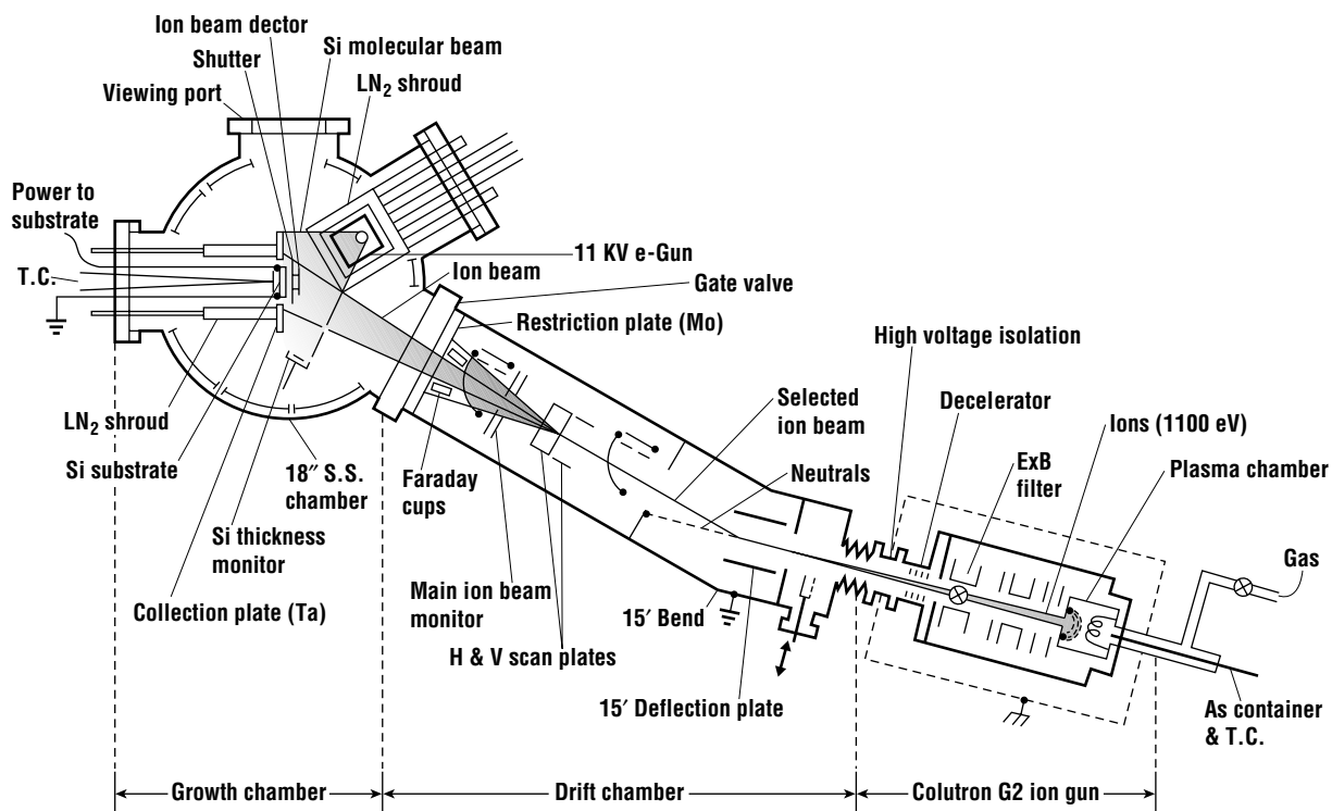
Figure 14.34 An ion implantation system for introducing impurities during silicon MBE (after Fujiwara et al. [90]).
