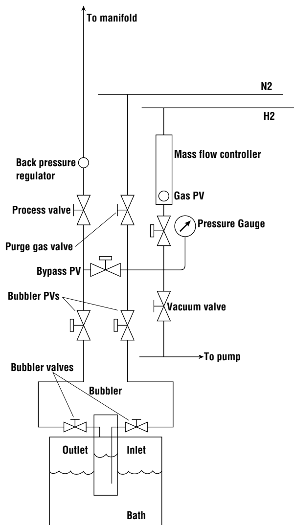
Figure 14.20 A typical OM source for MOCVD includes valves that isolate and bypass the bubbler during changeout, allowing cycle purging of the process line with nitrogen.
