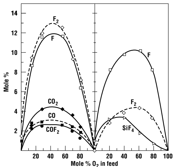
Figure 11.10 Species concentration in a \text{CF}_4 plasma as a function of the amount of oxygen in the feed gas (after Smolinsky and Flamm, reprinted by permission, AIP).
