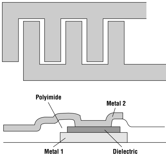
Figure 17.8 Interdigitated and simple overlay capacitor.
