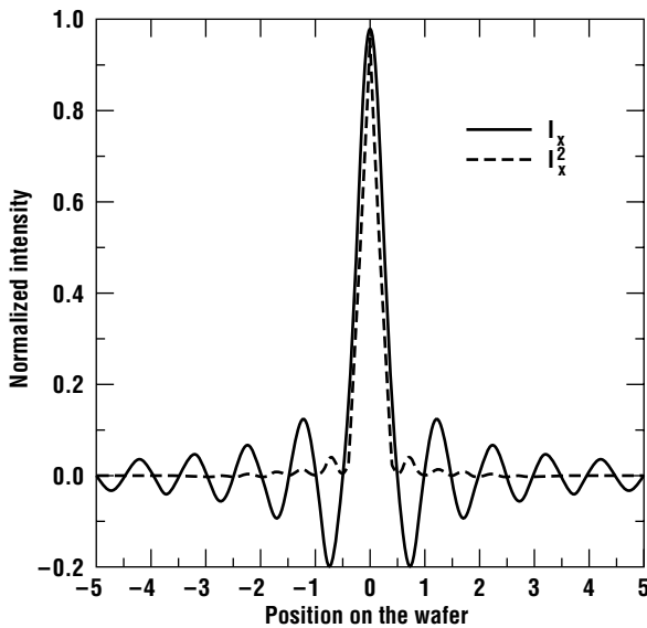
Figure 7.8 Typical far field (Fraunhofer) image.
