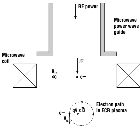
Figure 10.21 In an ECR plasma, an alternating field causes the electrons to move in circular orbits, dramatically increasing the ion density.
