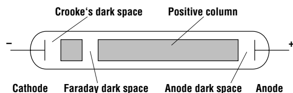
Figure 10.16 Structure of a dc plasma.
