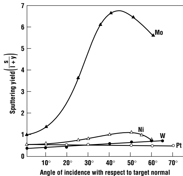
Figure 12.16 Typical angular dependence of the sputter yield for several different materials. The sputter profiles follow a cosine distribution (after Wehner, reprinted by permission, AIP).
