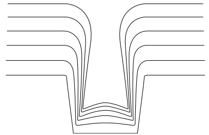
Figure 12.22 Cross section of the time evolution of the typical step coverage for unheated sputter deposition in a high aspect ratio contact.
