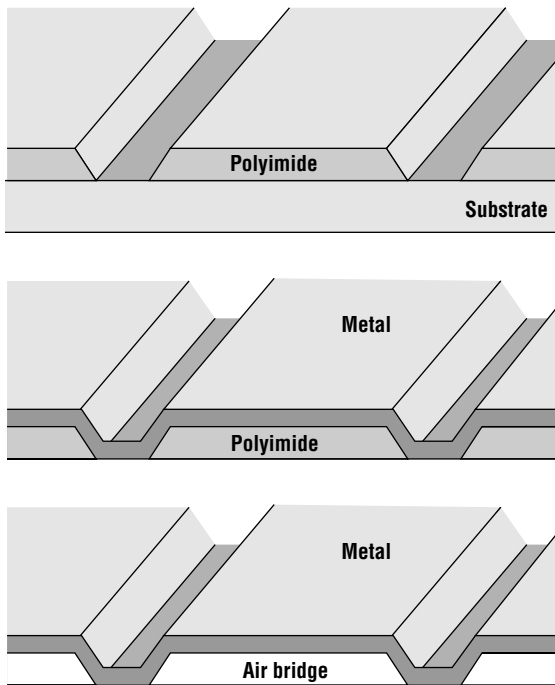
Figure 17.9 Air bridge process flow.
