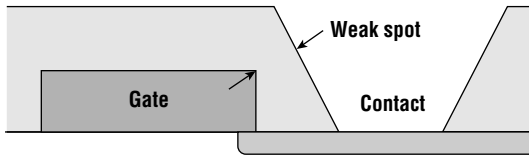
Figure 16.13 Gate to source/drain shorts caused by misalignment and/or contact blowout during etch.
