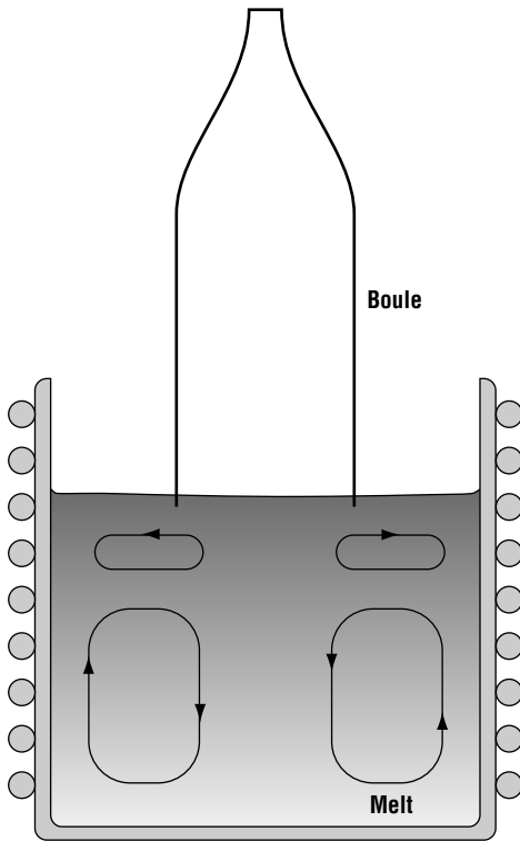
Figure 2.17 Idealized schematization of the formation of recirculation cells in a melt.
