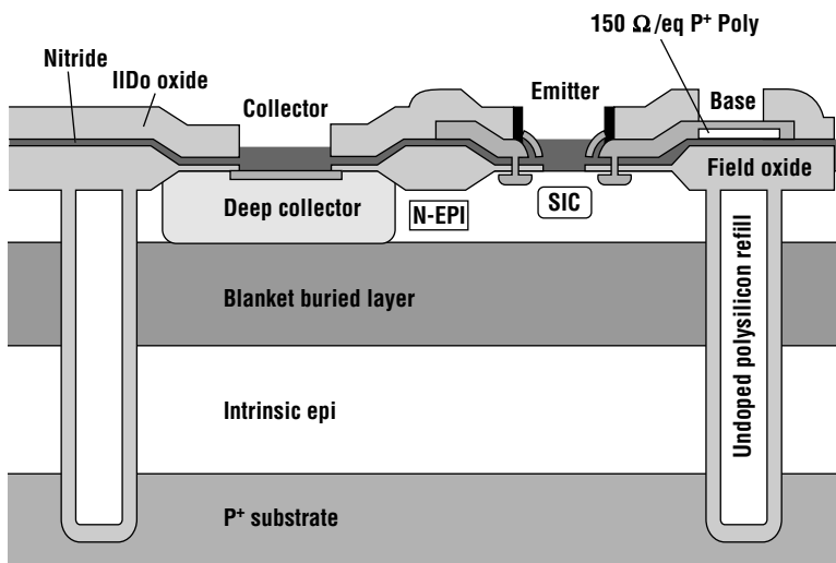
Figure 17.22 A cross section of a self-aligned bipolar technology called Mosaic (after de la Torre et al., ©1991 IEEE).
