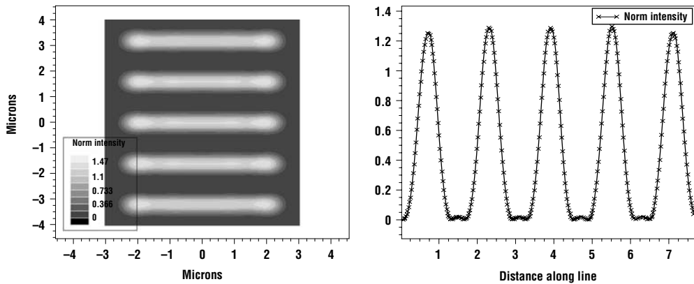
Figure 7.11 Contour plot (left) and 1-D slice through the center of projected intensity as a function of position for a grating with 1.6 μm pitch, exposed at R = 436 nm and NA = 0.43 .
