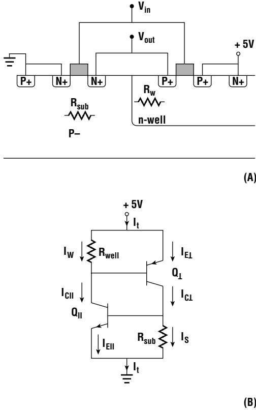
Figure 16.18 (A) Cross section of an n-well CMOS inverter with parasitic elements superimposed. (B) Equivalent circuit.
