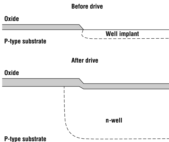
Figure 16.4 Cross-sectional views of an inverter structure before and after well drive.
