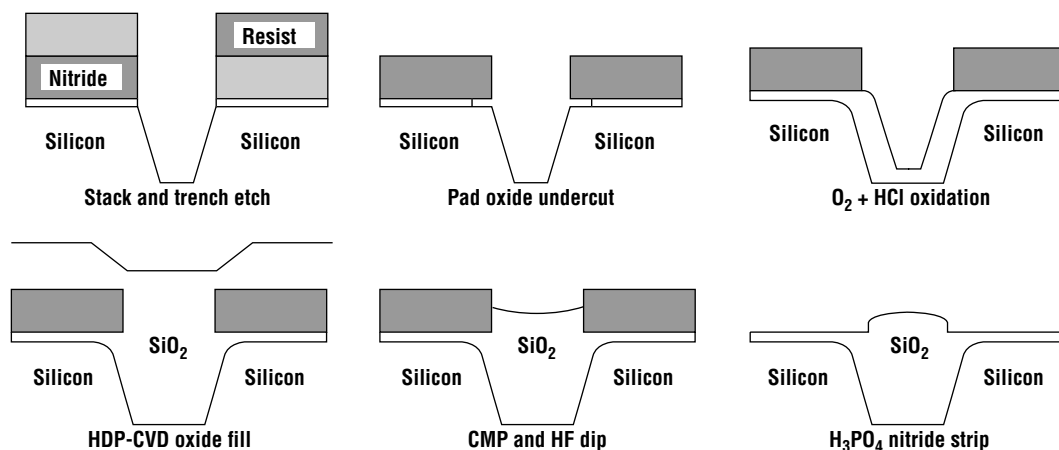
Figure 15.12 Schematic of a shallow trench isolation module (after Chatterjee et al., used with permission, APS, 1997).
