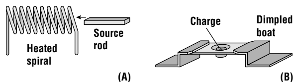
Figure 12.7 Resistive evaporator sources. (A) Simple sources including heating the charge itself and using a coil of refractory metal heater coil and a charge rod. (B) More standard thermal sources including a dimpled boat in resistive media.
