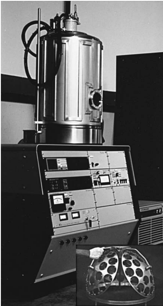
Figure 12.10 A commercial evaporator. Inset shows a planetary (photographs courtesy of CHA Industries).
