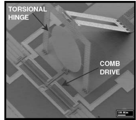
Figure 19.30 SEM photograph of a fast mirror used in a raster scanner. The mirror scans the beam in a direction parallel to the substrate (after Hagelin [60], reprinted with permission, SPIE).
