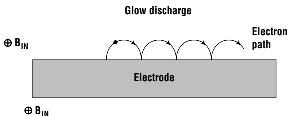
Figure 10.20 In a simple magnetically confined plasma, electrons ejected from the cathode are confined by the Lorentz force to stay in the cathode dark space.
