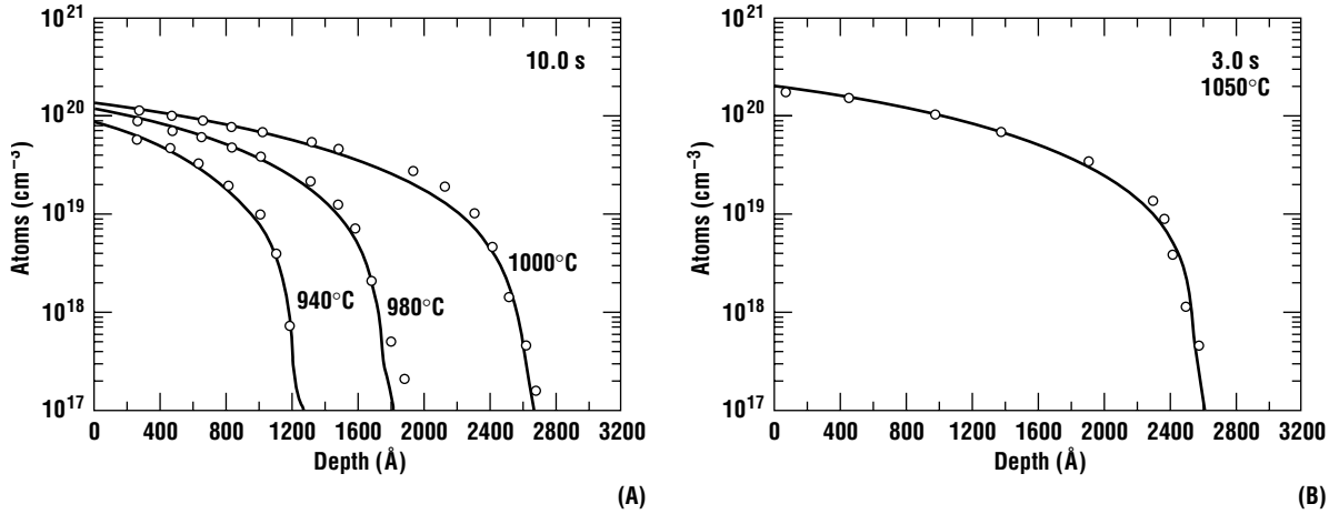
Figure 3.12 Diffusion of silicon in GaAs (after Kahen et al., used with permission, Materials Research Society).
