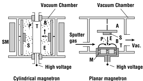
Figure 12.17 Planar and cylindrical magnetron sputtering systems T: target; P: plasma; SM: solenoid; M: magnet; E: electric field; B: magnetic field (after Wasa and Hayakawa, reprinted by permission, Noyes Publications).
