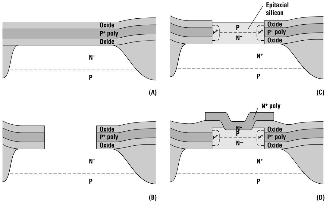
Figure 17.25 The sidewall contacted (SICOS) structure provides the least parasitic base–collector capacitance but is difficult to manufacture.
