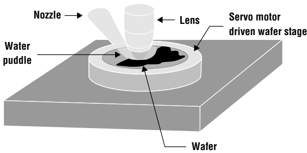
Figure 7.24 Setup of an immersion system using surface tension (from Switkes et al. , reprinted from the May 2003 edition of Microlithography World . Copyright 2003 by PennWell.)
