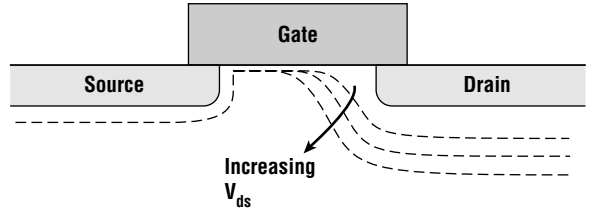
Figure 16.11 Schematic of device cross section showing enlarged depletion regions that give rise to short-channel behavior.
