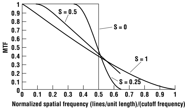
Figure 7.22 Modulation transfer function as a function of the normalized spatial frequency for a projection lithography system with spatial coherence as a parameter.
