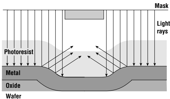
Figure 7.29 Light from the exposed regions can be reflected by wafer topology and be absorbed in the resist in nominally unexposed regions.
