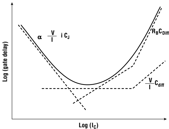
Figure 17.16 Log/log plot of ECL gate delay versus the collector current.
