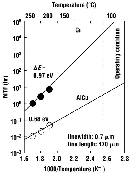
Figure 15.36 Median time to failure of Cu and AlCu lines (from Sun, reprinted with permission IEEE).
