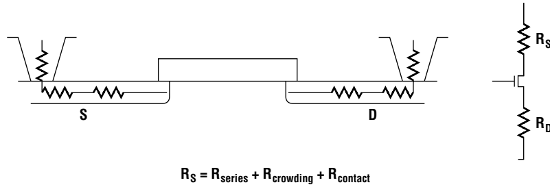
Figure 16.12 Equivalent circuit for MOSFET with source/drain series resistances displayed.
