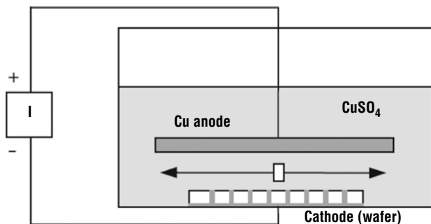
Figure 13.26 Basic electroplating setup.
