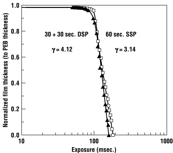
Figure 8.10 Contrast curves for Megaposit SPR500 resist using MF CD-26 developer (courtesy Shipley).
