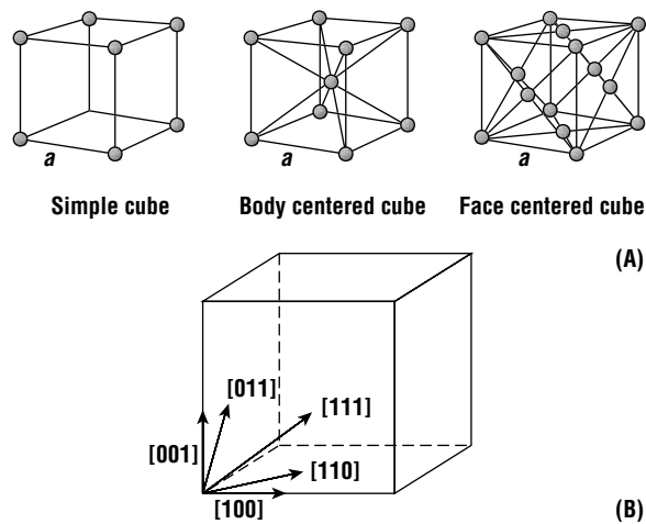
Figure 2.5 (A) Common cubic crystals: simple cubic, body-centered cubic, and face-centered cubic. Lattice sites are indicated by the small circles. (B) Crystal orientations in the cubic system.
