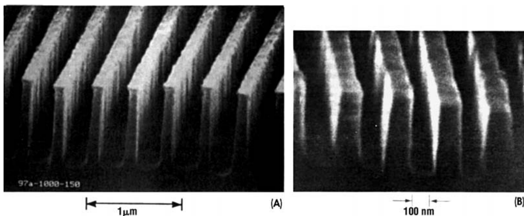
Figure 8.17 Imaging of (A) 0.2 \mu\text{m} and (B) 0.15 \mu\text{m} lines in a 300-Å poly( n -butylsilylne) resist over a novolac resin (after Kunz et al. , used by permission, SPIE).
