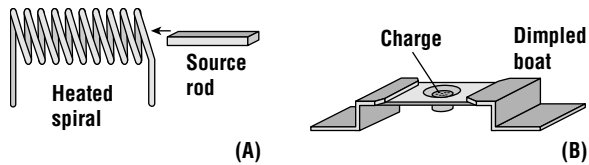
Figure 12.7 Resistive evaporator sources. (A) Simple sources including heating the charge itself and using a coil of refractory metal heater coil and a charge rod. (B) More standard thermal sources including a dimpled boat in resistive media.
