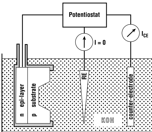
Figure 19.15 Generic electrochemical etch stop setup.
