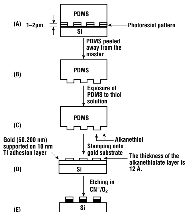
Figure 9.30 Schematic description for the \mu cp fabrication of Au patterns using an elastomer called PDMS (Sylgard 184, Corning): (A) PDMS stamp fabrication, (B) PDMS detach from the master, (C) exposure to the alkanethiol ink, (D) contacting with Au substrate, and (E) etching Au on the substrate ( reprinted with permission from Applied Physics Letters, from Ref. 88. ) Copyright 2002, American Institute of Physics.
