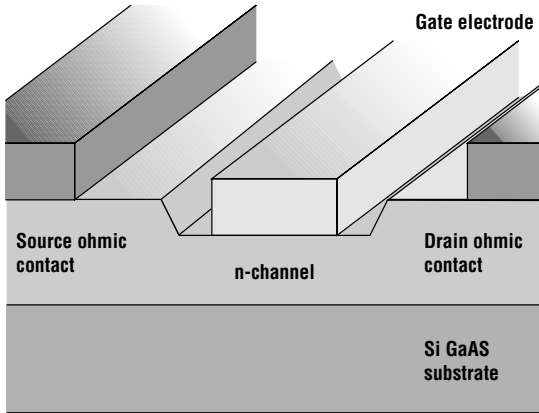
Figure 17.1 Cross section of a simple mesa-isolated MESFET.
