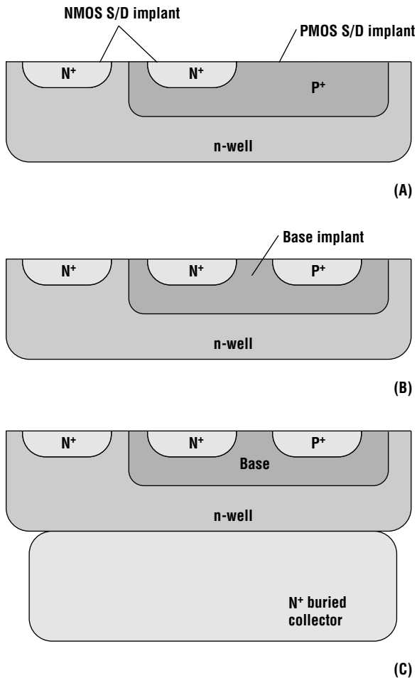
Figure 17.30 Diffused bipolar transistors that can be fabricated in a CMOS technology: (A) the emitter and base are formed by the N^+ and P^+ source/drain diffusions, respectively, while the n -well serves as a collector, (B) a separate intrinsic base implant is done to set the BJT gain, and (C) a buried layer is added beneath the n -well.
