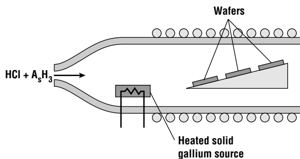
Figure 14.13 A halide transport system for growing GaAs epitaxially. Gaseous gallium chlorides are created in the chamber and are transported to the wafer surface.
