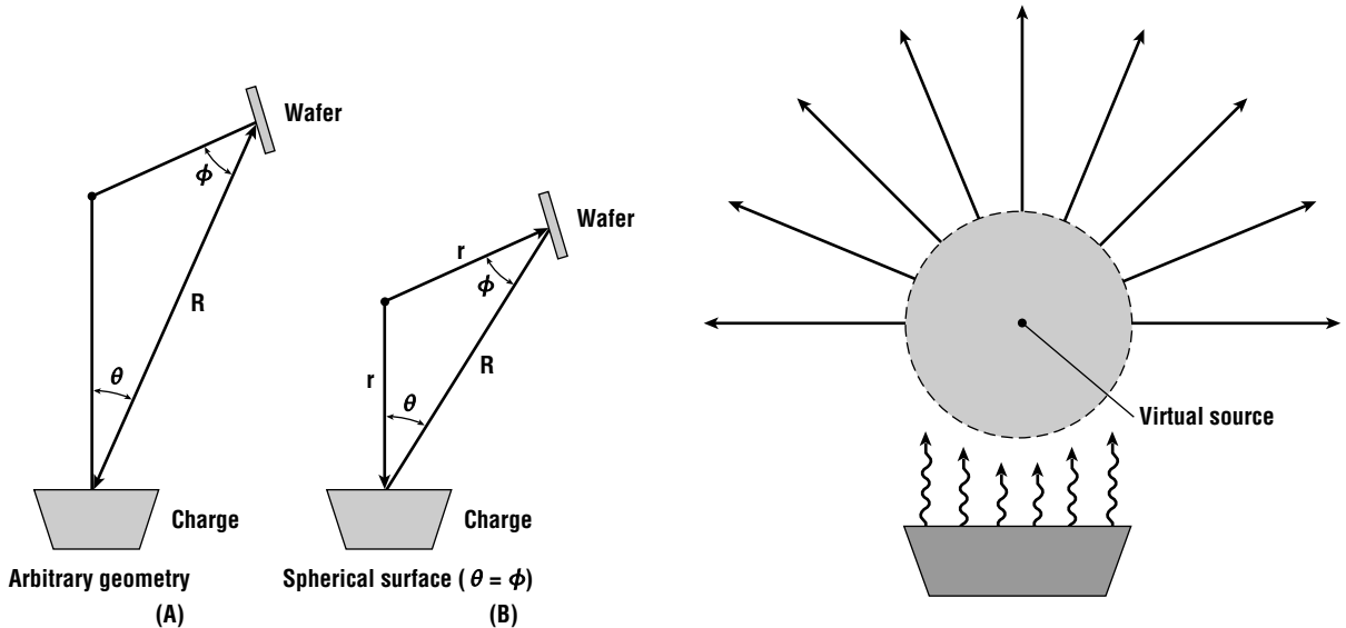
Figure 12.4 At high deposition rates, the equilibrium vapor pressure of the charge puts the region just above the crucible into viscous flow, creating a virtual source up to 10 cm above the top of the crucible.
