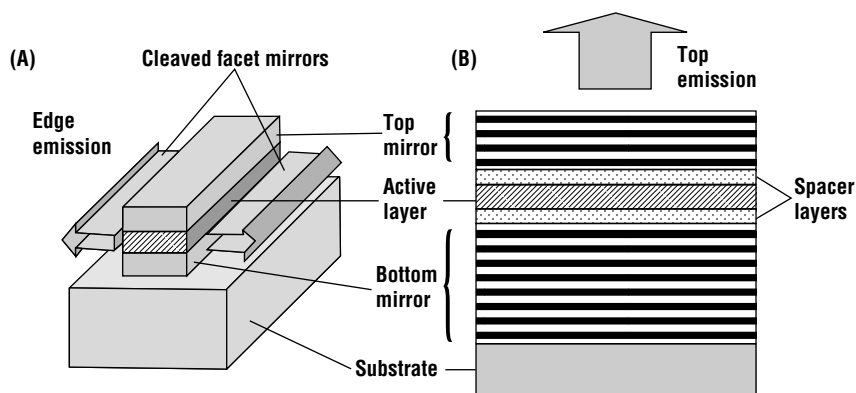
Figure 18.4 (A) Edge-emitting and (B) VCSEL laser structures.
