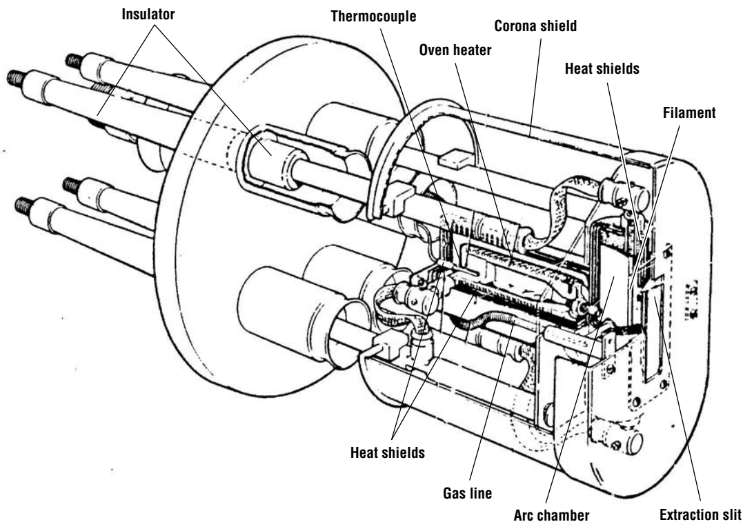
Figure 5.2 Schematic for a Freeman ion source. Solids can be vaporized in the oven heater, while gaseous sources may be injected directly into the arc chamber, newer system's use a Bernas ion source ( reprinted by permission, Elsevier Science, after Freeman in Mayer et al. ).
