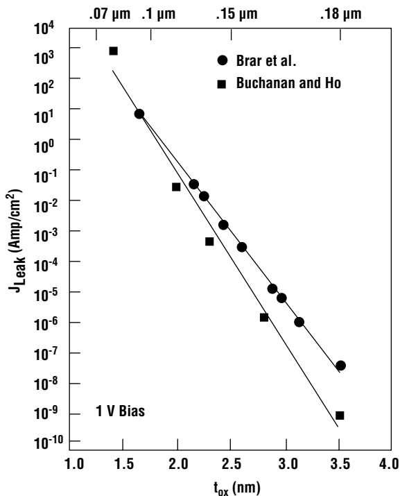
Figure 4.22 Measured leakage current at 1 V supply for different physical oxide thicknesses.
