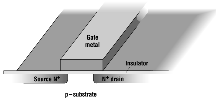
Figure 1.6 Cross section of an MOS transistor showing gate, source, drain, and substrate electrodes. The “+” and “−” indicate very heavy and very light dopings, respectively.
