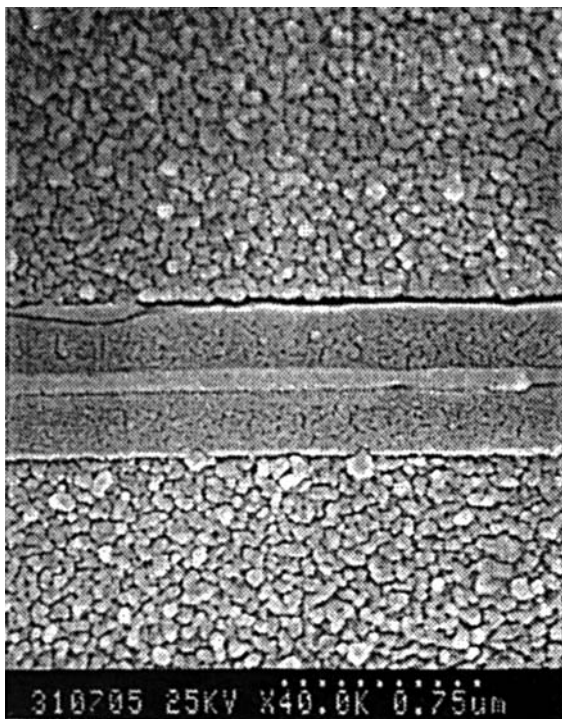
Figure 15.14 Wafer bonding method for achieving silicon on insulator (after Quenzer and Benecke, reprinted with permission, Elsevier Sequoia S.A.).
