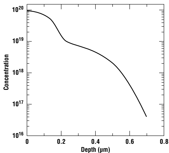
Figure 3.9 Typical profile for a high concentration phosphorus diffusion.
