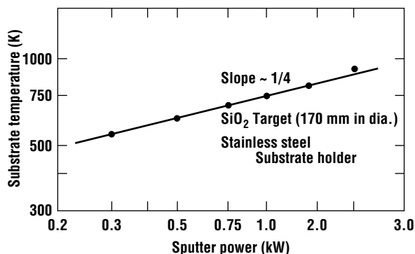
Figure 12.23 The temperature rise of substrates as a function of the plasma power for an argon RF plasma with an \text{SiO}_2 target (after Wasa and Hayakawa, reprinted by permission, Noyes Publications).
