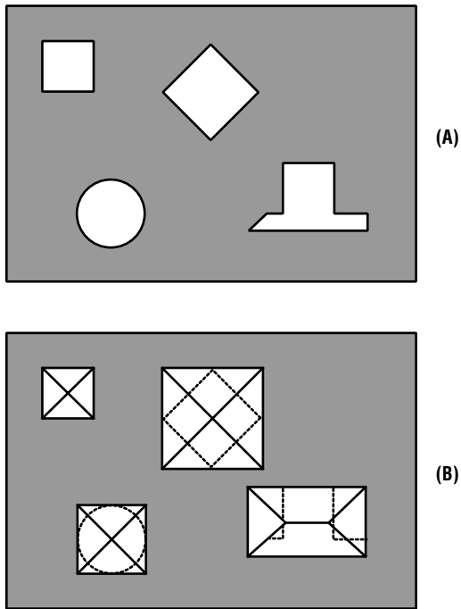
Figure 19.11 Effect of mask opening orientation on the etch profile. (A) Top view of mask openings as oriented to the \langle 110 \rangle direction. (B) Etched structures resulting for an anisotropic etchant on (100) silicon.
