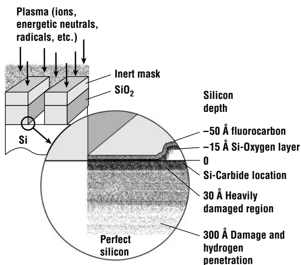
Figure 11.21 A cross section schematic of the results of a typical etch of SiO 2 down to Si using CF 4 /H 2 (after Oehrlein, Rembetski, and Payne, reprinted by permission, AIP).
