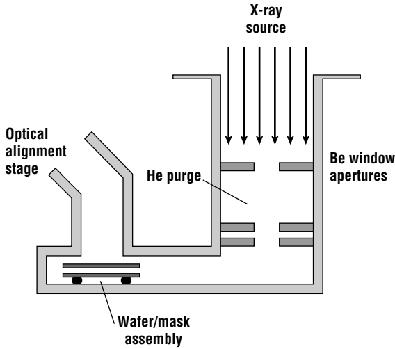
Figure 9.18 Simple proximity x-ray lithography aligner. The basic system is very similar to optical proximity systems.
