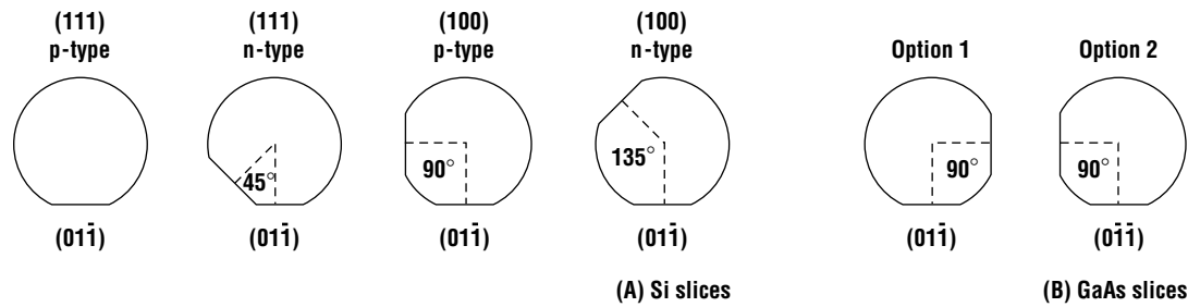
Figure 2.23 Standard flat orientations for different semiconductor wafers.
