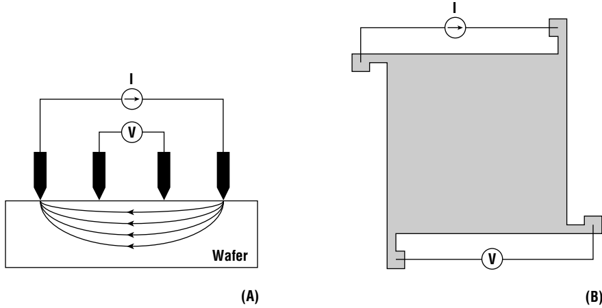
Figure 3.13 The four-point probe (A) and Van der Pauw (B) methods for determining the resistivity of a sample.
