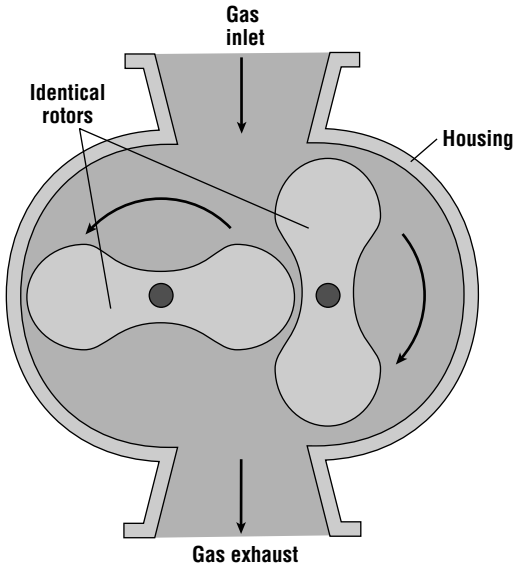
Figure 10.7 Schematic diagram of a Roots blower.
