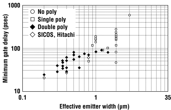
Figure 17.26 Ring oscillator gate delay of various bipolar technologies as a function of the emitter stripe width ( After Zbedel, used by permission, IEEE ).
