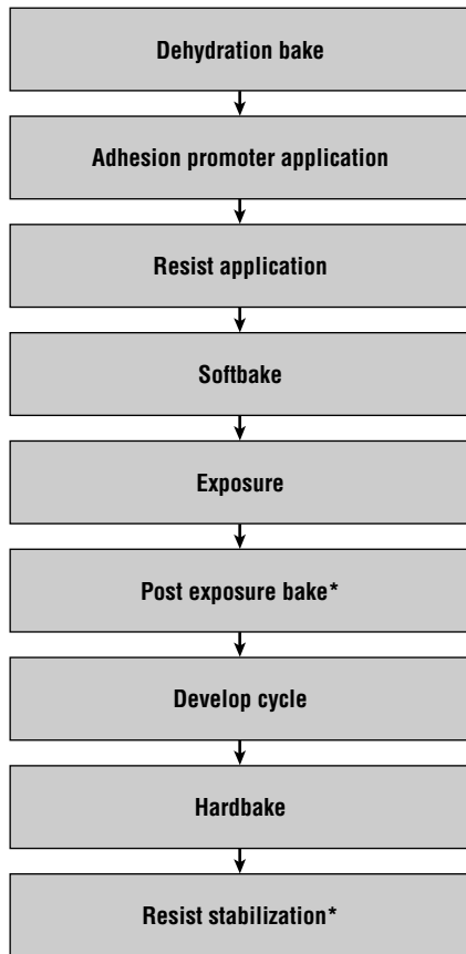
Figure 8.9 Typical process flow in a photolithography step.
