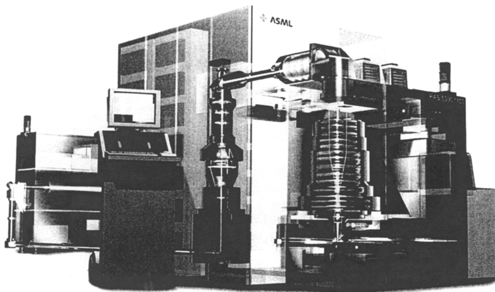
Figure 7.26 Configuration of Step-and-Scan 193-nm system. The laser is at the left. The reticle is at the upper right, while the wafer is at the lower right ( photo courtesy ASML ).
