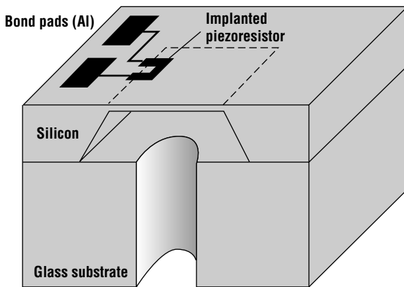
Figure 19.17 Simplified drawing of a typical piezoresistive bulk micromachined silicon pressure sensor (after Kovacs [14], reprinted with permission, The McGraw-Hill Companies).
