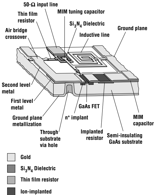
Figure 17.7 Cross-sectional view of a typical MMIC (after Decker).
